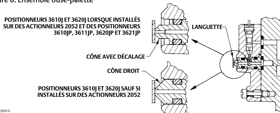
Figure 8. Ensemble buse-palette
