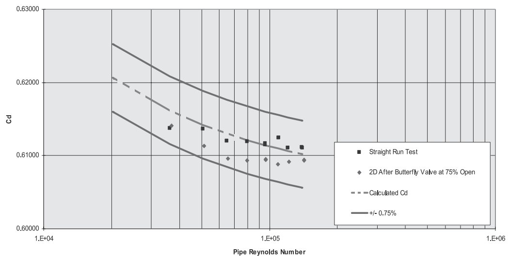
Figure 3-26: Test results for sensor 12402 in water
