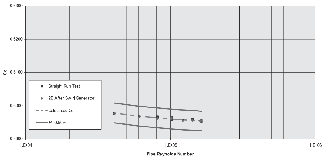
Figure 3-23: Test results for sensor AT24261 in water
