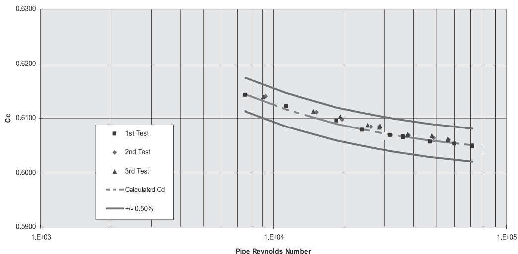
Figure 3-4: Sensor 08261 test results
