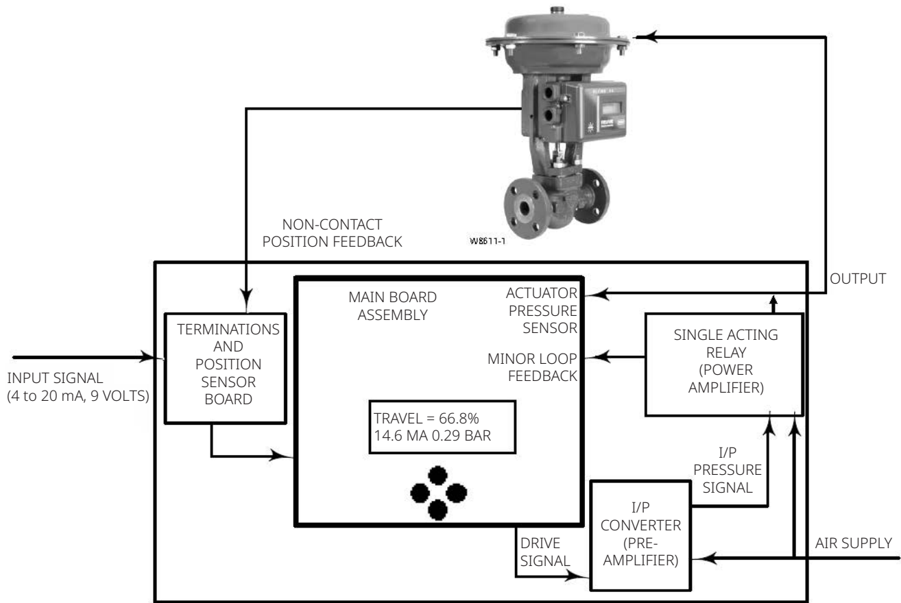
Figure 3. Block Diagram
