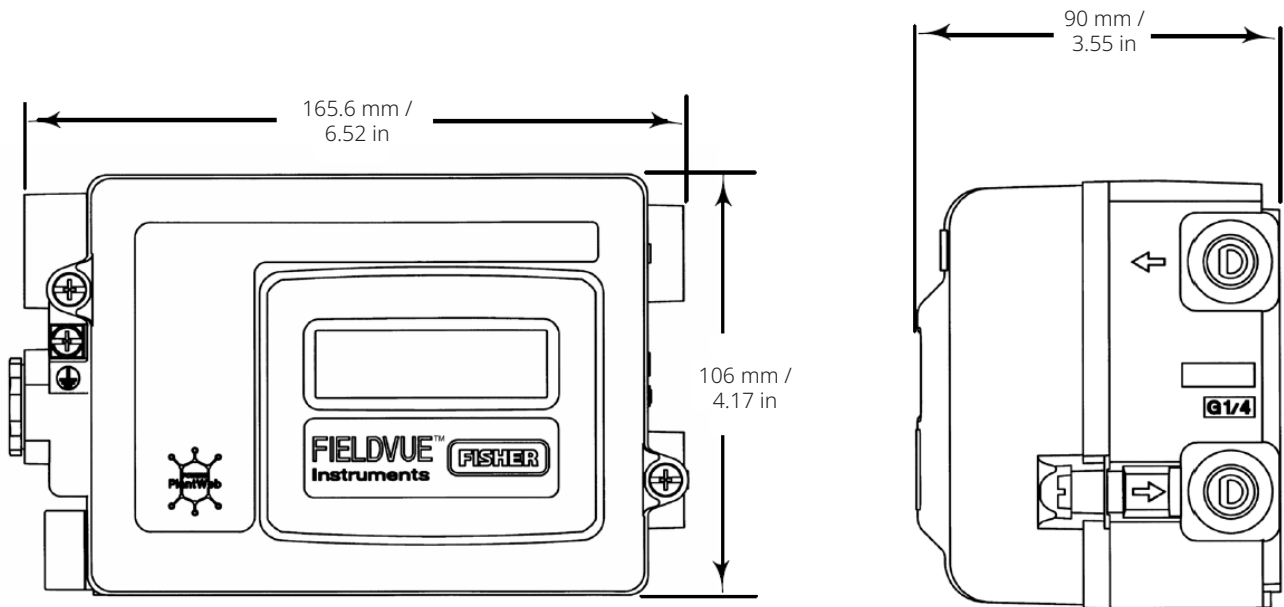
Figure 4. Dimensions
