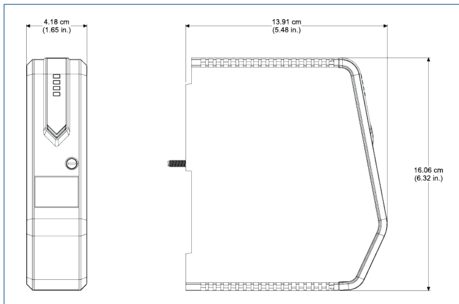
DeltaV MX controller hardware dimensions.
