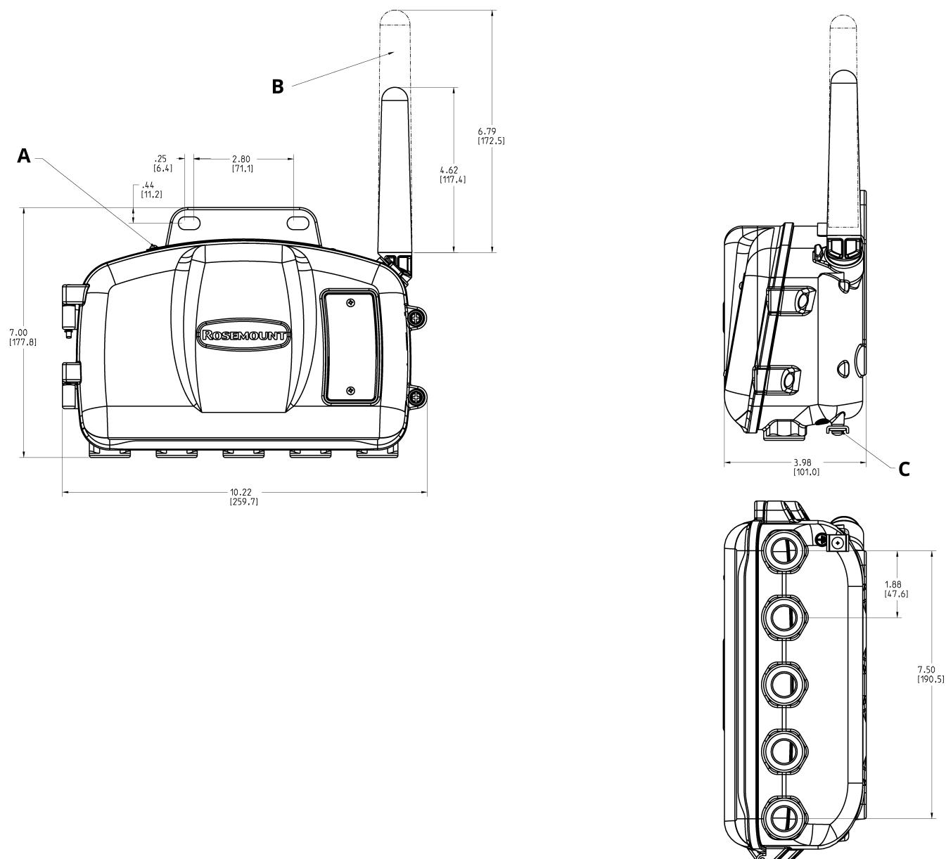
Figure 3: Rosemount 802 Wireless Multi Discrete I/O Transmitter
