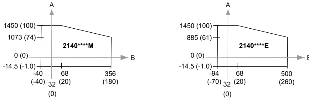
Figure 4: Operating Pressures
