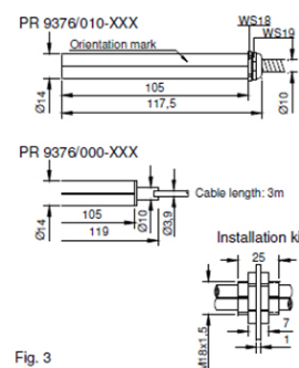
Fig. 3 Dimensions All dimensions in mm
