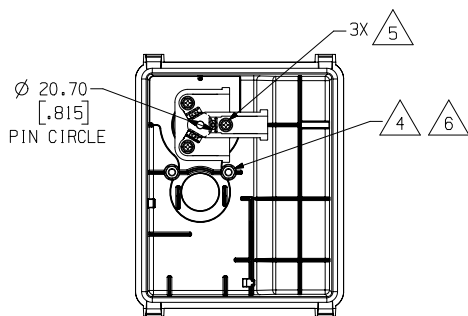
TERMINAL BOX LAYOUT STANDARD SCALE 1:2
