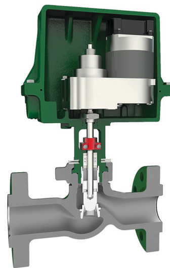
Cutaway of Fisher easy-Drive electric actuator
