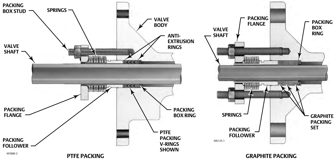
Figure 4. Optional ENVIRO-SEAL Packing Arrangements
