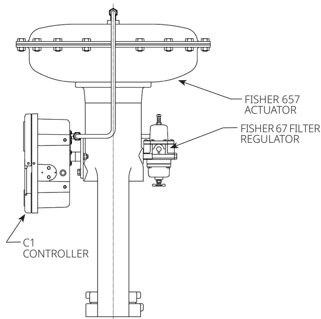
Figure 9. Typical Yoke Mounting
