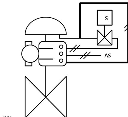
Figure 4. Solenoid Valve Testing
