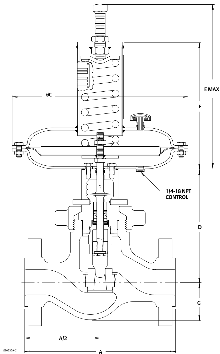
Figure 3. Fisher D4 Valve Dimensions, Spring-To-Close (also see tables 12 and 13)
