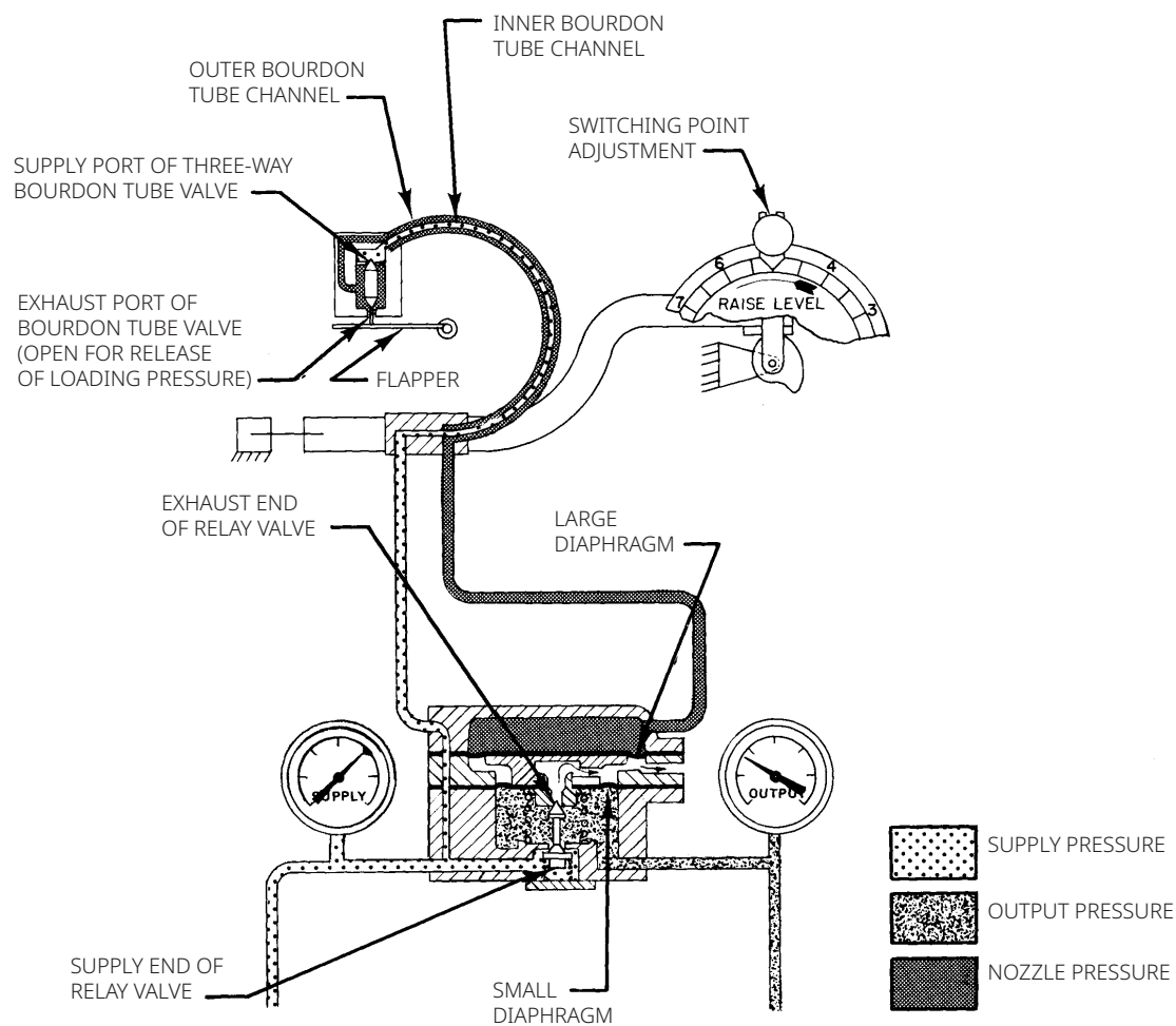
Figure 7. Schematic of Reverse-Acting Fisher 2503R Controller
