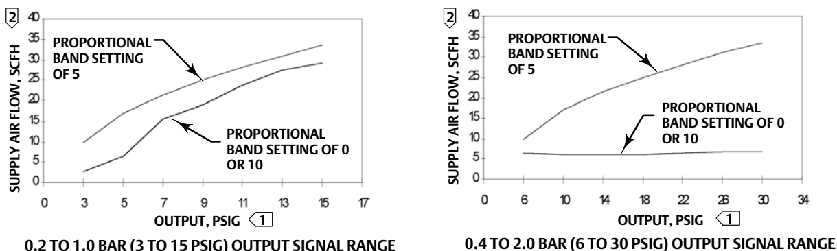
Figure 1. Steady-State Air Consumption
