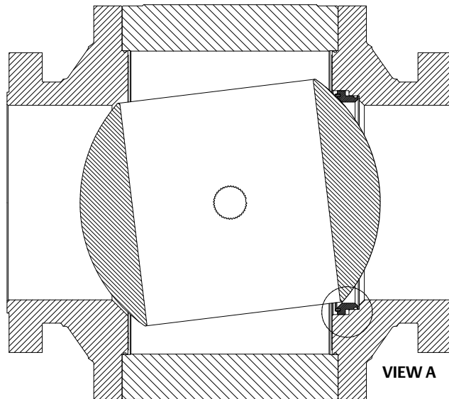
Figure 7. Dead Angle (also see table 4)
