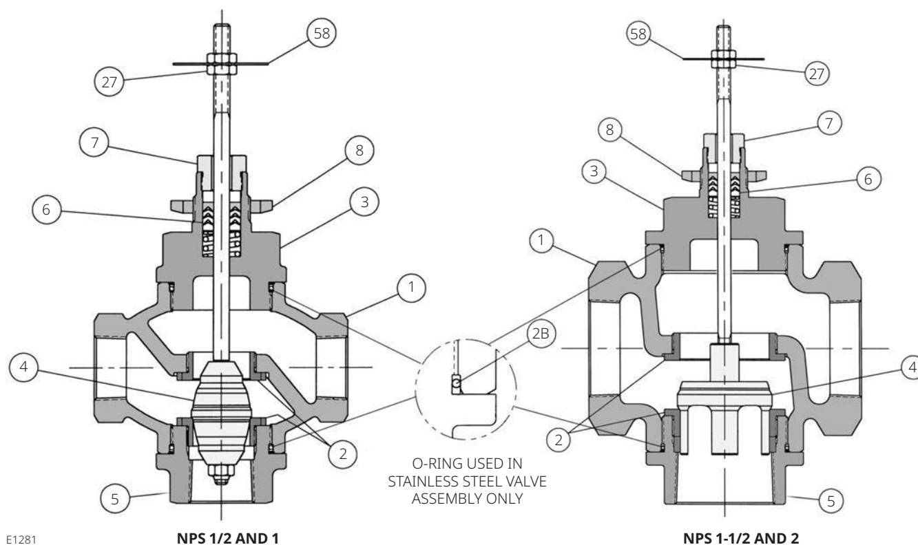
Figure 1. 24003 Valve Body with Standard Bonnet and NPS 1 Integral Seat
