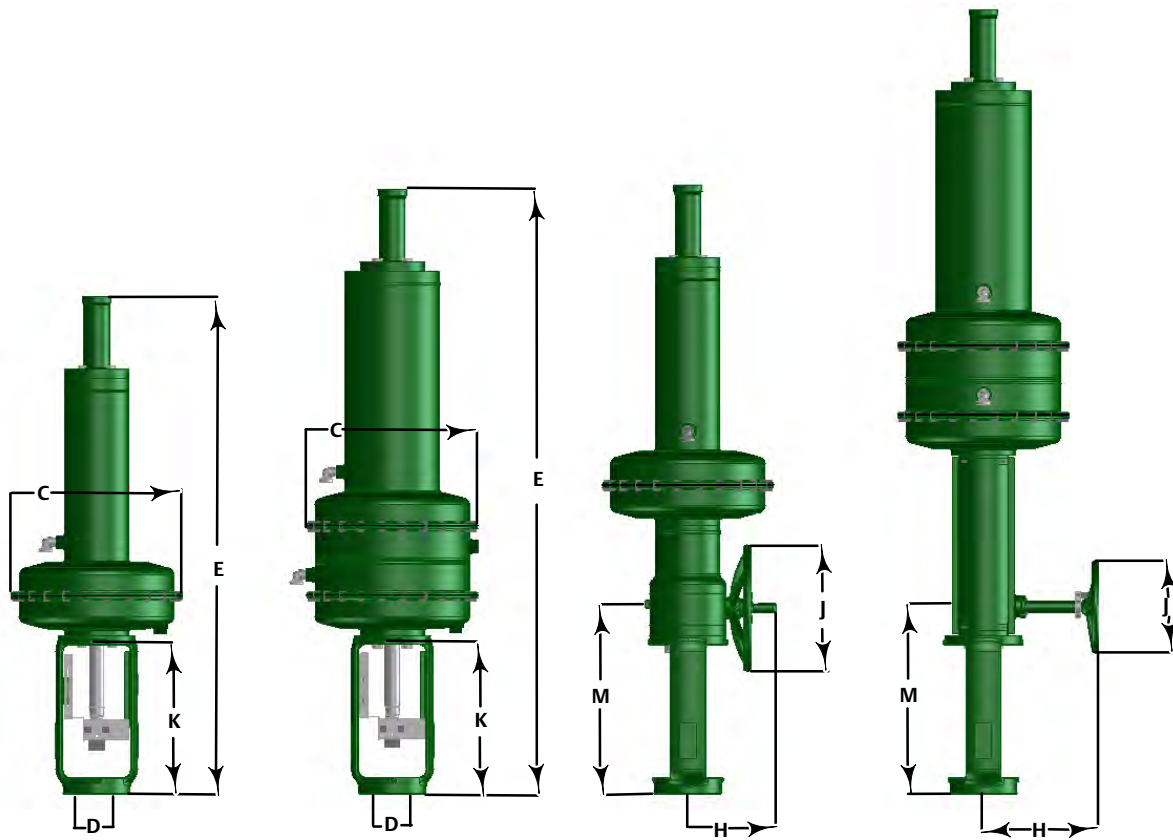
Figure 5. Dimensions (See Table 7)
