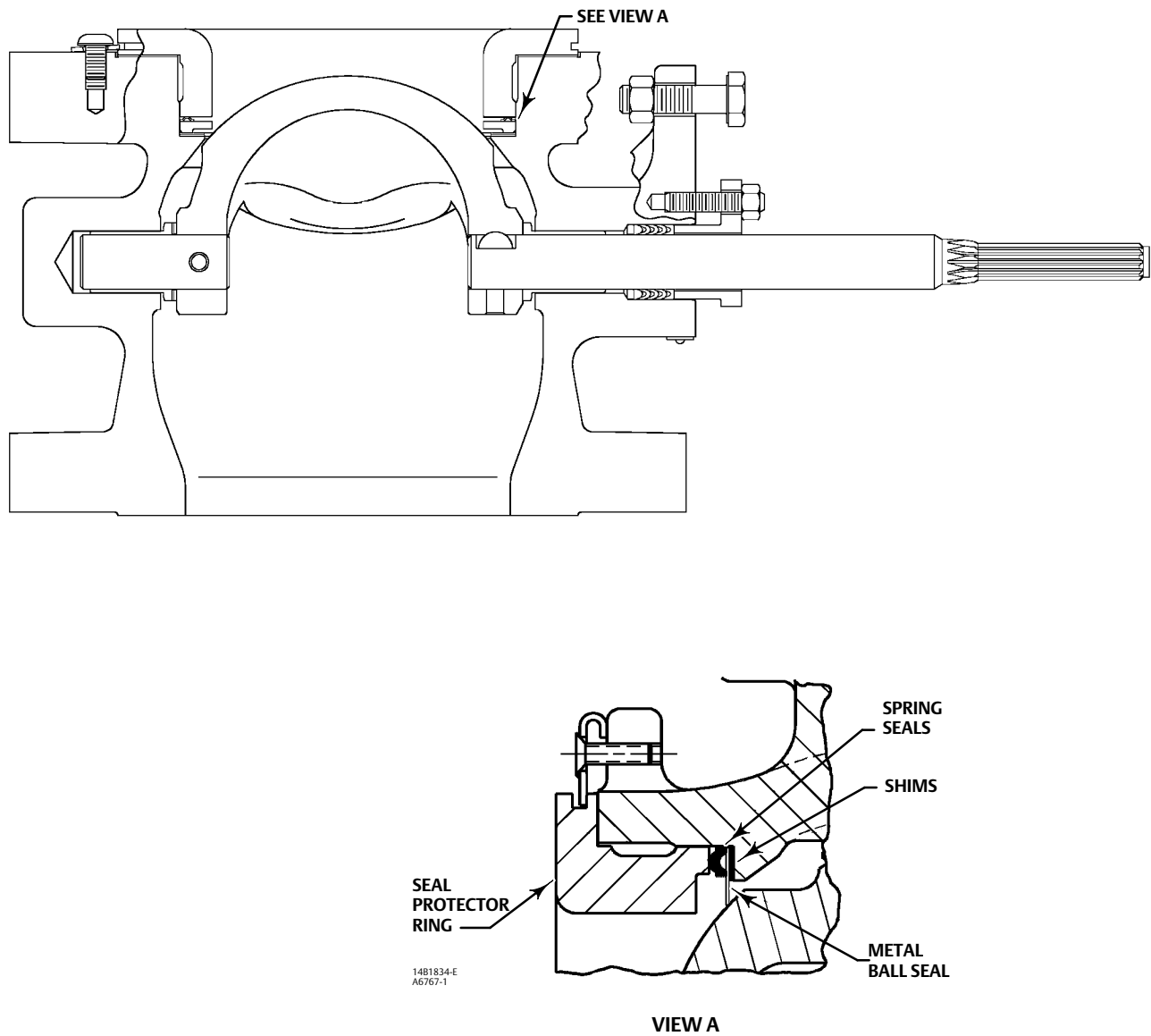
Figure 1. Fisher SS-252B Construction Features
