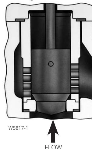
Figure 14. Fisher HPS Trim with Micro-Form Valve Plug
