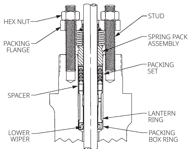
Figure 11. KALREZ with Vespel CR-6100 Packing
