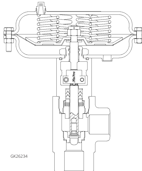
AIR-TO-CLOSE
