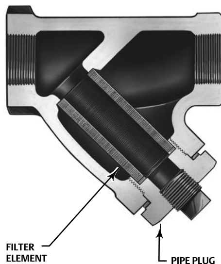
Figure 1. Construction Details
