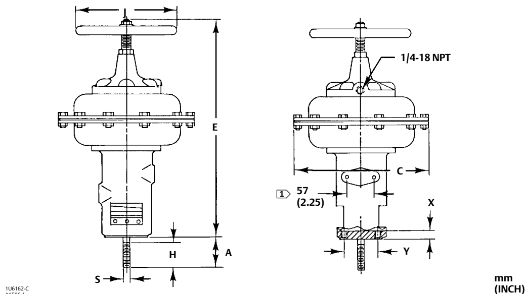
Figure 1. Dimensions (also see table 3)
