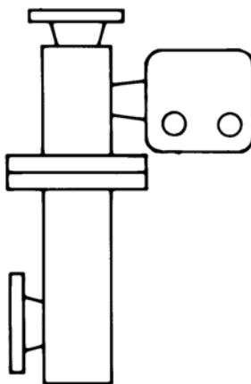
Figure 10. Cage Connection Styles
