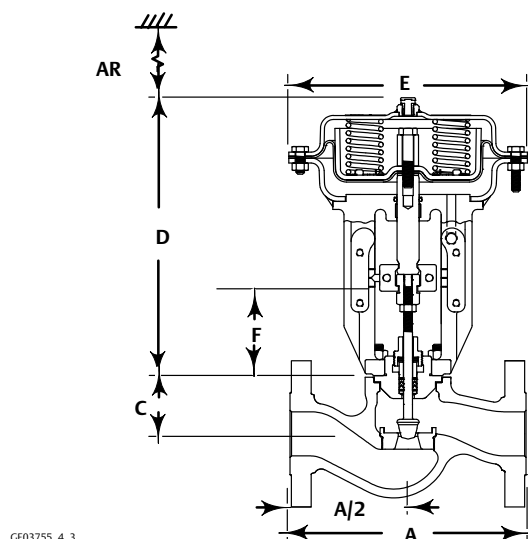
Figure 18. Fisher GX Long Face-to-Face Dimensions (also see table 22)
