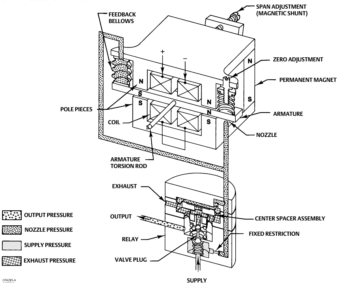
Figure 2. Transducer Schematic
