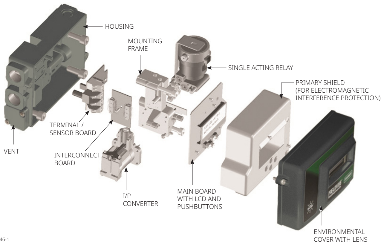
Figure 2. FIELDVUE DVC2000 Digital Valve Controller Assembly (Exploded View)
