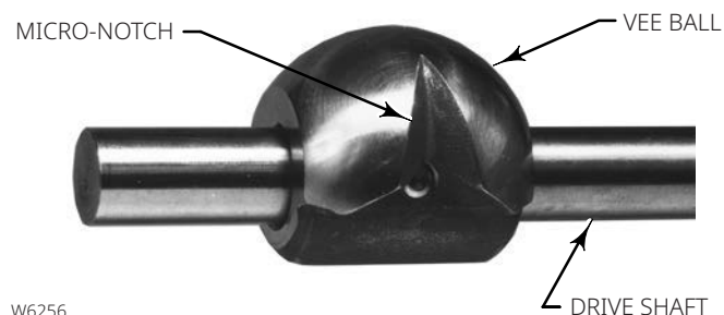
Figure 4. Typical Micro-Notch Ball and Shaft
