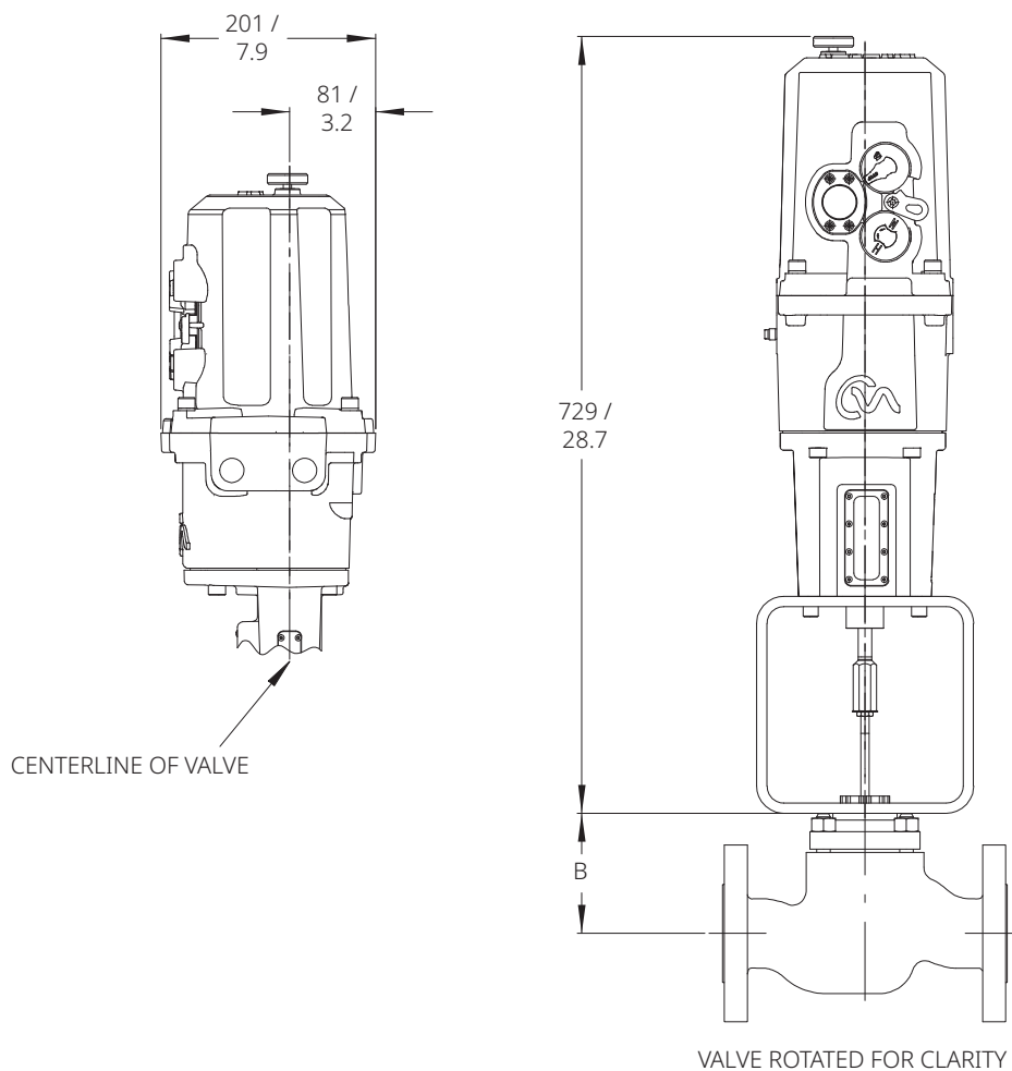
Figure 3. CML-750 Dimensions
