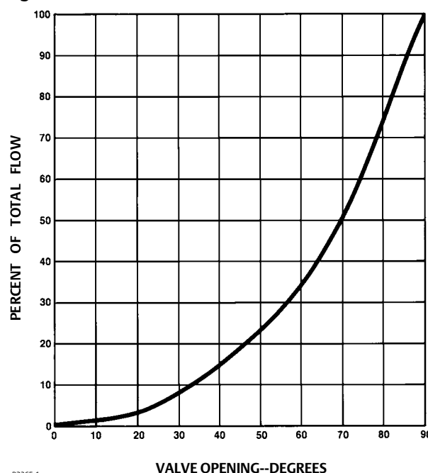
Figure 3. Valve Characteristics
