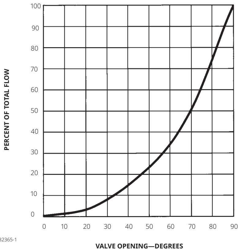
Figure 3. Valve Characteristics
