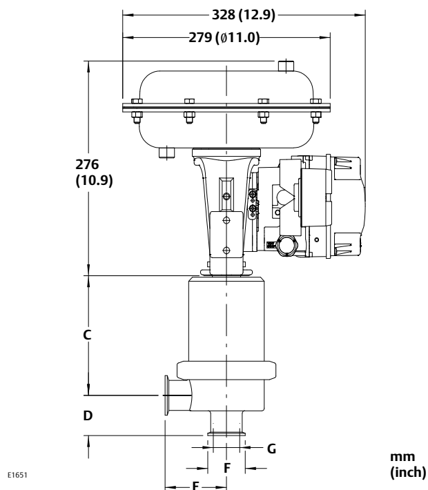
Figure 9. Dimensional Drawing for Baumann 84000 NPS 1-1/2 and 2 Angle Valve with FIELDVUE Digital Valve Controller
