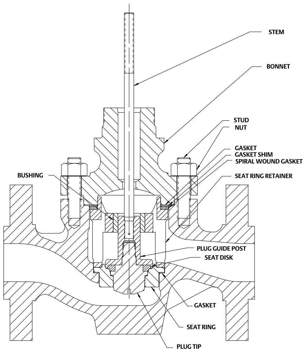
Figure 6. Fisher EZ-OVT Valve Assembly
