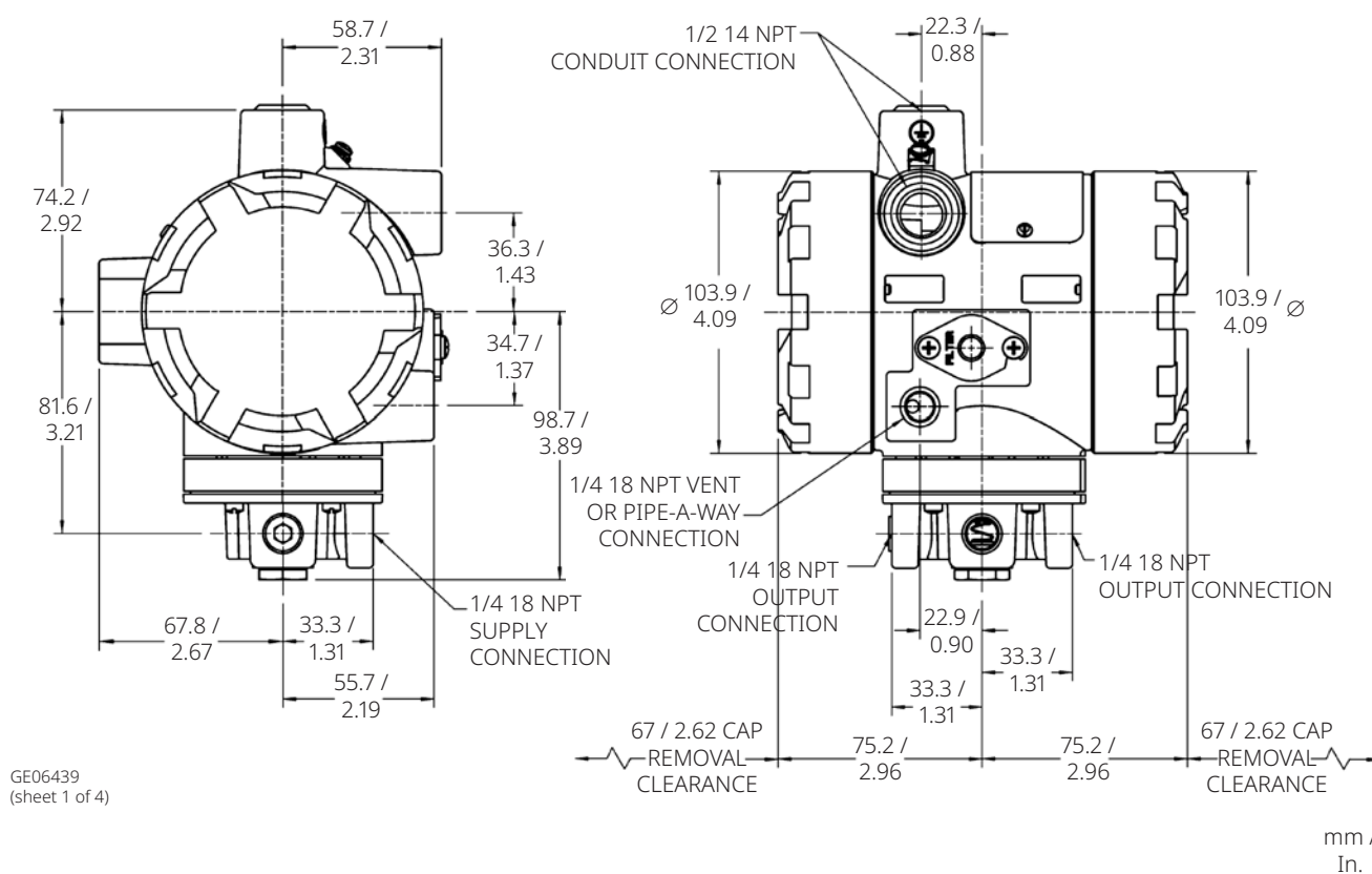
Figure 6. Dimensions
