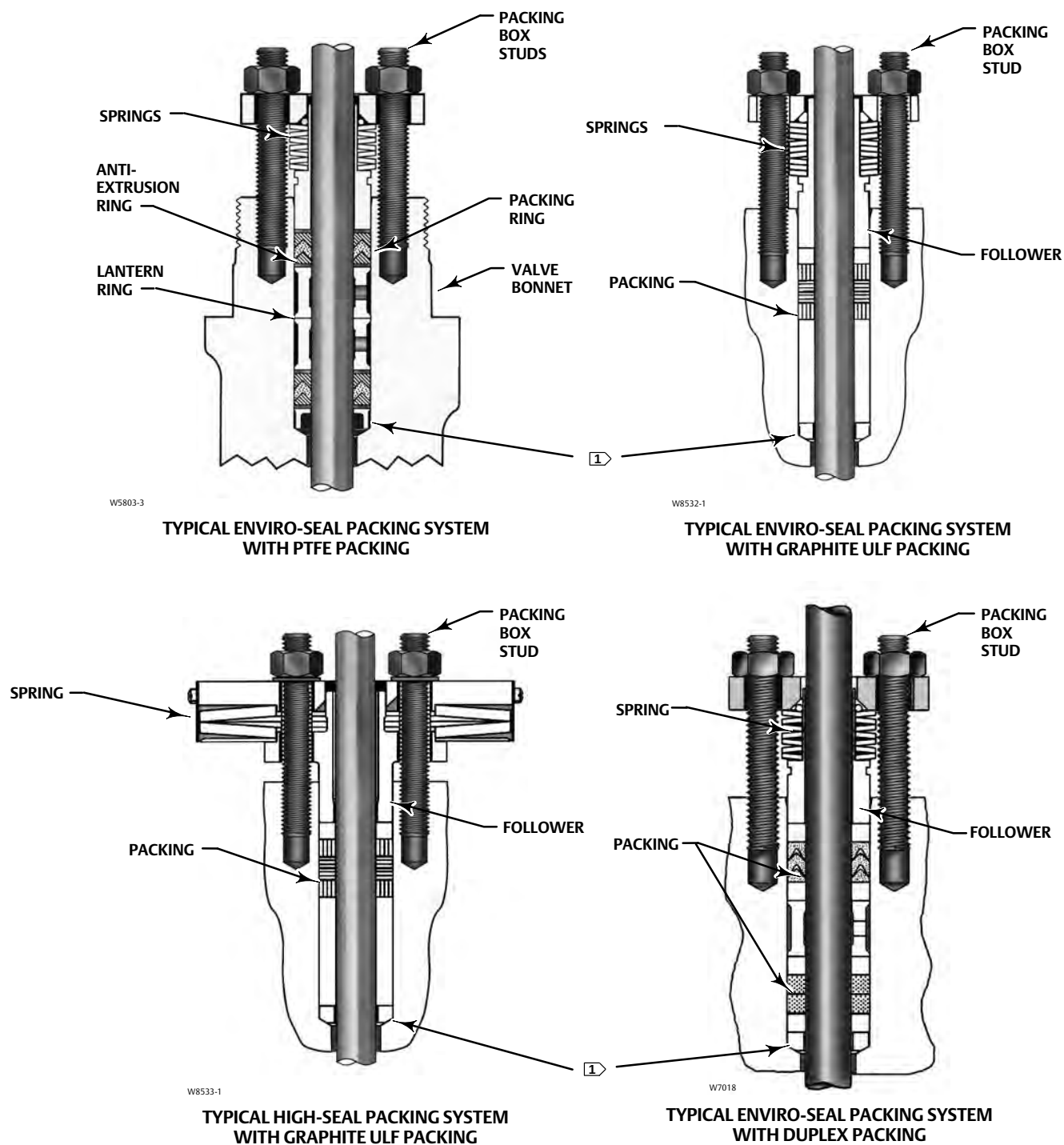
Figure 4. ENVIRO-SEAL and HIGH-SEAL Packing Systems
