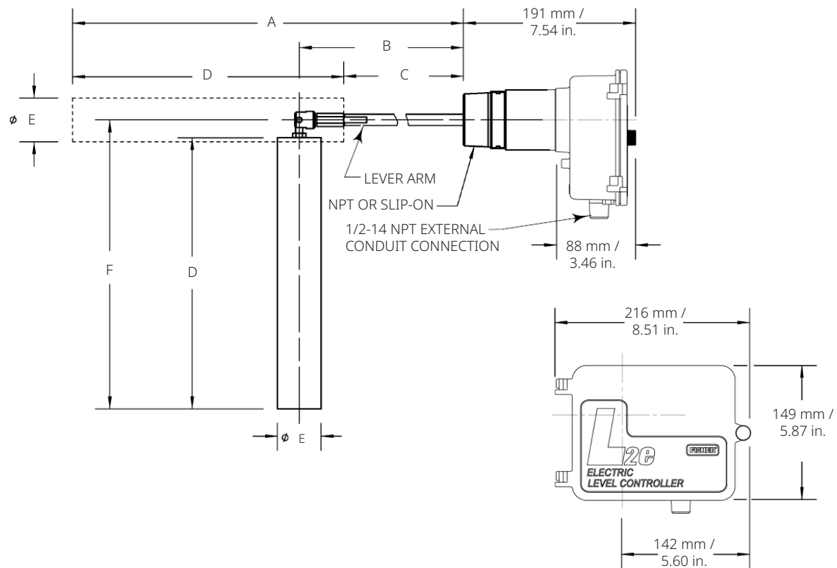
Figure 3. Dimensions
