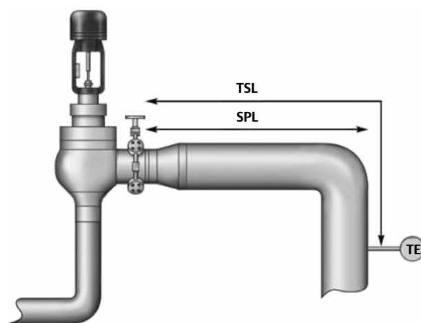
Figure 6. Application Schematic
