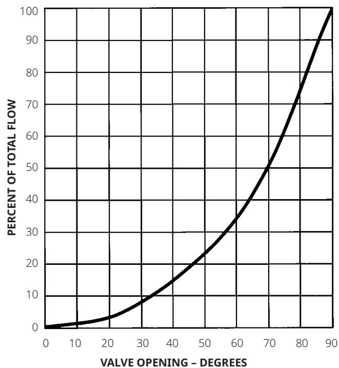
Figure 5. Severe Service Trim Valve Characteristics
