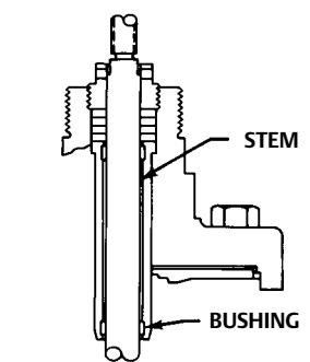
DETAIL OF BONNET FOR NPS 3 AND 4 VALVES 40B4190-D A3598-3
