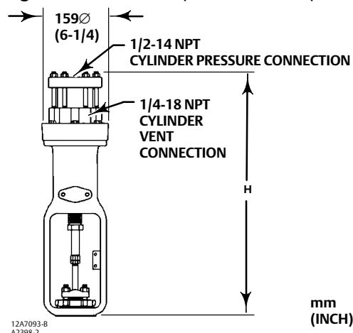
Figure 2. Dimensions (also see table 2)
