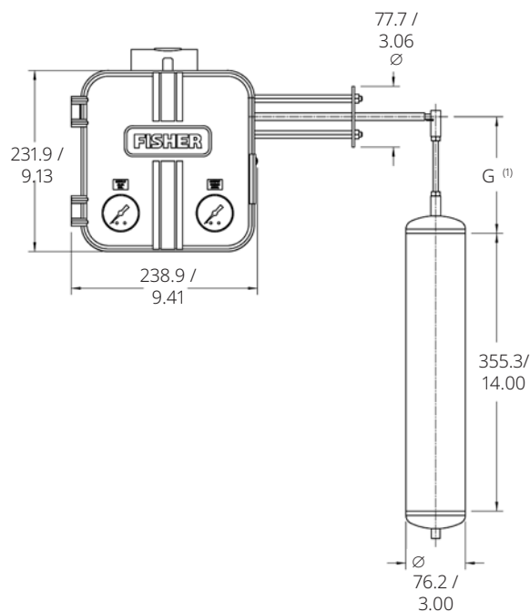
RIGHT-HAND MOUNT
