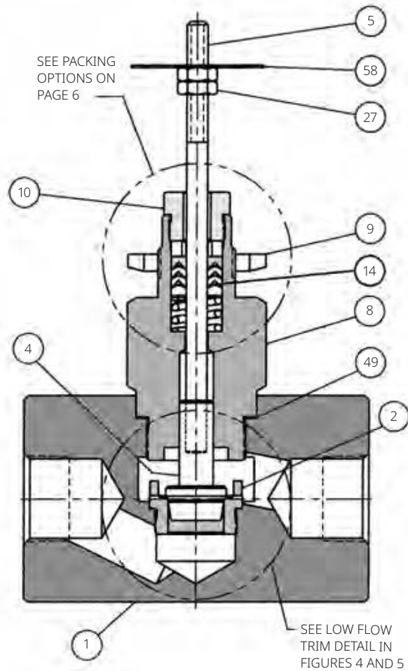
Figure 2. Valve Body Sub-Assembly with Standard PTFE Spring-Loaded V-ring Packing
