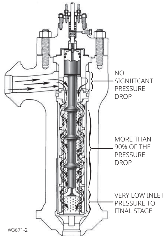
Figure 5. Staged Pressure Drop Patterns
