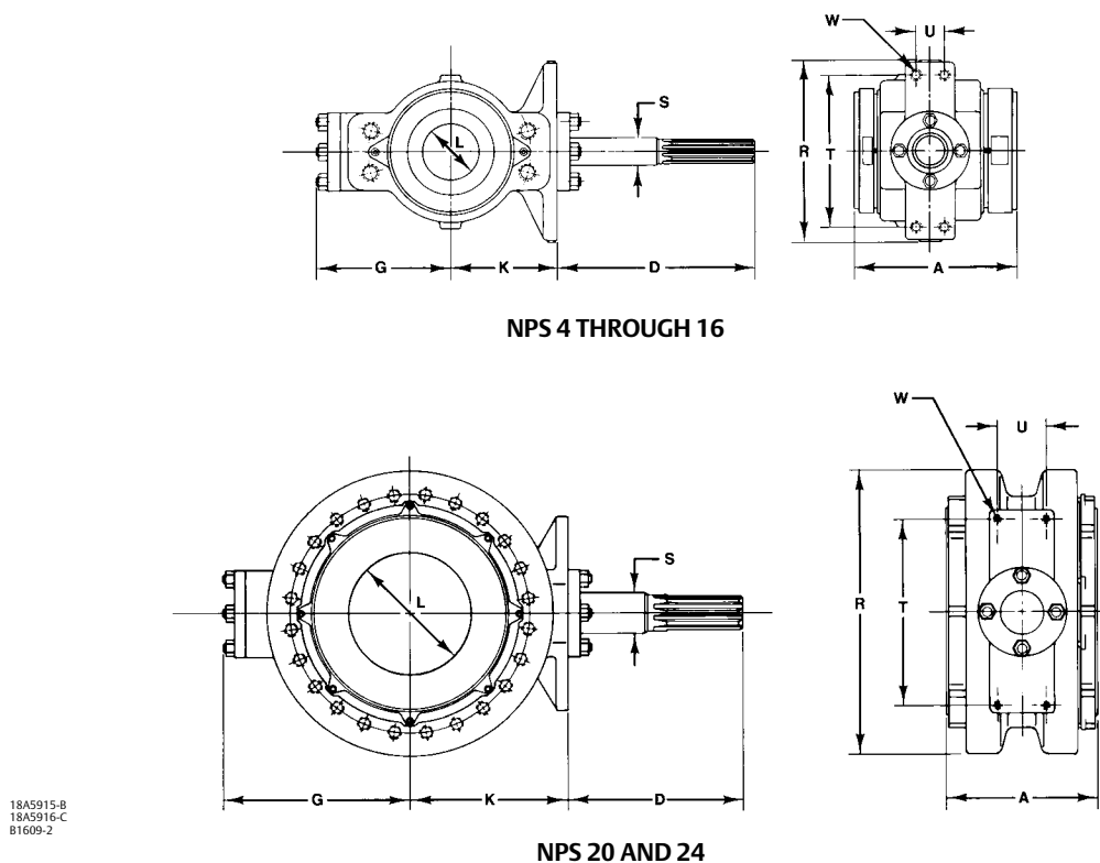
Figure 7. Dimensions (also see table 3)
