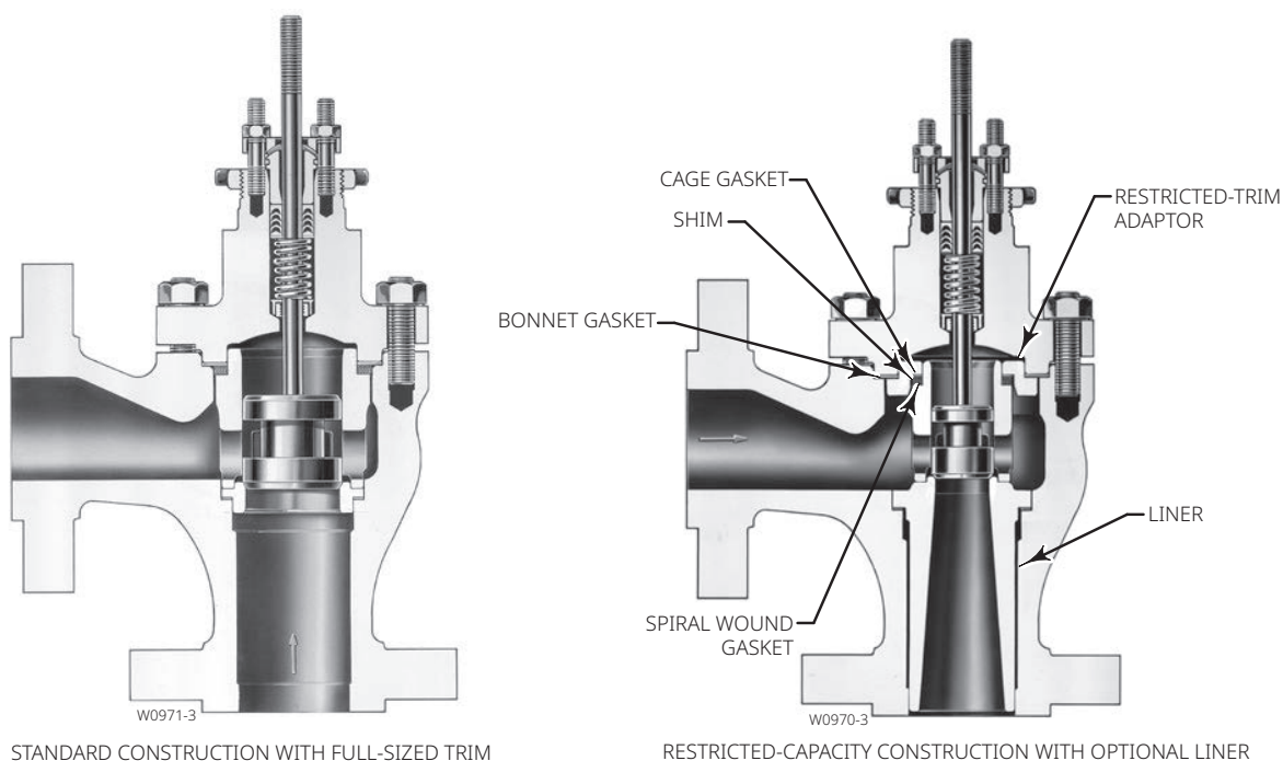
Figure 2. Fisher EAS Sectional
