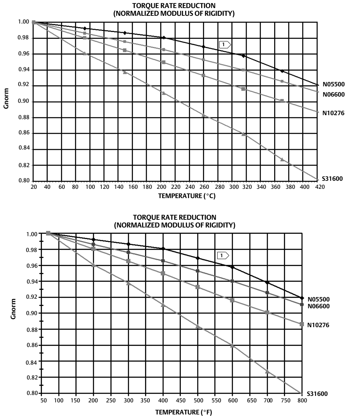
Figure 5. Theoretical Reversible Temperature Effect on Common Torque Tube Materials
