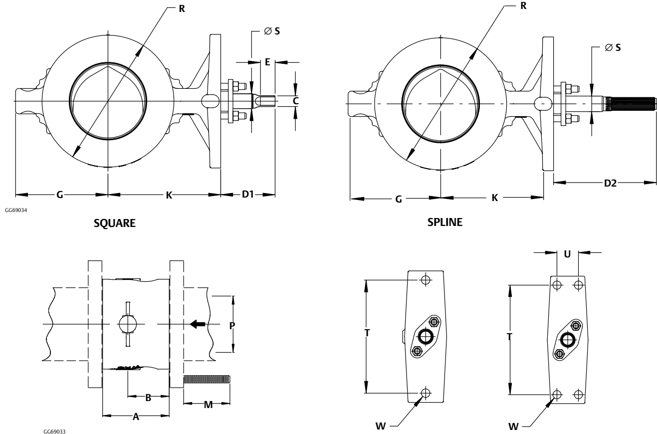
Figure 5. Fisher V200U Dimensions with Square and Spline Shaft (also see tables 6 and 7)
