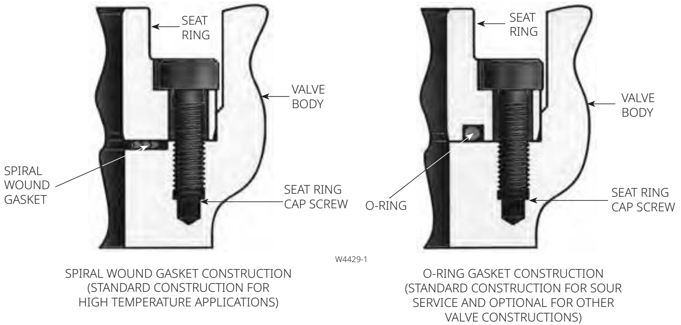
Figure 13. Seat Ring Gasket Constructions (NPS 8 through 14 Globe Valves)
