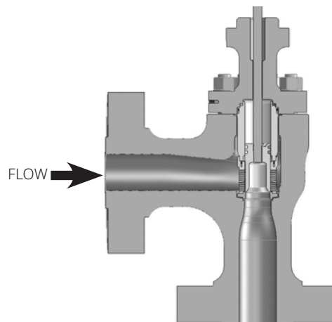
Figure 8. Fisher HPAT Valve Assembly, NPS 6 to 12
