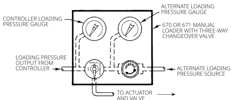
Figure 7. Schematic of Manual Backup Changeover Hookup
