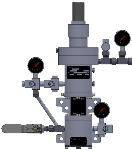
Figure 3. Direct-Acting Configuration
