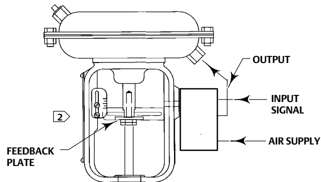
Figure 1. Mounting Configurations (see table 3 for Positioner Action and Signals)
