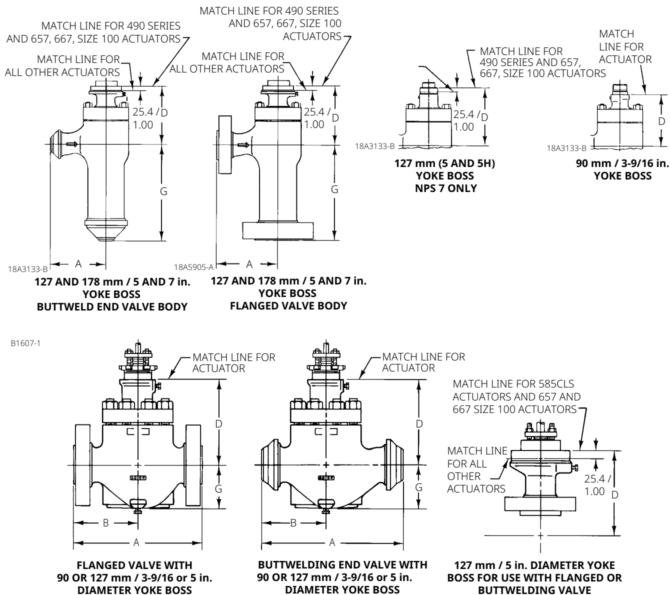
Figure 8. Dimensions (See Table 6)
