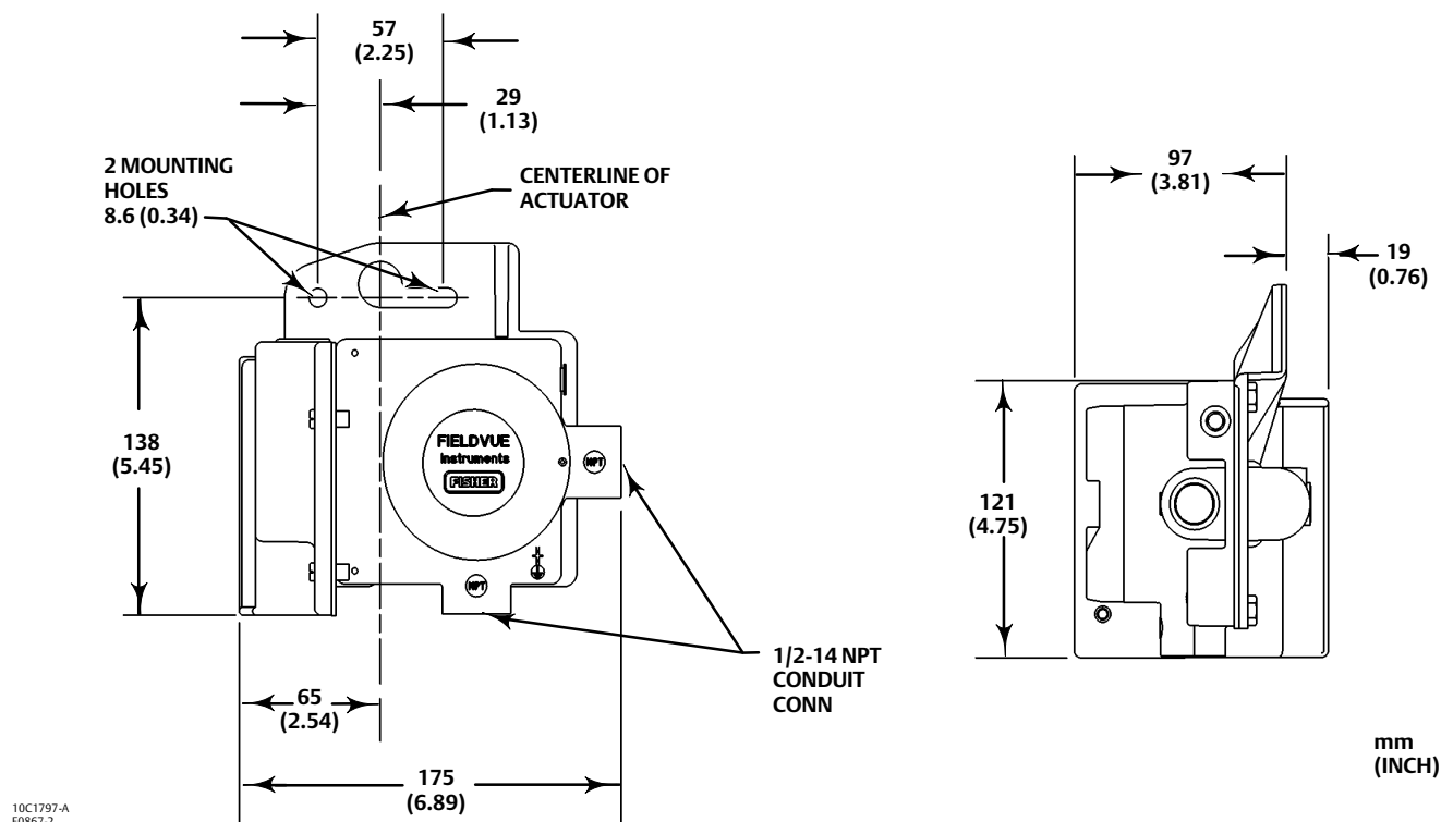
Figure 3. FIELDVUE DVC6015 Feedback Unit; Sliding-Stem Actuator Mounting up to 102 mm (4 inch) Travel
