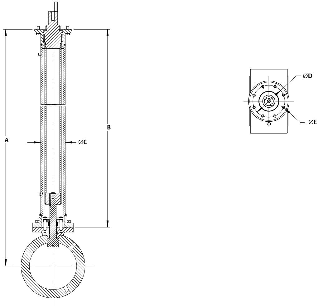
Figure 2. Envelope Dimensions (see tables 2 and 3)
