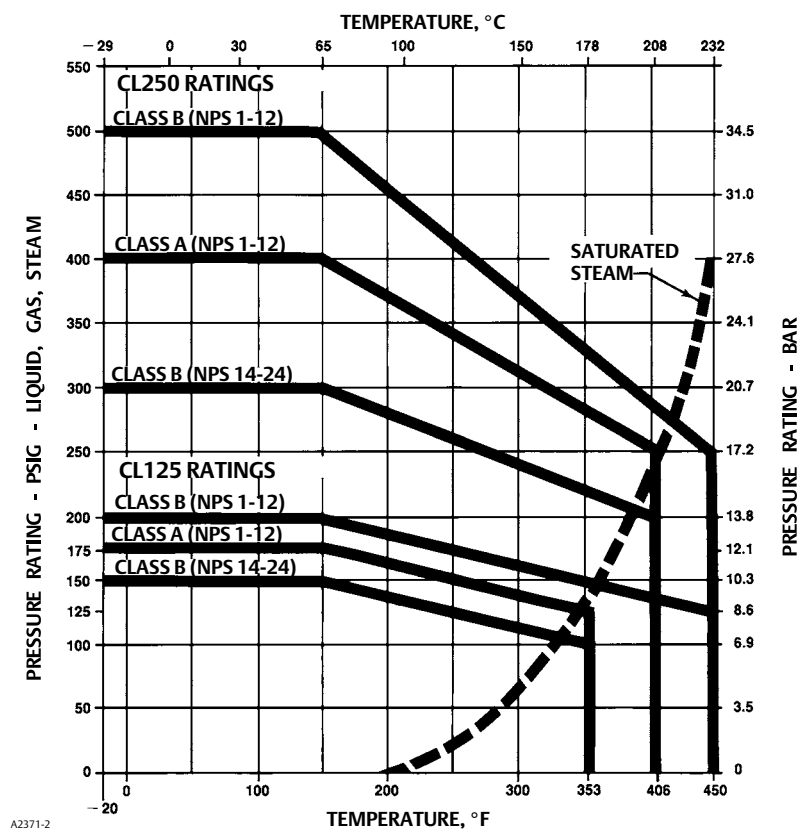
Pressure/Temperature Ratings
