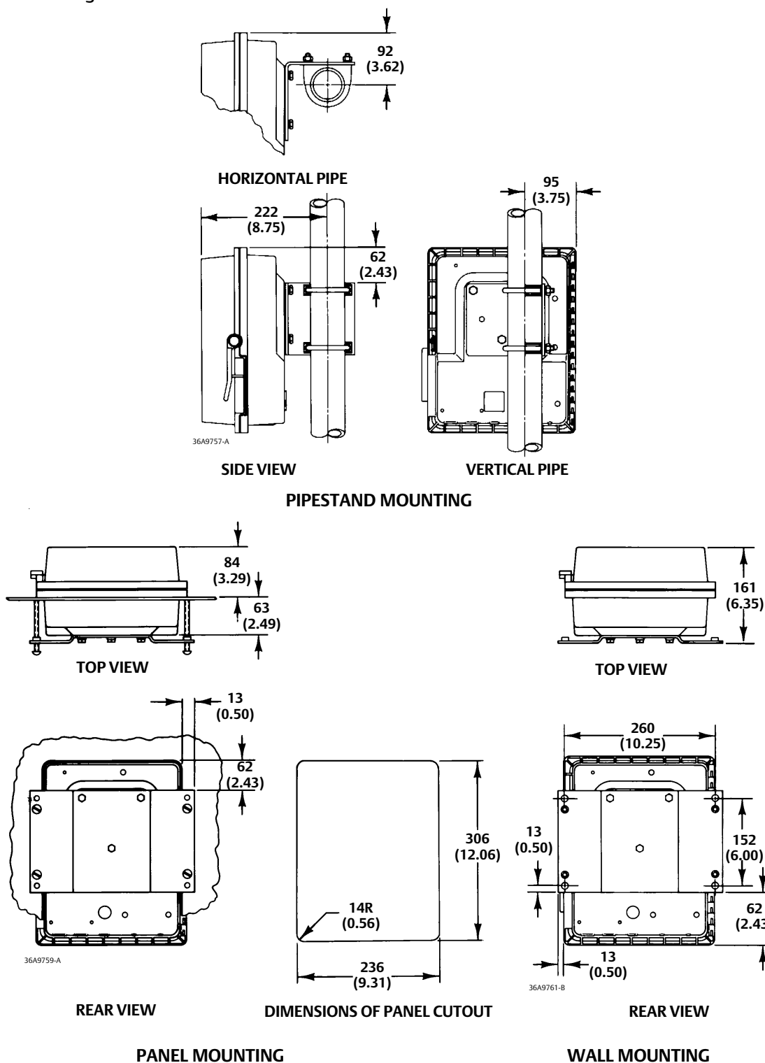
Figure 7. Mounting Dimensions
