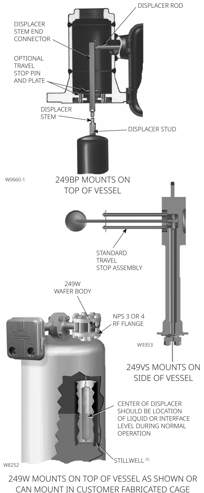
Figure 3. Typical Cageless Sensors
