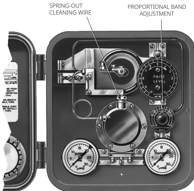
DIRECT-ACTING 2500 CONTROLLER
