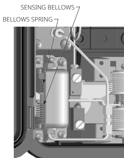
BELLOWS DETAILS
