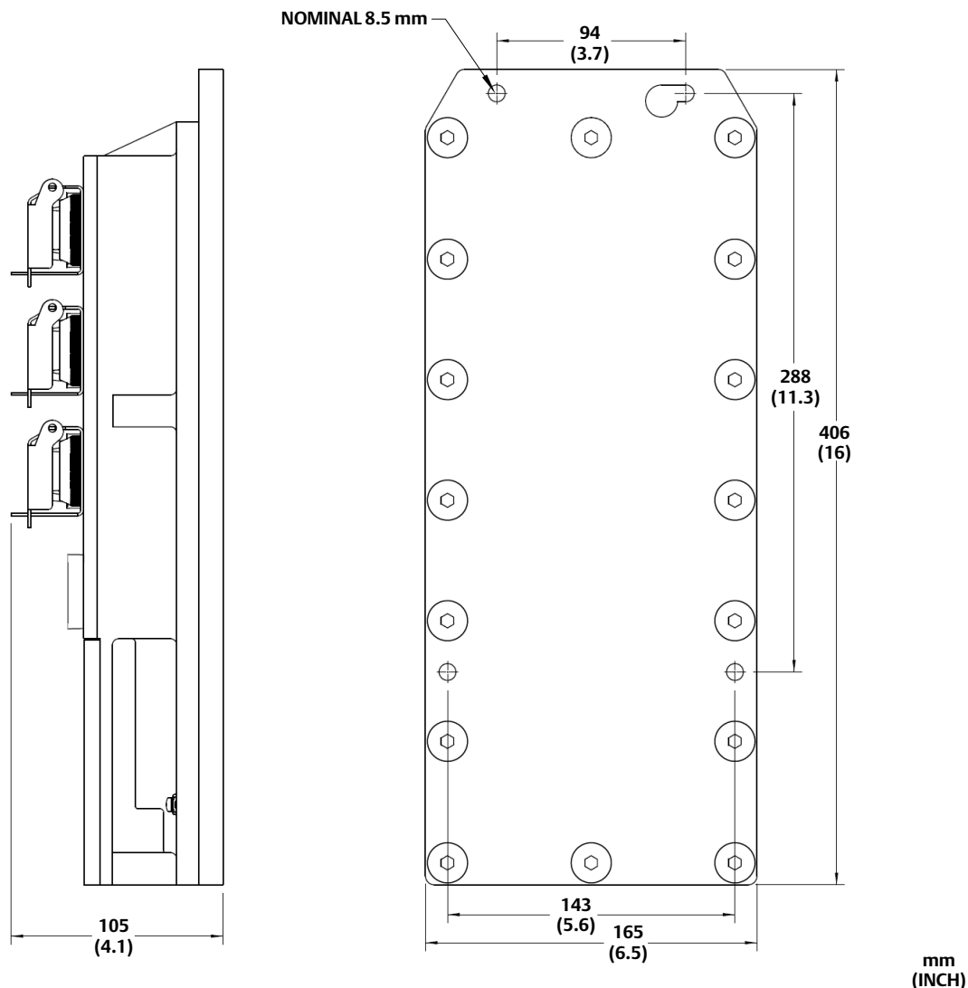
Figure 2. Dimensions
