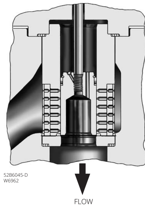
Figure 3. Fisher HPT with Cavitrol III Three-Stage Trim
