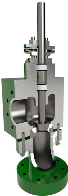
Figure 2. Fisher EHU Valve
