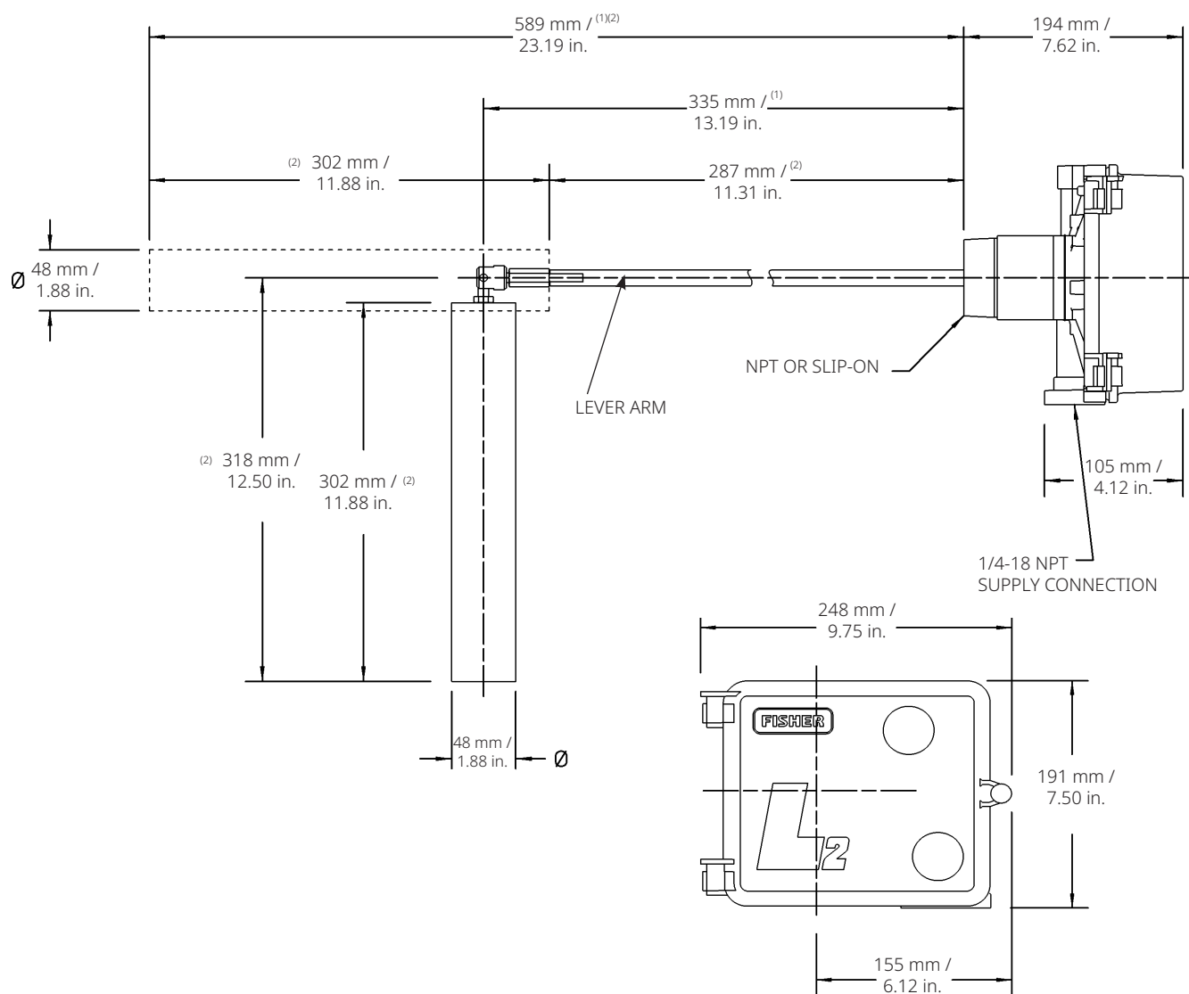
Figure 2. Dimensions
