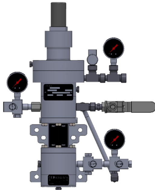
Figure 4. Reverse-Acting Configuration
