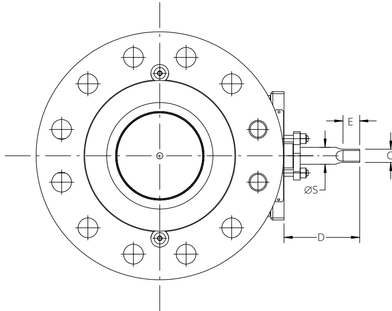
Figure 19. Fisher Vee-Ball Square Shaft Dimensions (also see Table 18)
