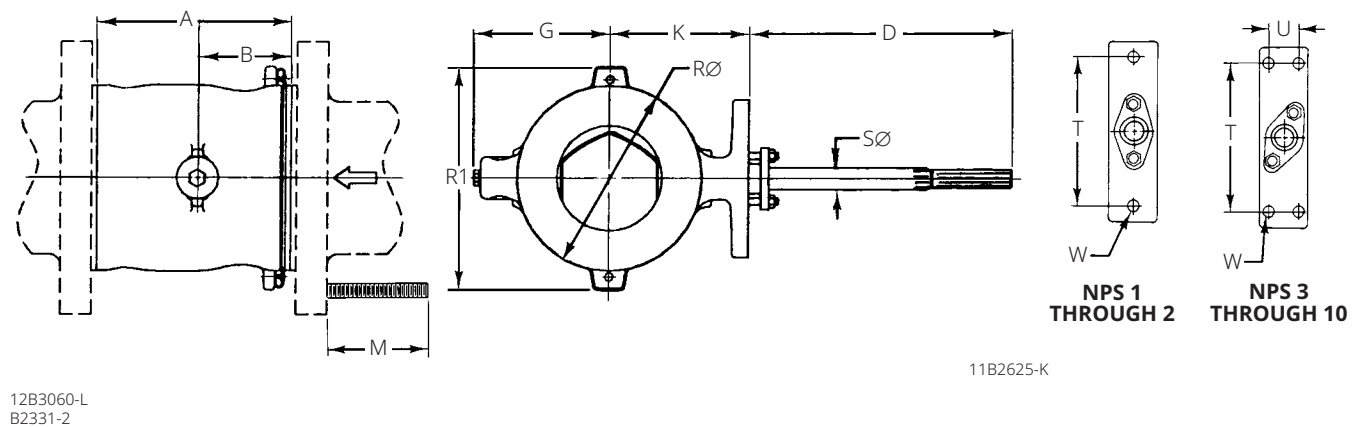
Figure 15. Fisher V200 Dimensions (also see Table 12)
