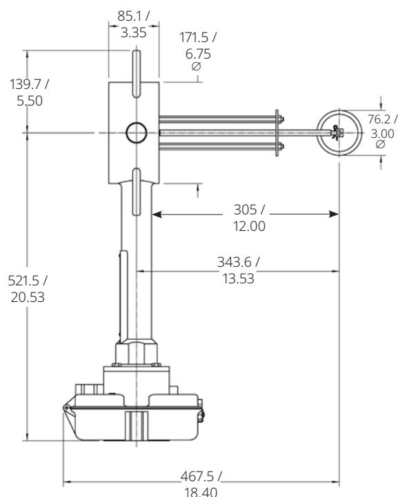
RIGHT-HAND MOUNT
