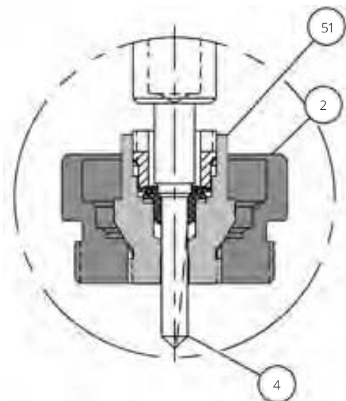
Figure 4. Optional 151 Low Flow Trim Assembly
