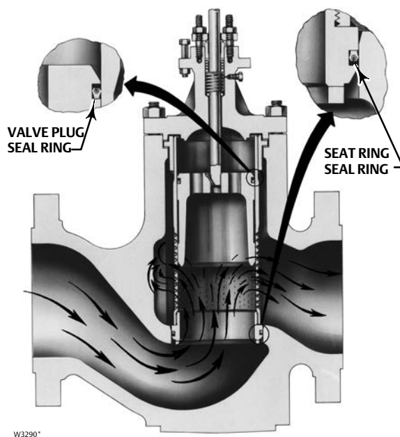
Figure 2. Fisher EWNT-2, NPS 12x8 Valve with Seat Ring Threaded Into the Cage
