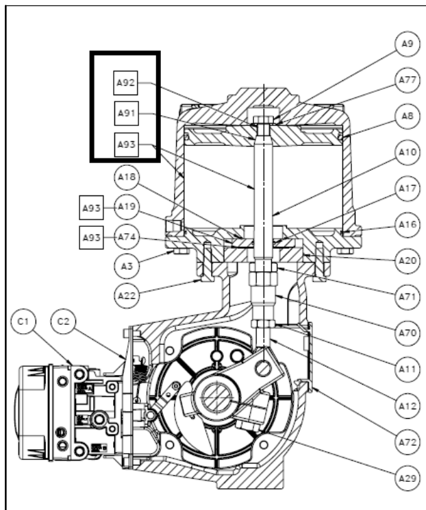
Figure 4. Lubricant Call-Outs
