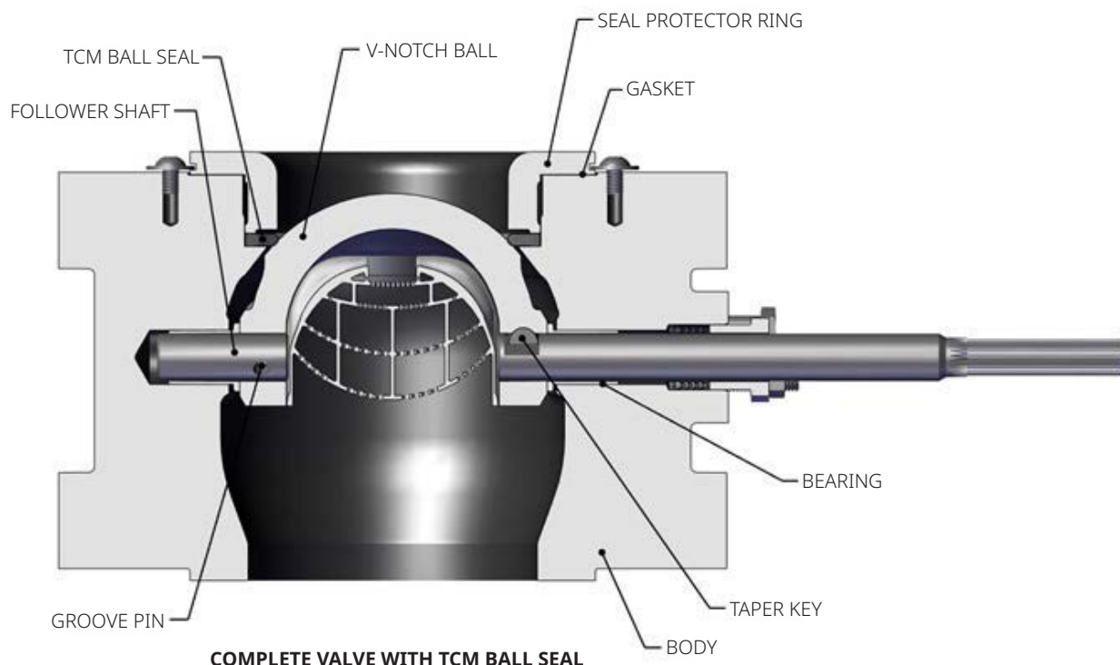
Figure 12. Fisher Vee-Ball Series Whisper NXV Construction
