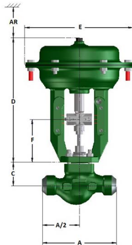
Figure 2. Fisher GX Dimensions
