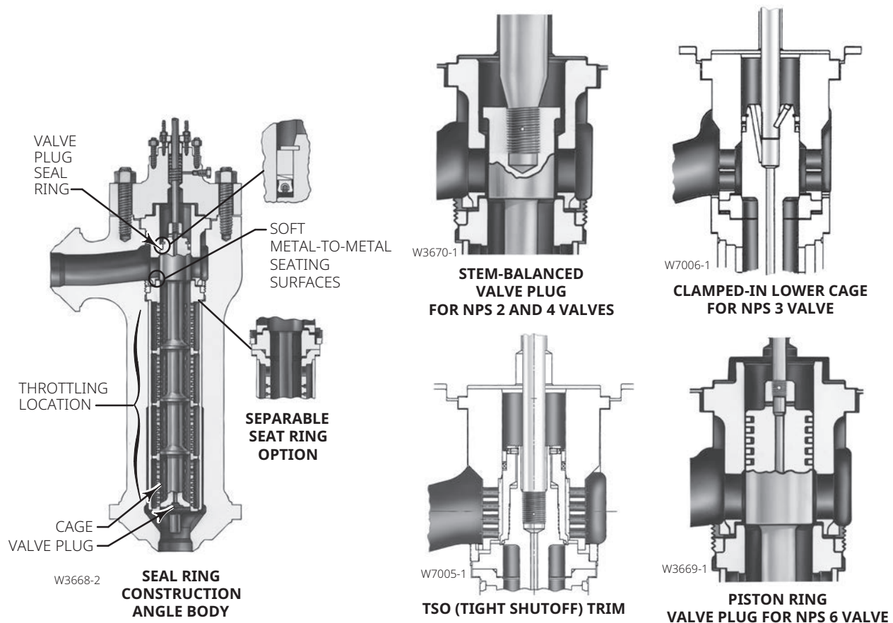
Figure 2. Sectional View of Fisher CAV4 Angle Valve Body with Cavitrol IV Trim
