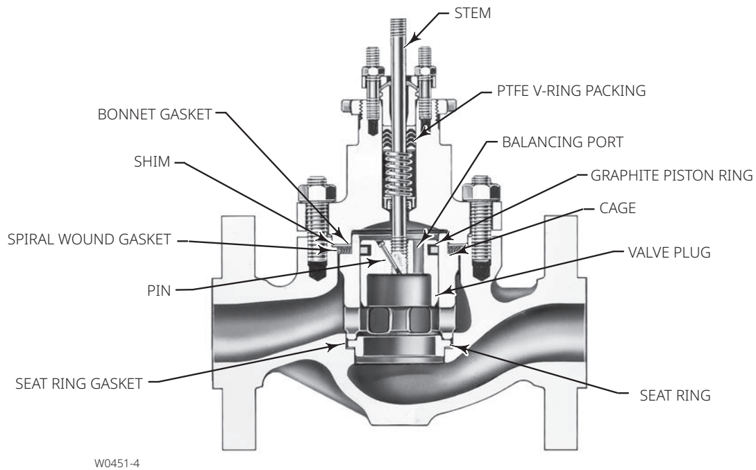
STANDARD NPS 1 THROUGH 6 CONSTRUCTION
