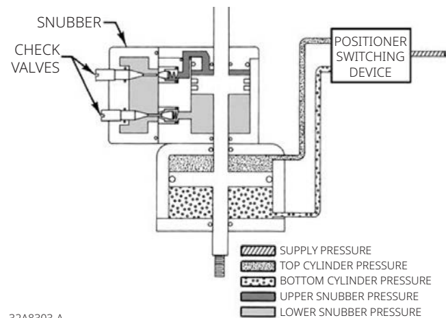
Figure 5. Operation of Actuator with Snubber
