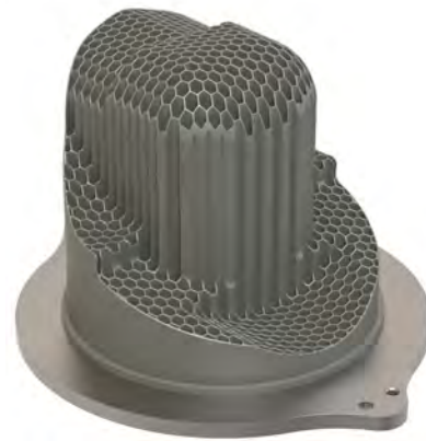
Figure 5. Fisher NPS 10 Fisher CV500 Cavitrol Hex Trim
