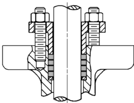
Figure 10. Graphite Packing
