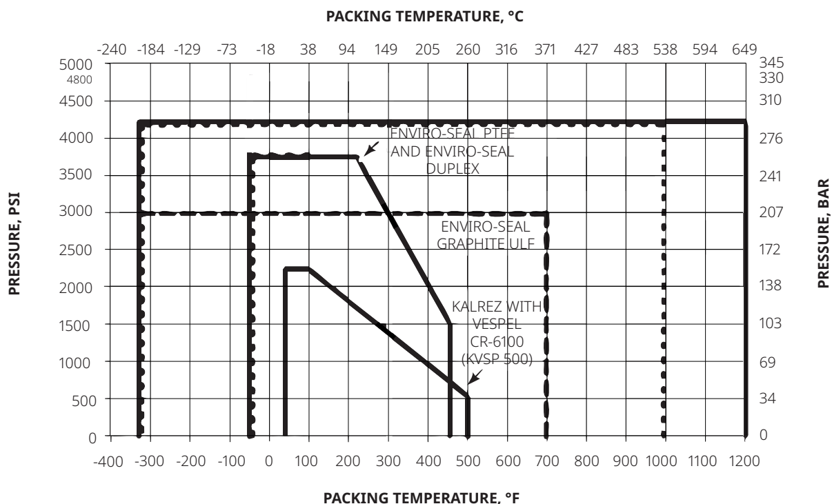
Figure 2. Applications Guidelines Chart for Extended Service Life
