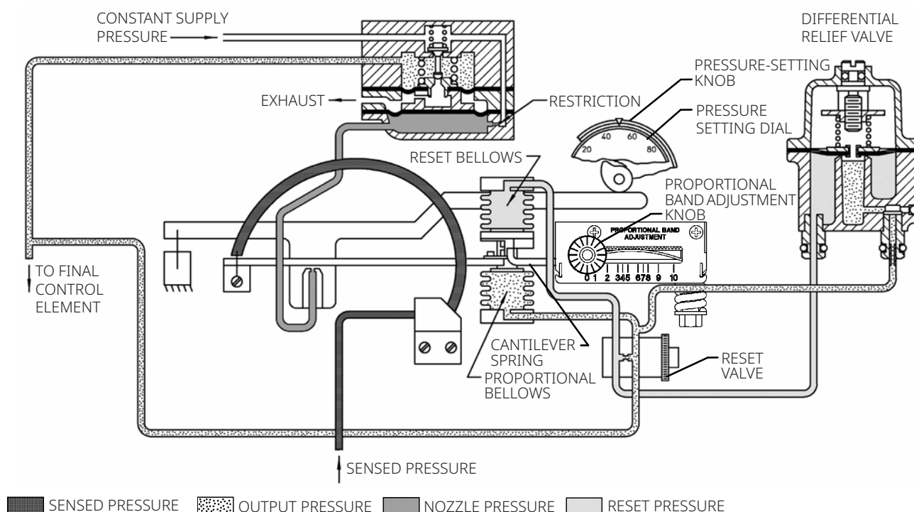
Figure 3. Schematic of Reverse-Acting Proportional-Plus-Reset Controller with Anti-Reset Windup
