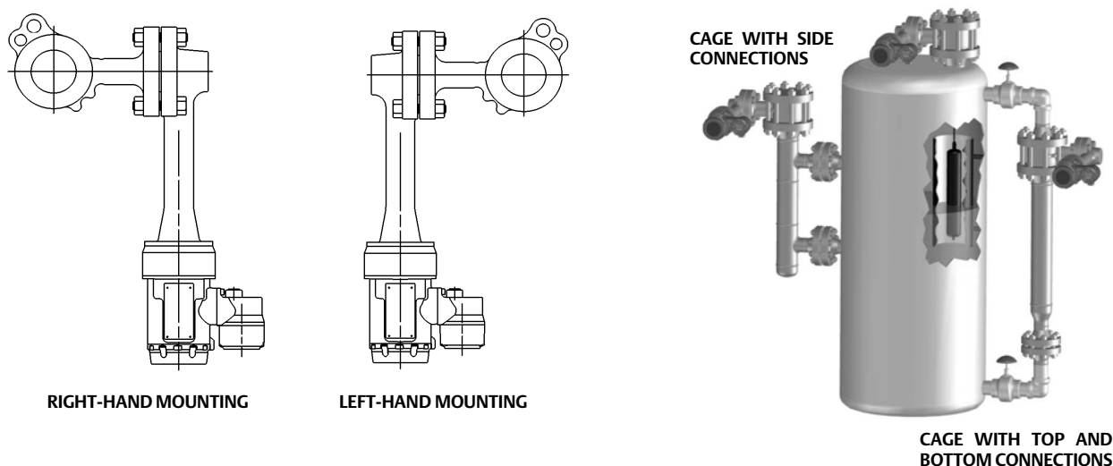
Figure 11. Mounting Positions—Wafer Style (Customer Supplied Cage)
