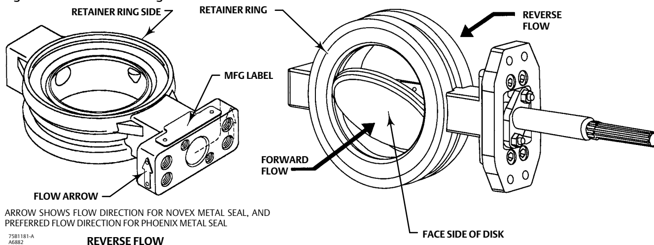
Figure 7. Actuator Mounting
