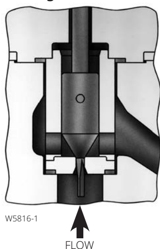
Figure 13. Fisher HPS Trim with Micro-Flute Valve Plug
