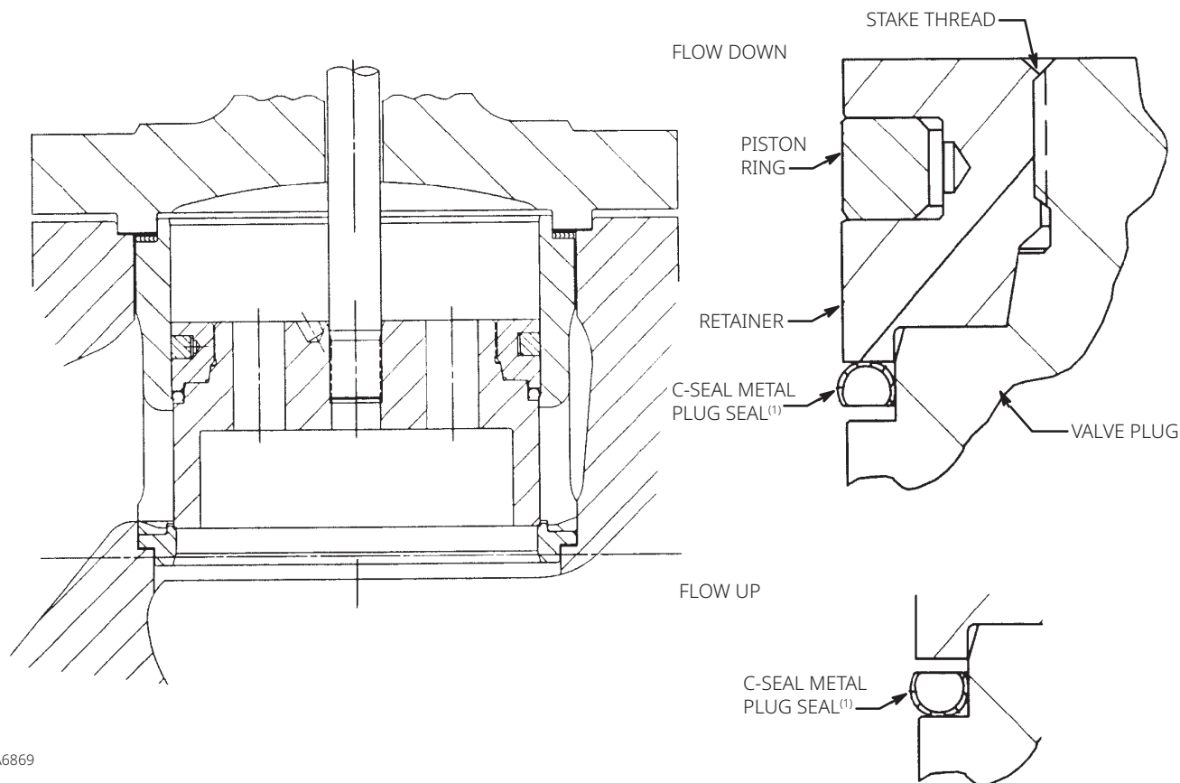
Figure 6. C-seal Trim
