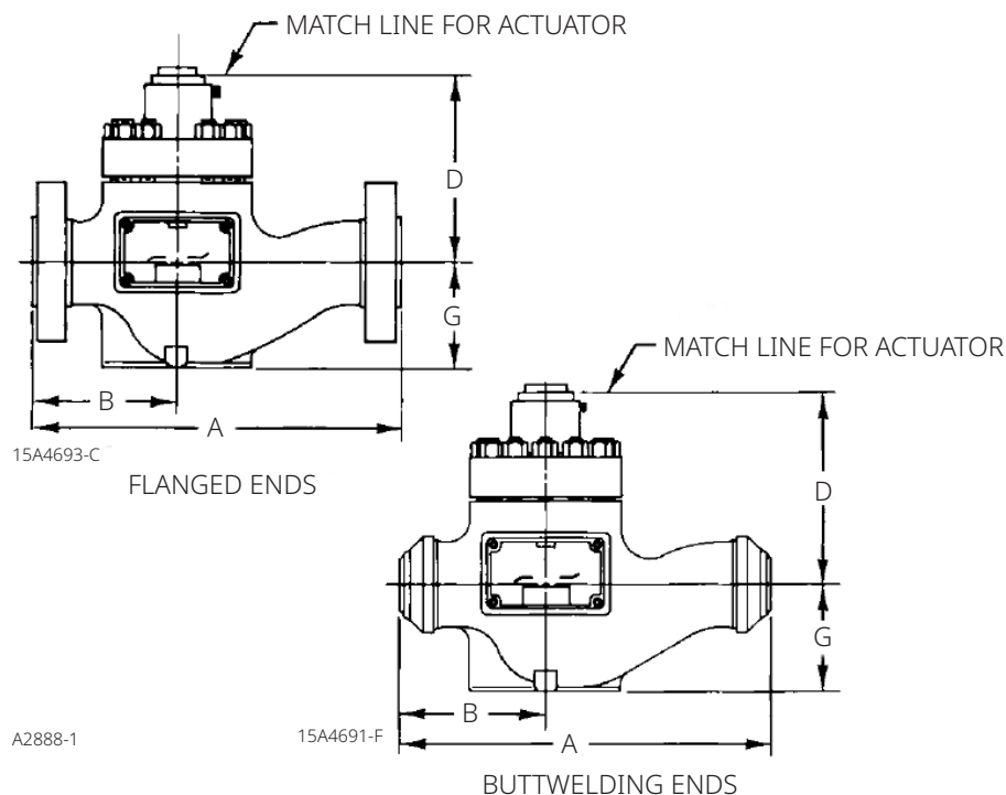
Figure 26. Dimensions (NPS 8 through 14 Fisher EHD and EHT Valves) (Also See Tables 27, 28 and 29)
