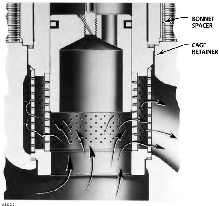
Figure 1. Whisper Trim III Cage in Fisher ED Valve
