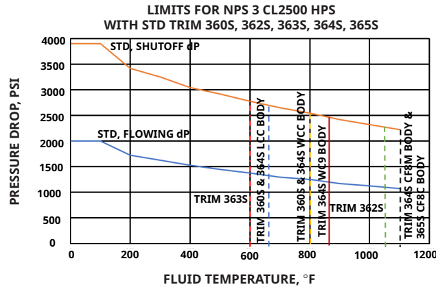
Figure 21. Pressure-Temperature Limits for Standard Window Cage (also refer to Table 7)
