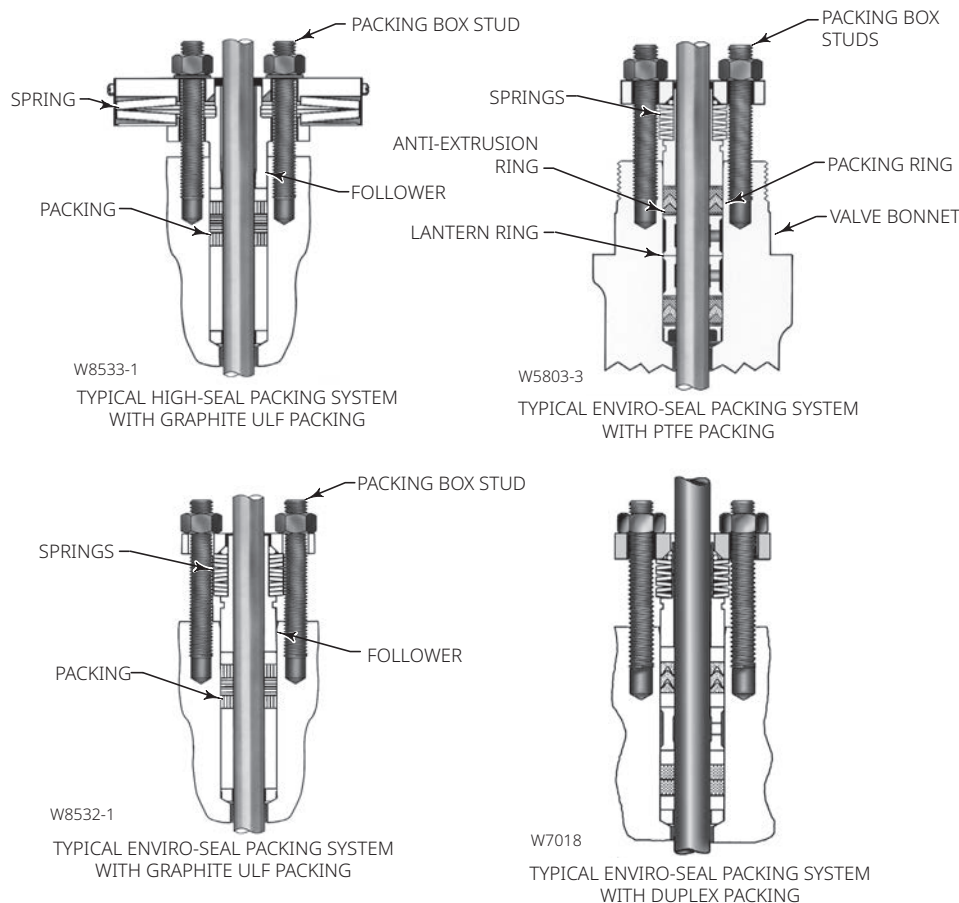
Figure 3. ENVIRO-SEAL and HIGH-SEAL Packing Systems
