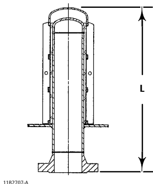
Figure 5. Fisher 6012 Vent Diffuser Dimensions
