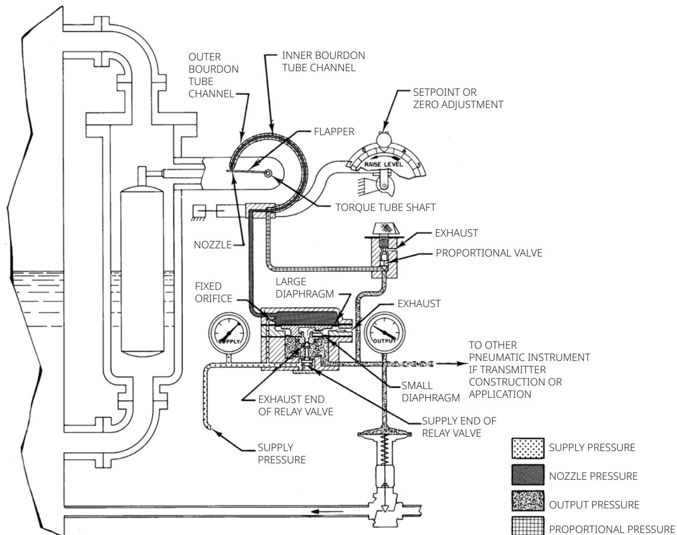
Figure 5. Schematic of Direct-Acting Fisher 2500-249 Proportional Controller (or Transmitter) Shown with Right-Hand Mounting
