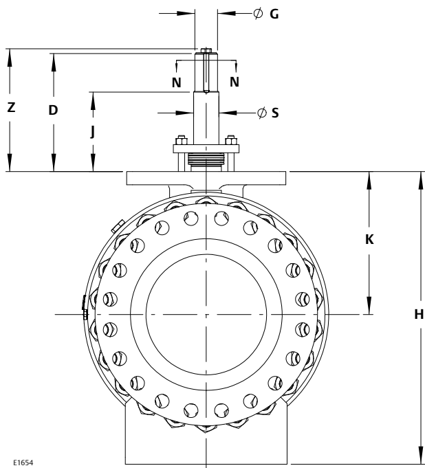
Figure 3. Envelope Dimensions (see table 2 and 3)
