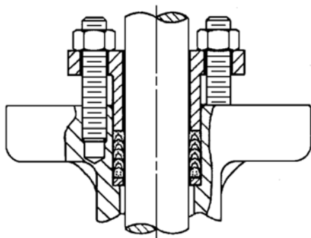
Figure 9. PTFE Packing
