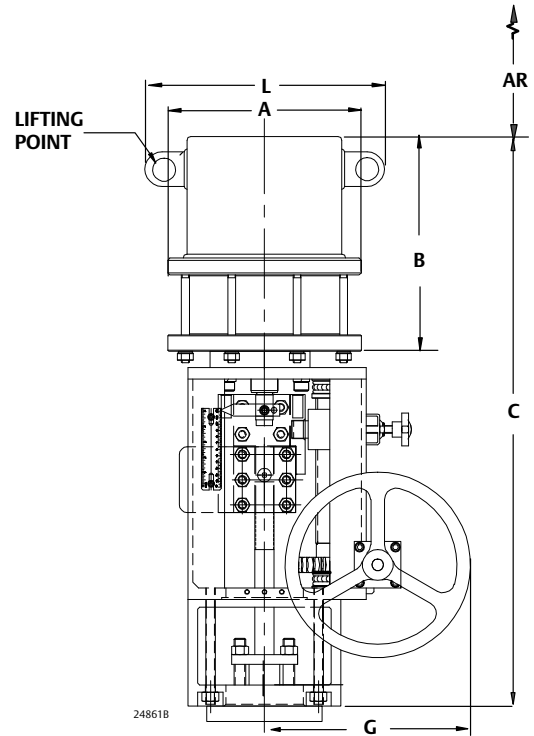
FRONT VIEW OF ACTUATOR WITH HANDWHEEL MANUAL OVERRIDE
