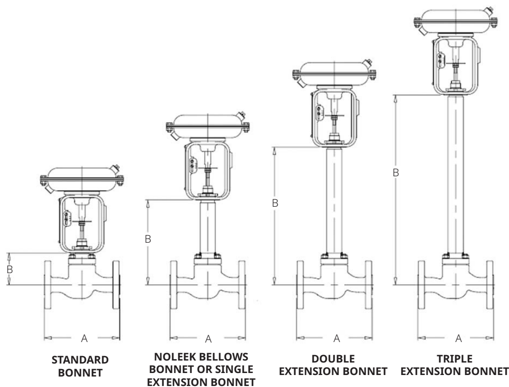
Figure 13. 24000SVF Stainless Steel Control Valves with Extension Bonnets Dimensional Drawing
