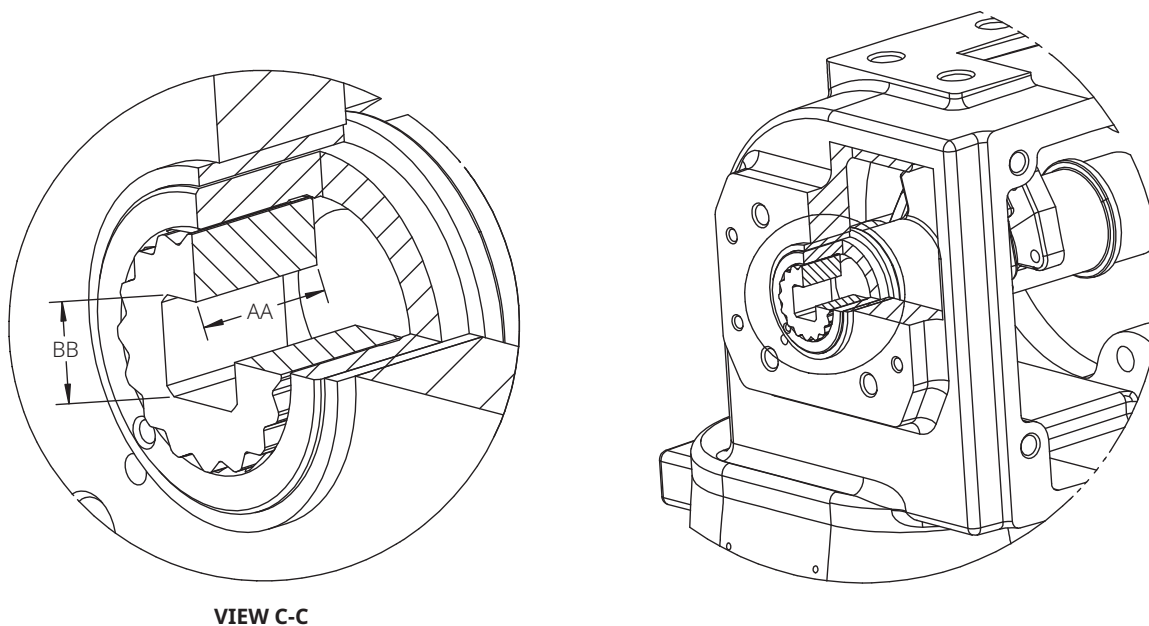
Figure 8. ISO 5211 Square Lever Insert Dimensions (also see Table 11) (1)
