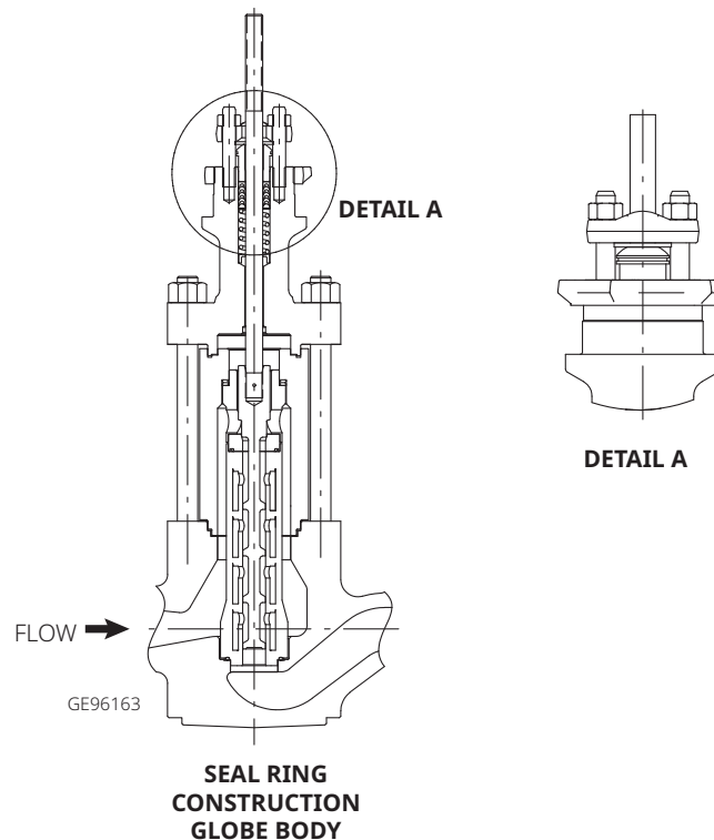
Figure 3. Standard Cage-Style Anti-Cavitation Trim
