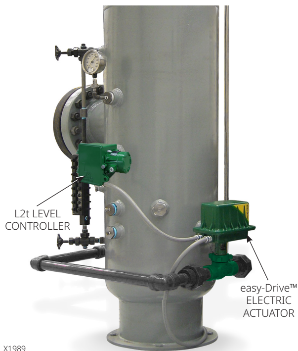
Figure 1. Fisher L2t Liquid Level Controller
