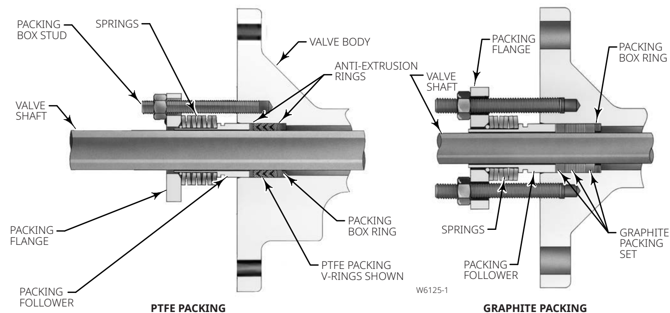
Figure 13. Typical ENVIRO-SEAL Packing Arrangements
