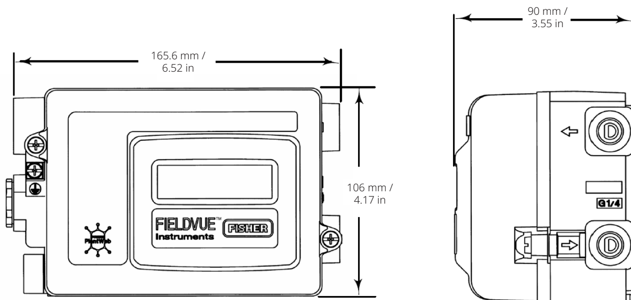
Figure 4. Dimensions
