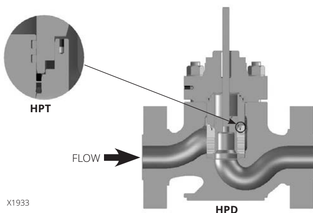
Figure 4. Fisher HPD and HPT Valve Assembly, NPS 16 to 24
