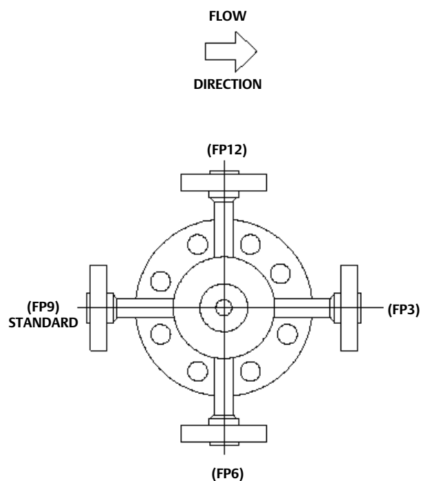
Figure 8. Water Flange Positions
