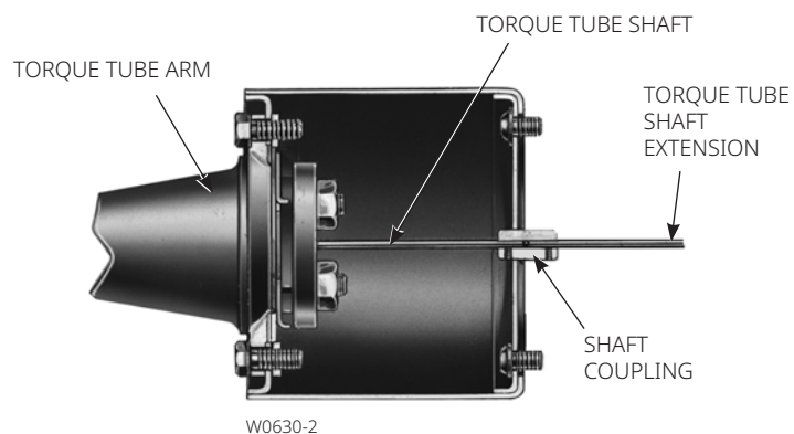
Figure 8. Optional Heat Insulator Assembly
