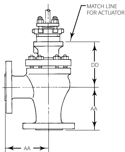
Figure 8. Fisher EAS Dimensions (also see Tables 17 and 18)
