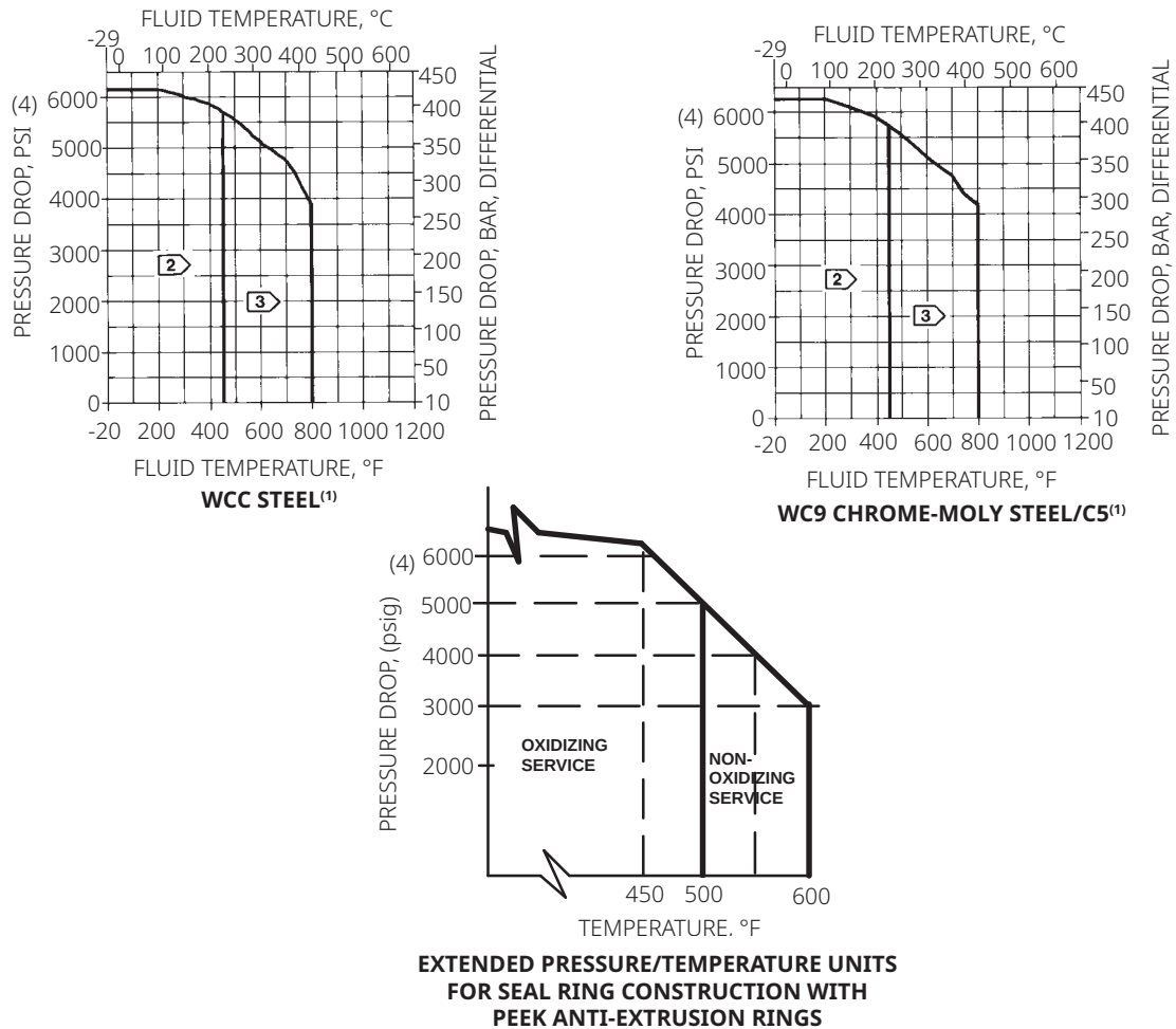
Figure 6. Pressure Drop/Temperature Capabilities
