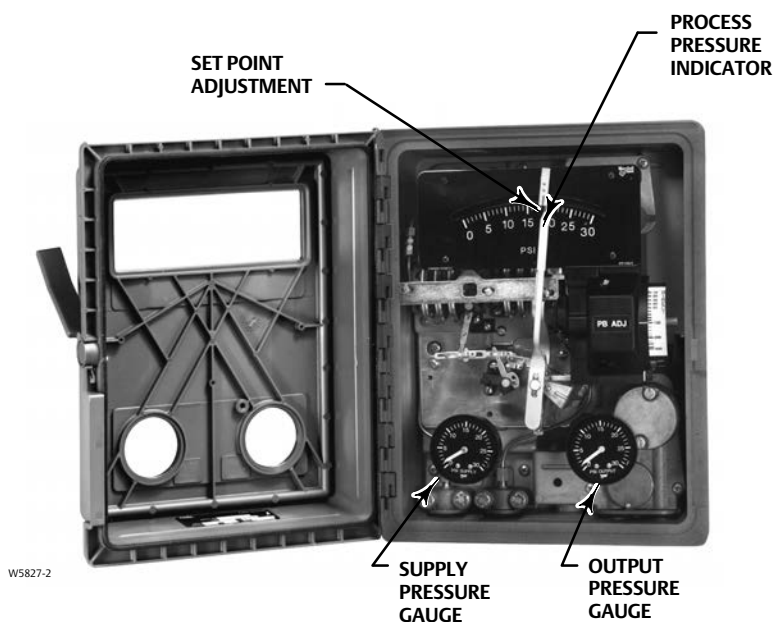
INTERIOR OF CONTROLLER
