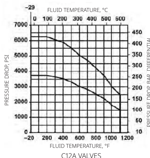
Figure 22. Pressure/Temperature Limits for CL1500 and 2500 Valves (NPS 8 through 14 Valves)
