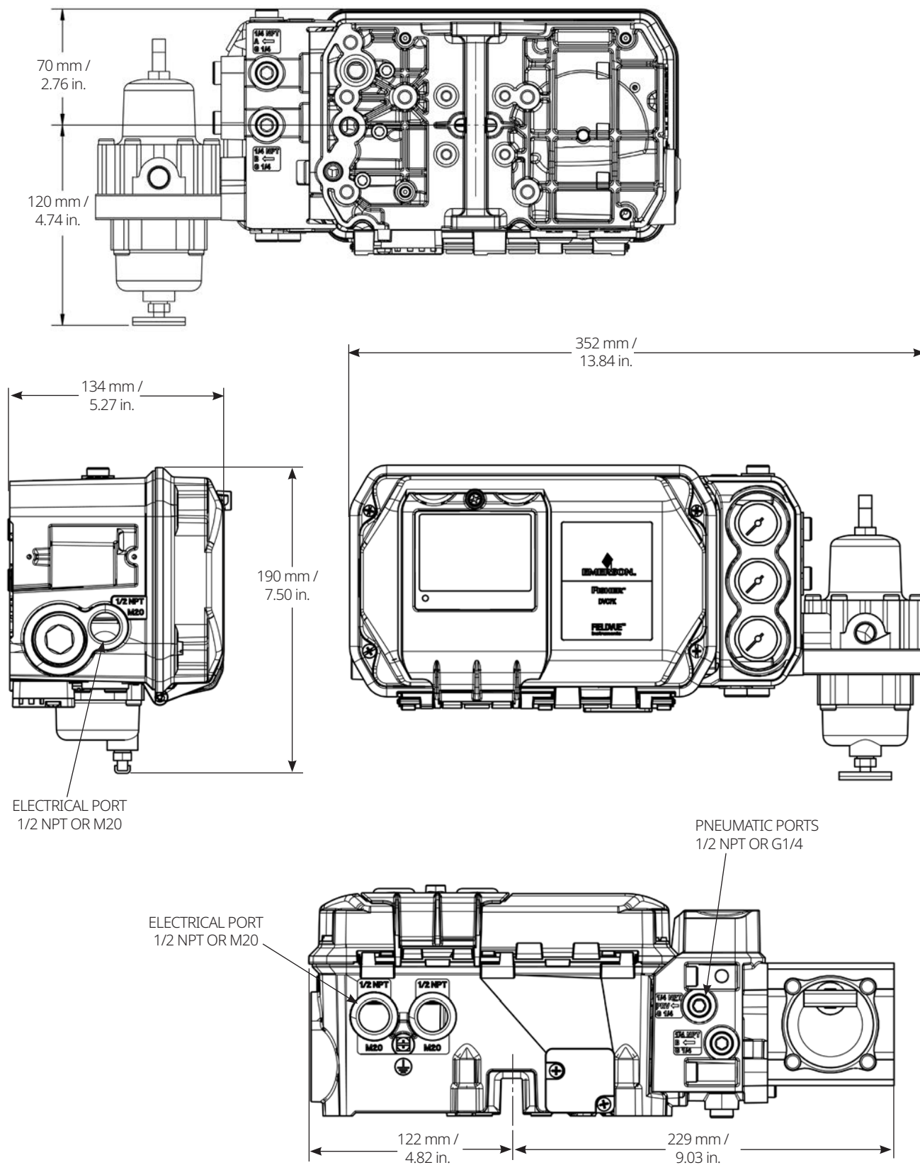
Figure 3. With Optional Gauge Block and Integrally Mounted Filter Regulator (Position 1) Dimensions
