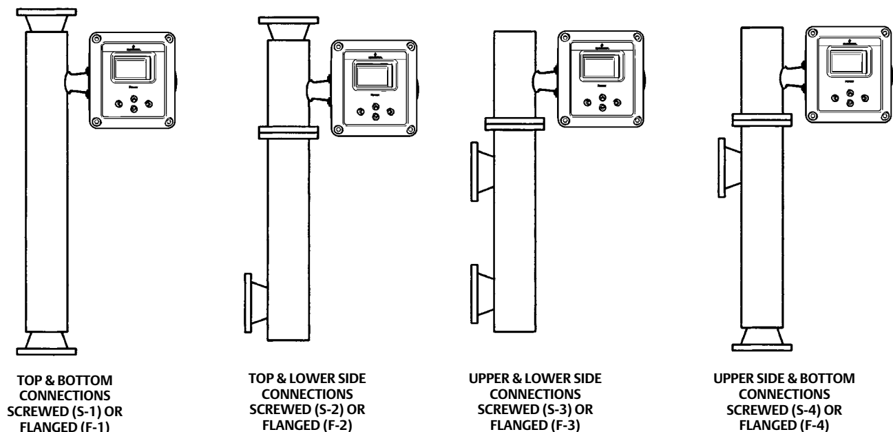
Figure 8. Style Number of Equalizing Connections
