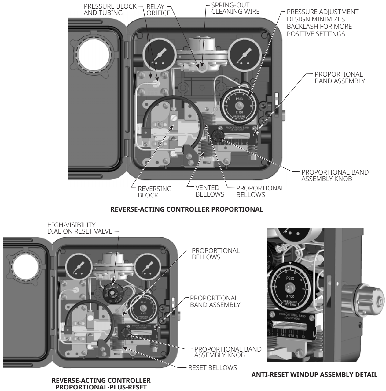
Figure 5. Fisher C1 Constructions
