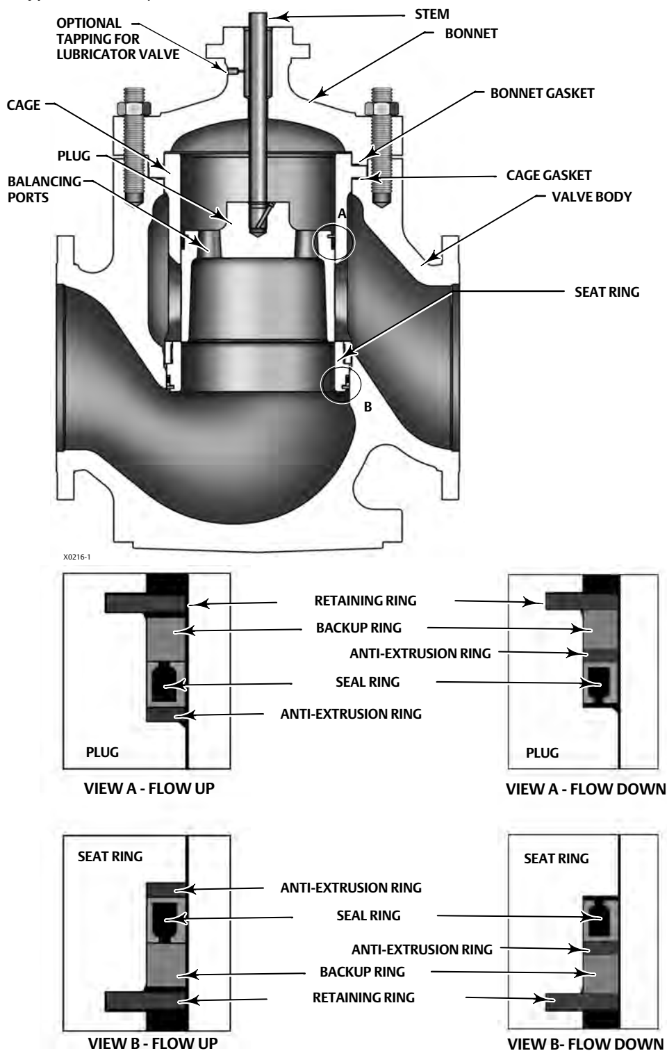
Figure 4. Typical Fisher ET/EWT Valve with HTS1 Seal
