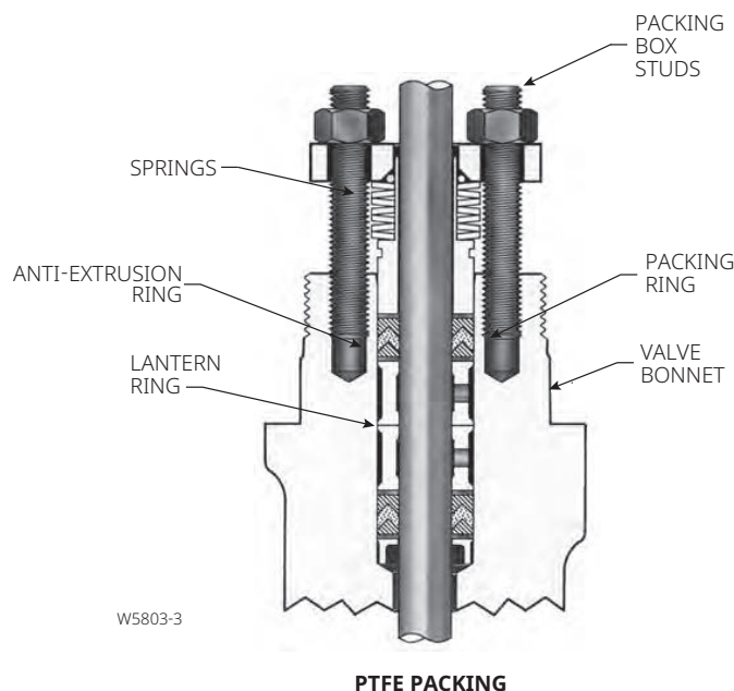
Figure 6. ENVIRO-SEAL Packing Systems
