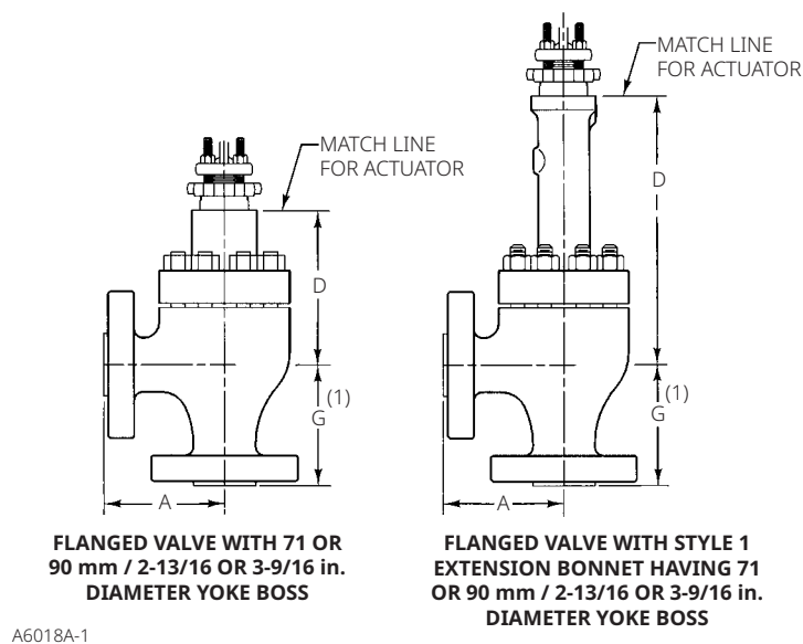
Figure 27. Angle Valve Dimensions with Standard/Style 1 Extension Bonnet (also see Tables 19 and 20)
