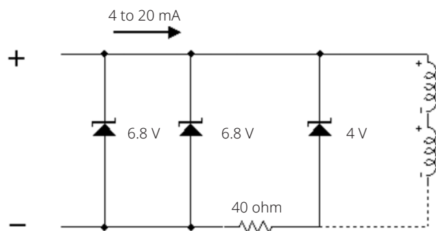
Figure 4. Equivalent Circuit
