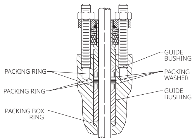
Figure 6. Enhanced ENVIRO-SEAL Graphite ULF Packing
