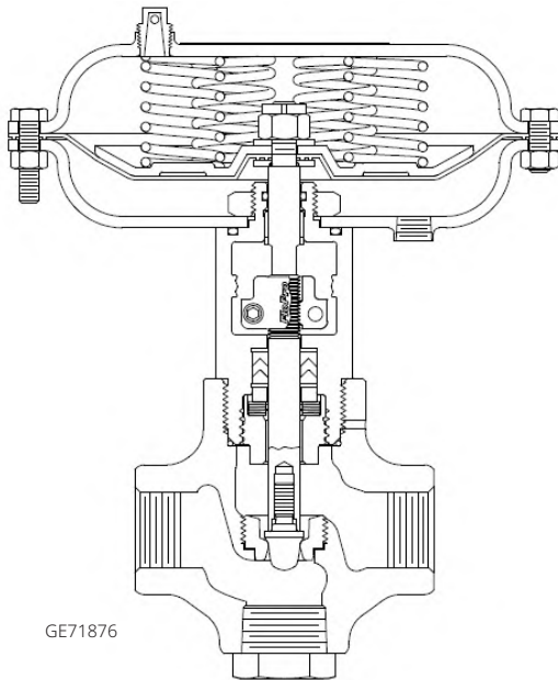
AIR-TO-OPEN
