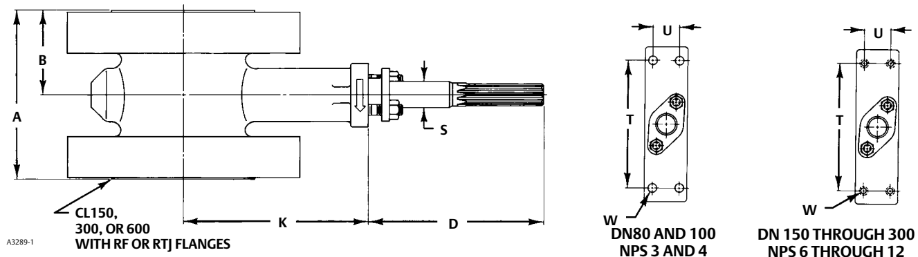
Figure 7. Fisher CV500 Valve Body Dimensions (also see table 7)
