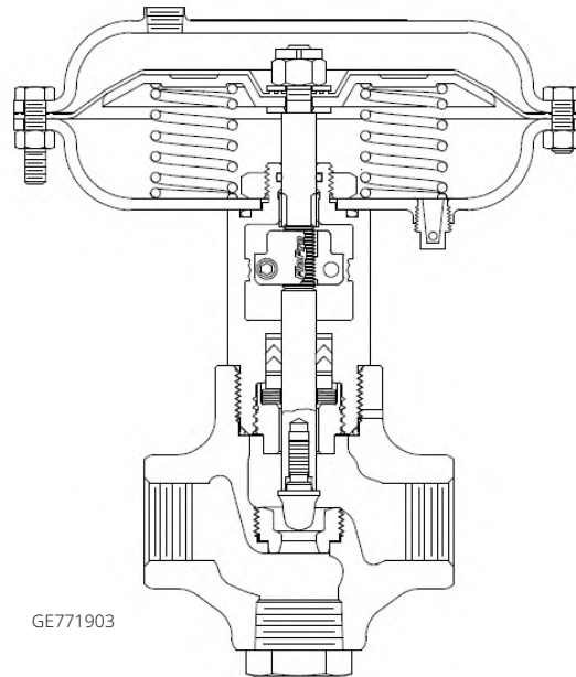
AIR-TO-CLOSE
