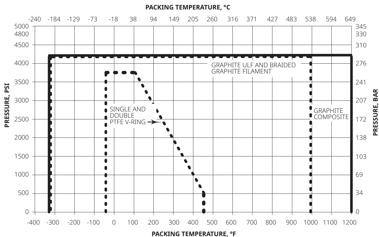
Figure 13. Applications Guidelines Chart for Services Not Requiring Fugitive Emission Control
