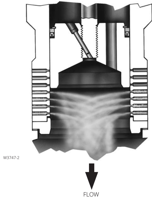
Figure 2. Operation of Cavitrol III One-Stage Trim
