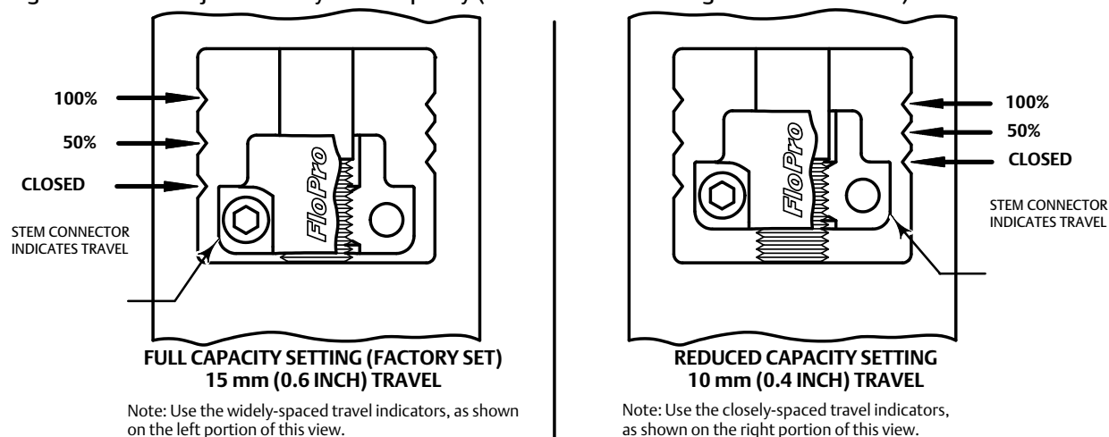
Figure 1. FloPro Adjusts to Vary Flow Capacity (Shown with Valve Plug in Seated Position)
