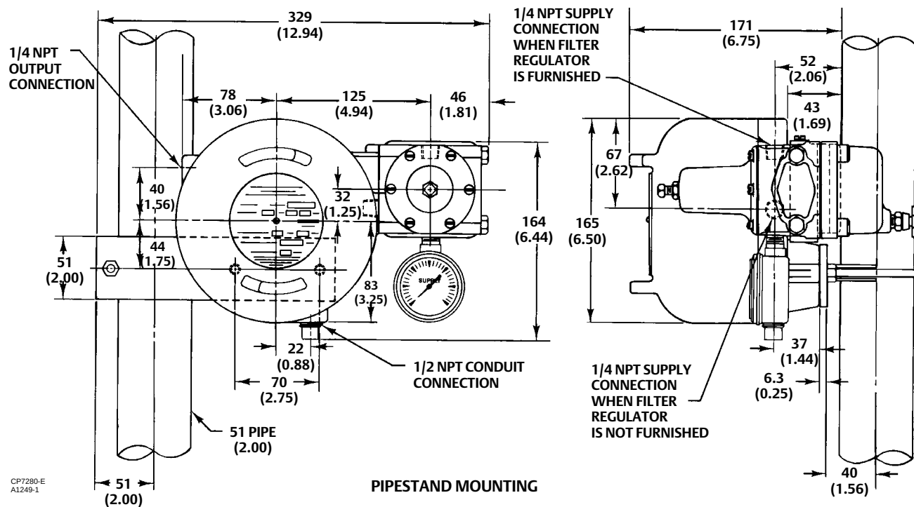
Figure 4. Dimensions
