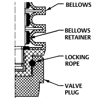
DETAIL OF HEAVY DUTY PTFE BELLOWS CONSTRUCTION
