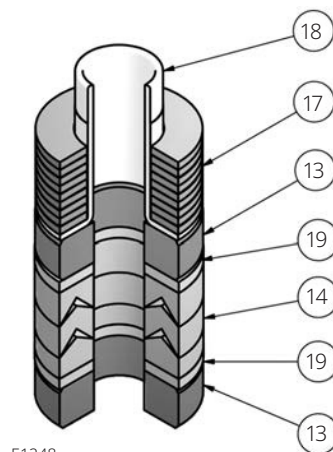
Figure 4. Fisher enhanced ENVIRO-SEAL Packing Kit (Optional for Stainless Steel Only)
