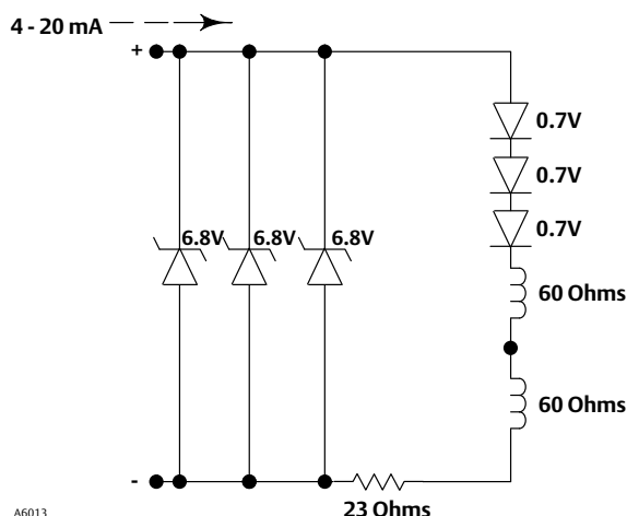
Figure 1. Equivalent Circuit
