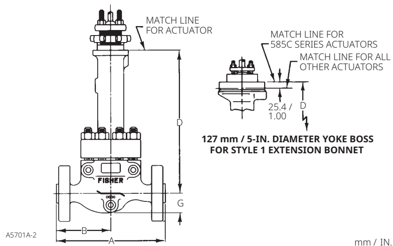
Figure 7. Valve Dimensions
