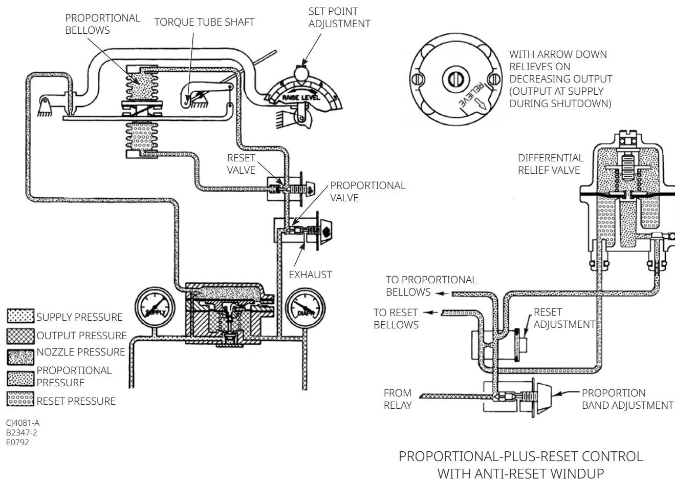
Figure 6. Schematic of Direct-Acting Proportional-Plus-Reset Controller
