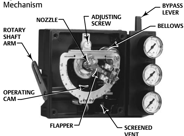
Figure 4. Fisher 3582 Pneumatic Valve Positioner Mechanism
