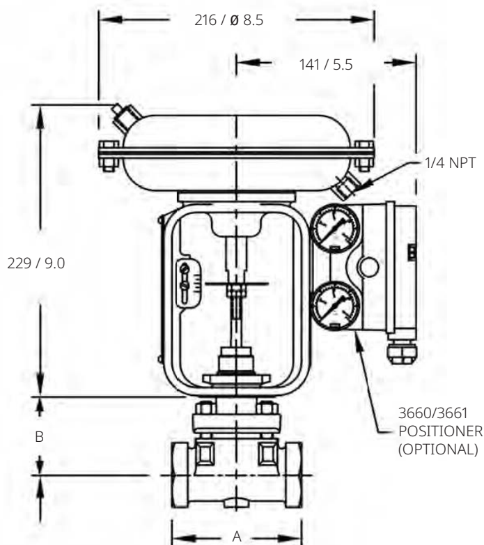
24000S WITH 32 ATO ACTUATOR
