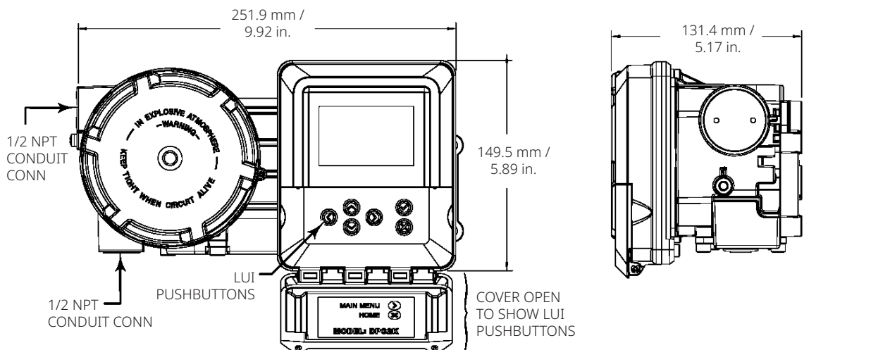
BASE UNIT WITH ANALOG OUTPUT
