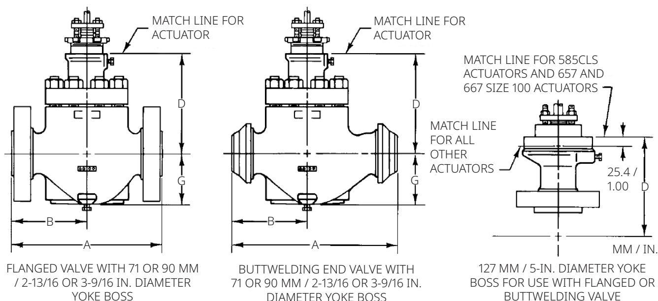
Figure 23. NPS 1-1/2 x 1 through 6 Globe Valve Dimensions with Standard Bonnet (Also See Tables 22, 23 and 24)
