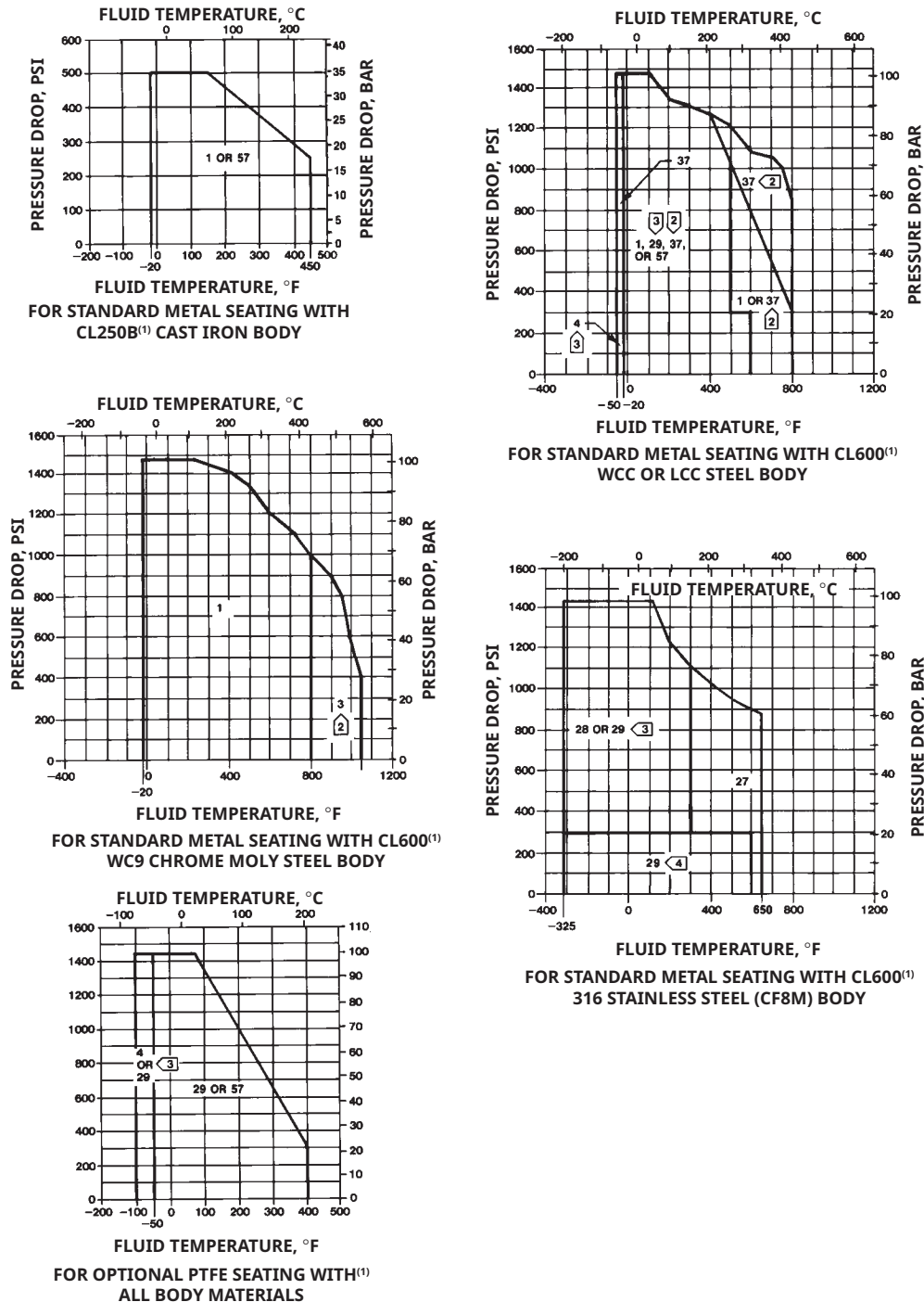
Figure 6. Typical Trim Use for All Valve Bodies Except Those for NACE Specifications
