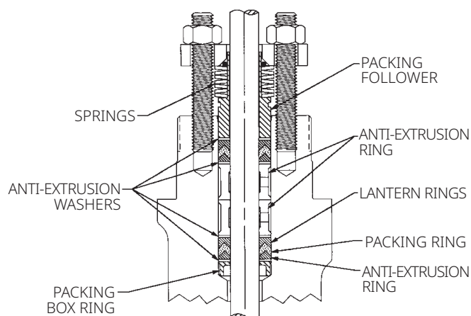
Figure 3. Enhanced ENVIRO-SEAL PTFE Packing
