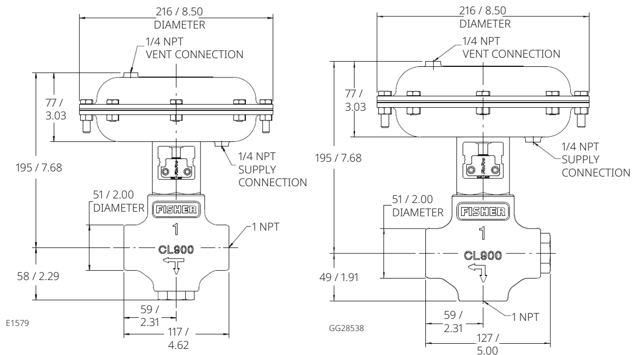
Figure 5. Fisher D2T Valve Dimensions (Air-to-Open Configuration Shown)
