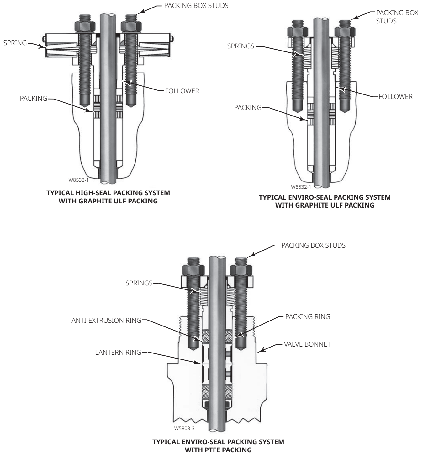
Figure 10. ENVIRO-SEAL and HIGH-SEAL Packing Systems
