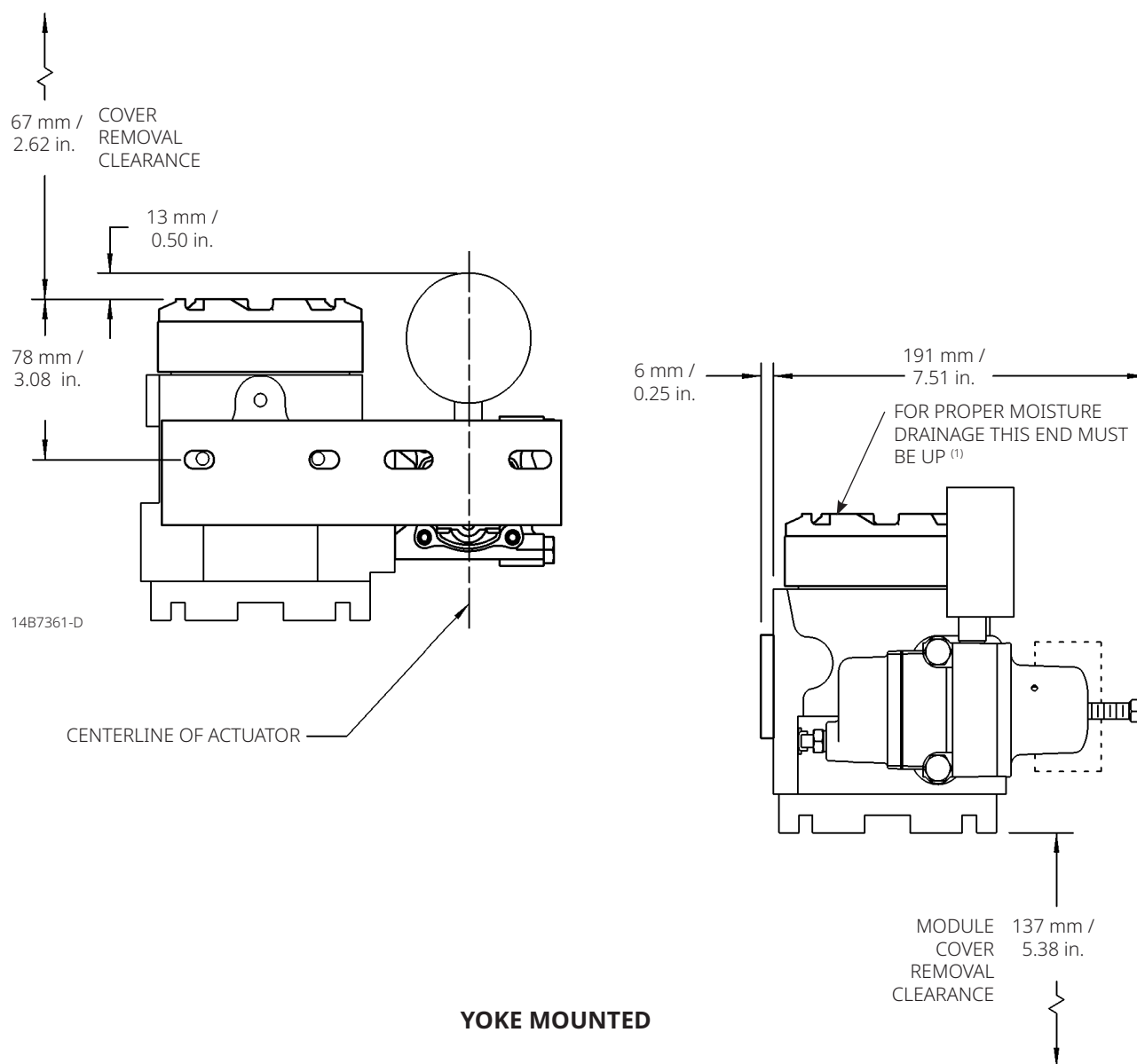
Figure 7. Dimensions with Optional Fisher 67CFR Filter-Regulator (Yoke Mounted)
