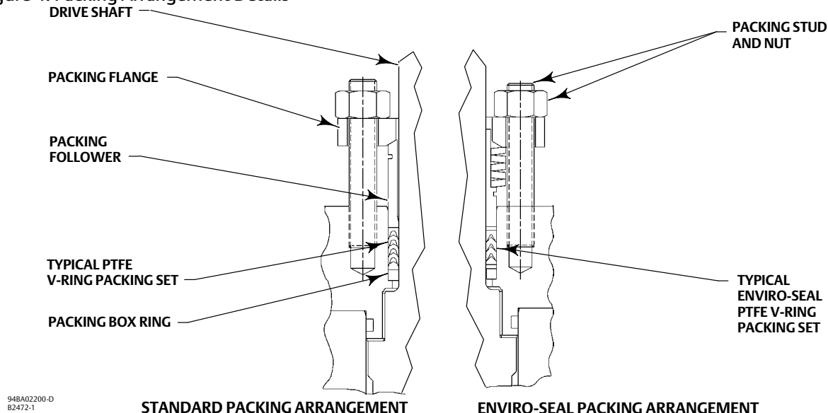
Figure 4. Packing Arrangement Details
