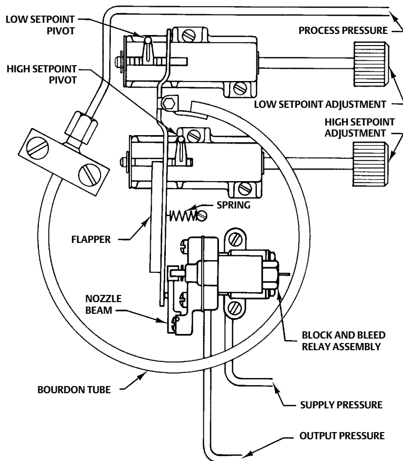
Figure 3. Principle of Operation Schematic
