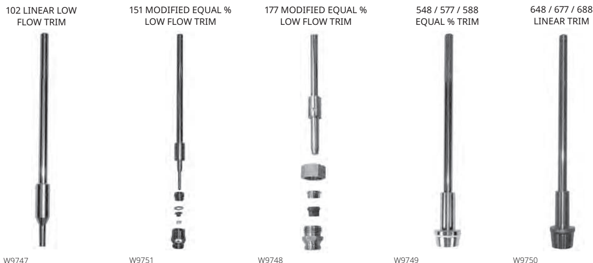
Figure 9. Fisher Baumann 24000SB Trims
