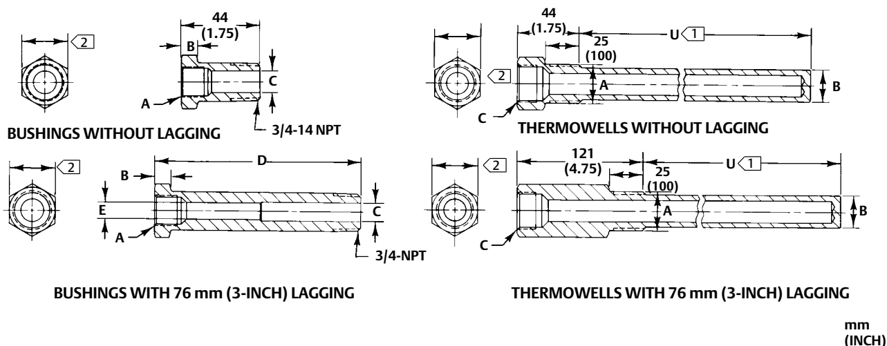
Figure 7. Bushing and Thermowell Dimensions (also see tables 6 and 7)
