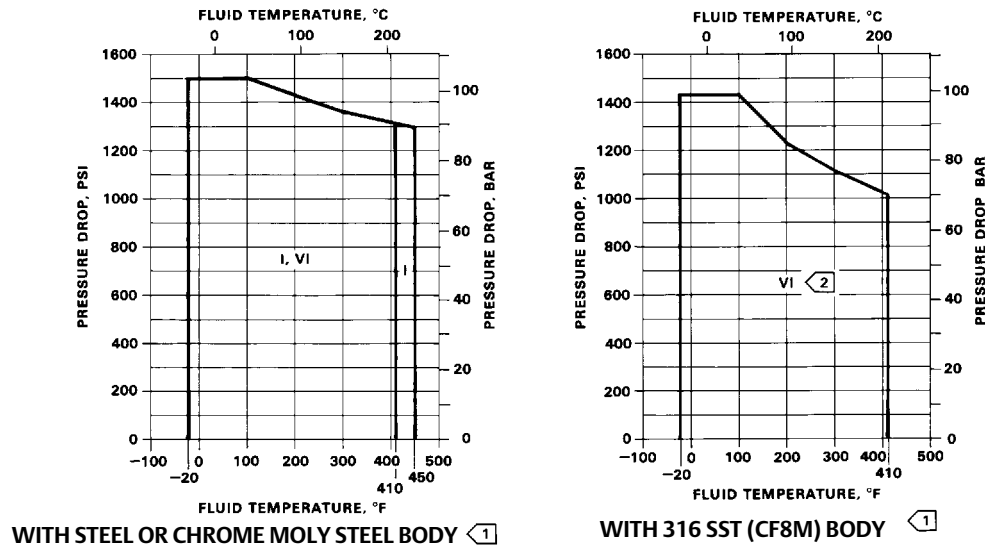
Figure 4. Typical Trim Use in Fisher EWNT-2 Valve Bodies
