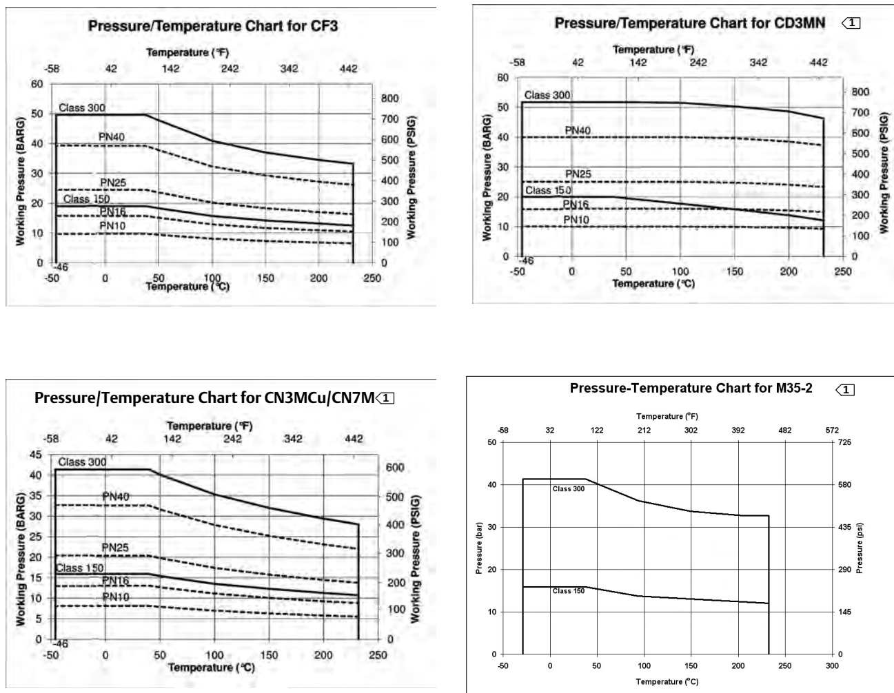
Figure 10. Material Pressure/Temperature Curves
