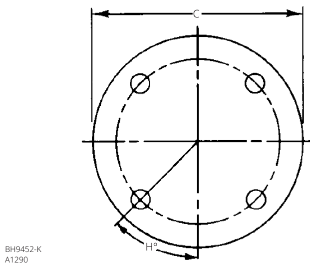
Figure 6. Cylinder Diameter and Bolt Center Location, All Actuators (refer to Table 3)
