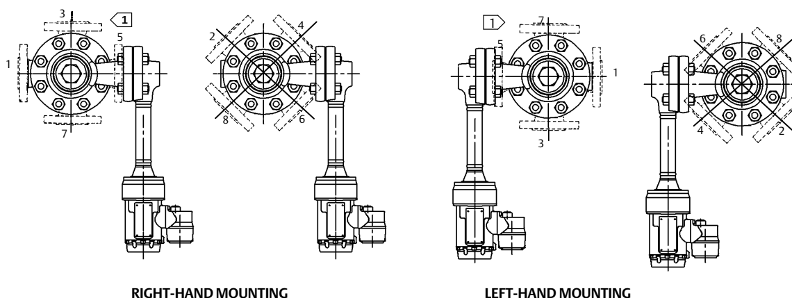
Figure 10. Mounting Positions—Caged Displacers
