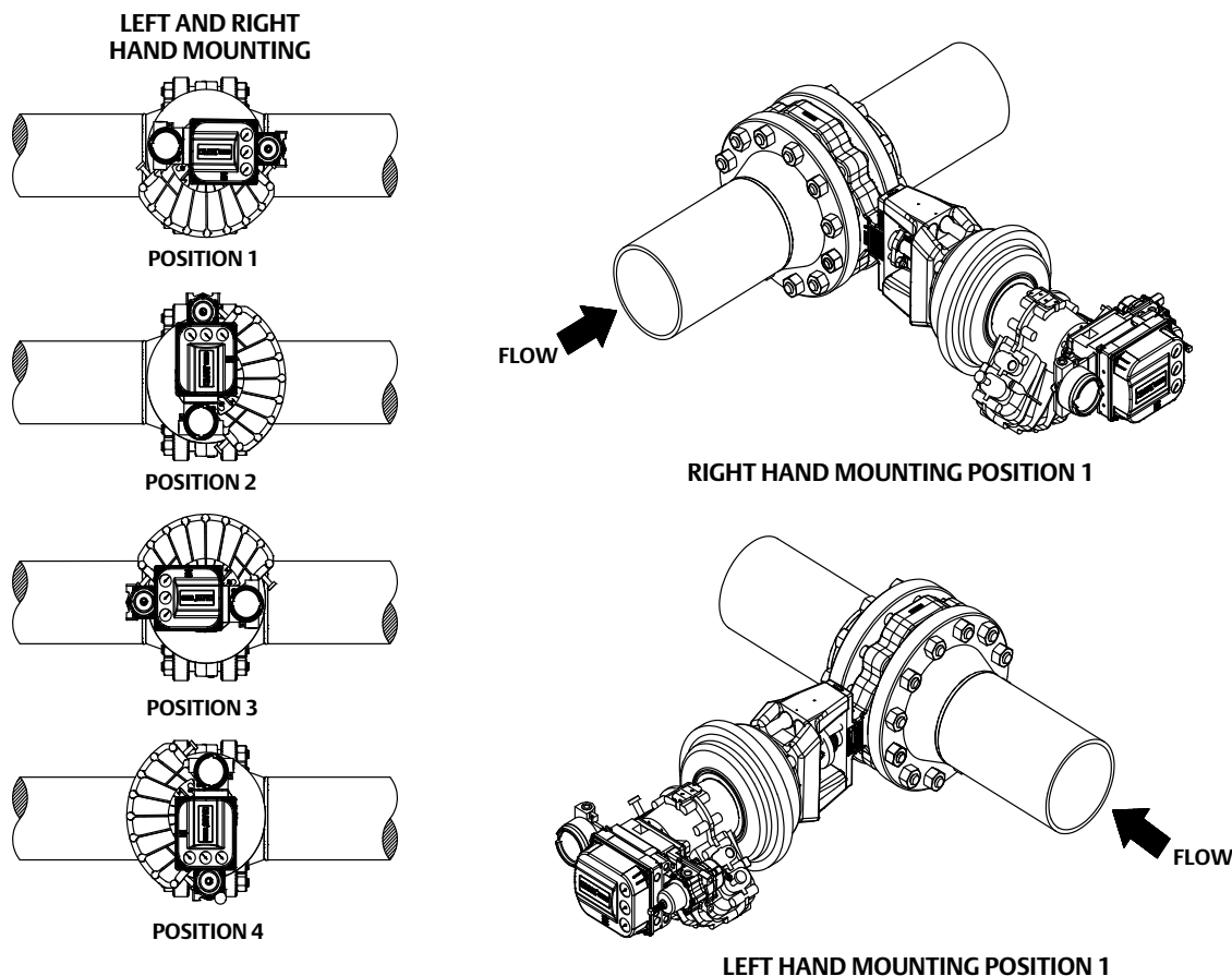
Figure 5. 1068 Actuator Mounting
