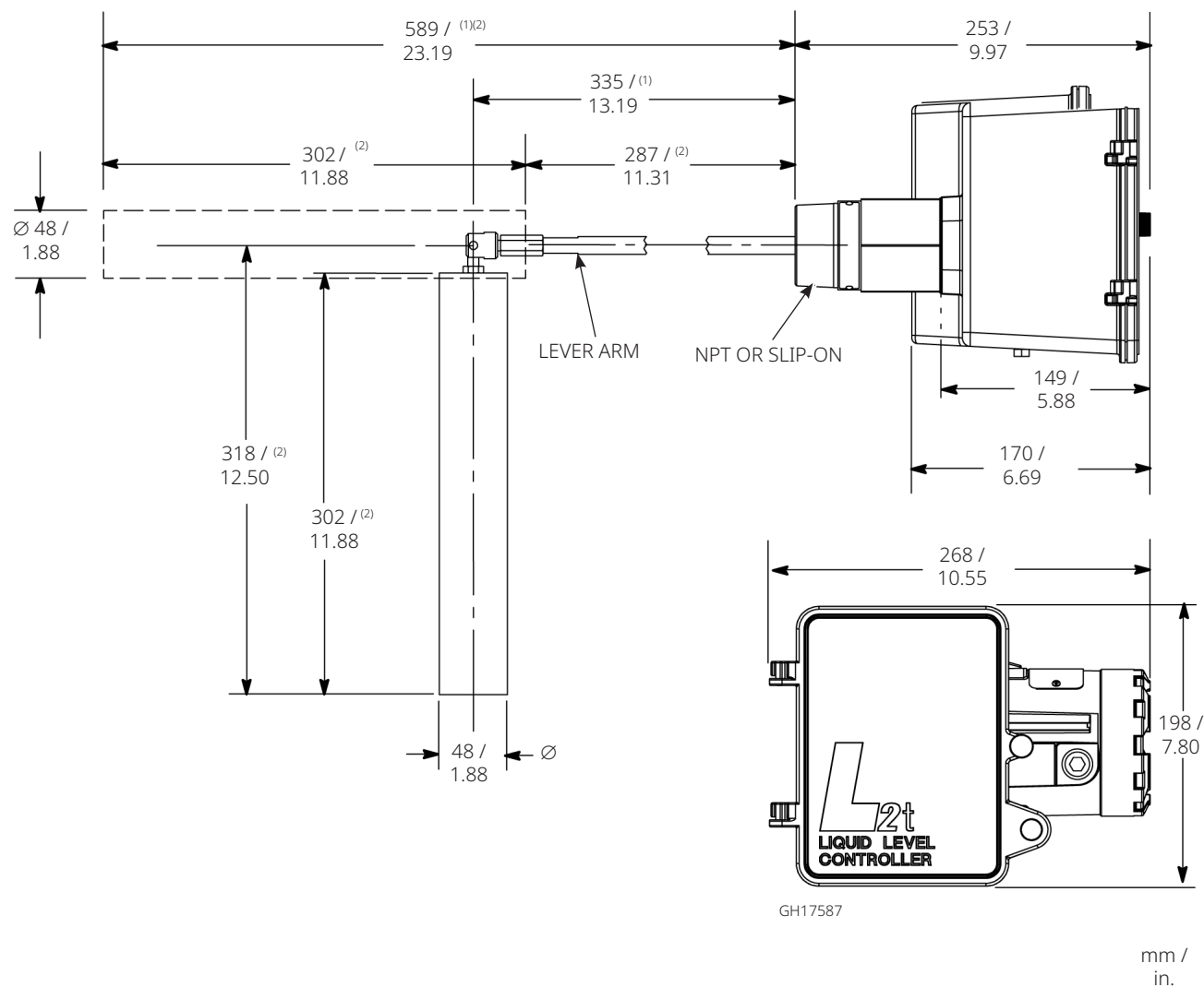
Figure 2. Dimensions
