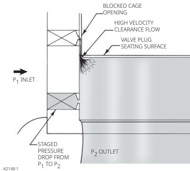
Figure 3. Standard Cage-Style Anti-Cavitation Trim
