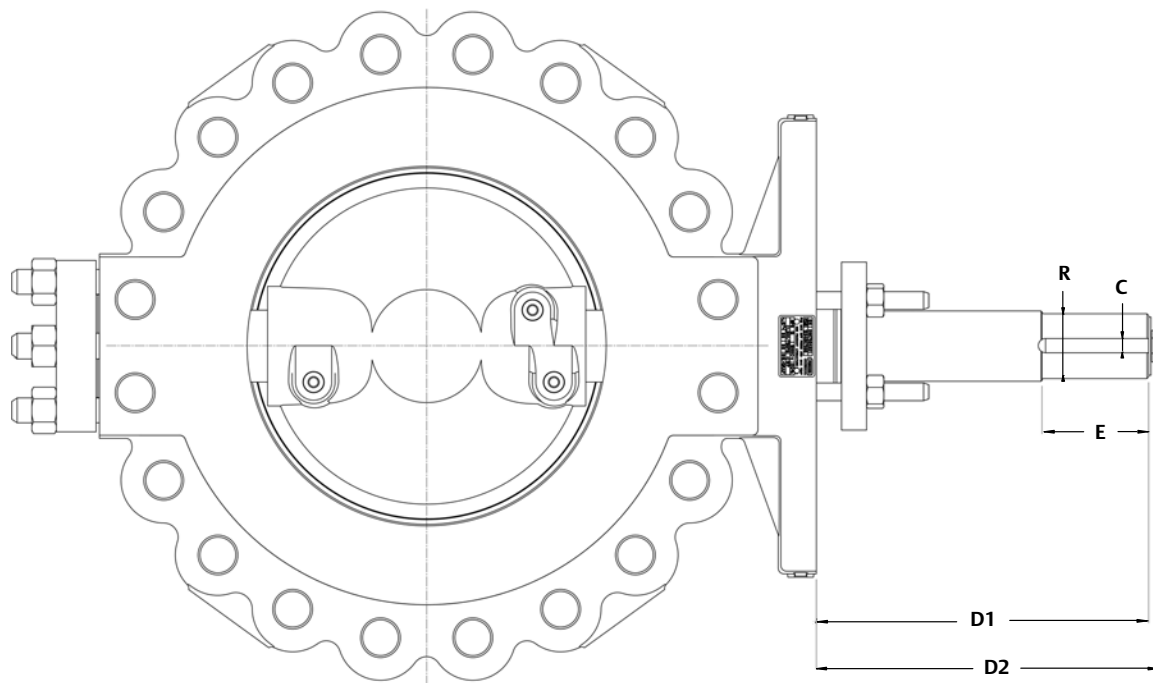
Figure 9. Dimensions for Fisher 8590 NPS 14 to 24 Valve with Keyed Shaft (also see table 9)
