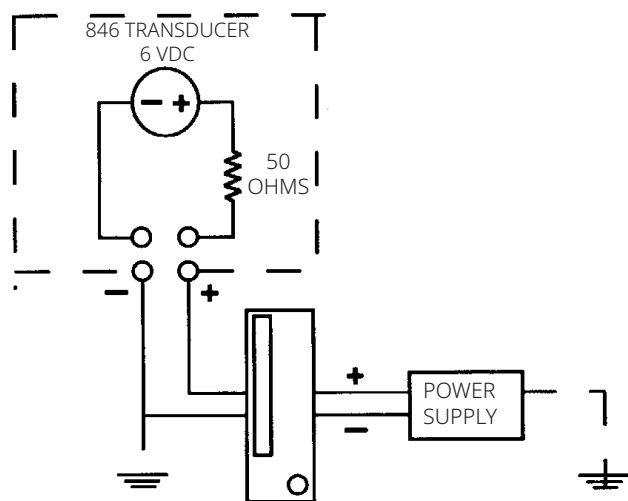
Figure 5. Equivalent Circuit
