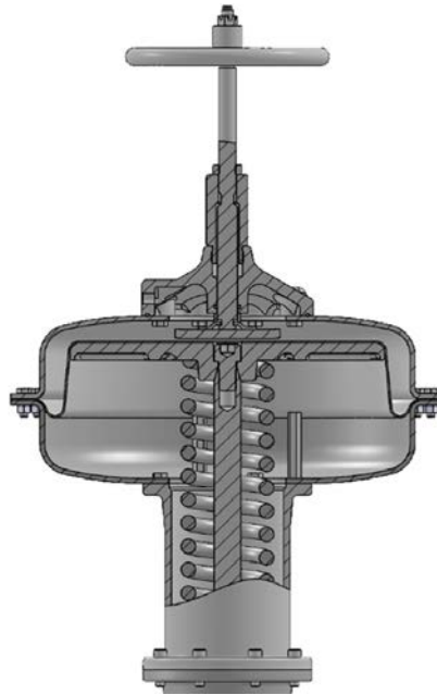
Figure 3. Fisher 657C Series Top-Mounted Handwheel
