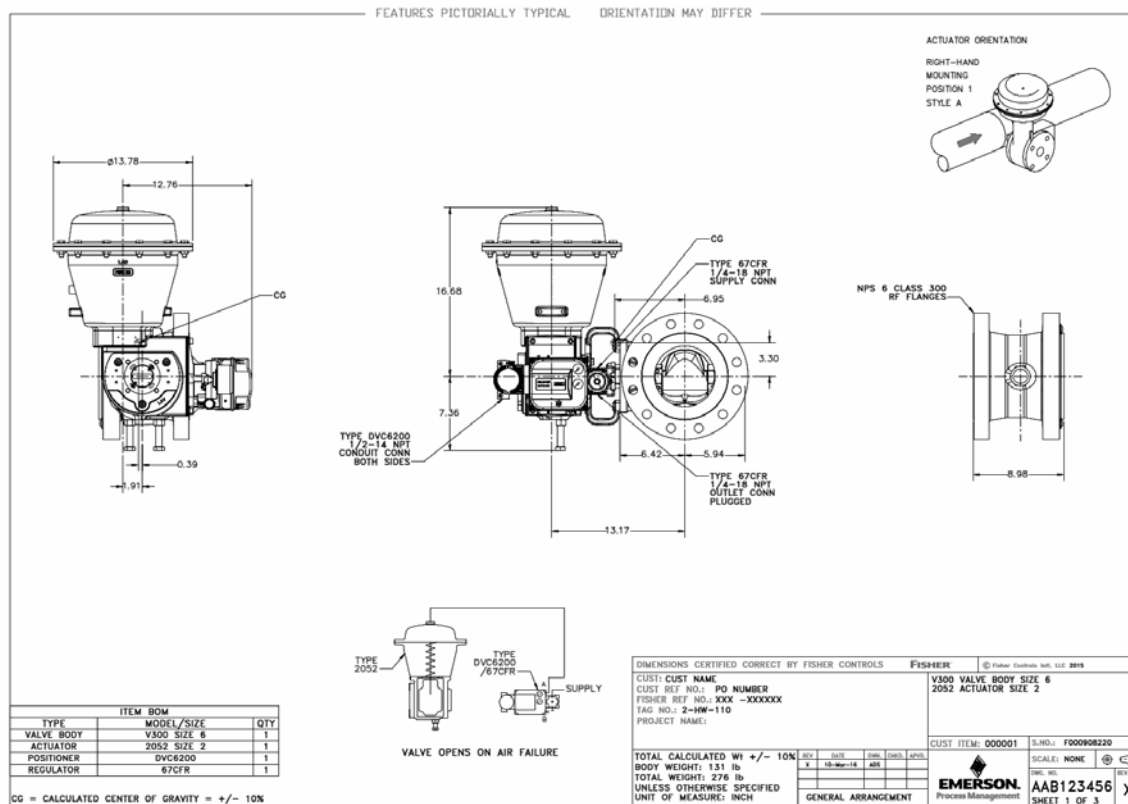
Figure 13. LEVEL 3 Drawing - Rotary (Sheets 1 and 2)
