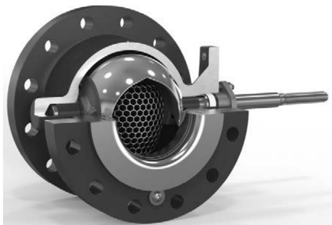
Figure 8. Fisher NPS 6 V300 Cutaway Image with Optional Cavitrol Hex Anti-Cavitation Trim
