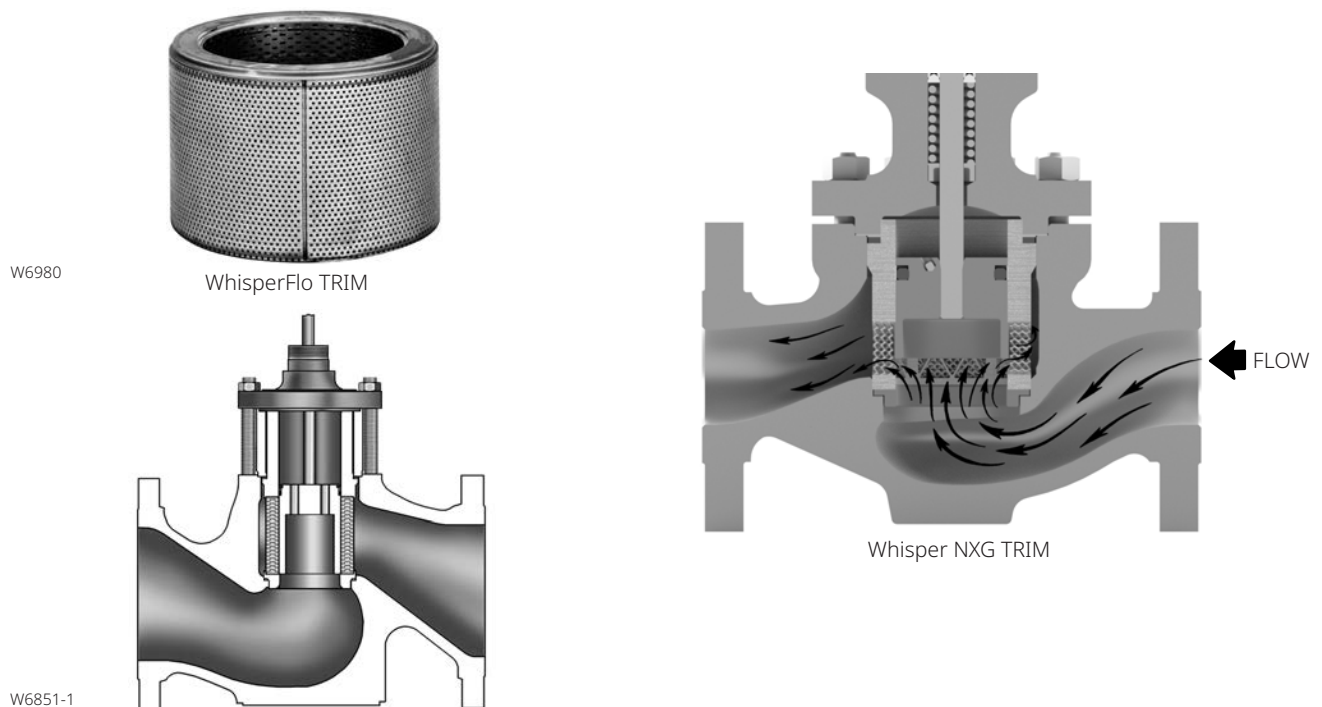
Figure 5. Typical Valve with WhisperFlo Aerodynamic or Whisper NXG Trim
