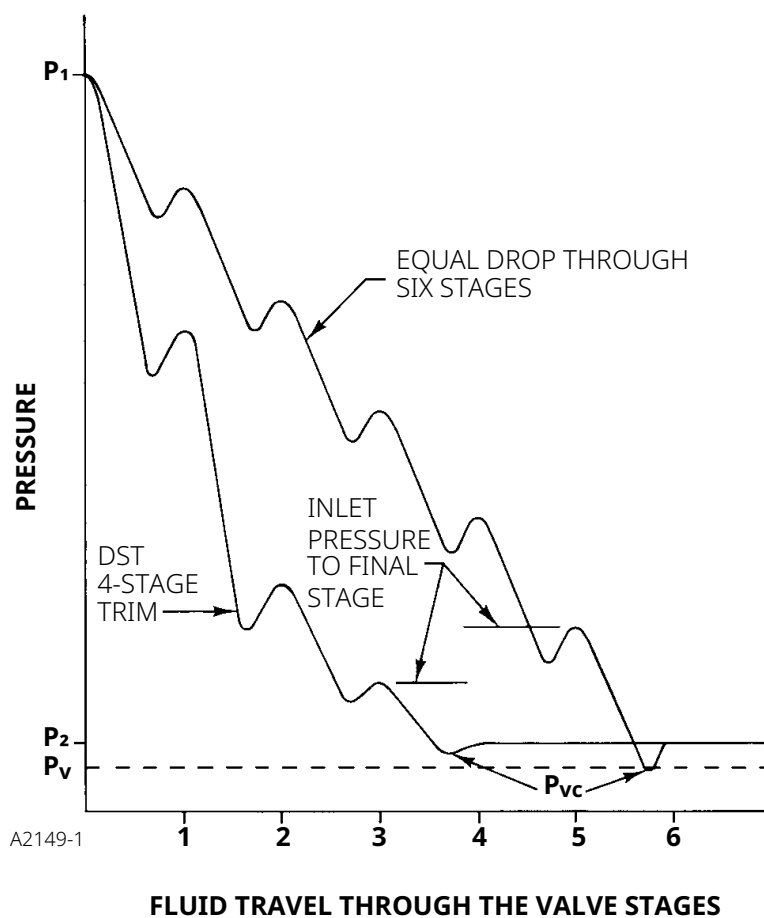
Figure 2. Staged Pressure Drop Patterns
