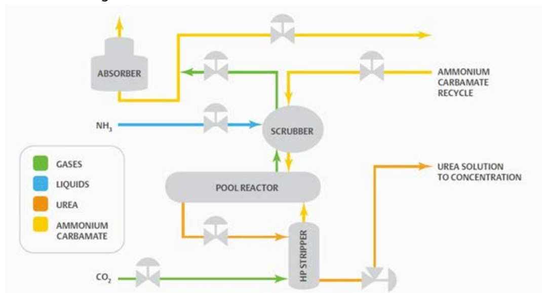
Figure 4. Process Diagram
