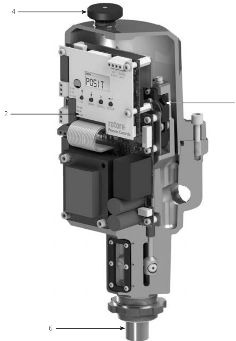
Figure 4. CML Linear Actuator Key Actuation Components
