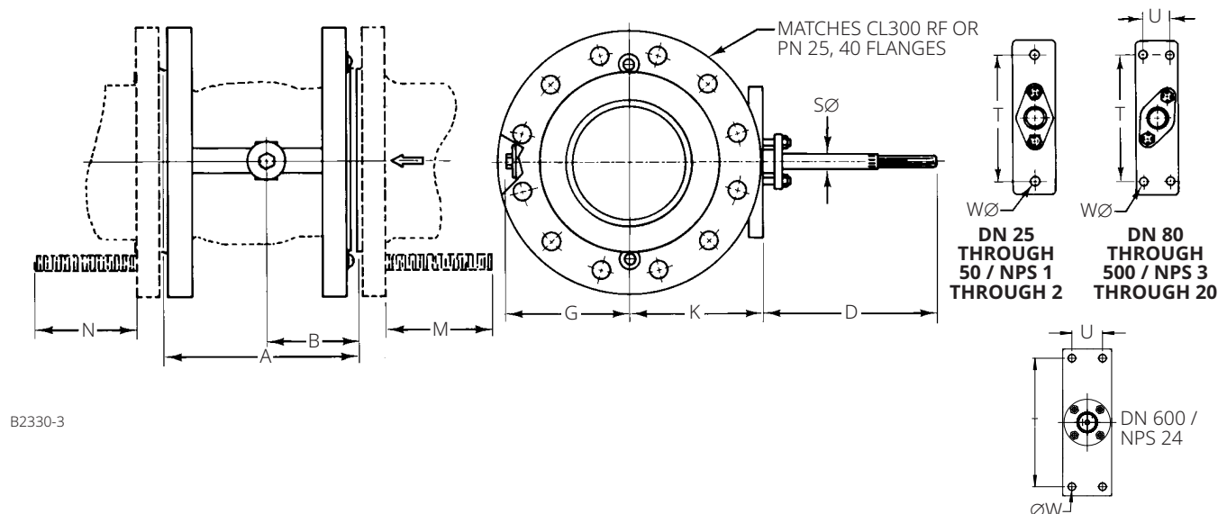
Figure 17. Fisher V300 Dimensions (also see Table 14)
