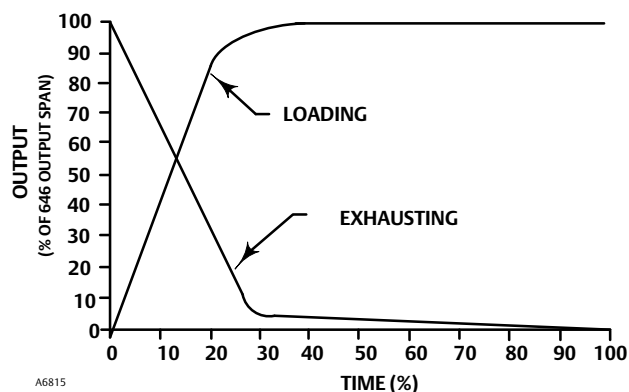
Figure 2. Output-Time Relationships
