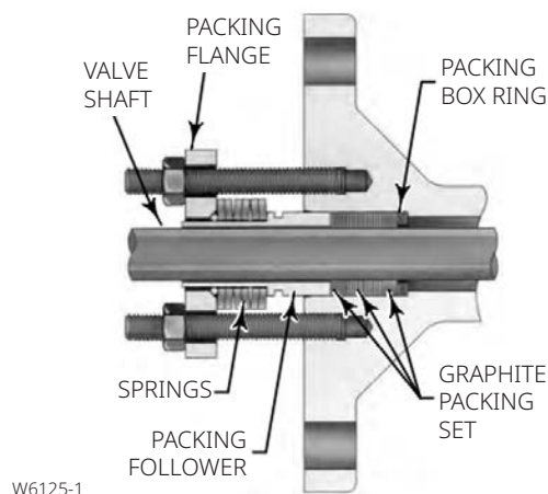
Figure 4. enhanced ENVIRO-SEAL Graphite ULF Packing
