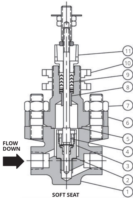
Figure 2. NPS 1/4 and 1/2 / 6.35 and 12.7 mm Soft Seat Cage Design for C_v = 0.00013 to 0.45 Class VI Shutoff (N10276 Nickel Alloy Construction Available)
