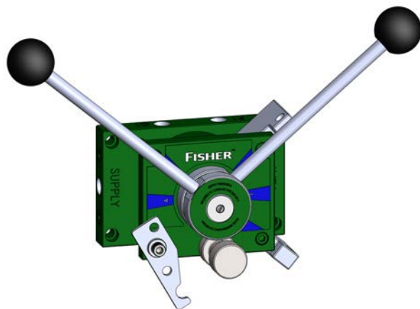
MANUAL CLOSE MODE: VALVE IS CLOSING
