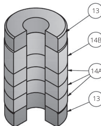
Figure 4. Molded Graphite (Flexible Graphite) Packing Kit (Optional)
