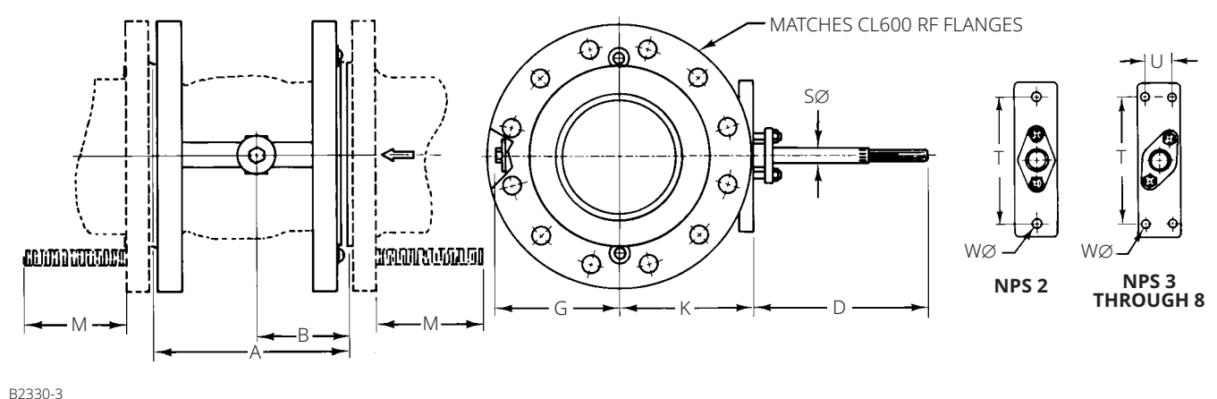
Figure 16. Fisher V200 CL600 Flanged Dimensions (also see Table 13)
