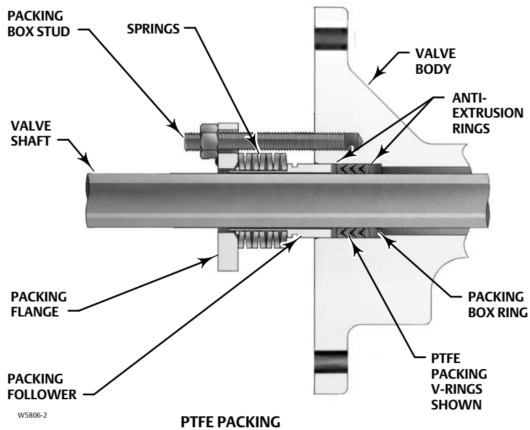
Figure 2. Typical ENVIRO-SEAL Packing Arrangements
