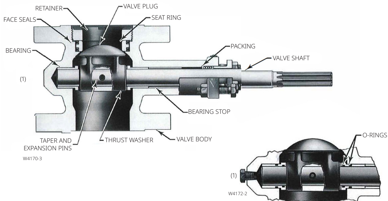
Figure 1. Sectional of Fisher V500 Control Valve
