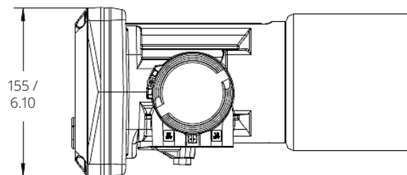
SIDE VIEW WITH HEAT INSULATOR
