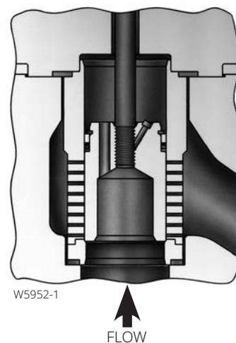
Figure 18. Fisher HPT Trim with Whisper Trim III Level A1 Cage (also available in HPD NPS 2 to 6 and HPS NPS 2 and 3)
