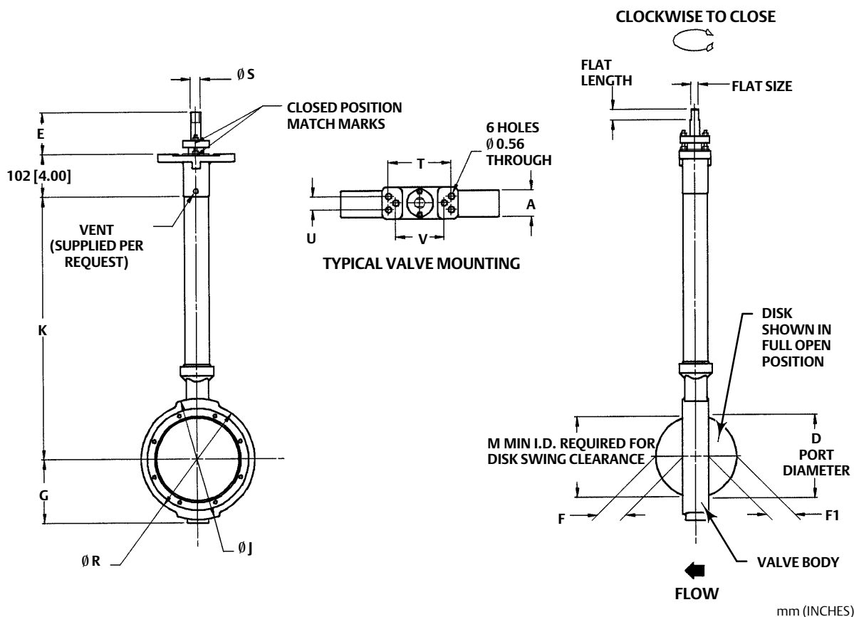
Figure 5. Dimensions, Wafer Style Valves, CL150, NPS 3 through 8 (also see table 3)
