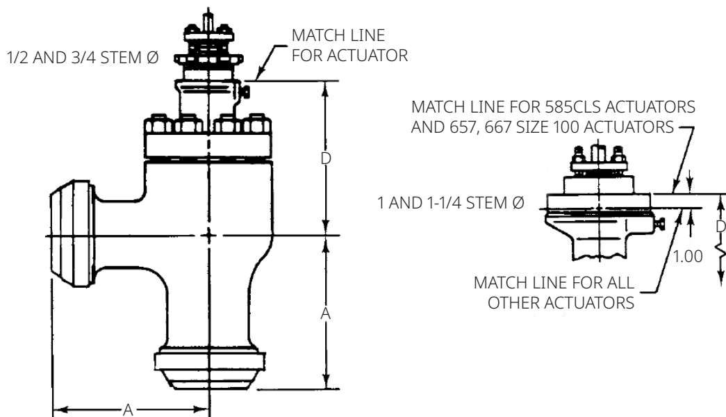
Figure 25. NPS 1 through 6 Angle Valve CL2500 Dimensions with Standard Bonnet and Style 1 Extension Bonnet (Also See Table 26)
