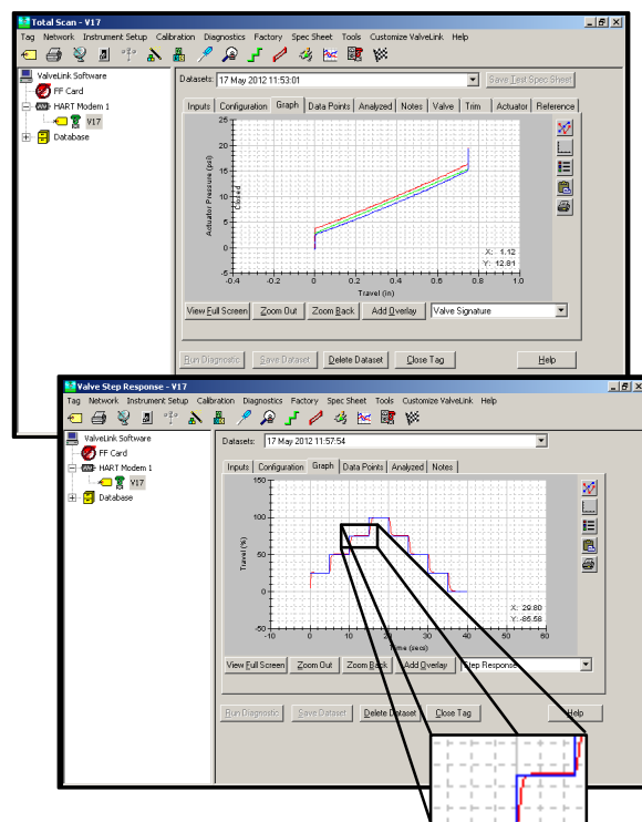
Figure 2. Performing a Diagnostic Test with ValveLink Software Provides an Analysis of Control Valve Operating Parameters
