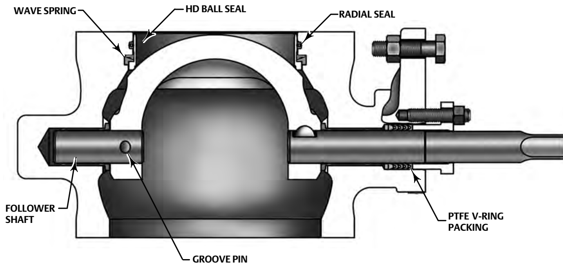
Figure 3. Fisher V200U Construction Features, DN 150 through DN 250 (NPS 6 through 10)
