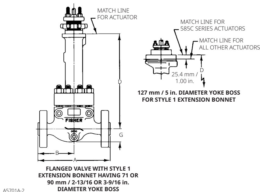
Figure 26. Dimensions D for Style 1 Extension Bonnet (A, B and G Dimensions Listed in Figure 25 Do Not Change When Extension Bonnet is Used) (also see Table 17)
