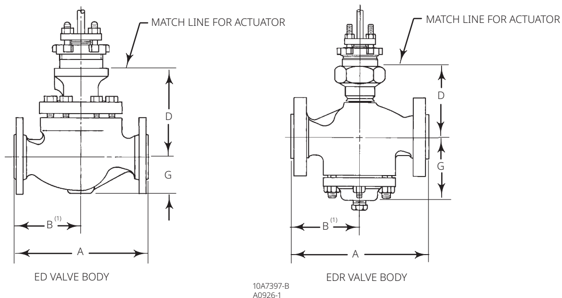
Figure 13. Fisher ED and EDR Dimensions (also see Tables 14, 15 and 16)
