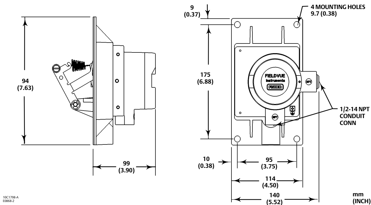
Figure 4. FIELDVUE DVC6025 Feedback Unit; Rotary and Long-Stroke Sliding-Stem Actuator Mounting
