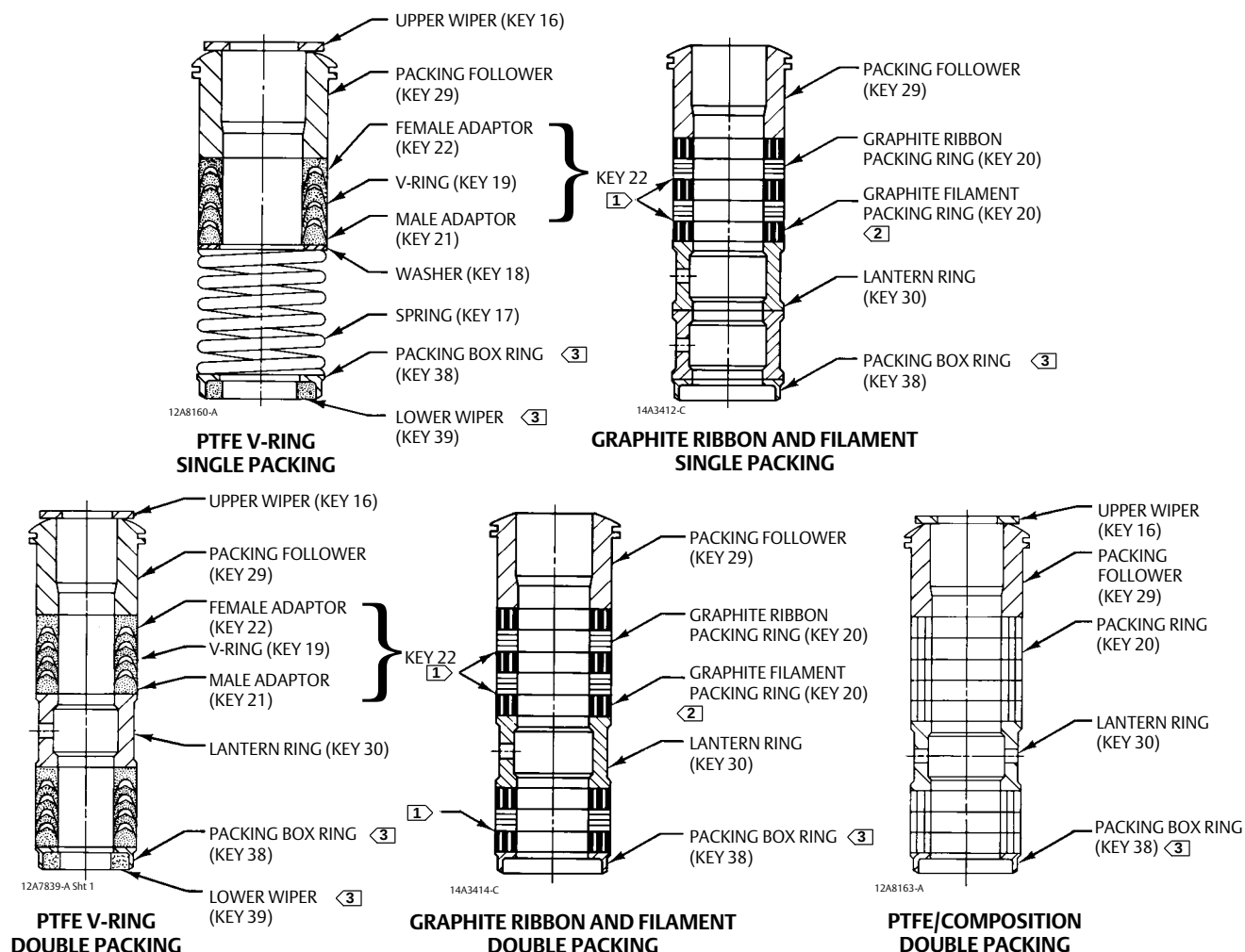
Figure 5. Packing Arrangements
