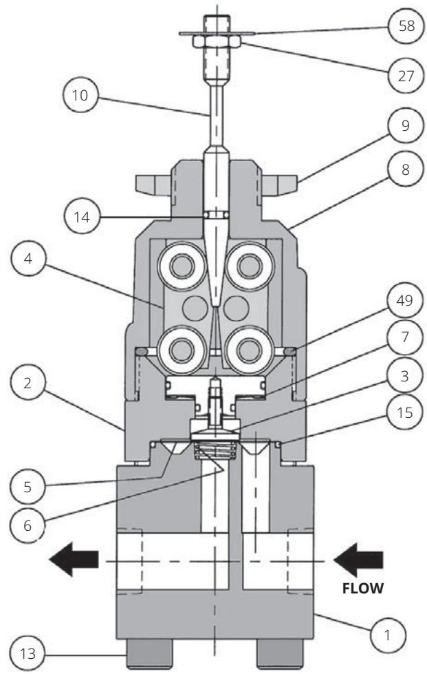
Figure 3. Fisher Baumann 81000 NPS 1/2 Inline Valve Body
