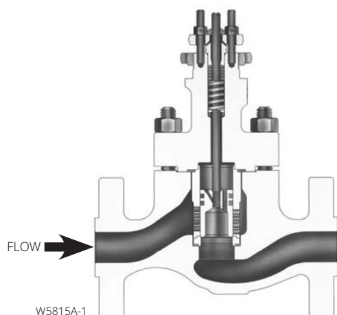
Figure 2. Fisher HPD Valve Assembly, NPS 2 to 6
