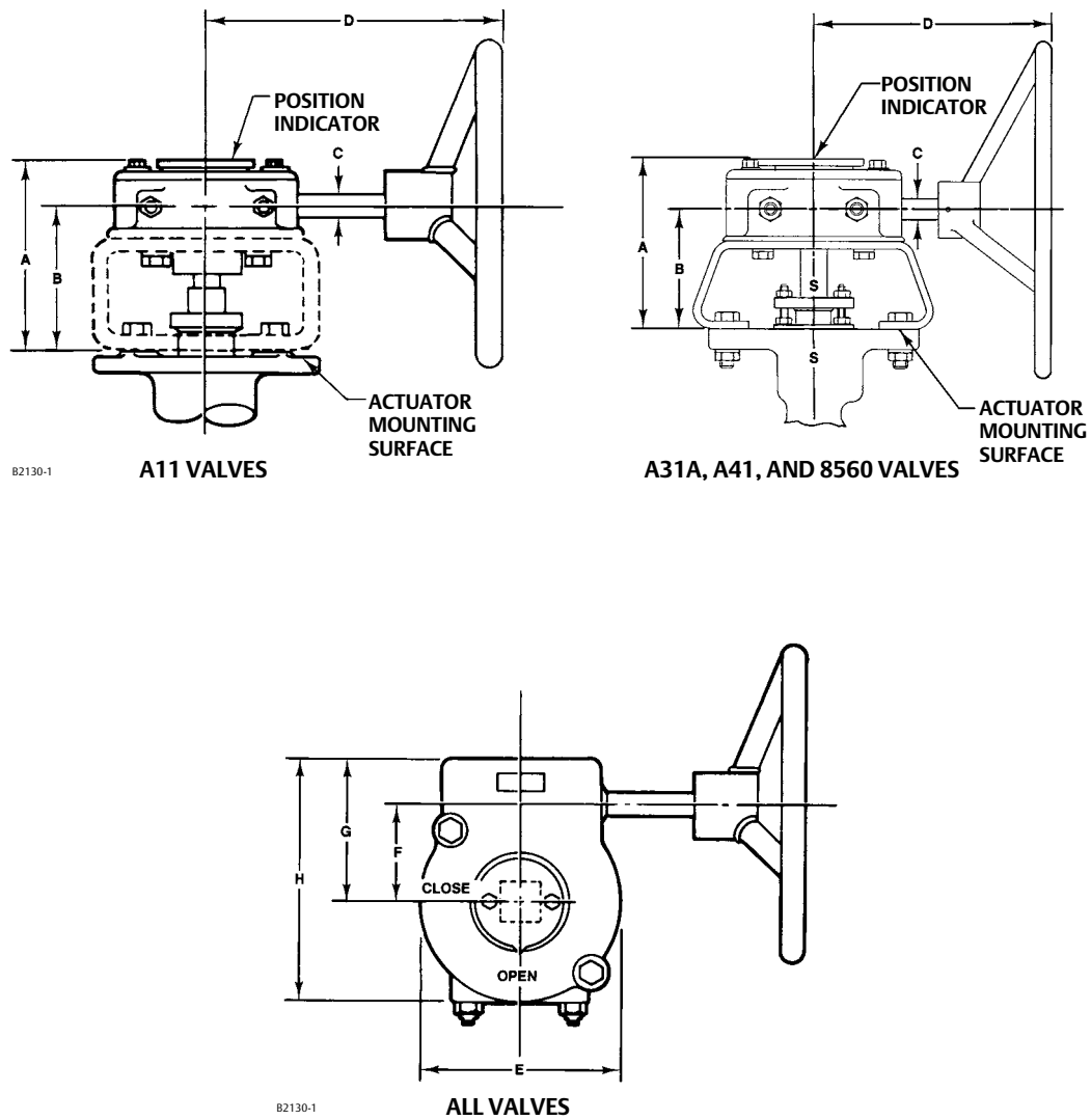
Figure 2. M Series Dimensions (also see tables 4 and 5)
