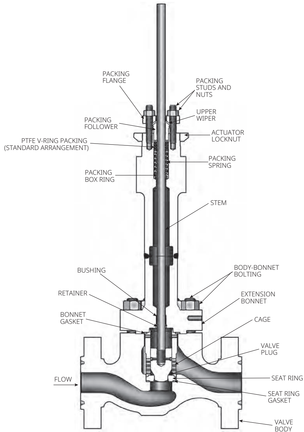
Figure 5. Fisher HPS-C Valve Assembly Detail NPS 1 through 3
