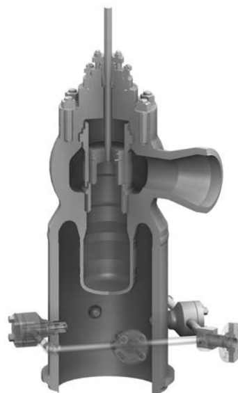
FISHER CVX STEAM CONDITIONING VALVE
