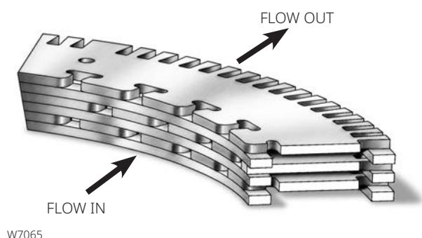
Figure 5. Typical WhisperFlo Trim Cut Section View for Fisher HP Valve
