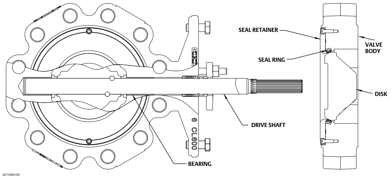
Figure 2. 8590, NPS 3 to 8, Valve Body Assembly
