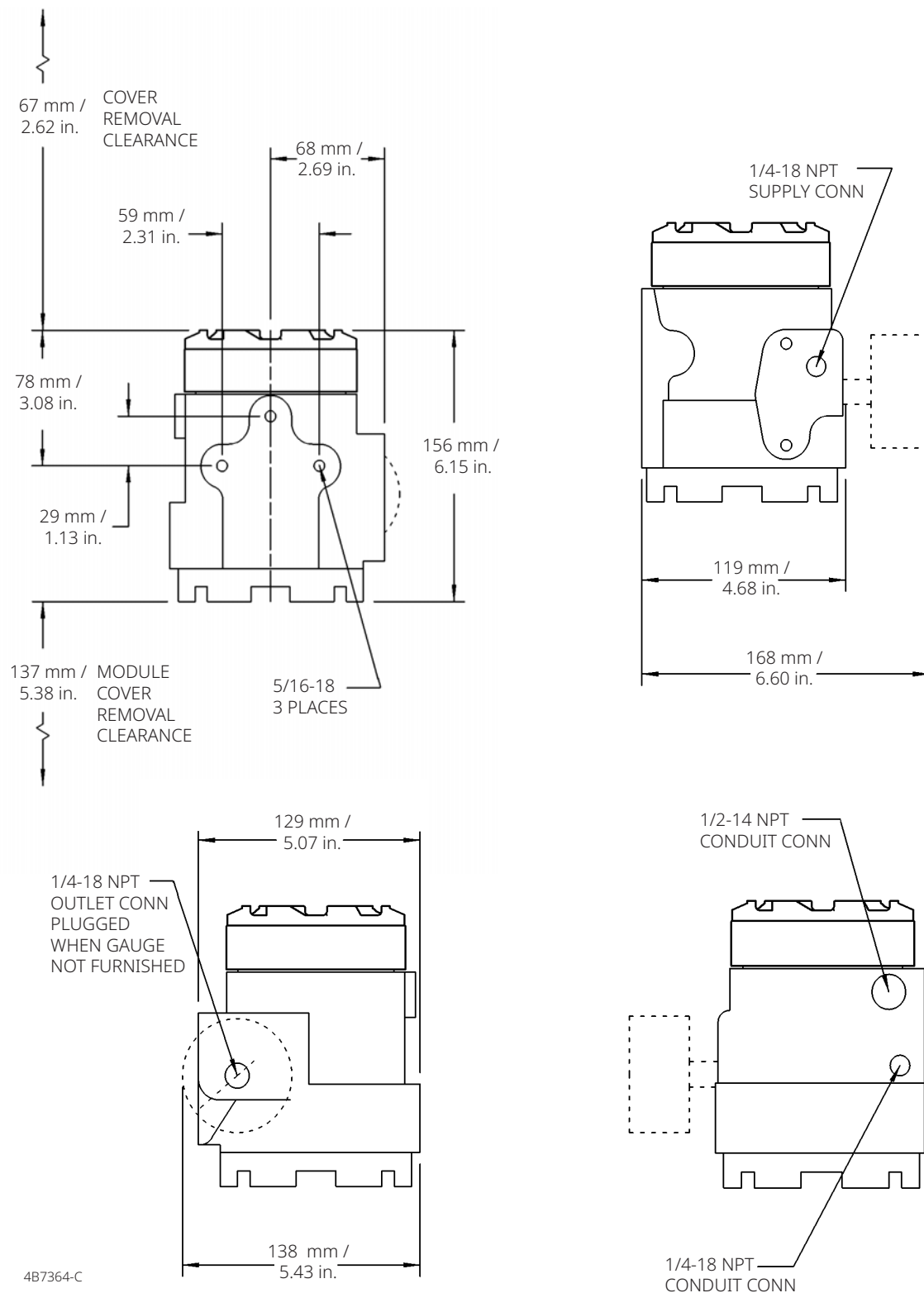
Figure 6. Dimensions
