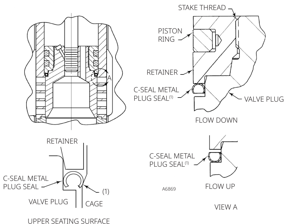
Figure 17. C-seal Trim
