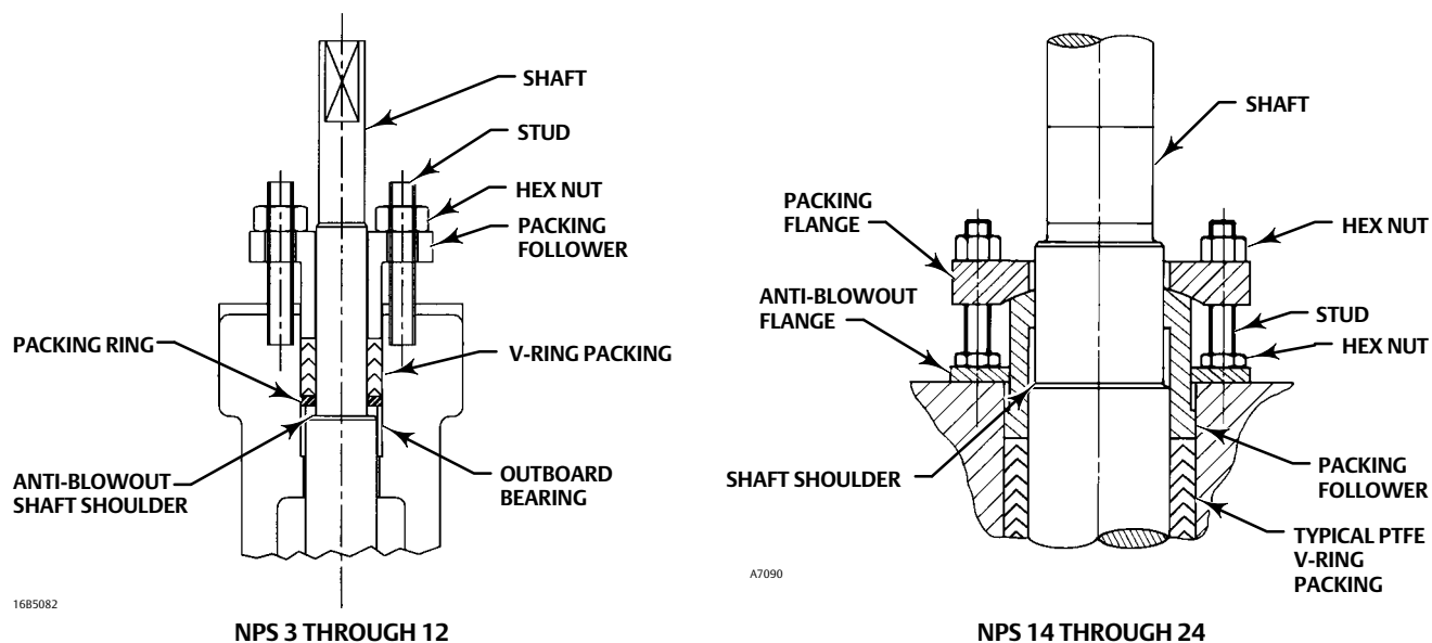
Figure 4. Anti-Blowout Protection
