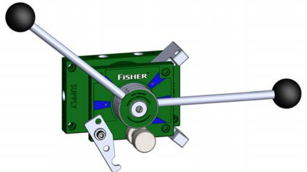
MANUAL LOCK MODE: VALVE IS LOCKED IN CURRENT POSITION
