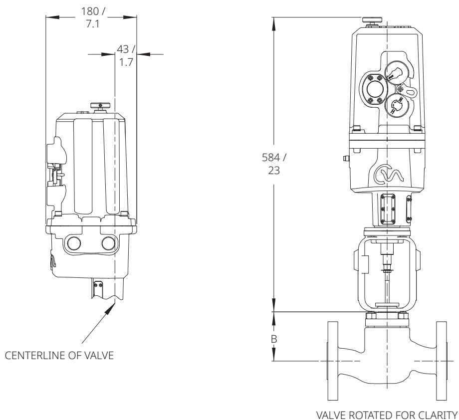
Figure 2. CML-250 Dimensions
