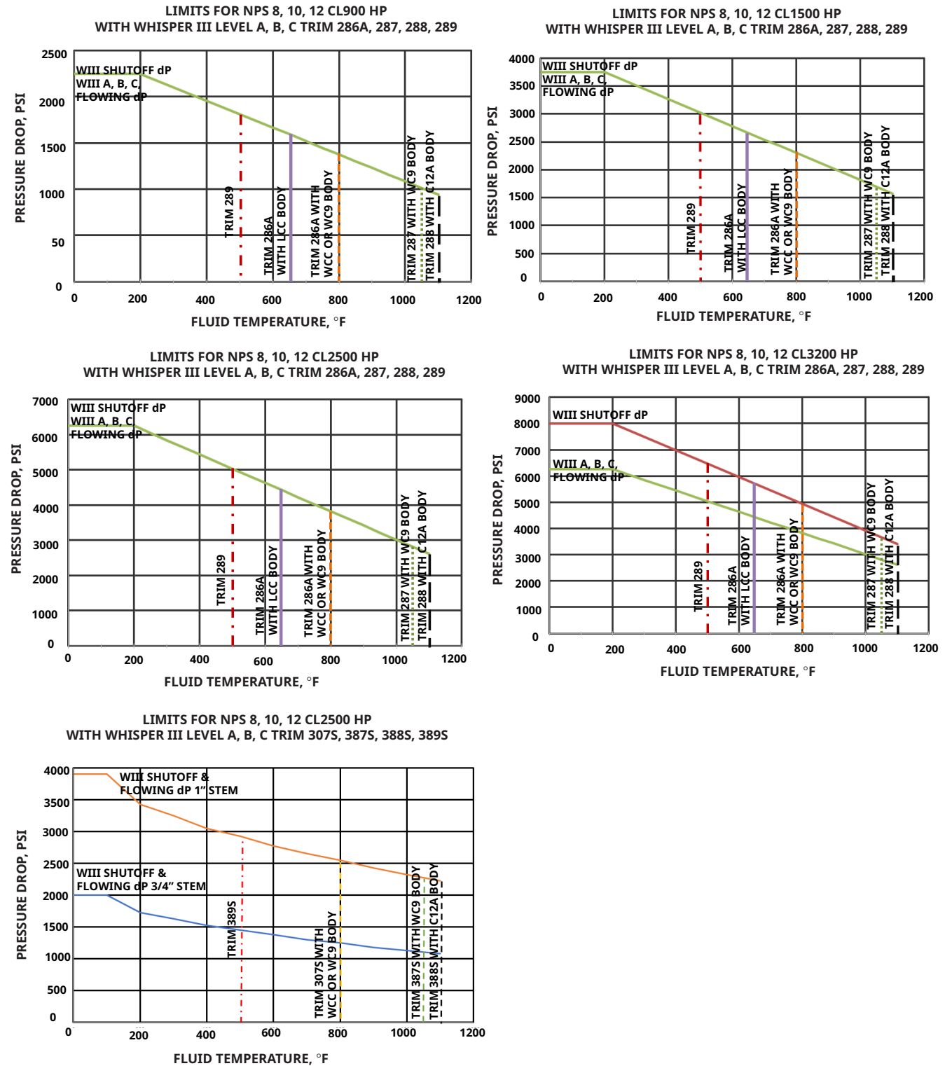
Figure 23. Pressure-Temperature Limits for Whisper III A, B, C Cage (also refer to Table 7)
