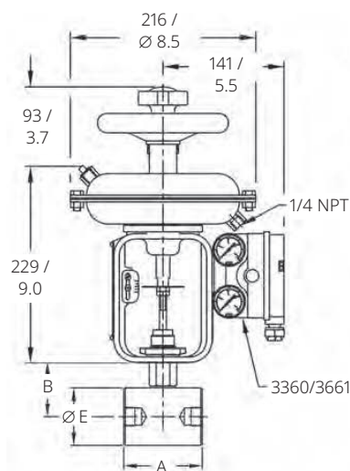
THREADED (NPT) VALVE BODY (VALVE ROTATED 90° FOR CLARITY) 32 ATO / FAIL CLOSE WITH HANDWHEEL
