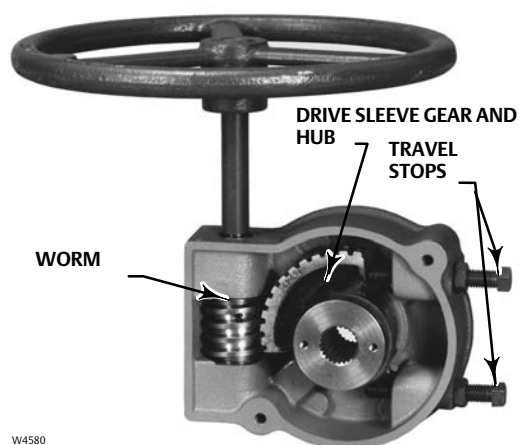
Figure 1. Gearbox Subassembly
