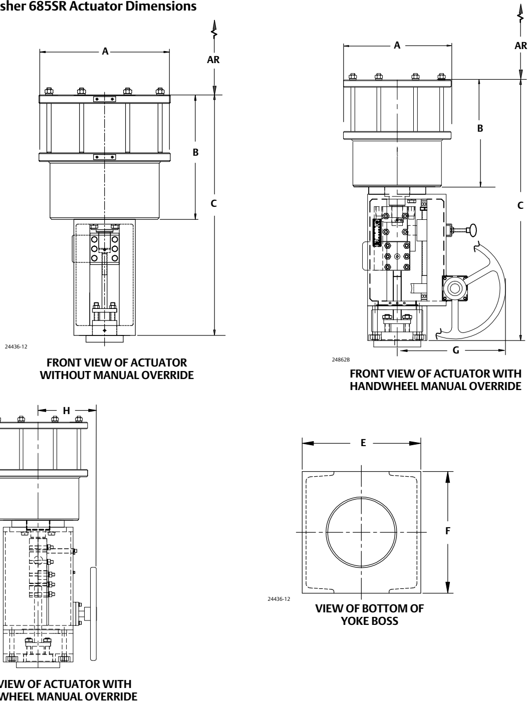
Figure 3. Fisher 685SR Actuator Dimensions
