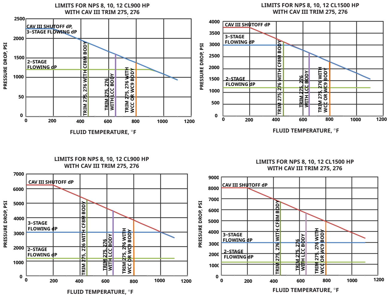
Figure 22. Pressure-Temperature Limits for Cavitrol III Cage (also refer to Table 7)
