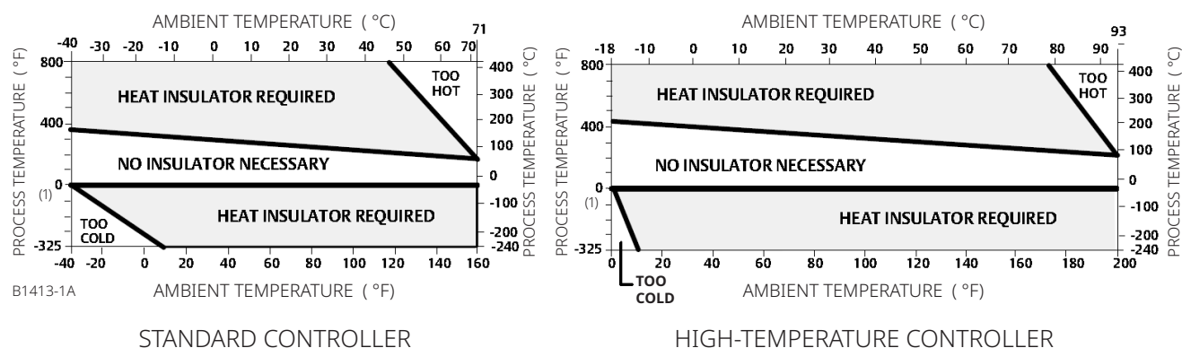
Figure 4. Guidelines for Use of Optional Heat Insulator Assembly
