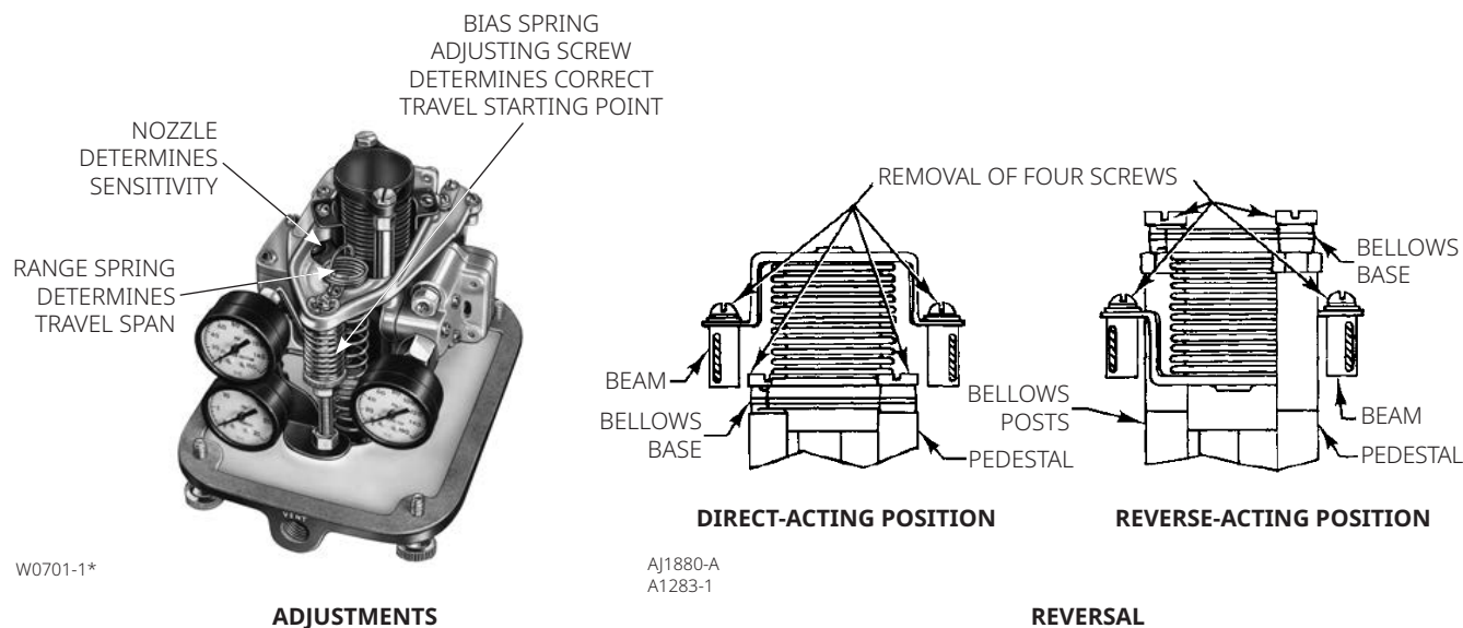
Figure 1. Positioner Simplicity
