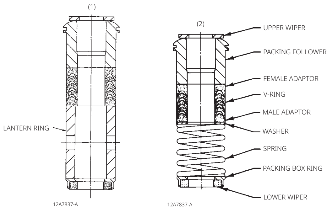
Figure 15. Typical Single PTFE V-Ring Packing Arrangement
