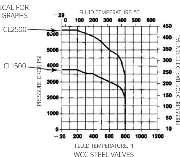
Figure 22. Pressure/Temperature Limits for CL1500 and 2500 Valves (NPS 8 through 14 Valves)
