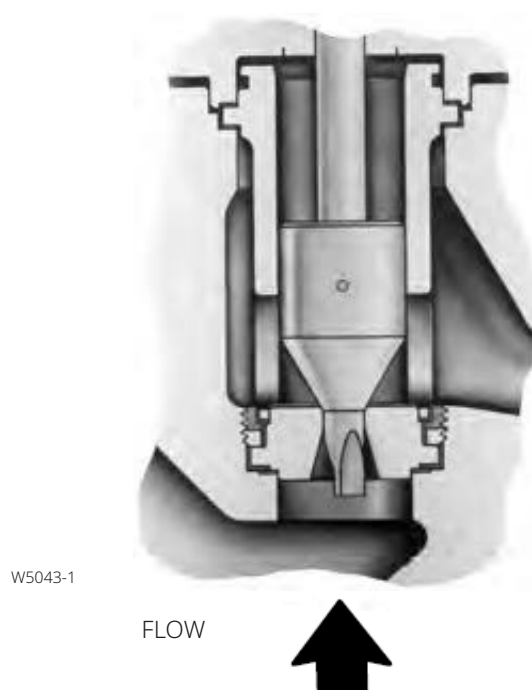
Figure 6. Fisher EHS Trim with Micro-Flute Valve Plug
