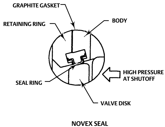
Figure 2. Available Seal Configurations
