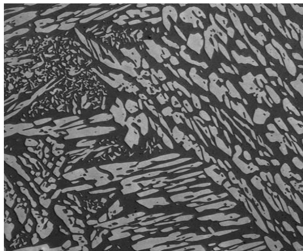
W8154 Photomicrograph of a Typical Cast Duplex Stainless Steel
