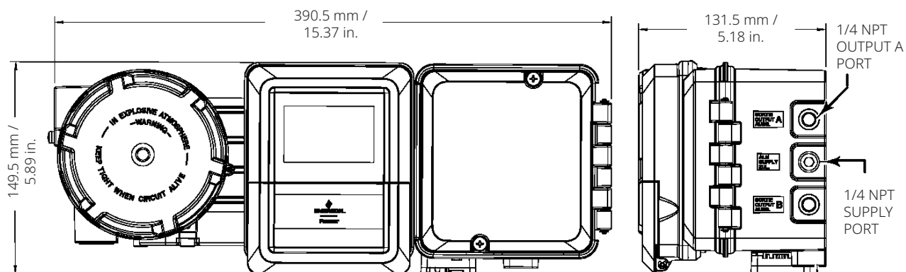
BASE UNIT WITH PNEUMATIC OUTPUT OPTION
