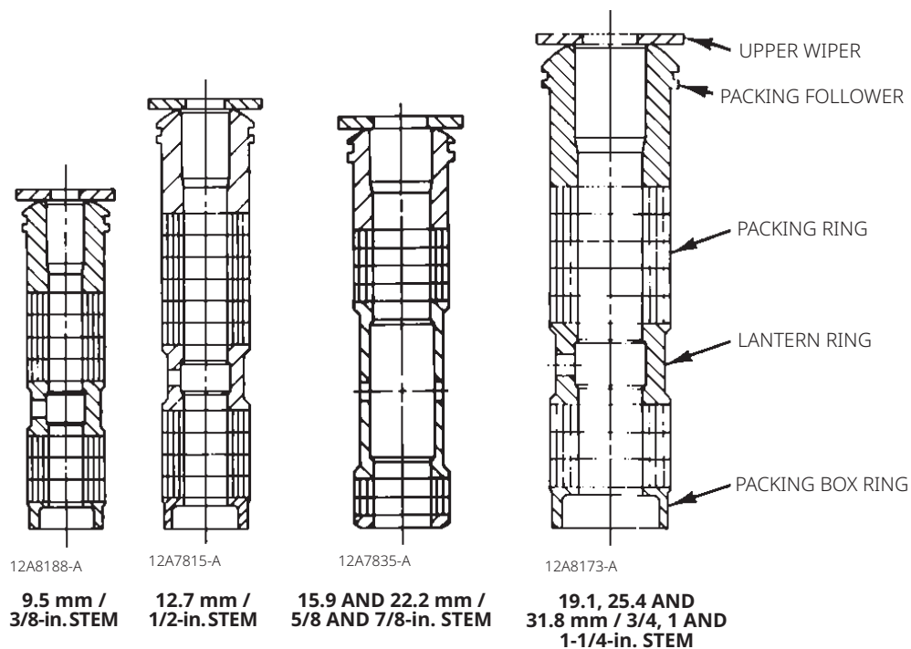
Figure 19. Typical Double PTFE Impregnated Composition Packing Arrangement
