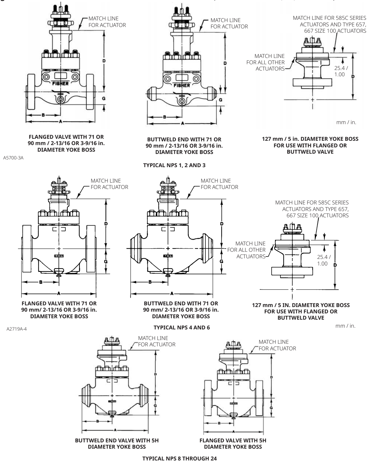
Figure 25. Globe Valve Dimensions with Standard Bonnet (also see Tables 15, 16, 17 and 18)
