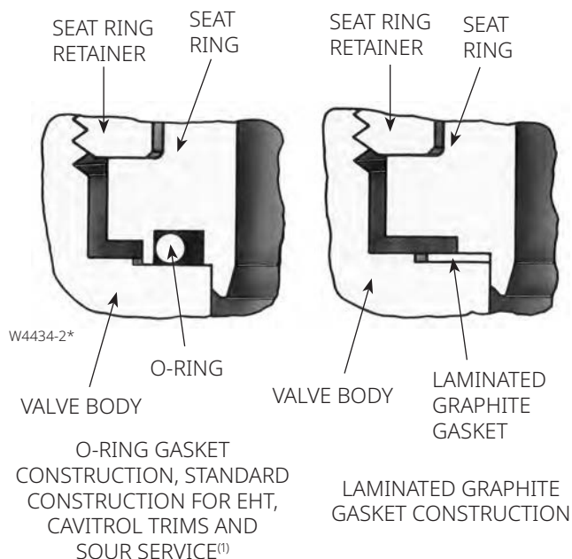
Figure 2. Seat Ring Gasket Constructions
