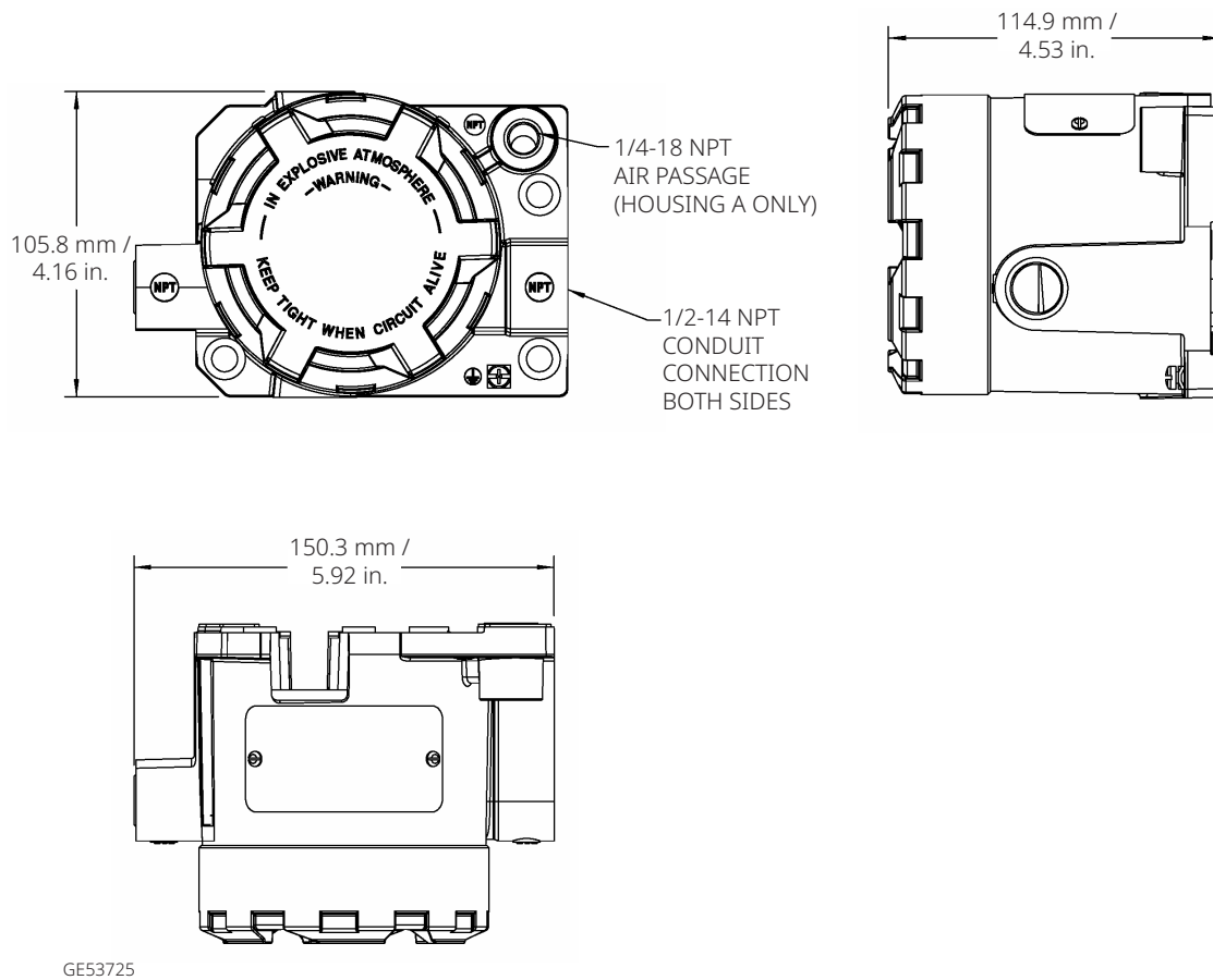
Figure 3. FIELDVUE DVC6215 Feedback Unit Envelope Dimensions
