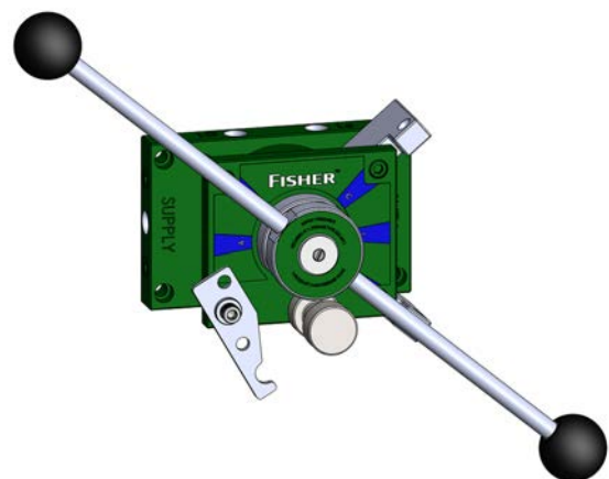
MANUAL OPEN MODE: VALVE IS OPENING
