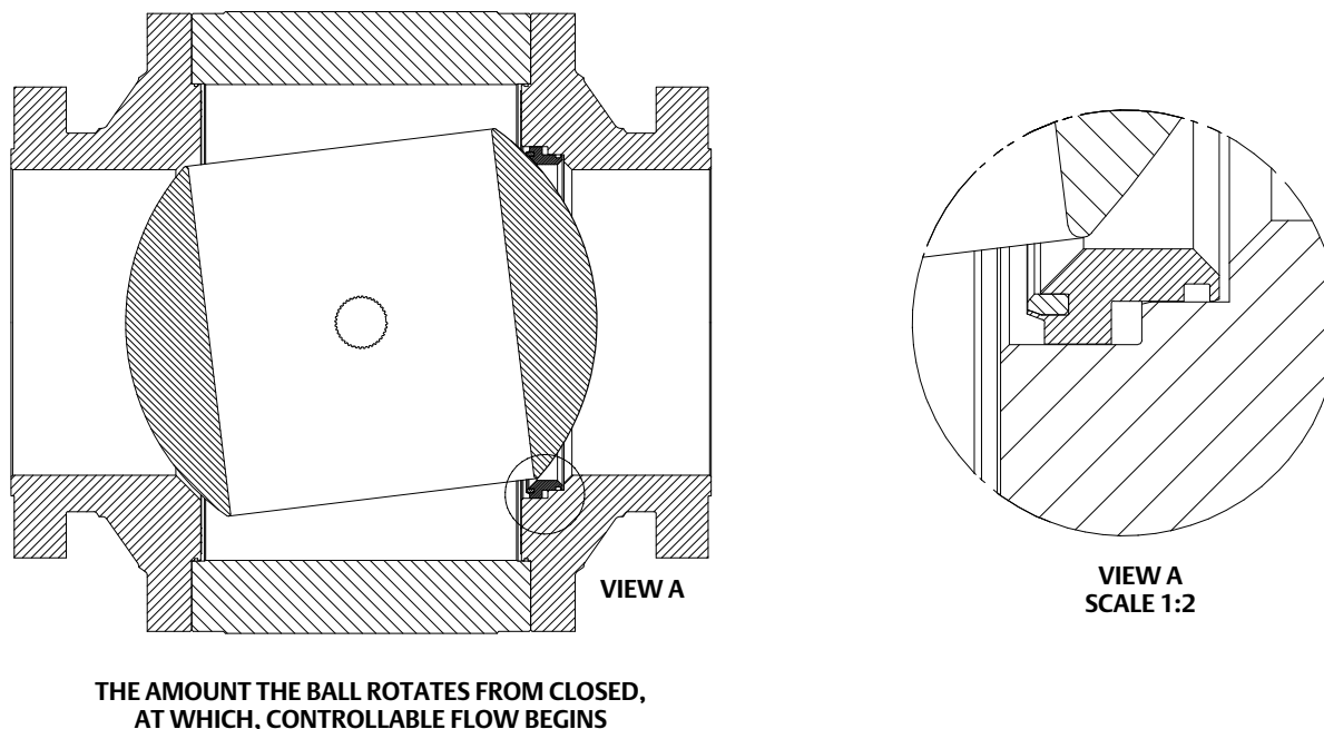
Figure 9. Dead Angle (also see table 4)
