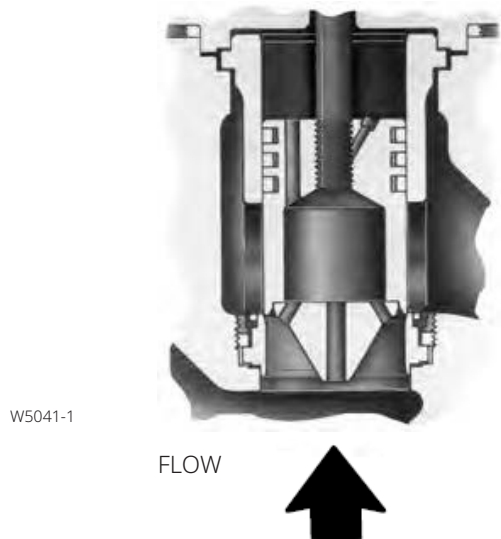
Figure 7. Diverter Cone Plug Used in NPS 6 Fisher EHD and EHT Valves (Flow Up Only)
