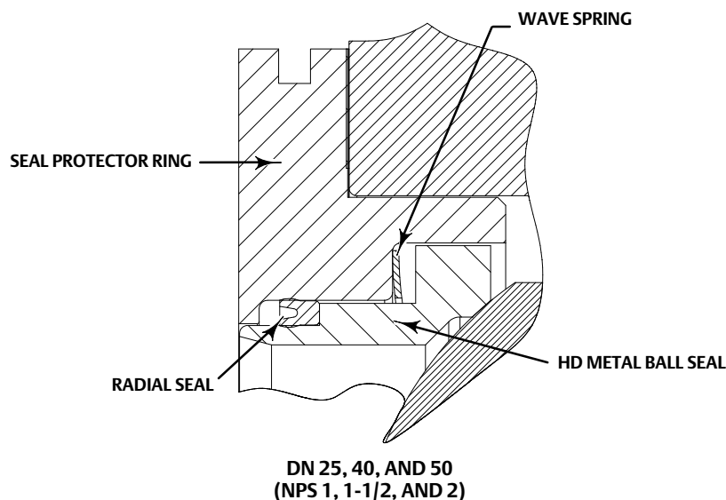
Figure 1. Fisher V200U Construction Features, DN 25, 40, and 50 (NPS 1, 1-1/2, and 2) HD Ball Seal
