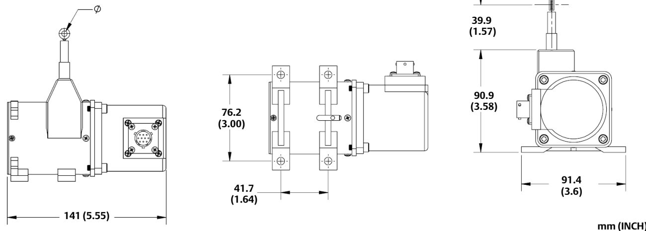
Figure 2. Dimensions
