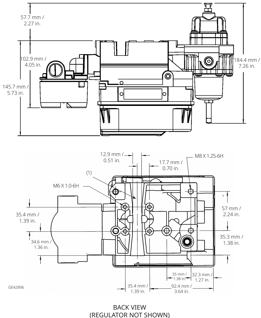
Figure 1. FIELDVUE DVC6200, DVC6200 SIS, DVC6200f, and DVC6200p Digital Valve Controller with Integrally Mounted Filter Regulator (continued)
