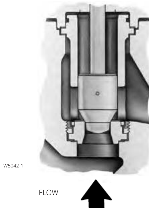
Figure 5. Fisher EHS Trim with Micro-Form Valve Plug
