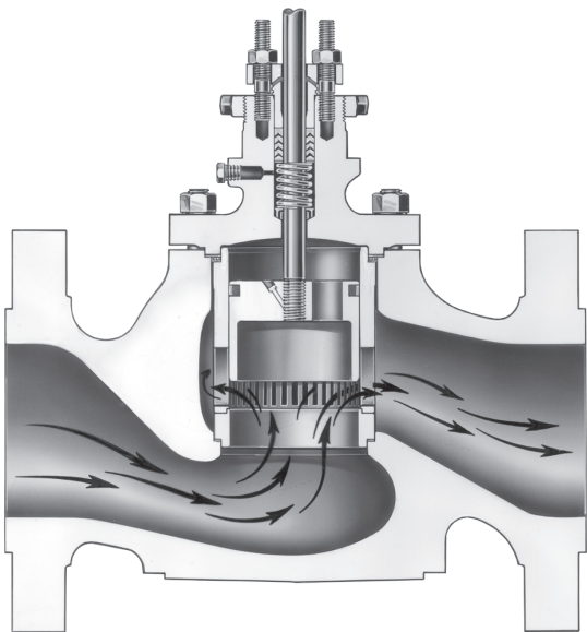
FISHER EWT METAL-SEAT VALVE WITH WHISPER TRIM I CAGE
