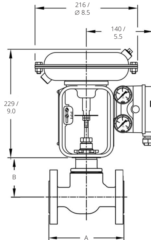
24000C WITH 32 ACTUATOR AND FISHER 3660/3661 POSITIONER
