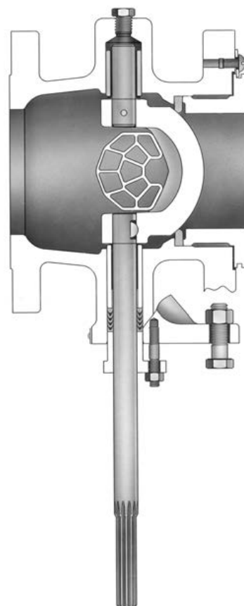
Figure 7. Fisher Vee-Ball Series Rotary Attenuator Construction
