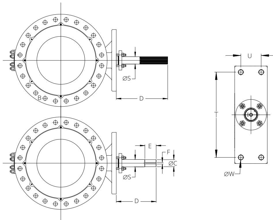
Figure 20. Fisher Vee-Ball Keyed Shaft Dimensions (also see Table 19)
