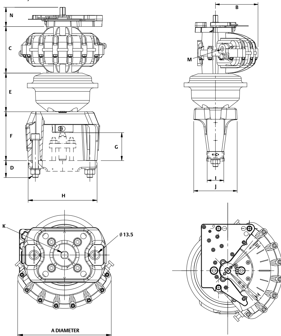
Figure 1. 1068 Actuator — Spring Return and Double Acting Dimension Drawing for 9 and 11 mm Square Shaft (see tables 7 and 8)
