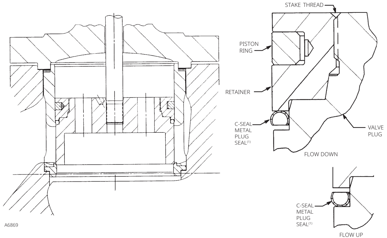
Figure 5. C-seal Trim
