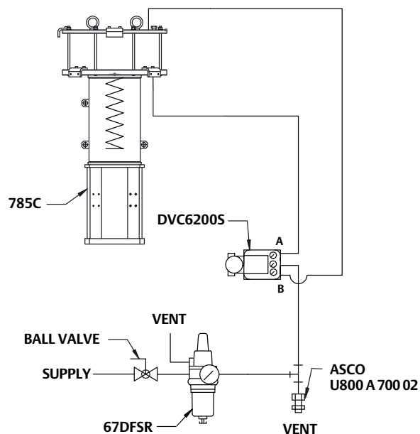
VALVE CLOSES ON AIR FAILURE
