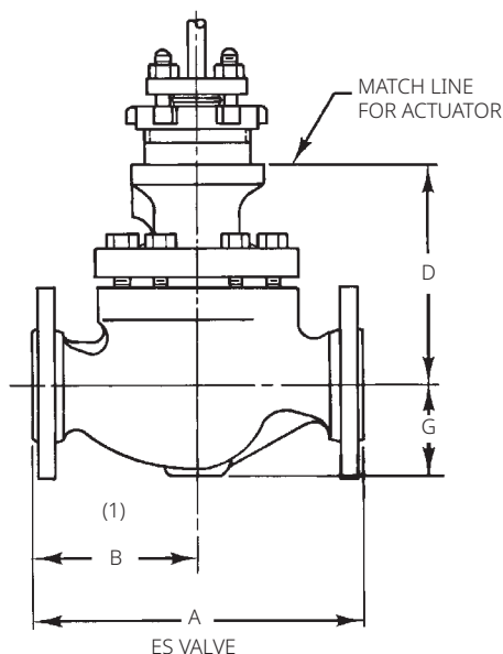
Figure 7. Fisher ES Dimensions (also see Tables 14, 15 and 16)
