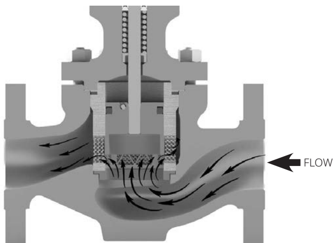
Figure 6. Fisher Whisper NXG Trim
