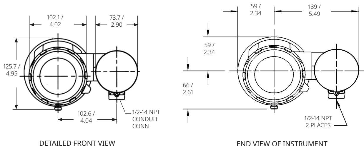
Figure 16. FIELDVUE DLC3020f Digital Level Controller Dimensions
