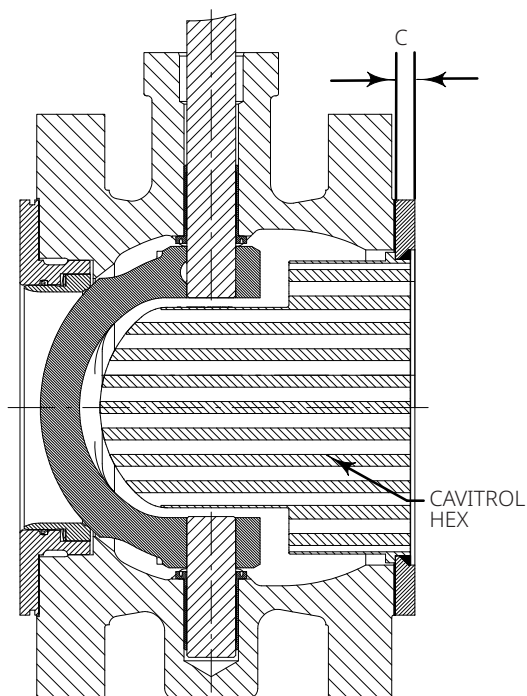
Figure 9. Fisher NPS 8 V300 Cavitrol Hex Cross Sectional View
