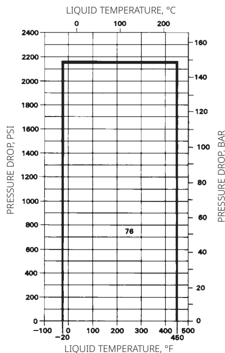
Figure 12. Typical Trim Used in Cavitrol III Cage Constructions with Steel or Stainless Steel Valves (see Table 15)
