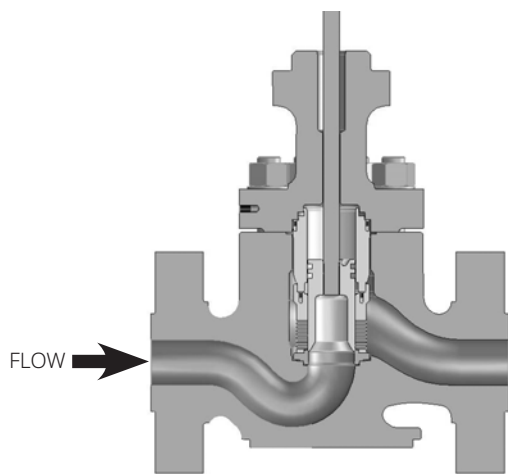
Figure 7. Fisher HPT Valve Assembly, NPS 3 to 6
