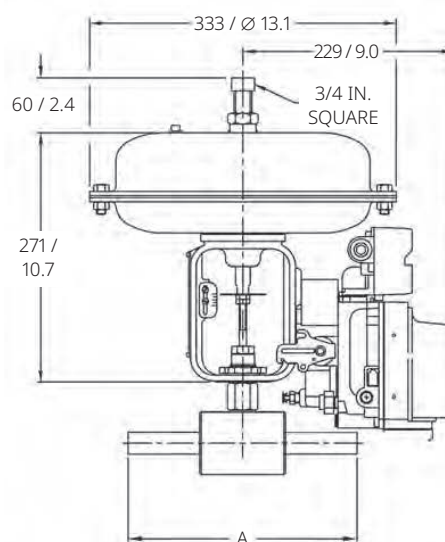
70 ATO ACTUATOR WITH BUTTWELD ENDS AND FISHER FIELDVUE DIGITAL VALVE CONTROLLER
