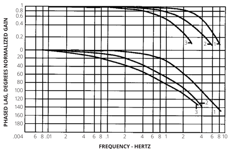
Figure 3. Frequency Response
