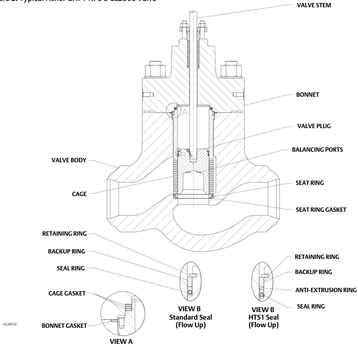
Figure 2. Typical Fisher CHPT NPS 8 CL2500 Valve
