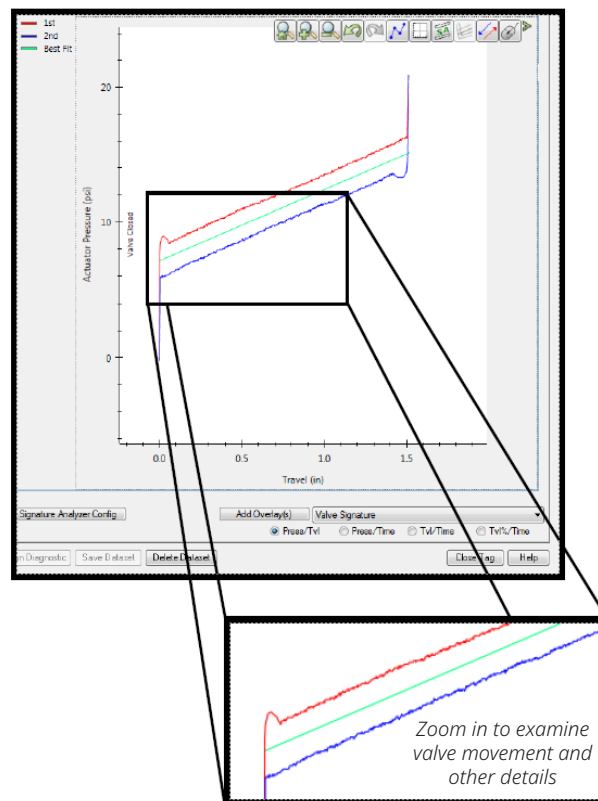
Diagnostic tests, such as the Valve Signature Diagnostic example shown here, help you detect emerging valve repair requirements before they impact performance
