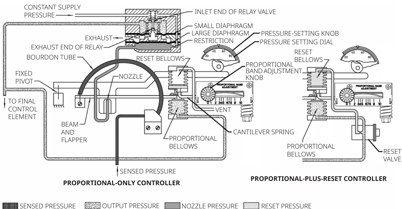
Figure 2. Schematic of Reverse-Acting Proportional-Only and Proportional-Plus-Reset Controllers
