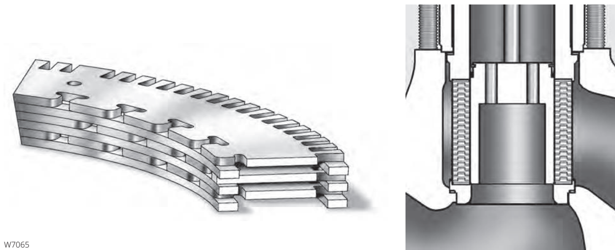
Figure 7. Typical WhisperFlo Cage
