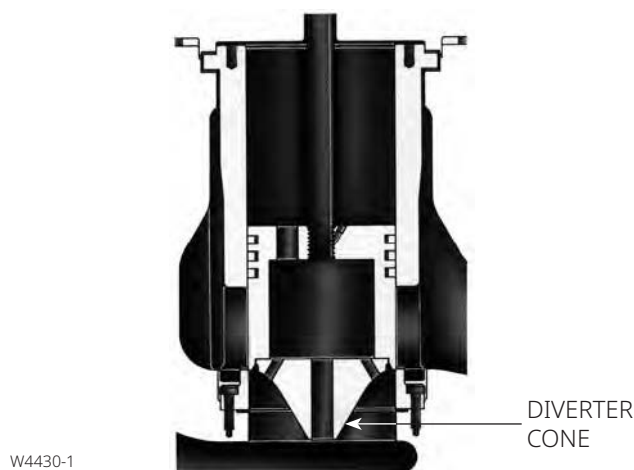
Figure 12. Diverter Cone Valve Plug Used in Fisher EHD and EHT Valves (NPS 8 through 14 Globe Valves, Flow Up Only)
