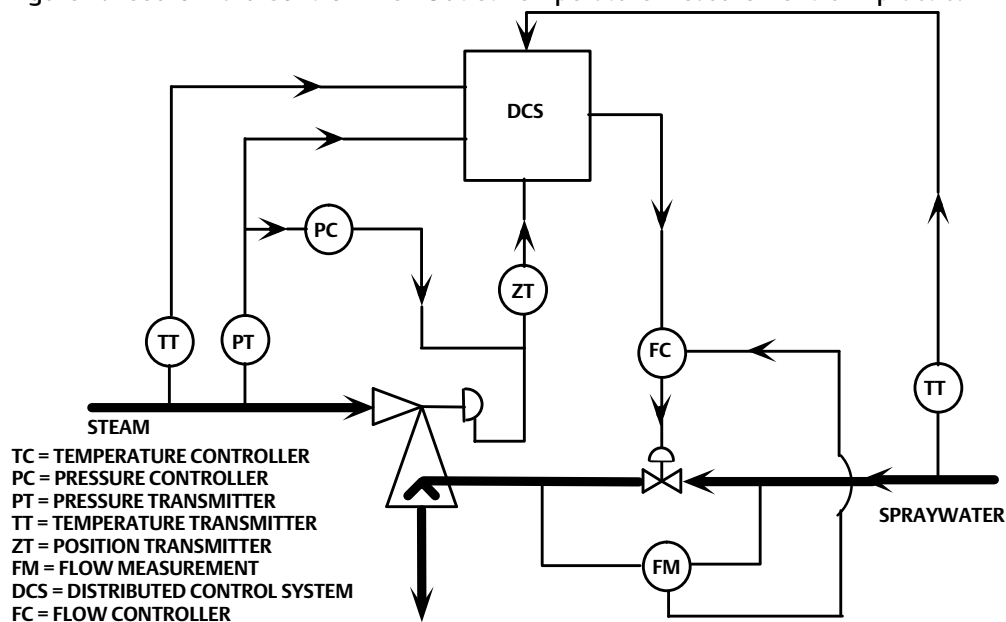
Figure 4. Feedforward Control when Outlet Temperature Measurement is Impractical
