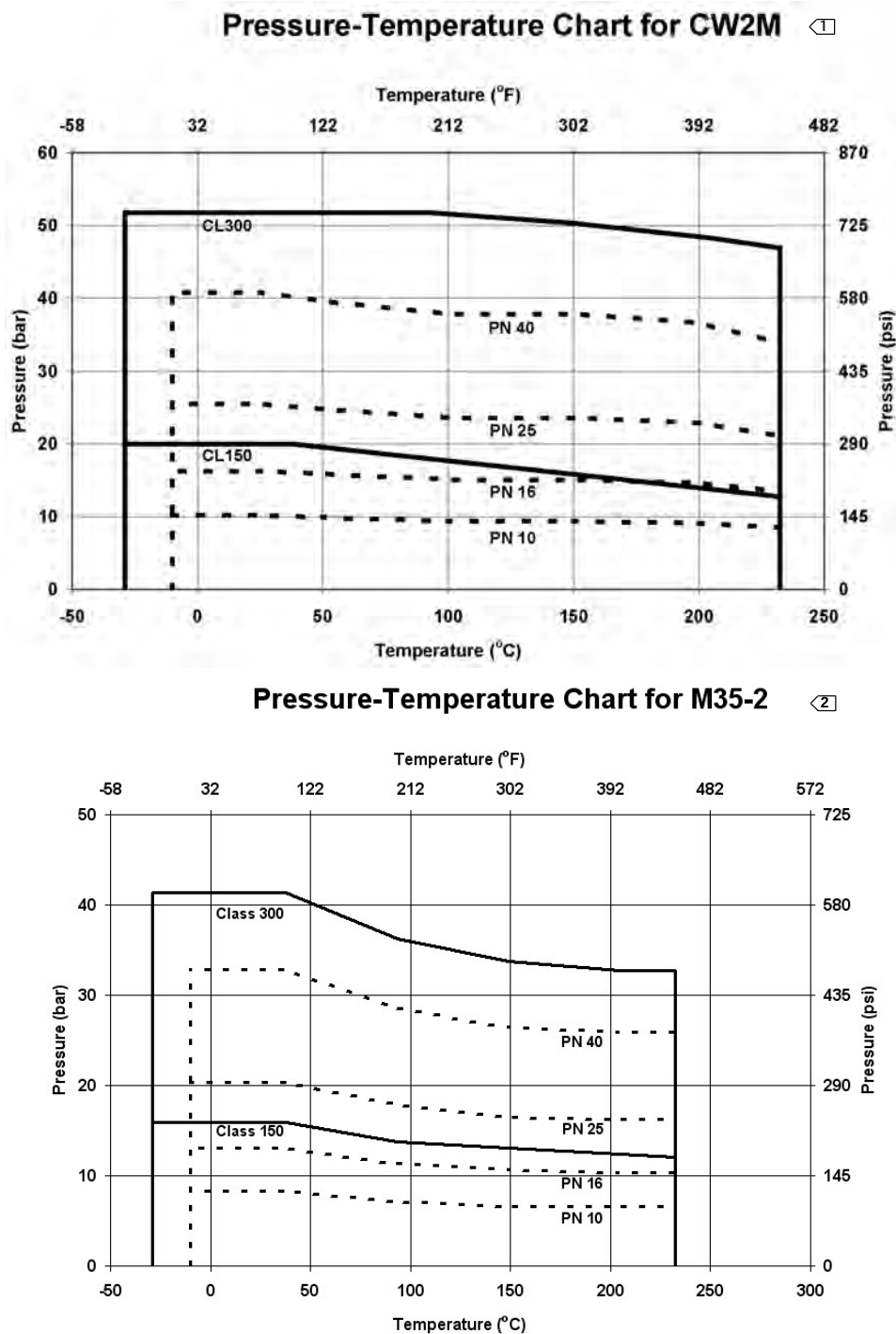
Figure 6. Material Pressure/Temperature Curves
