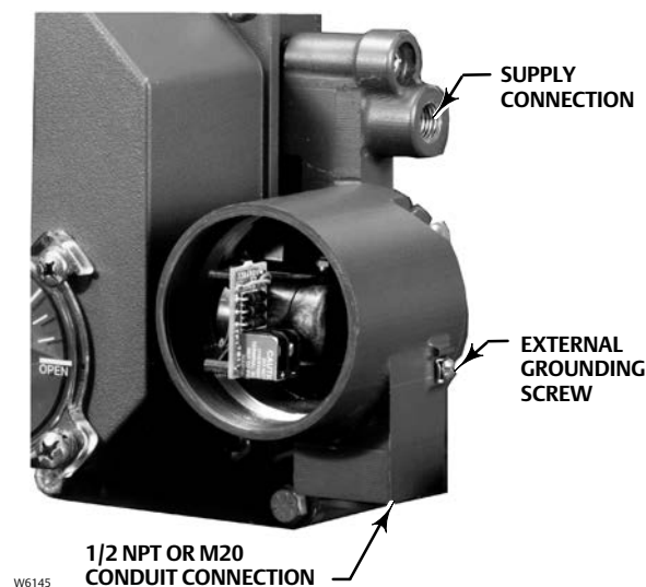
3722 ELECTRO-PNEUMATIC CONVERTER
