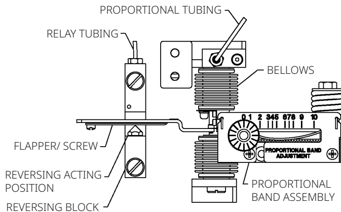
REVERSE-ACTING
