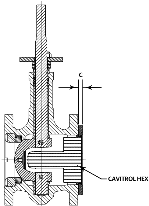
Figure 4. Fisher NPS 6 CV500 Cavitrol Hex Cross Sectional View
