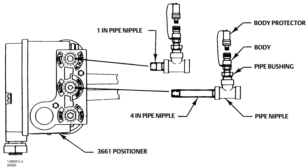
Fisher 3661 POSITIONER
