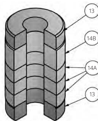
Figure 7. Molded Graphite (Flexible Graphite) Packing Kit (Optional)
