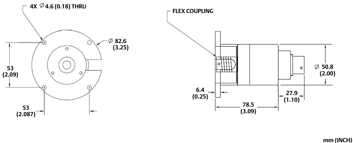
Figure 2. Dimensions
