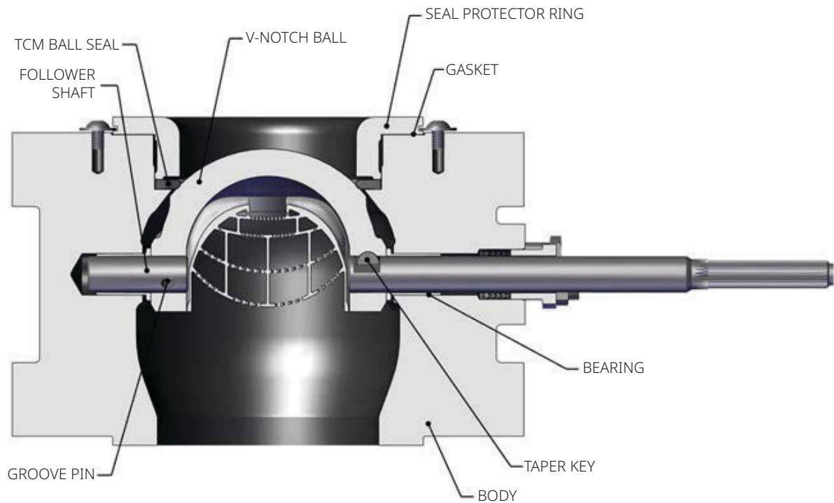
Figure 2. Fisher Vee-Ball Series Whisper NXV Construction
