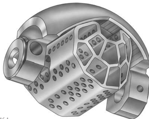
Figure 6. Fisher Vee-Ball Series Noise Attenuator Ball
