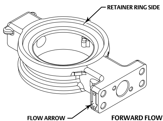
Figure 3. Flow Direction Arrow
