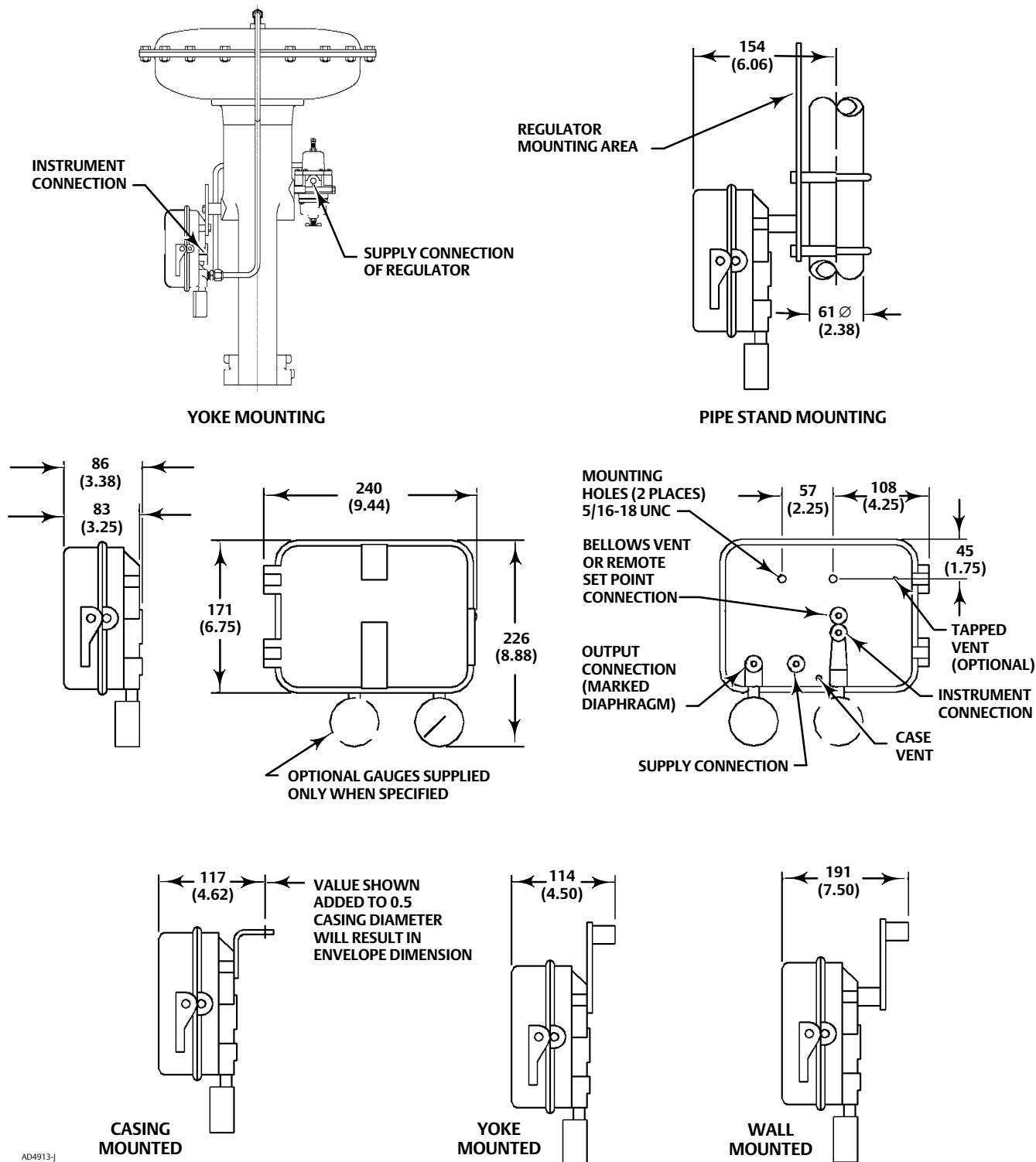
Figure 5. Dimensions
