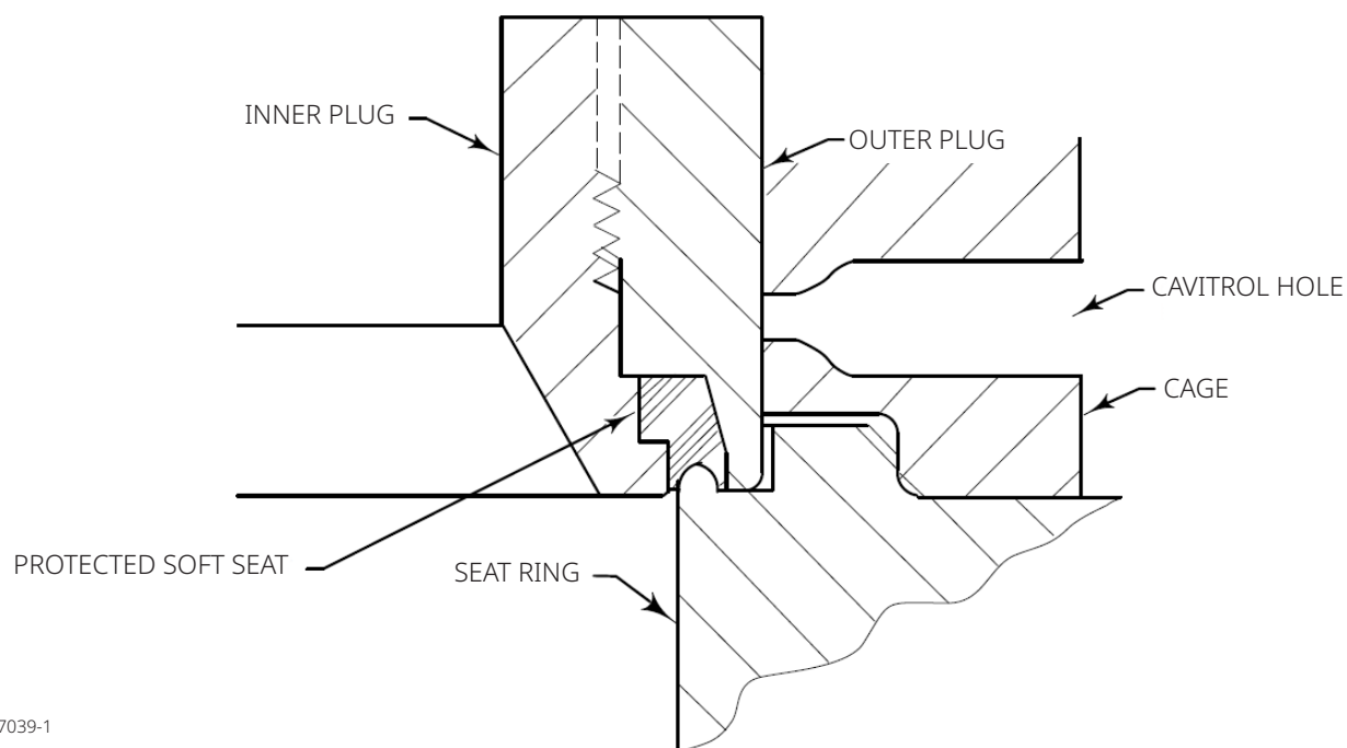
Figure 5. Detail of TSO (Tight Shutoff Trim) Protected Soft Seat
