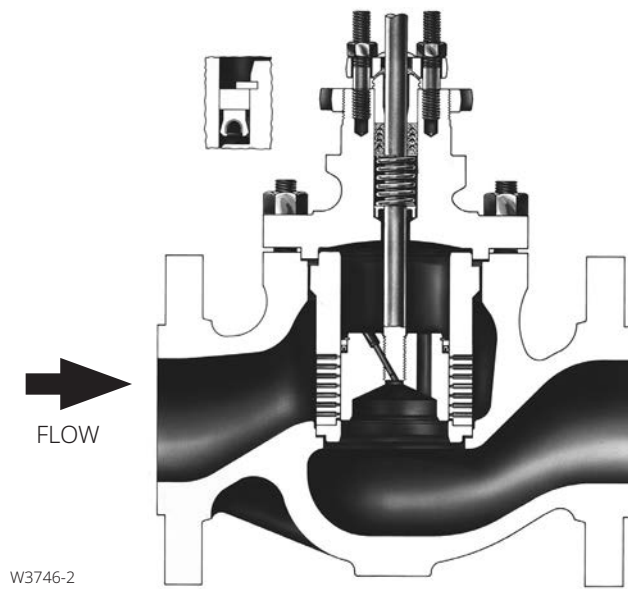
Figure 1. Sectional View of Fisher ET Valve with Cavitrol III One-Stage Trim
