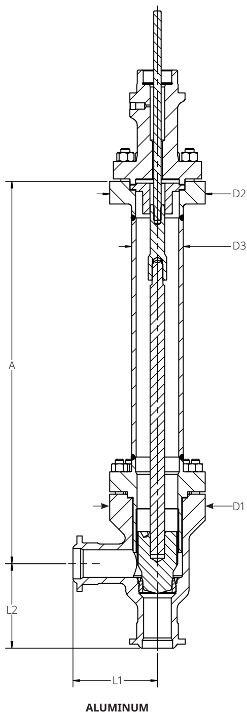
Figure 4. Fisher IC2 Angle Body Valve Dimensions (Also See Table 7)
