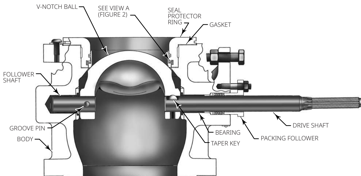
Figure 3. Vee-Ball Construction Features (Fisher V150 Shown)
