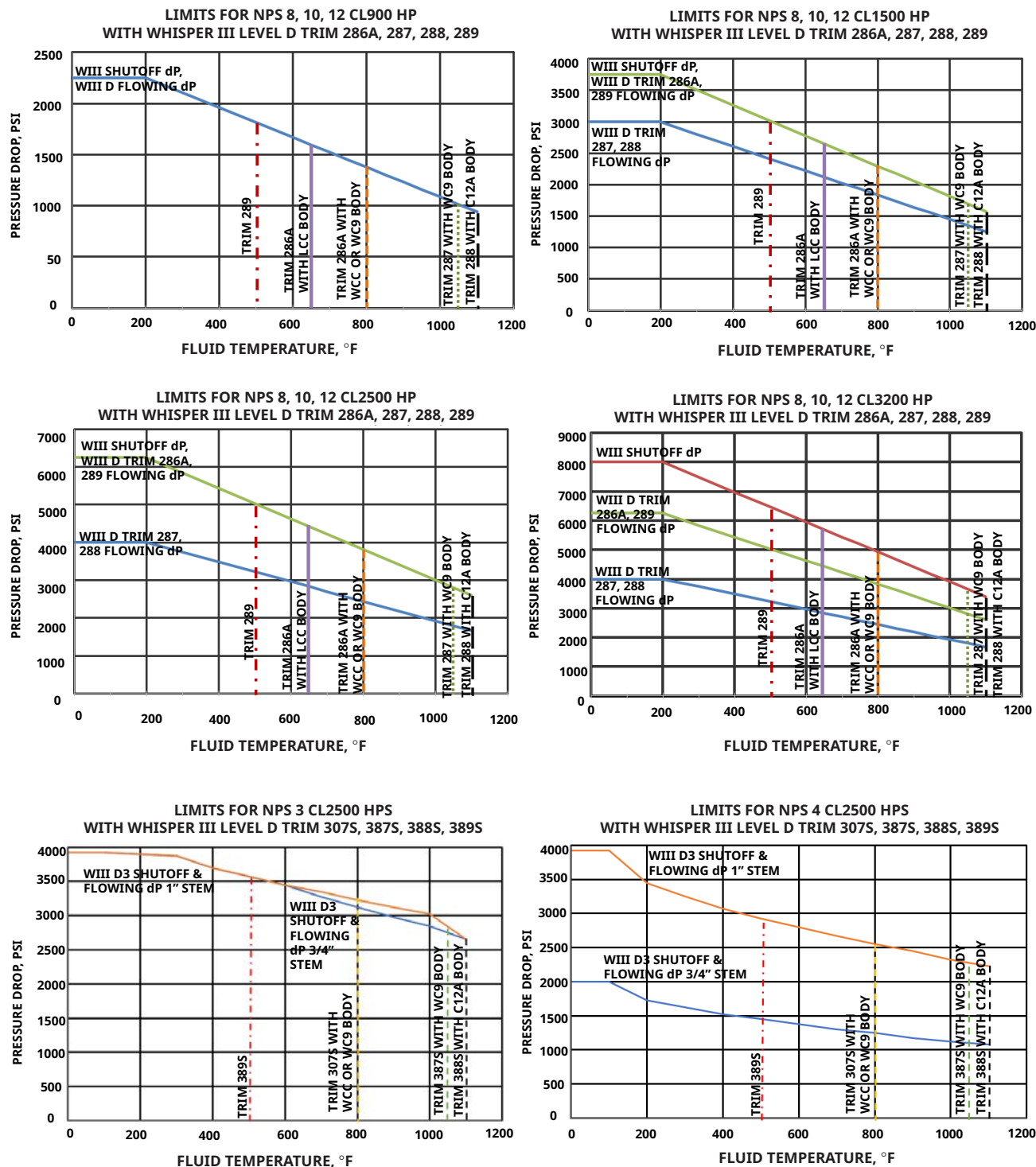
Figure 24. Pressure-Temperature Limits for Whisper III D Cage (also refer to Table 7)
