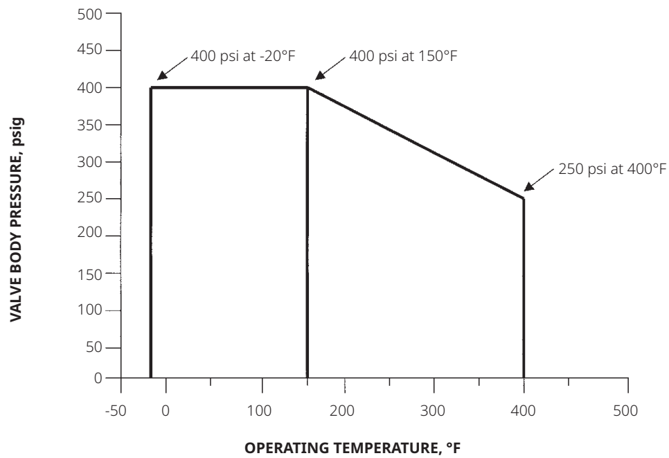
Figure 5. 24000 Pressure-Temperature Ratings
