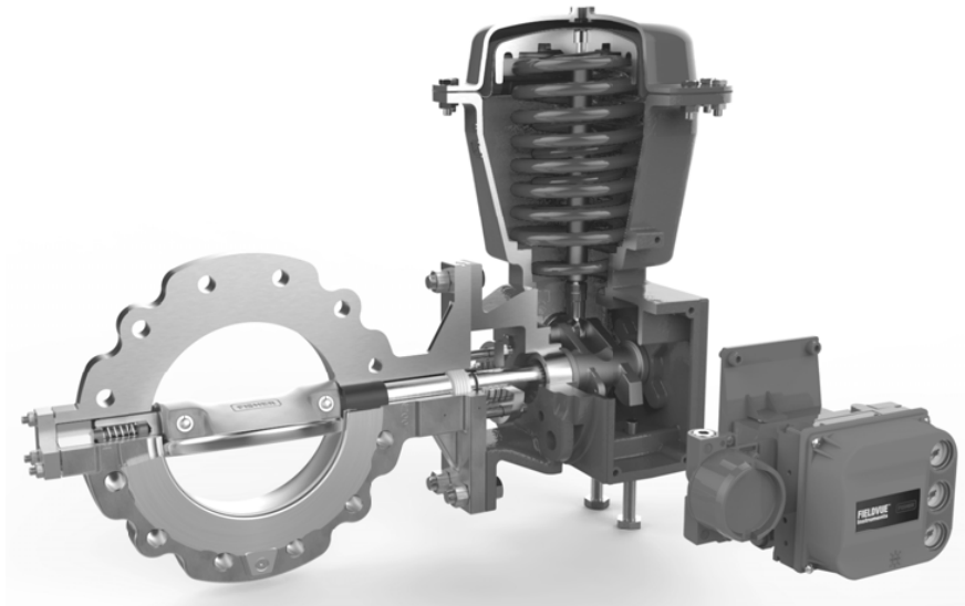
Figure 2. Fisher 2052 Assembly
