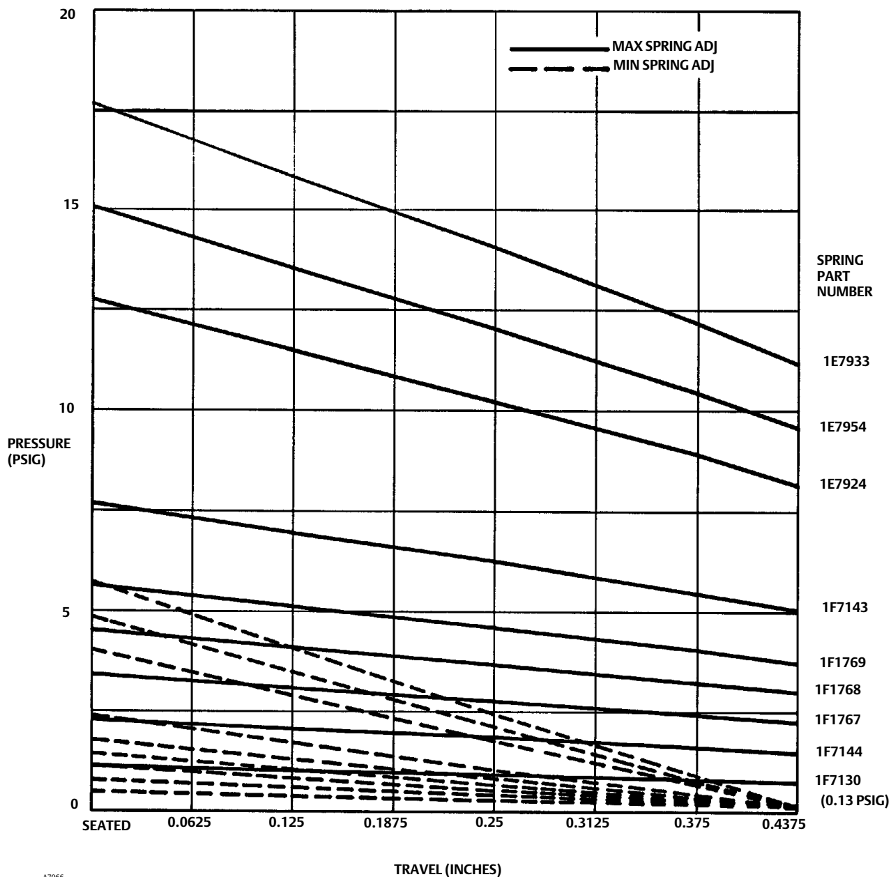
Figure 11. 655 ED, #60 Casing, Diaphragm Pressure versus Valve Travel
