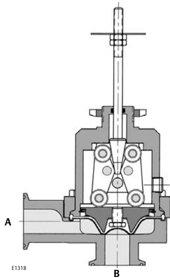
Figure 6. NPS 1 Angle and Inline Valve Body Orientations
