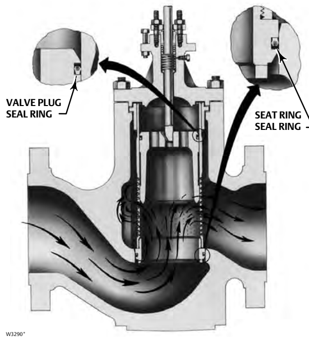
Figure 2. Whisper Trim III Cage in NPS 12 x 8 Fisher EWNT-2 Valve with Seat Ring Threaded Into the Cage
