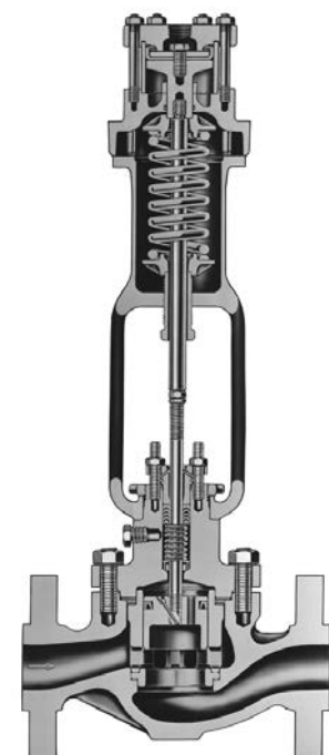
Figure 1. Fisher 1B-ED Pump Governor Sectional
