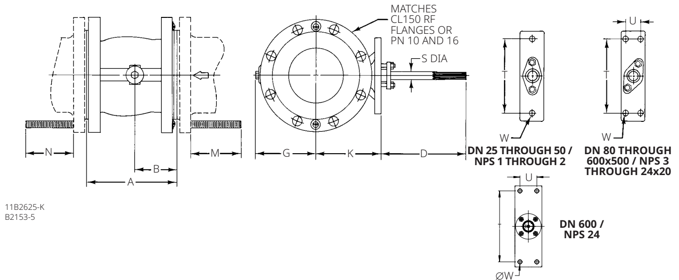
Figure 14. Fisher V150 Dimensions (also see Table 11)
