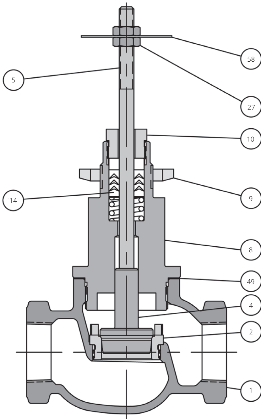
Figure 2. 24000 Valve Body Subassembly with Standard PTFE Spring-Loaded Packing
