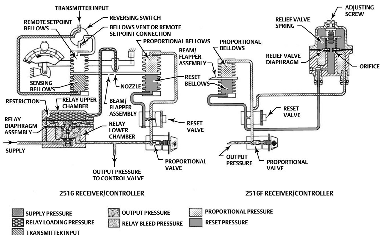
Figure 3. Fisher 2516 Receiver-Controller Schematic
