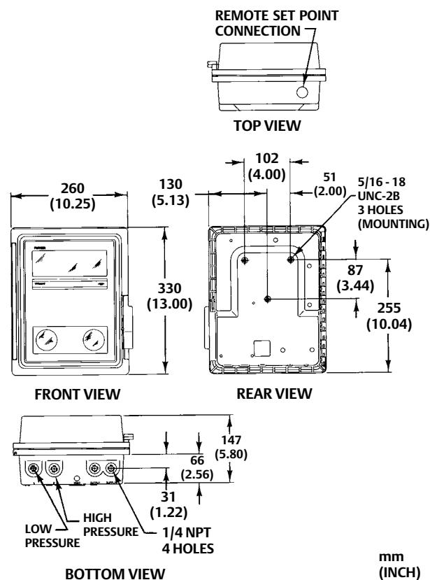
Figure 4. Controller Dimensions
