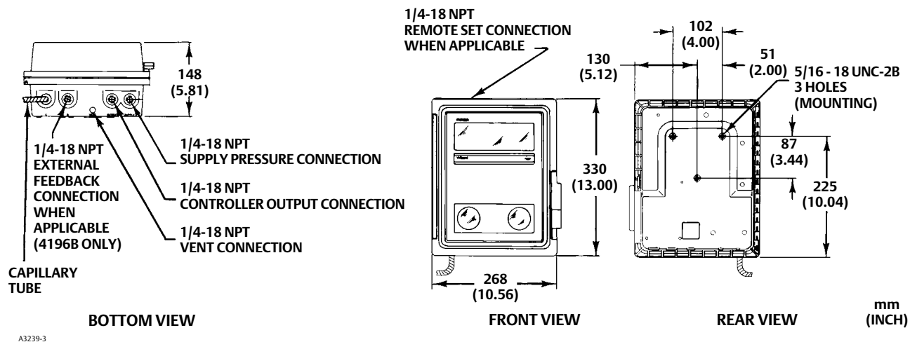
Figure 8. Controller Dimensions
