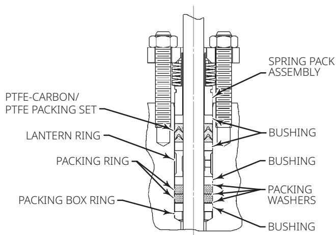
Figure 4. Enhanced ENVIRO-SEAL Duplex Packing
