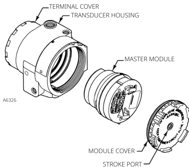
Figure 3. Master Module Construction
