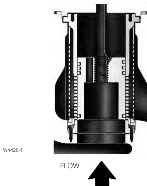
Figure 11. Fisher EHD Trim with Whisper Trim III Level D Cage (NPS 8 through 14 Globe Valves)
