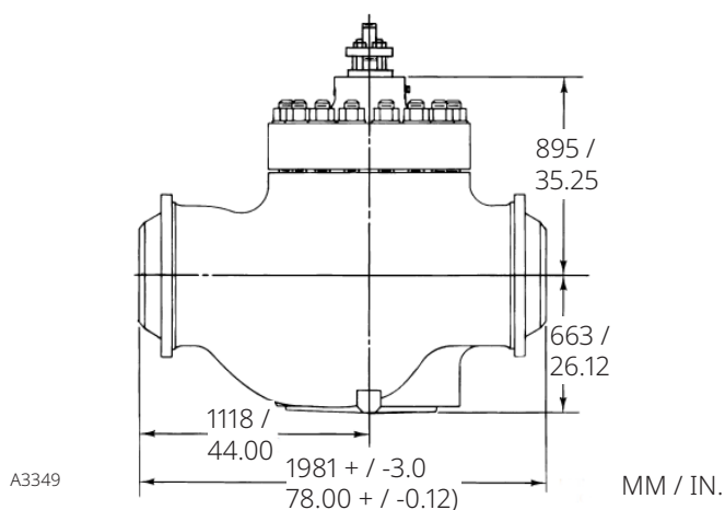
Figure 27. Dimensions (NPS 20 Fisher EHD Valve)
