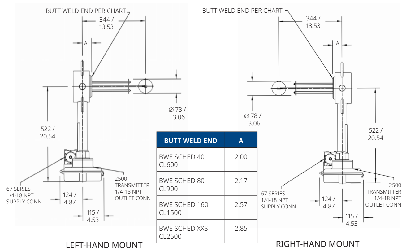
Figure 12. Fisher 249VS with 2500 Transmitter Envelope Dimensions; Butt Weld End
