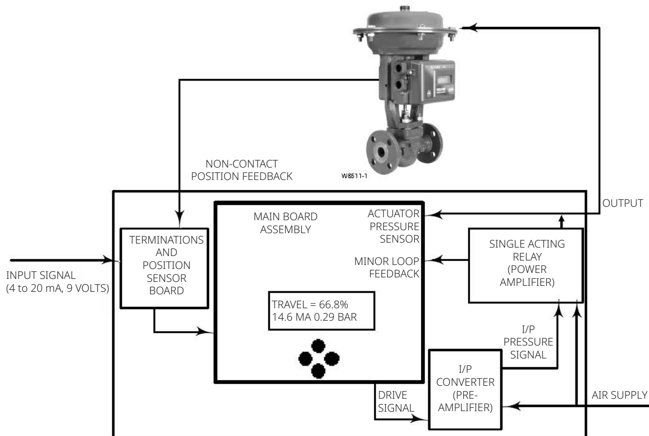
Figure 3. Block Diagram
