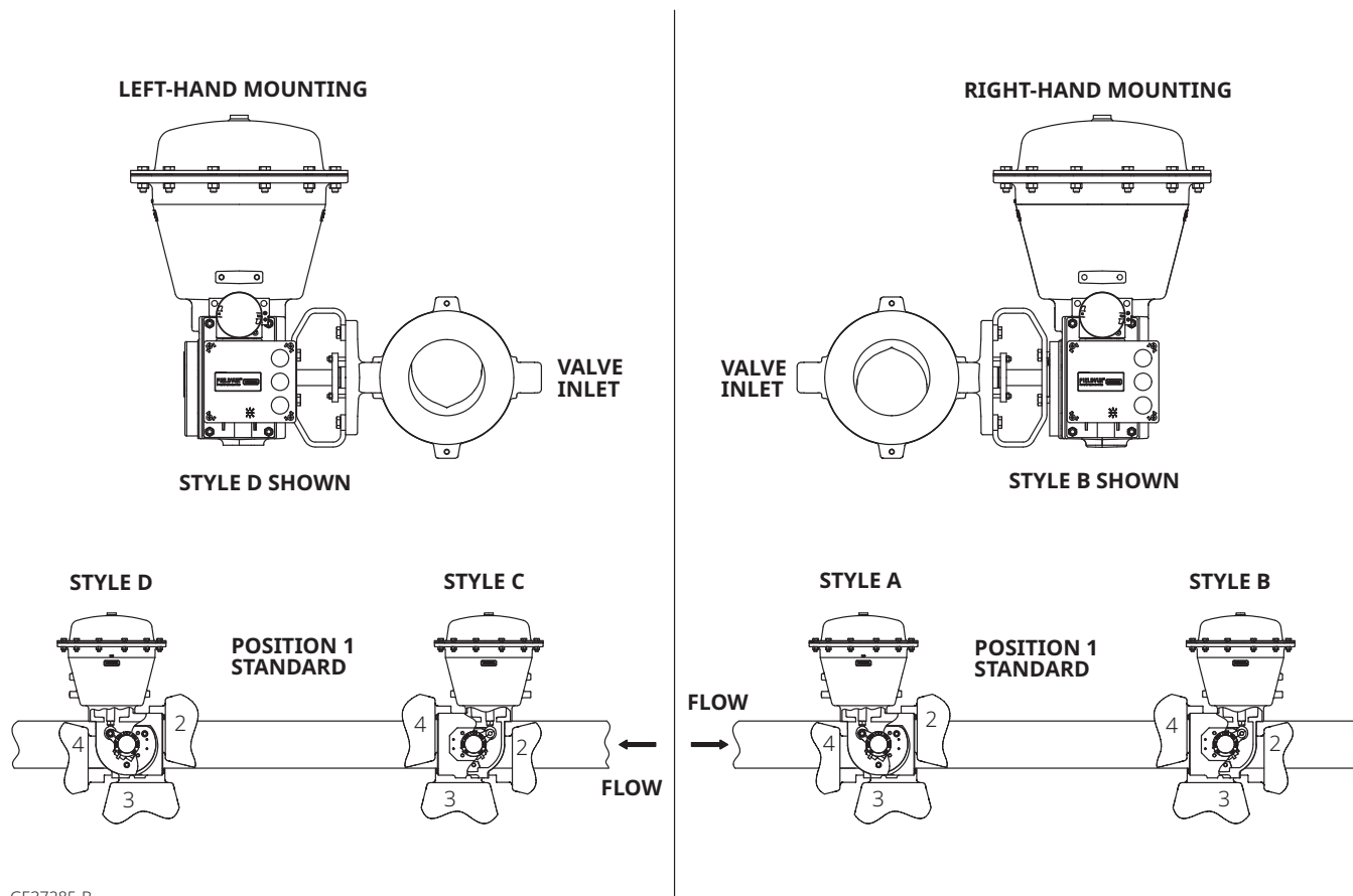
Figure 9. Fisher 2052 Actuator Mounting Styles (also see Table 13)
