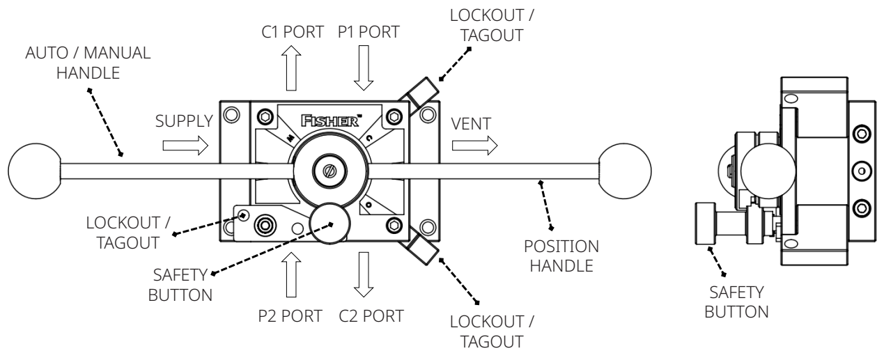
Figure 3. Product Constructions
