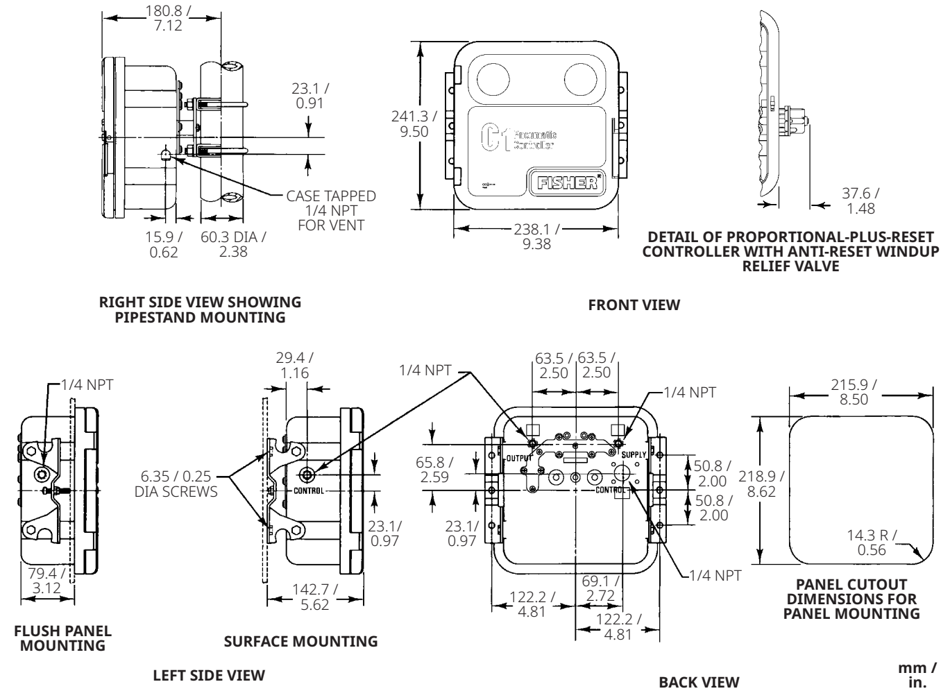
Figure 10. Dimensions
