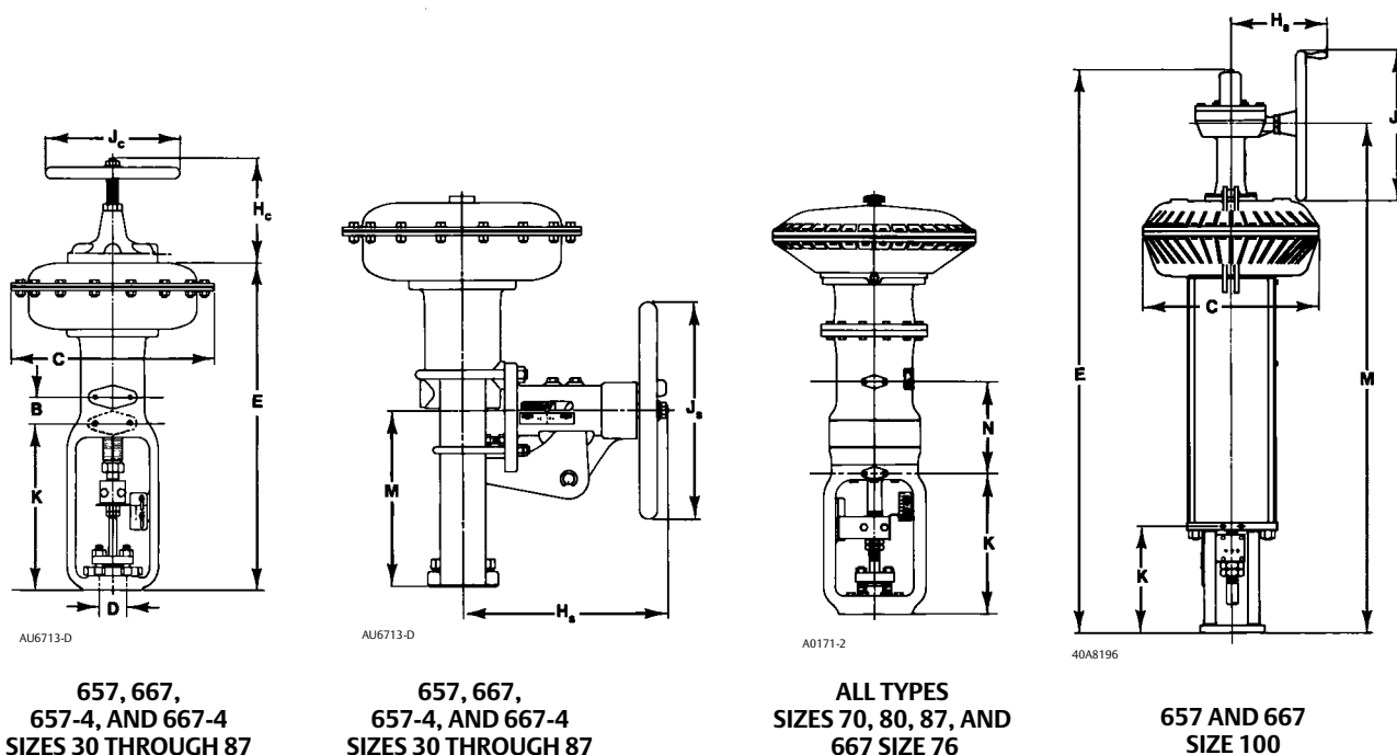
Figure 8. Dimensions (also see table 8)
