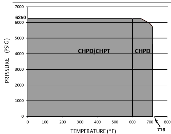
Figure 3. Pressure/Temperature Limit
