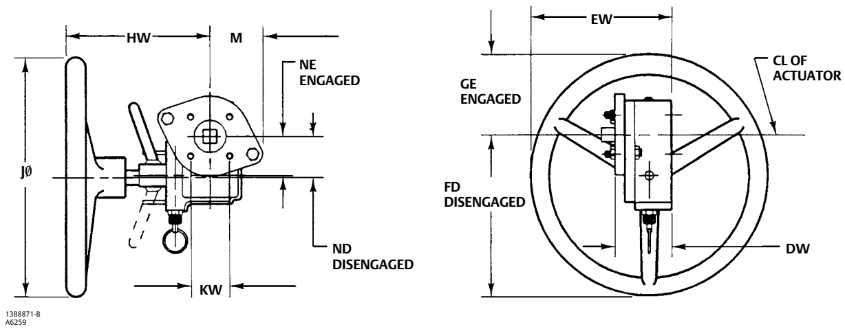
Figure 2. Dimensions (also see table 4)
