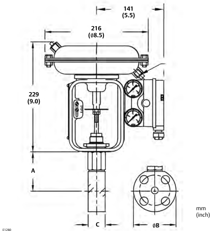
Figure 9. Dimensional Drawing
