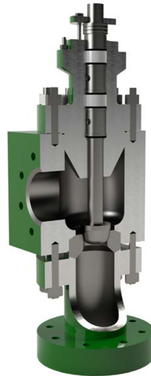
Figure 3. Fisher EHU Valve with Optional Top-Entry Bonnet
