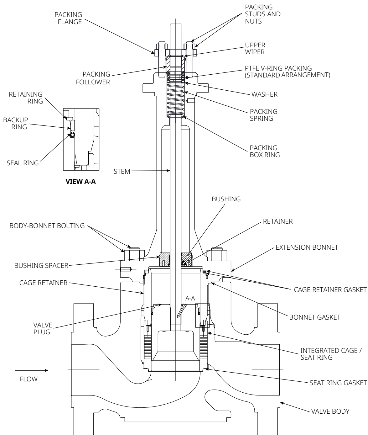
Figure 3. Fisher HPT-C Valve Assembly Detail with One-Piece Extension Bonnet NPS 4 and 6 (Short)
