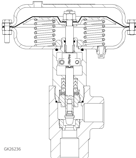
AIR-TO-OPEN
