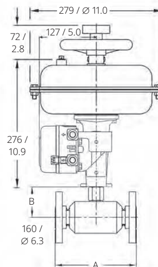
54 ATO FLANGED VALVE BODY ACTUATOR WITH FISHER FIELDVUE DVC2000 DIGITAL VALVE CONTROLLER
