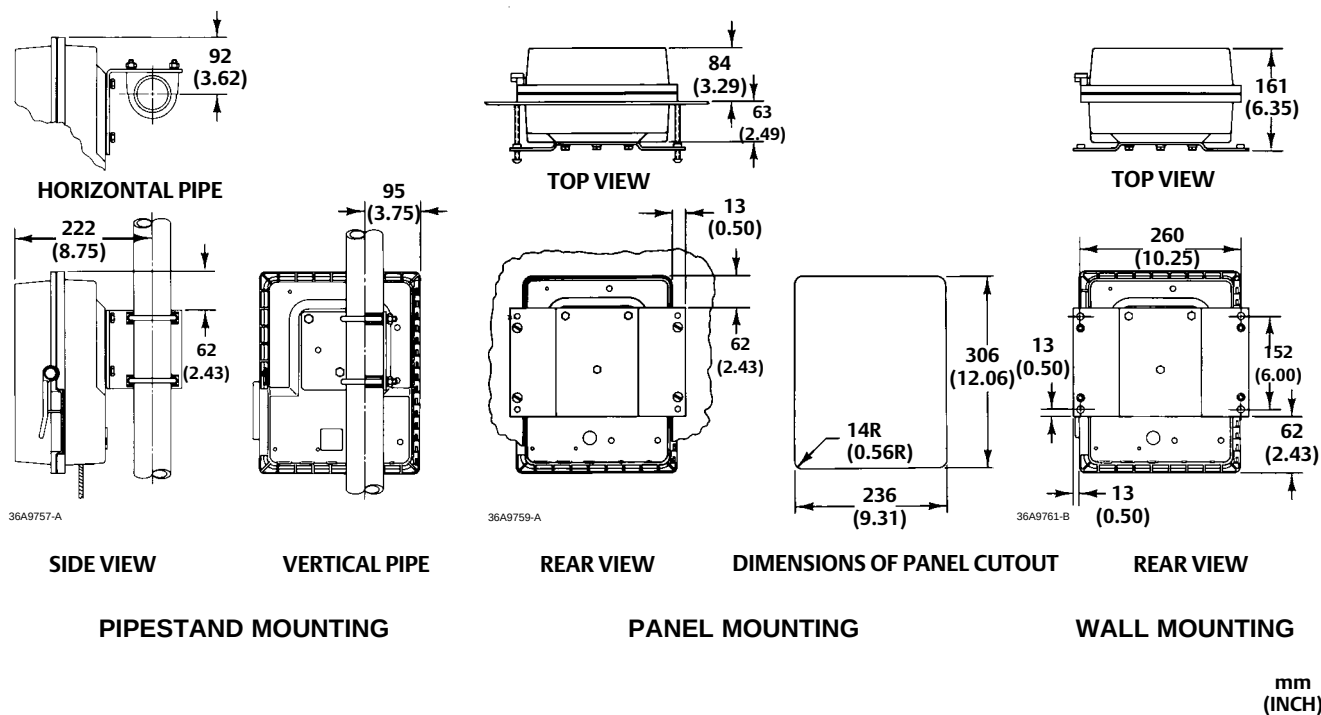
Figure 9. Mounting Dimensions
