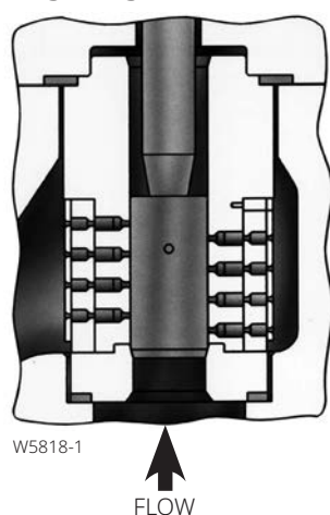
Figure 15. NPS 2 Fisher HPS Trim with Cavitrol III 3-Stage Cage
