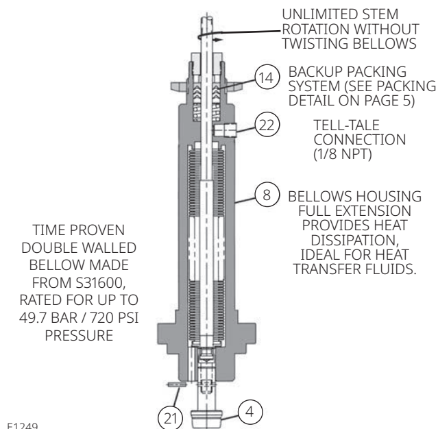
Figure 7. NOLEEK Bellow Bonnet Assembly
