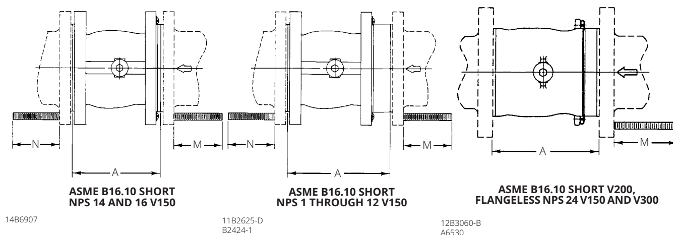
Figure 18. Fisher V150 and V200 Optional Dimensions (also see Tables 15, 16 and 17)
