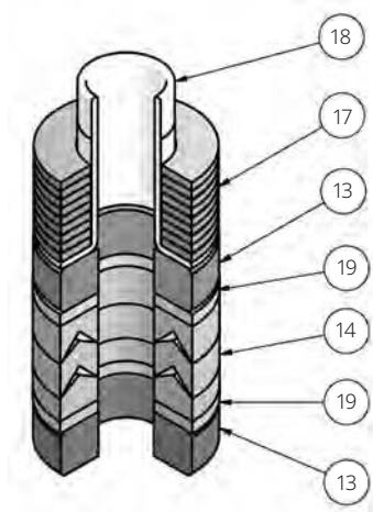
Figure 8. Fisher enhanced ENVIRO-SEAL Packing Kit (Optional)
