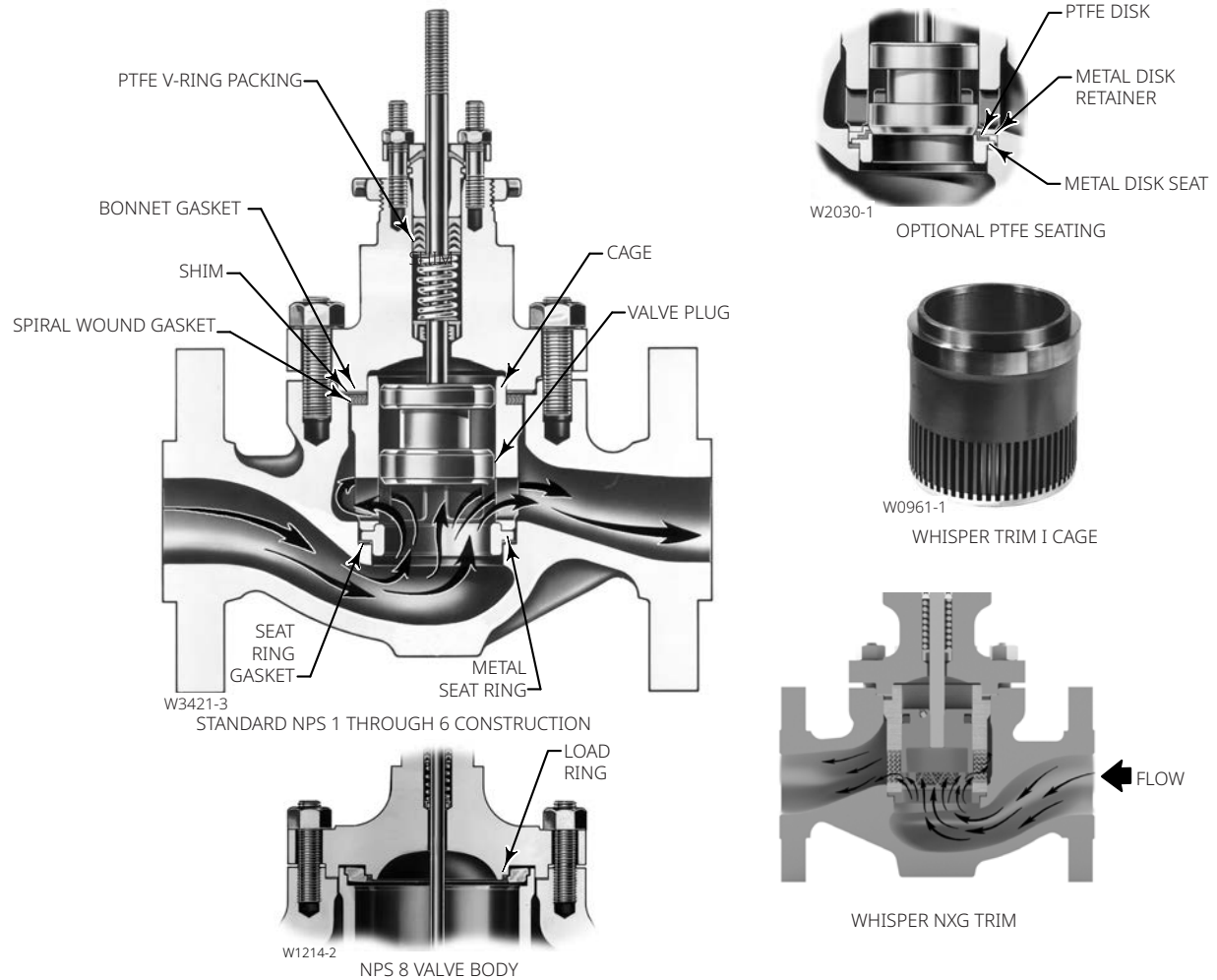
Figure 1. Fisher ES Sectional
