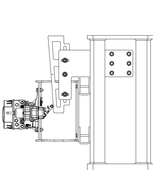
Figure 2. Fisher 785C Standard and High Performance DVC6200 Mounting Kits
