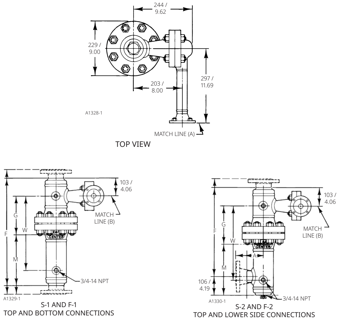
Figure 1. Fisher 249B and 249BF (1) (see Table 1, 2, 3, 4 and 5)
