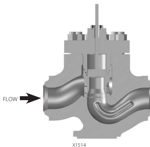
Figure 3. Fisher HPD Valve Assembly, NPS 8 to 14
