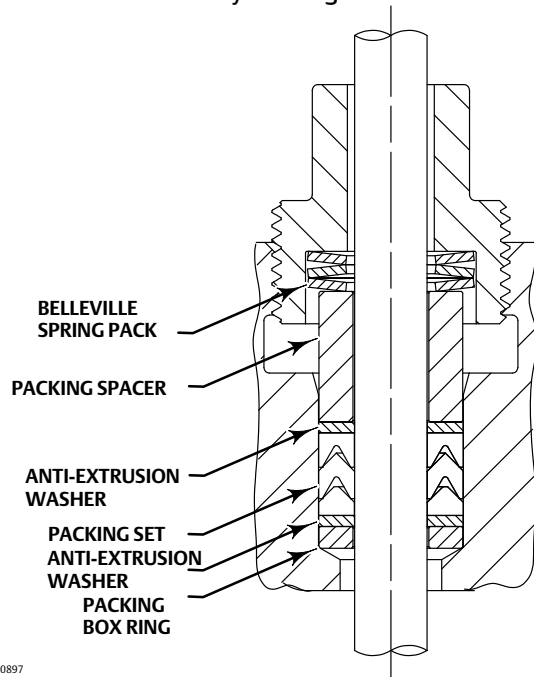
Figure 14. Fisher GX 3-Way Packing
