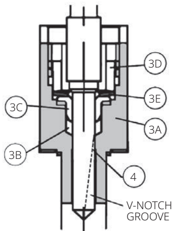
Figure 3. Soft Seat Cage Assembly
