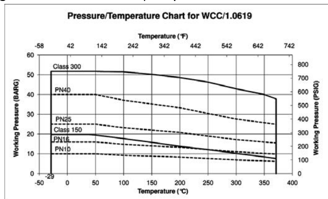
Figure 13. Material Pressure/Temperature Curves
