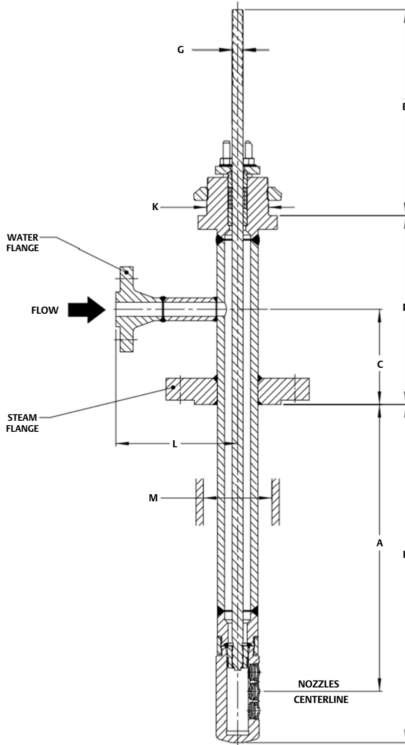
Figure 10. Yarway AT-38/48
