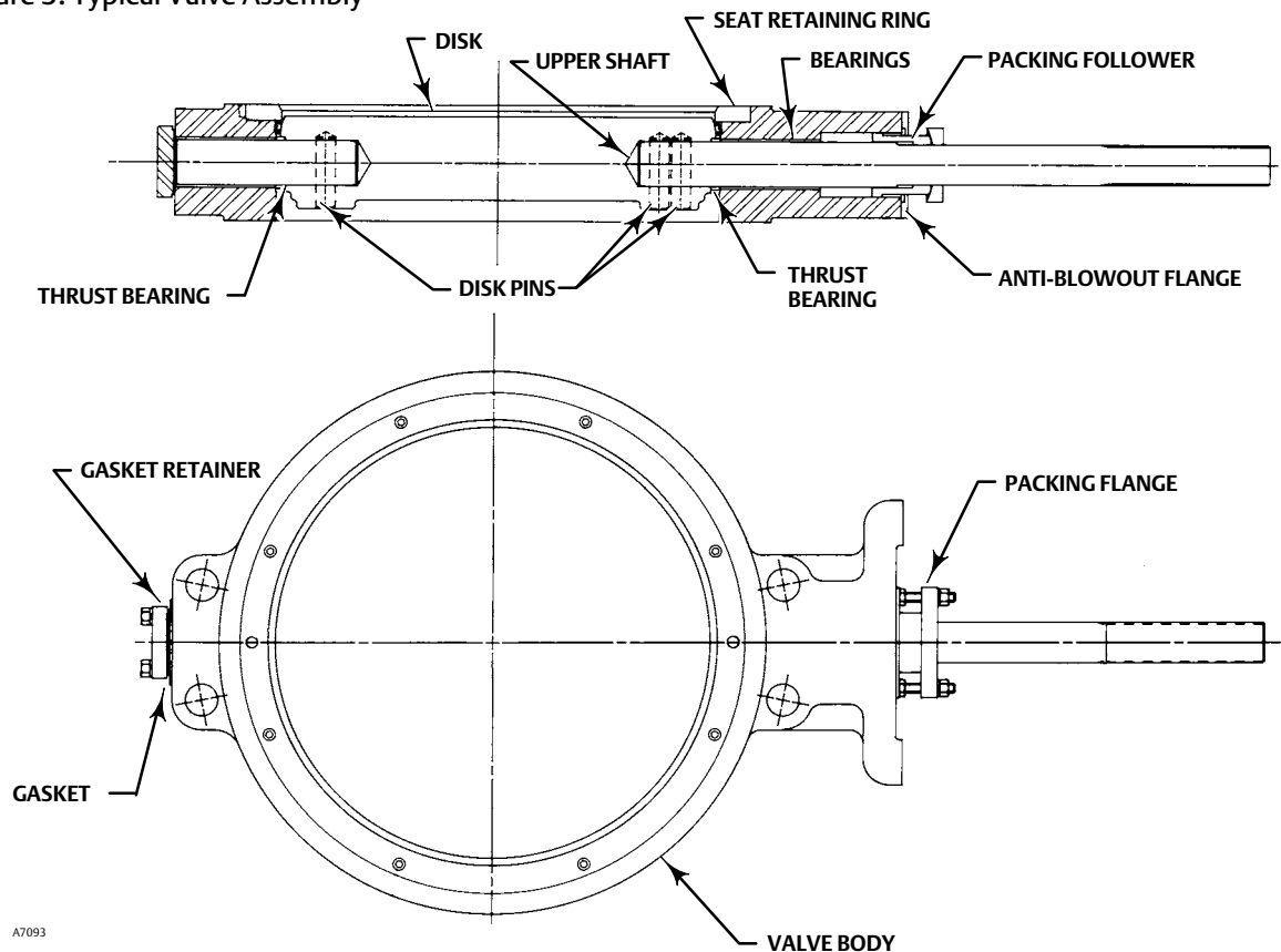
Figure 3. Typical Valve Assembly
