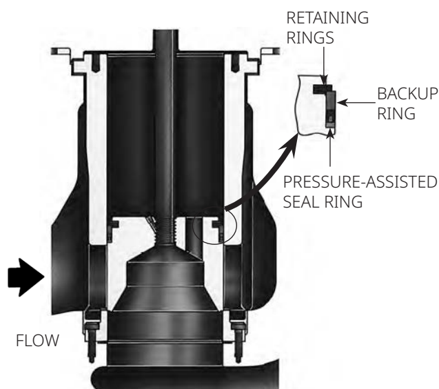
Figure 10. Fisher EHT Trim (NPS 8 through 14 Globe Valves)
