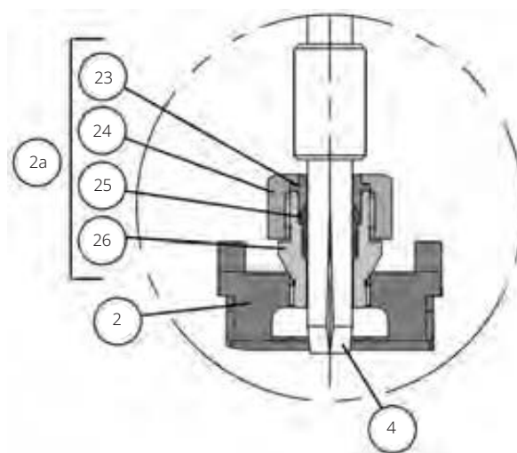
Figure 5. Optional 177 Low Flow Trim Assembly
