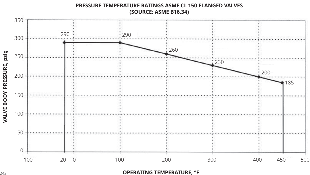
Figure 5. Pressure-Temperature Ratings
