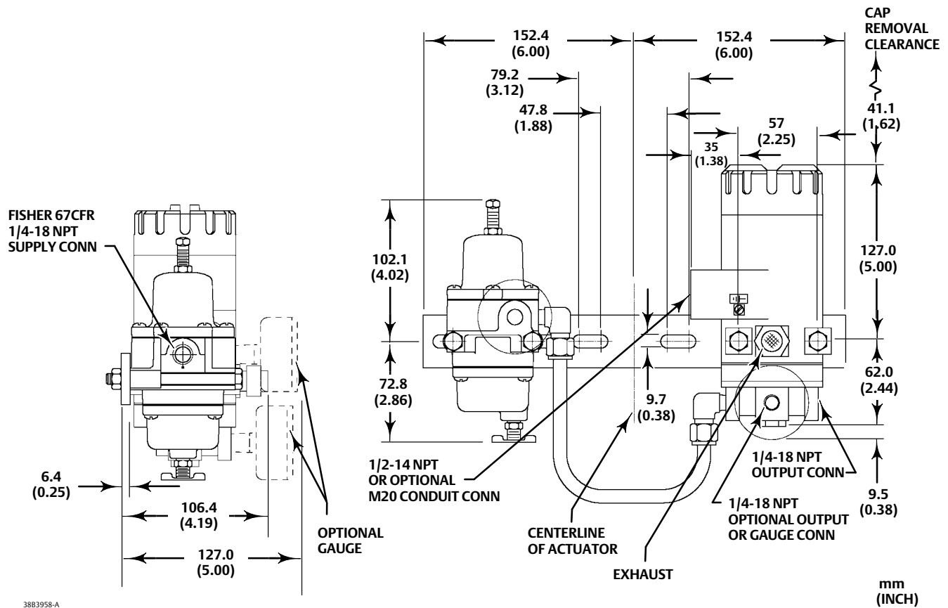
Figure 3. Dimensions
