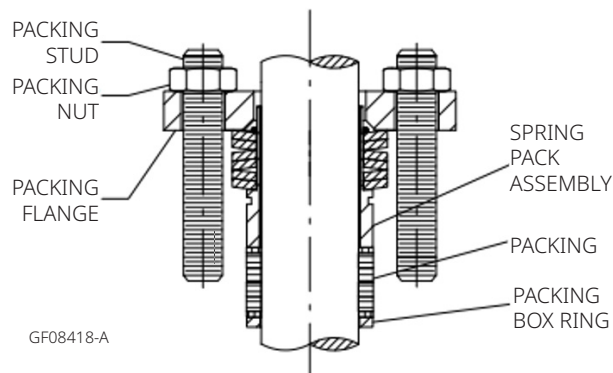
Figure 6. Fisher Vee-Ball Valve with Enhanced ENVIRO-SEAL IS Packing Arrangement
