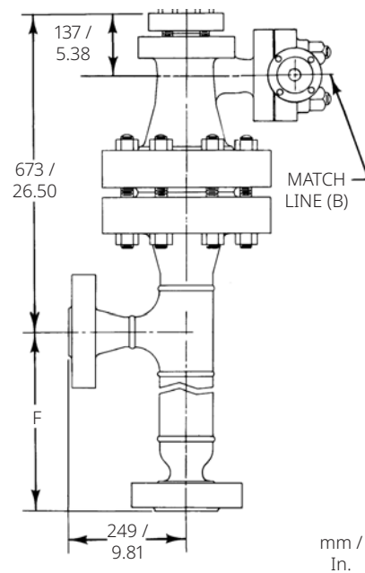
F4 UPPER SIDE AND BOTTOM CONNECTIONS (NPS 2 RTJ FLG.)
