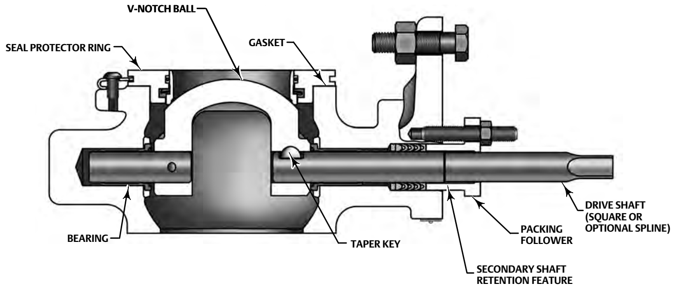
Figure 2. Fisher V200U Construction Features, DN 80 through DN 100 (NPS 3 and 4)
