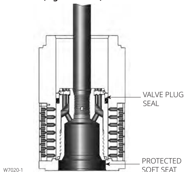
Figure 19. Typical Balanced TSO (Tight Shutoff) Trim
