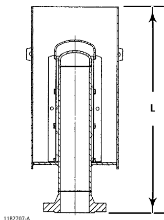
Figure 6. Fisher 6013 Vent Diffuser Dimensions
