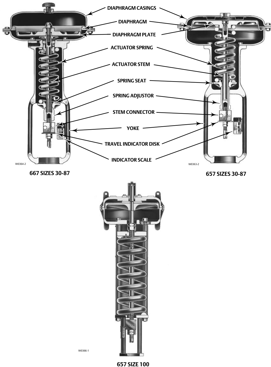
Figure 1. Typical Actuators
