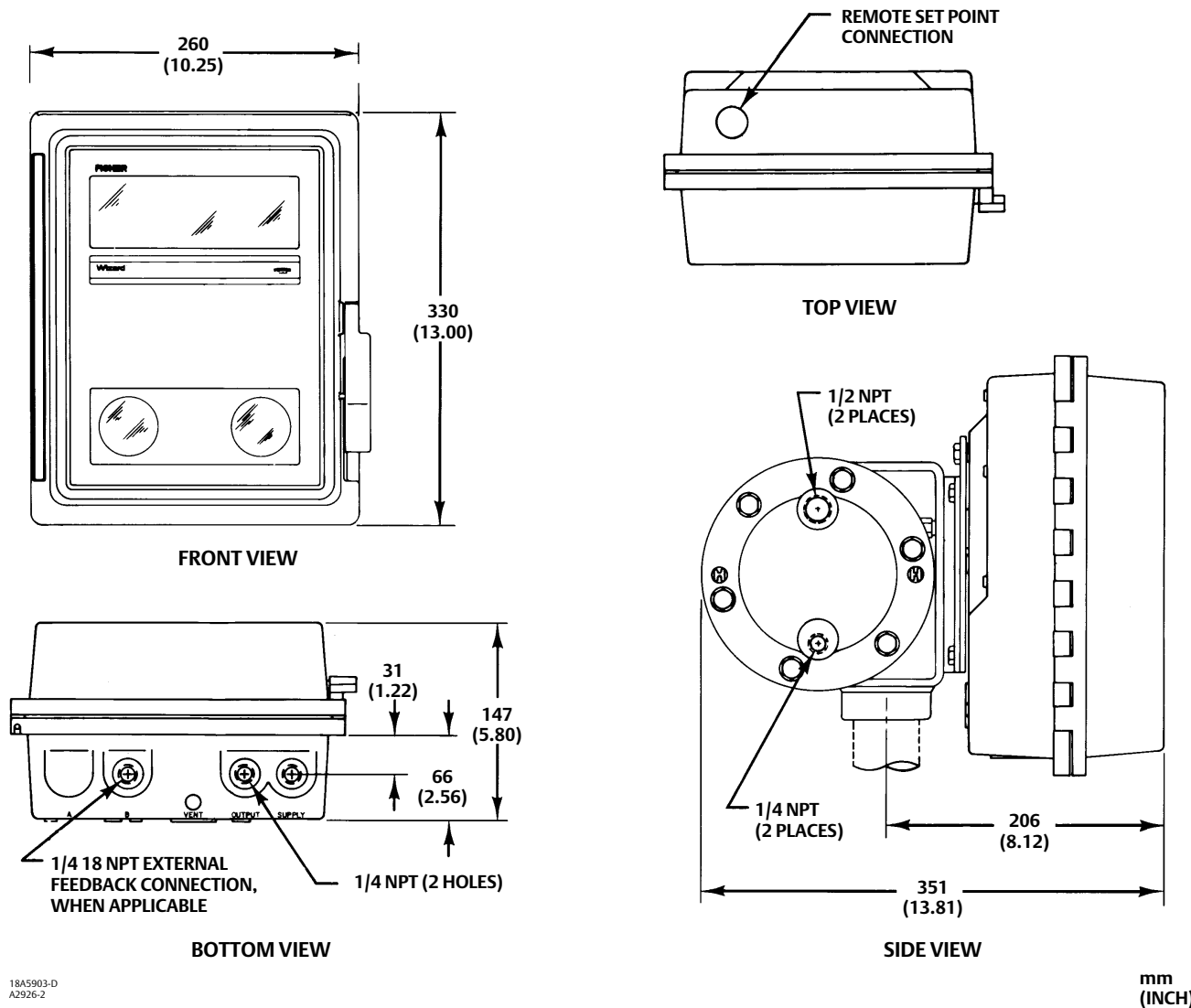
Figure 5. Dimensions
