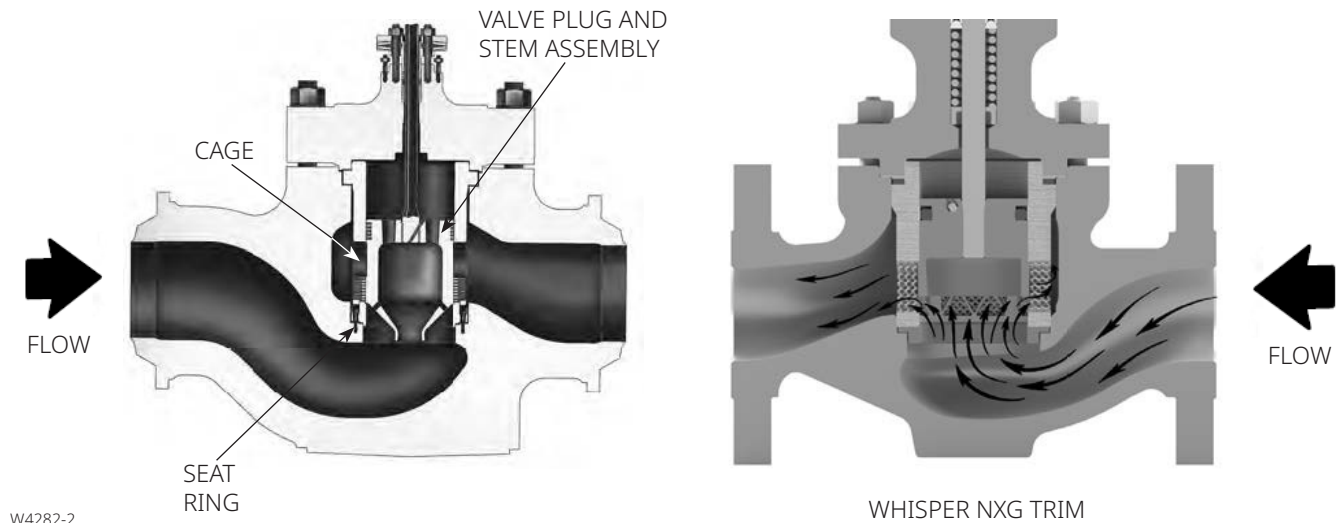
Figure 14. Sectional of NPS 20 Fisher EHD Control Valve Assembly
