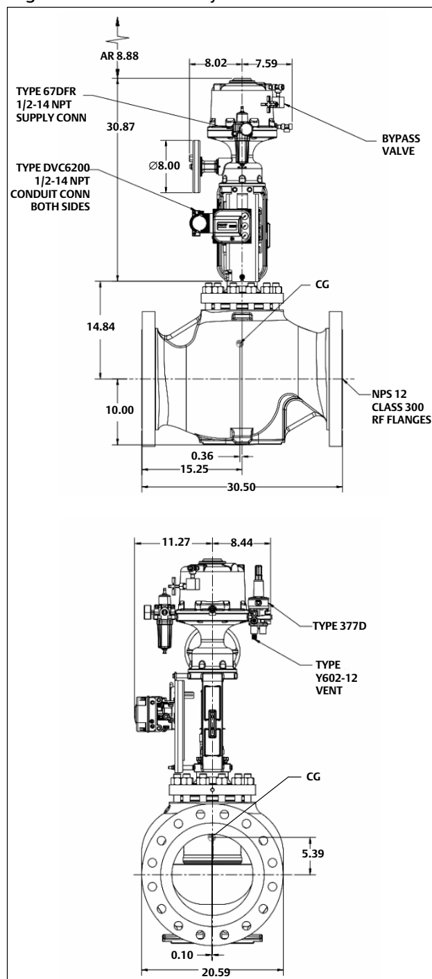
Figure 1. Center of Gravity
