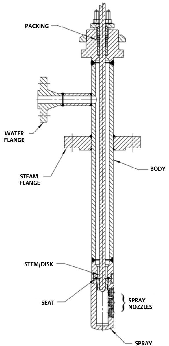
Figure 2. Yarway AT-38/48
