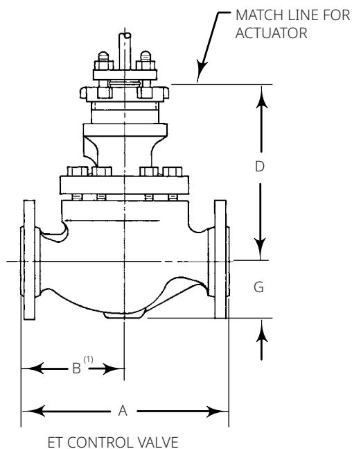
Figure 16. Fisher ET and ETR Dimensions (Also See Tables 25, 26 and 27)
