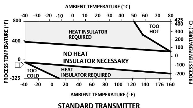
Figure 2. Guidelines for Use of Optional Heat Insulator Assembly
