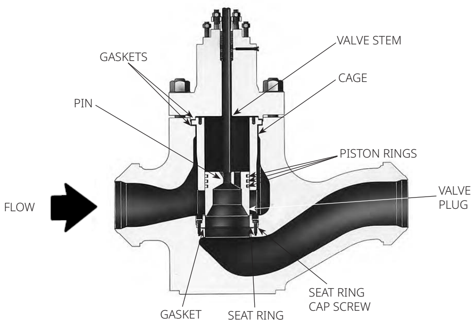
Figure 8. Fisher EHD Valve Assembly (NPS 8 through 14 Globe Valves)
