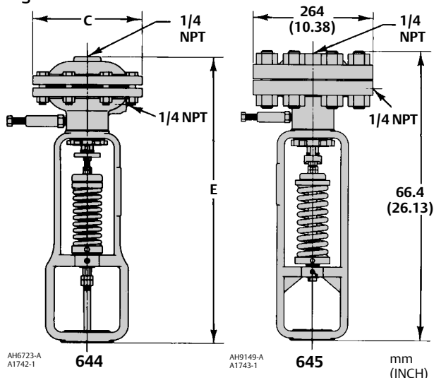
Figure 3. Dimensions
