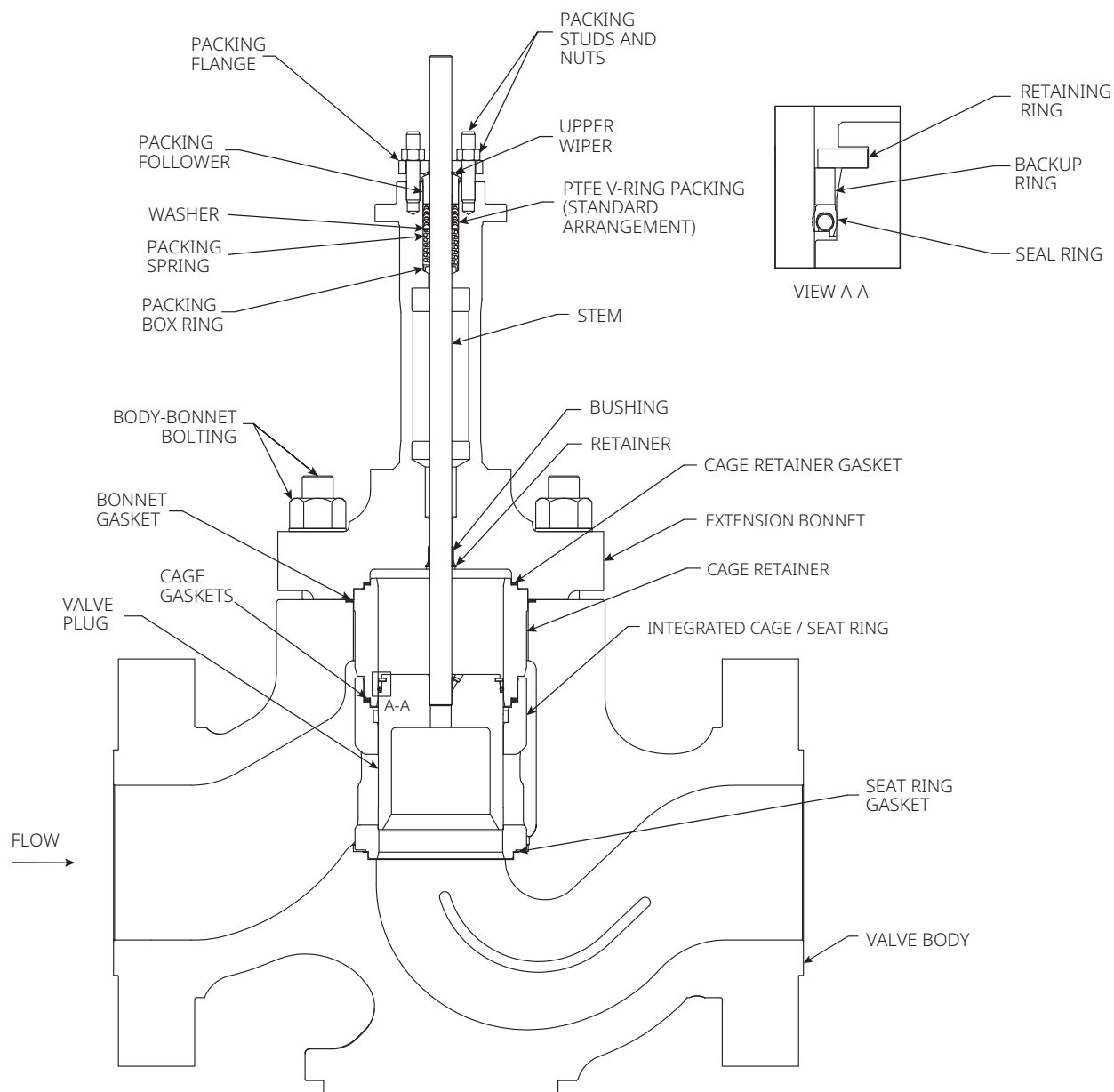
Figure 4. Fisher HPT-C Valve Assembly Detail with Fabricated Extension Bonnet NPS 8 through 12 (Long)
