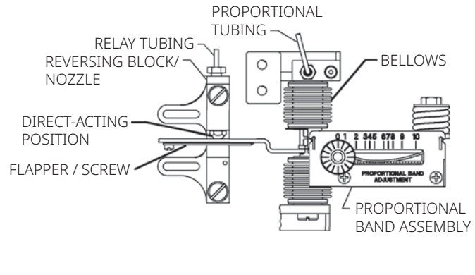
DIRECT-ACTING
