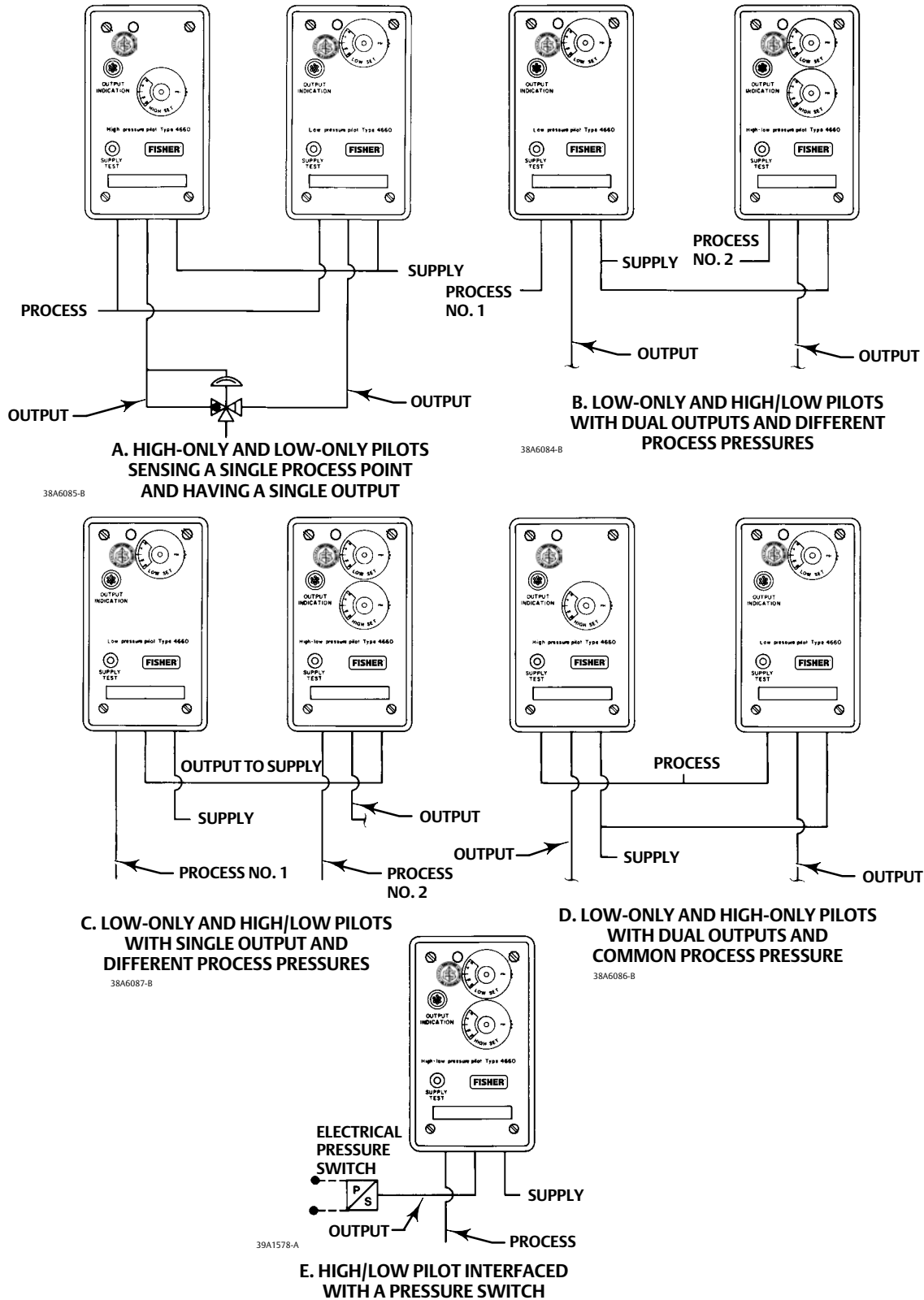
Figure 5. Typical Connection Schematics
