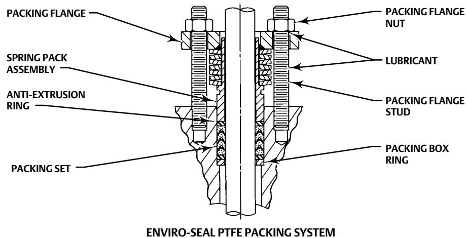
ENVIRO-SEAL PTFE PACKING SYSTEM
