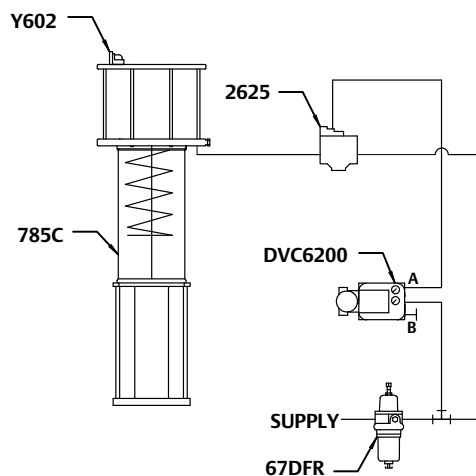
Figure 3. Fisher 785C Single-Acting Spring Return Installation Example
