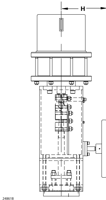
LEFT VIEW OF ACTUATOR WITH HANDWHEEL MANUAL OVERRIDE
