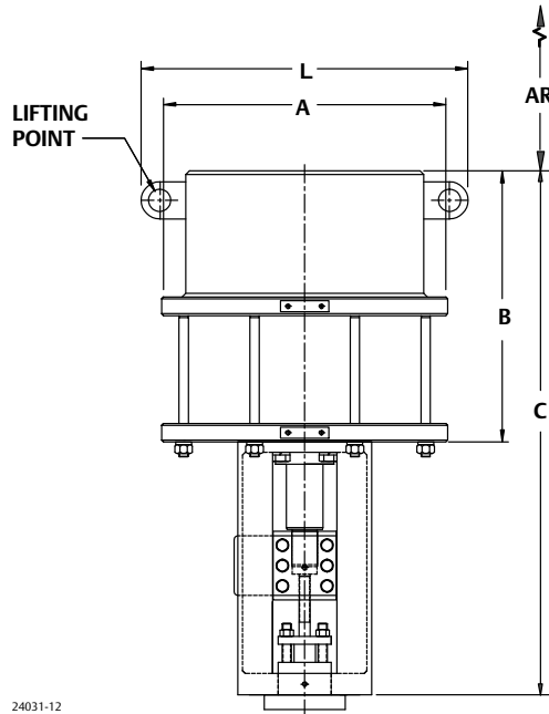
FRONT VIEW OF ACTUATOR WITHOUT MANUAL OVERRIDE
