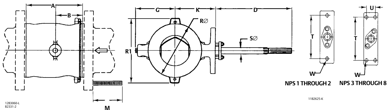
Figure 3. Fisher Flangeless SS-252B Dimensions (also see table 6)
