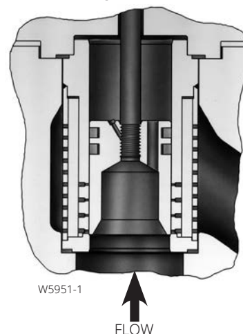
Figure 17. Fisher HPAS Trim with Micro-Flat Valve Plug
