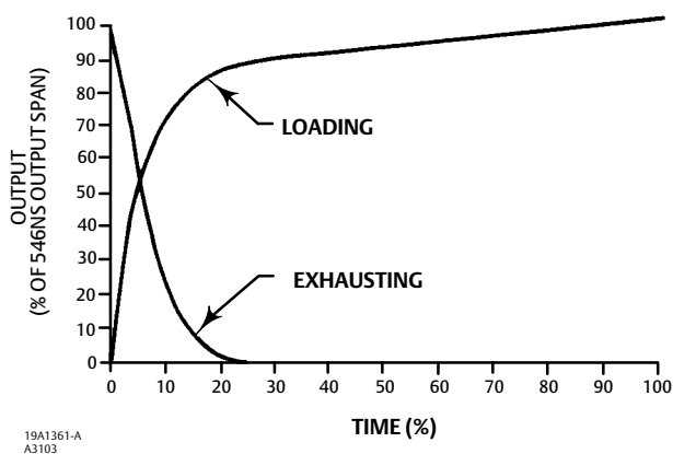
Figure 3. Output-Time Relationships
