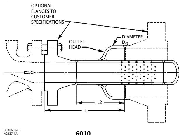
Figure 2. Fisher 6010 Diffuser Dimensions
