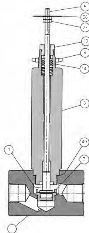
Figure 3. Valve Body with Extension Bonnet
