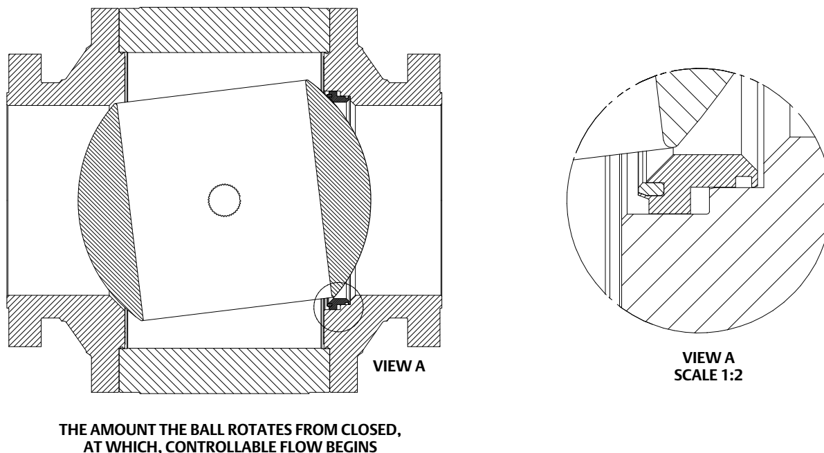
Figure 4. Dead Angle (also see table 4)
