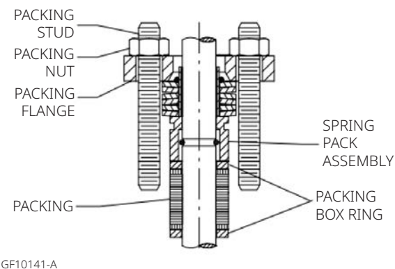
Figure 5. Fisher 8580 and Control-Disk Valves with Enhanced ENVIRO-SEAL IS Packing Arrangement
