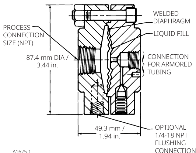
Figure 2. Internal Construction and Dimensions of Bowl
