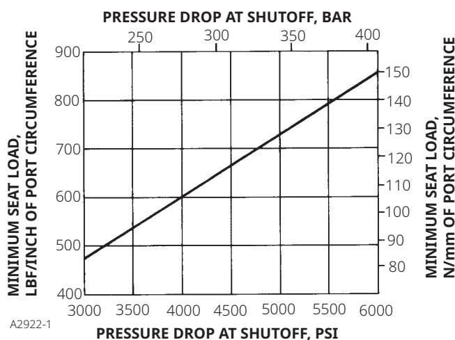
Figure 7. Recommended Seat Load Force for All Constructions
