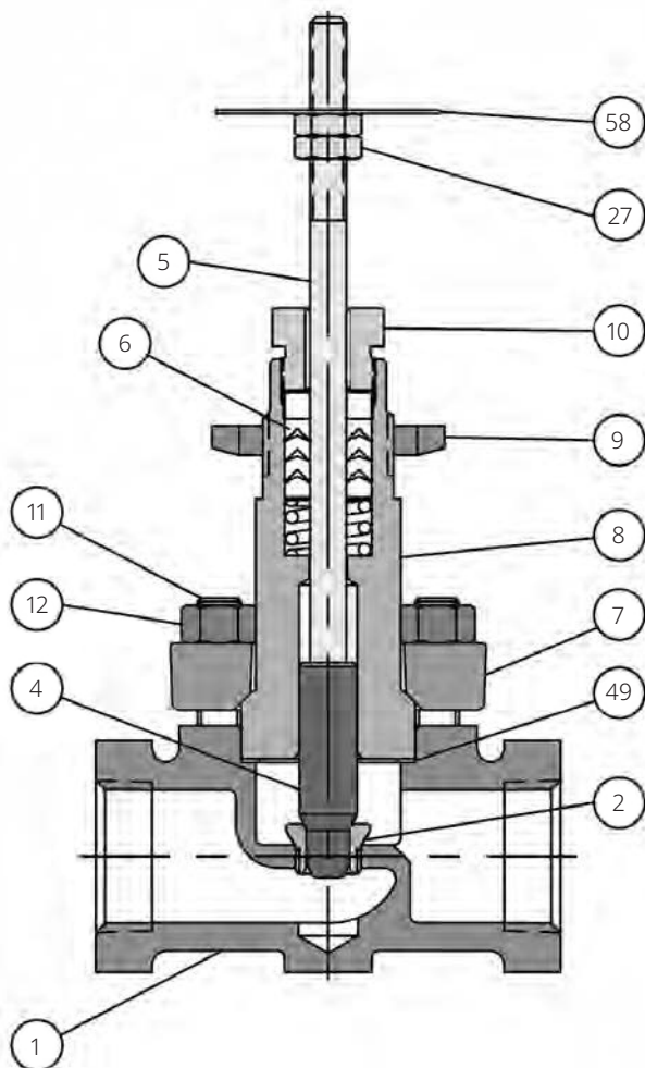
Figure 1. 24000S Valve Body Assembly
