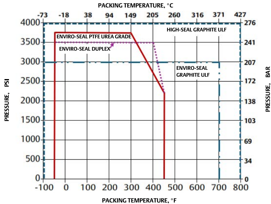
Figure 5. Application Guidelines for EHU Packing
