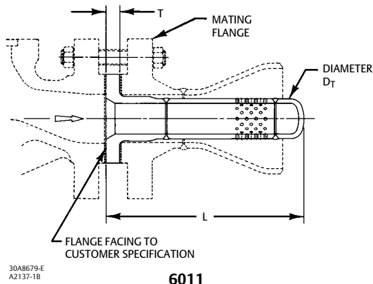
Figure 3. Fisher 6011 Diffuser Dimensions
