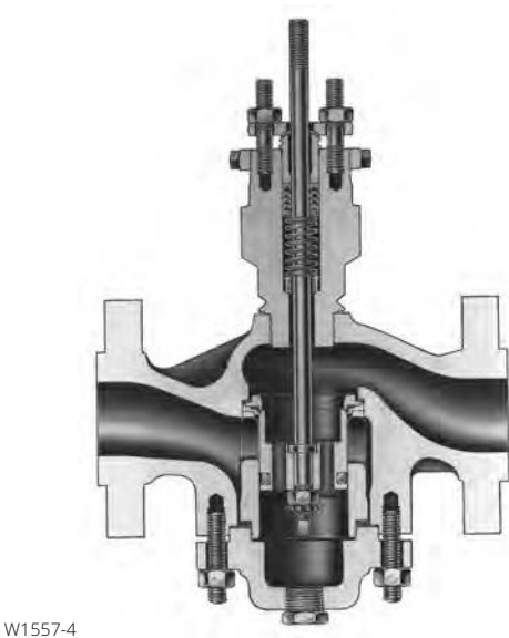
Figure 5. Fisher ETR Sectional
