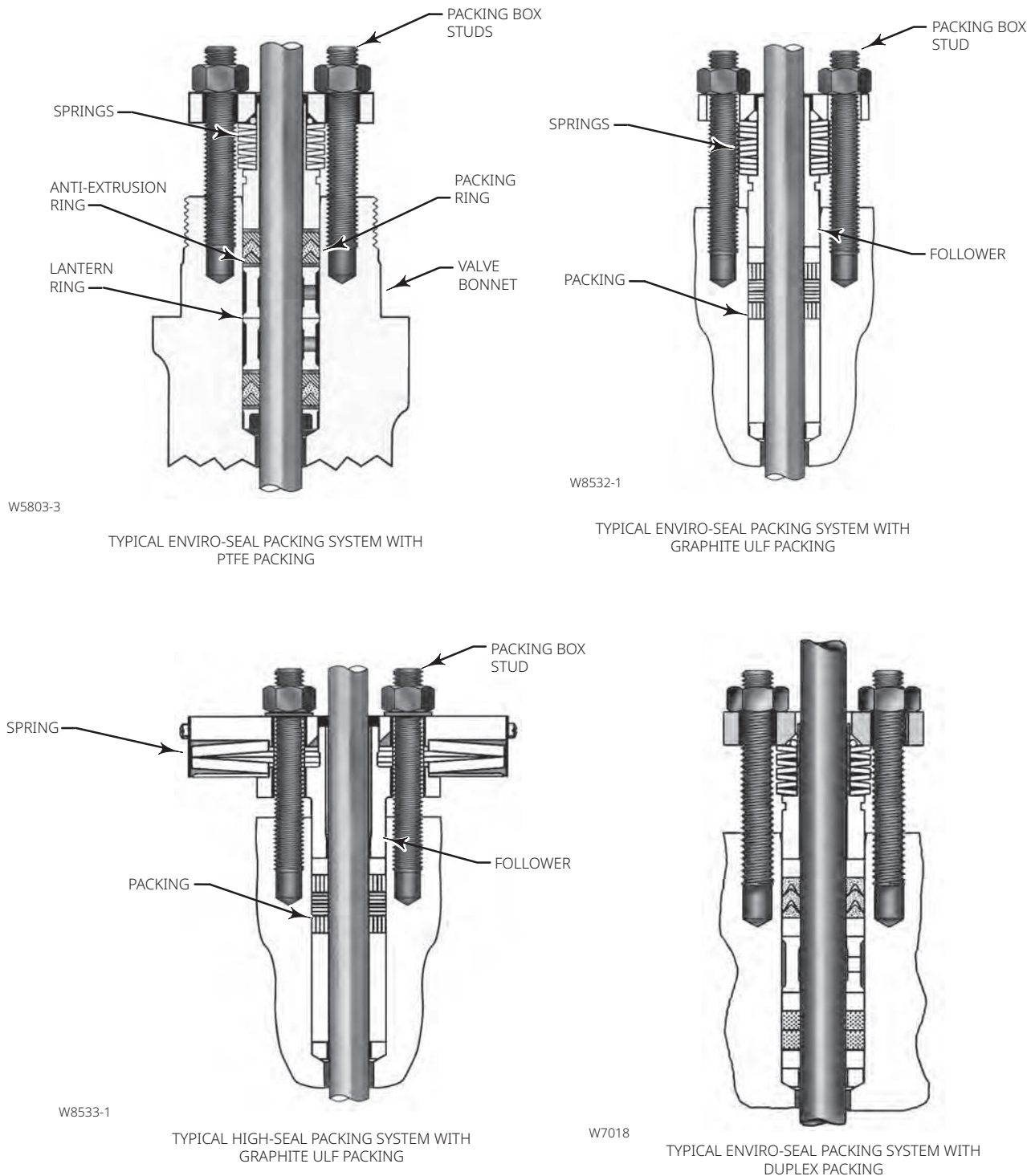
Figure 12. ENVIRO-SEAL and HIGH-SEAL Packing Systems
