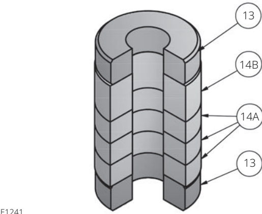
Figure 4. Molded Graphite (Flexible Graphite) Packing Kit (Optional)
