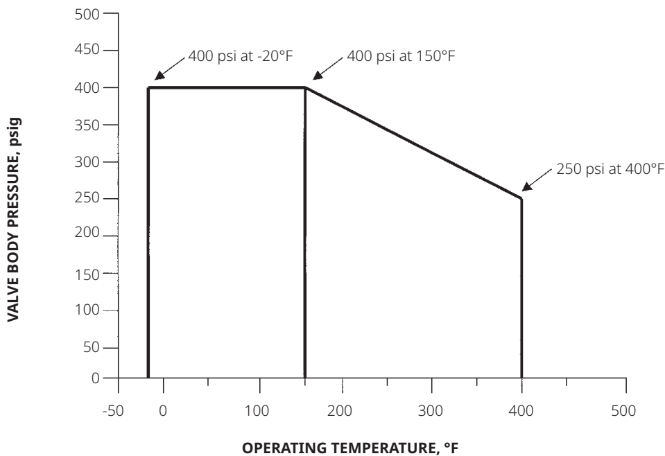
Figure 5. 24000 Pressure-Temperature Ratings
