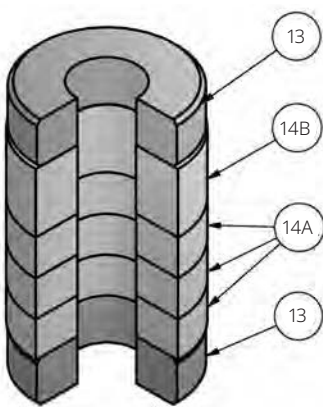
Figure 7. Molded Graphite (Flexible Graphite) Packing Kit (Optional)
