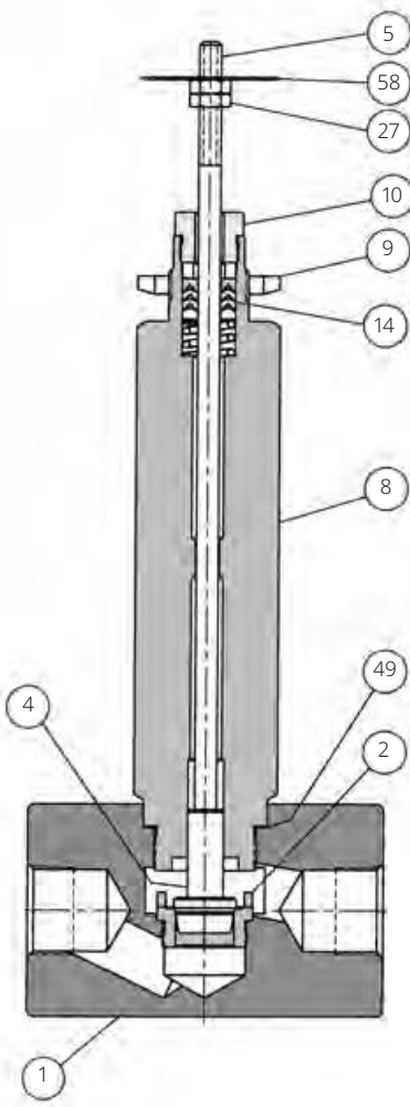
Figure 3. Valve Body with Extension Bonnet
