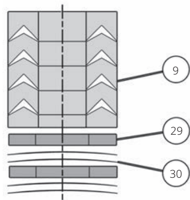
Figure 5. V-Ring Packing Kit
