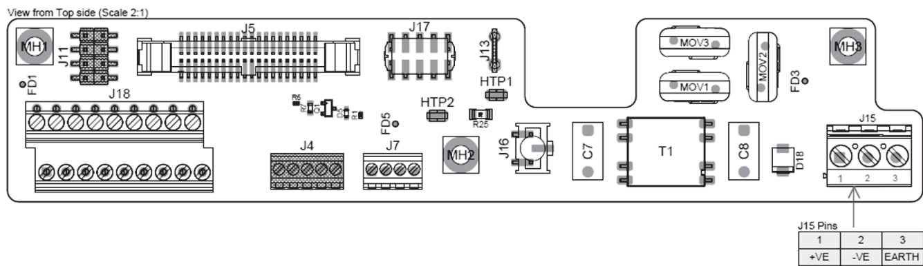
Figure 18. J15 Connector Board
