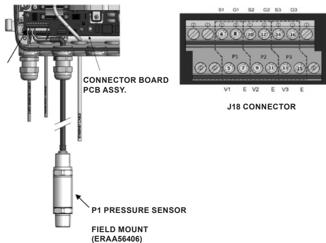
Figure 14. Pressure Sensor Installation
