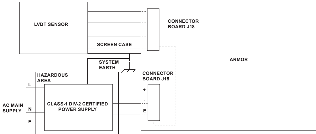
Figure 5. Hazardous Area Installation with Power Supply
