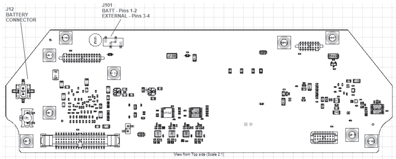
Figure 17. Battery Power Source Connection for ARMOR™ 8000 Series
