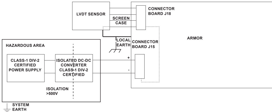
Figure 6. Isolated DC-DC Converter Installation
