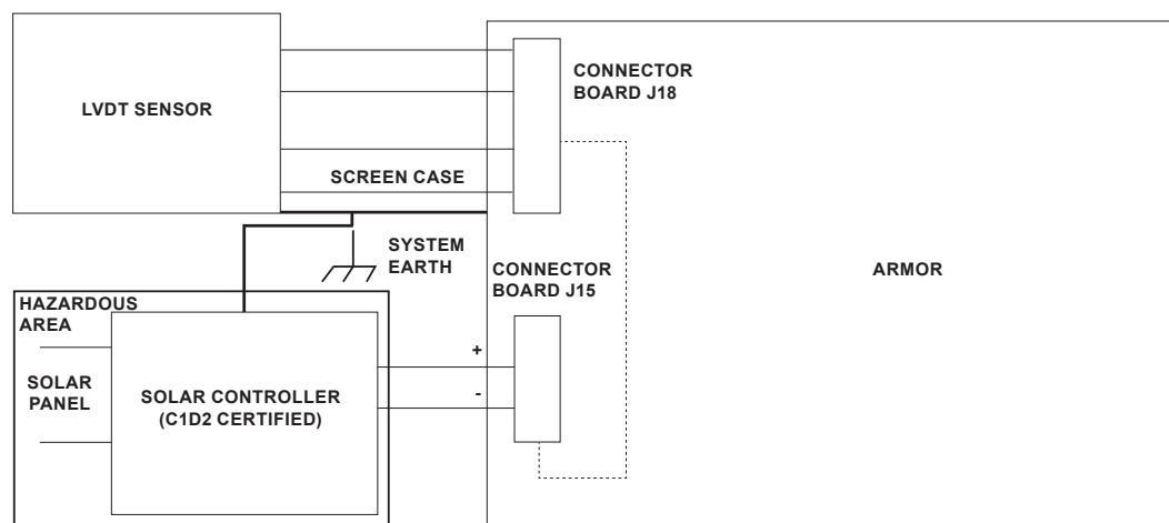
Figure 7. Hazardous Area Installation with Solar Controller
