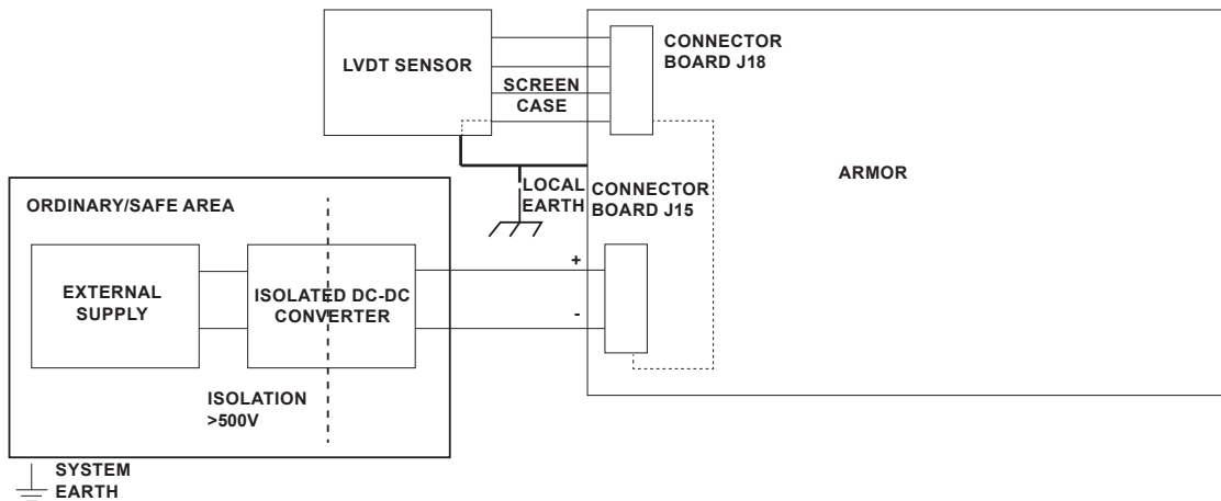
Figure 10. Isolated DC-DC Converter Installation for Safe Area
