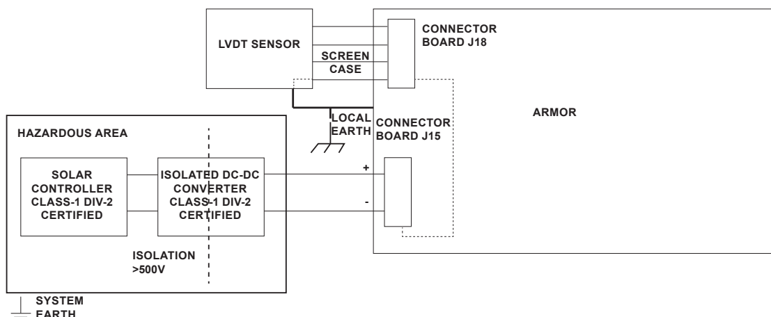
Figure 8. Class-1 Division-2 Certified Isolated DC-DC Converter Installation
