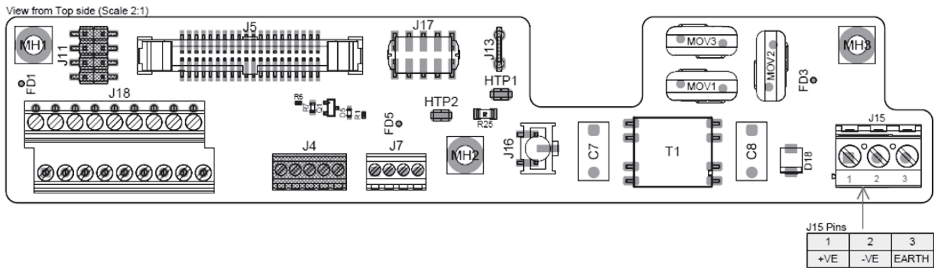
Figure 12. Screw Terminal Diagram for ARMOR 8000 Series Power Supply
