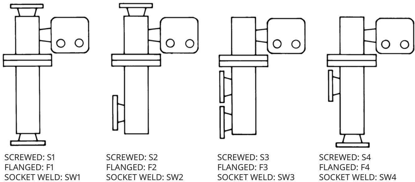
Figure 10. Cage Connection Styles
