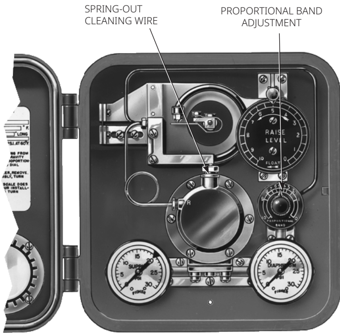
DIRECT-ACTING 2500 CONTROLLER
