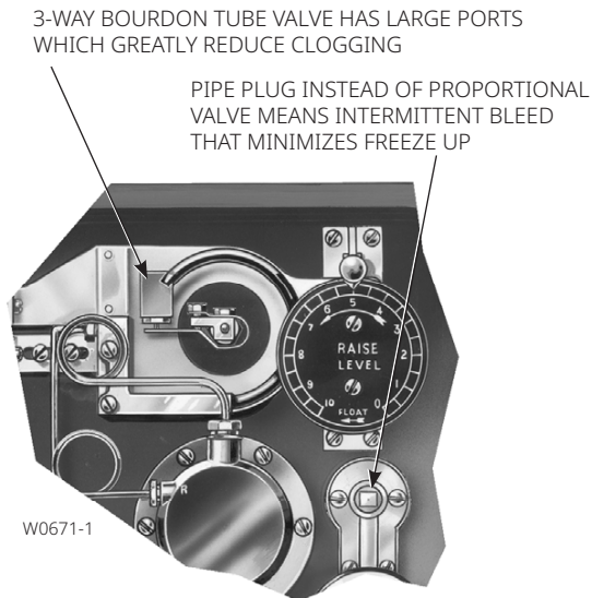
DETAIL OF REVERSE-ACTING 2503R ON/OFF CONTROLLER
