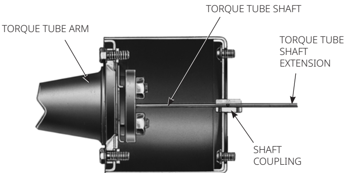
Figure 8. Optional Heat Insulator Assembly
