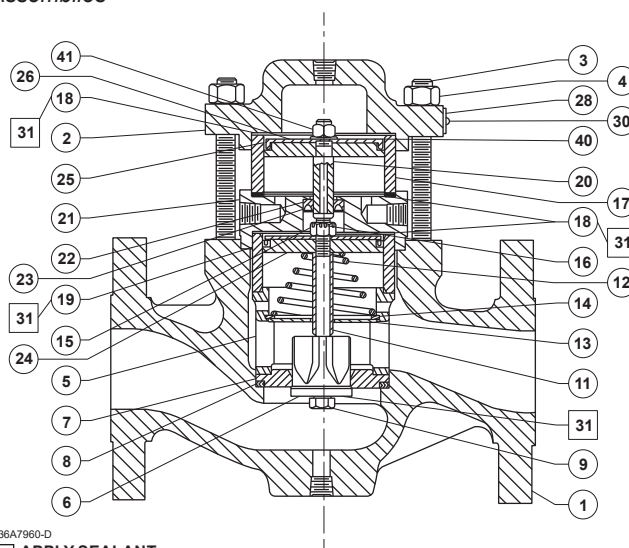
NPS 1, 1-1/2 OR 2 / DN 25, 40 OR 50 BODY SIZE
