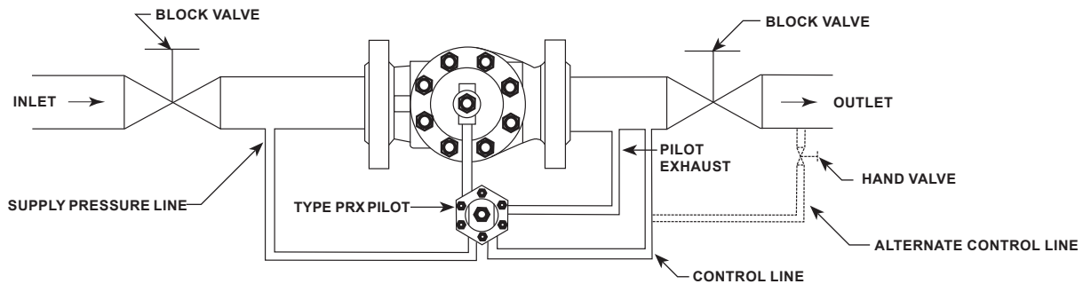
Figure 3. Typical Type EZR Single Installation Schematics
