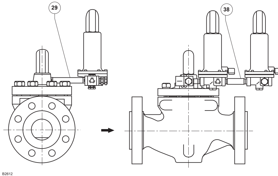
Figure 23. Pounds to Pounds (161EB Series Pilots) Working Monitor Mounting Parts
