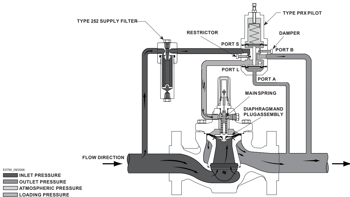
TYPE EZR WITH PRX SERIES PILOT AND TYPE 252 FILTER
