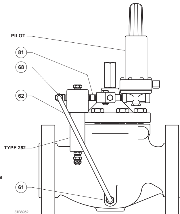
Figure 25. Pre-piped Type EZR with Type 161EB Pilot, Type 112 Restrictor and Type 252 Pilot Supply Filter
