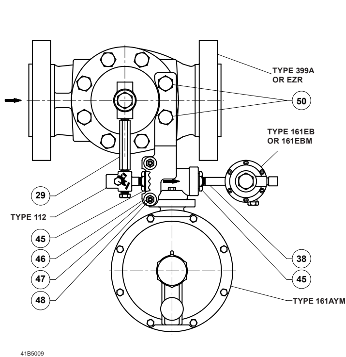
Figure 24. Pounds to Inches (161AY/161EB Series Pilots) Monitor System Mounting Parts
