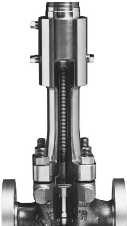
Figure 4. ENVIRO-SEAL Bellows Seal Bonnet
