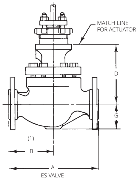
Figure 7. Fisher ES Dimensions (also see Tables 14, 15 and 16)
