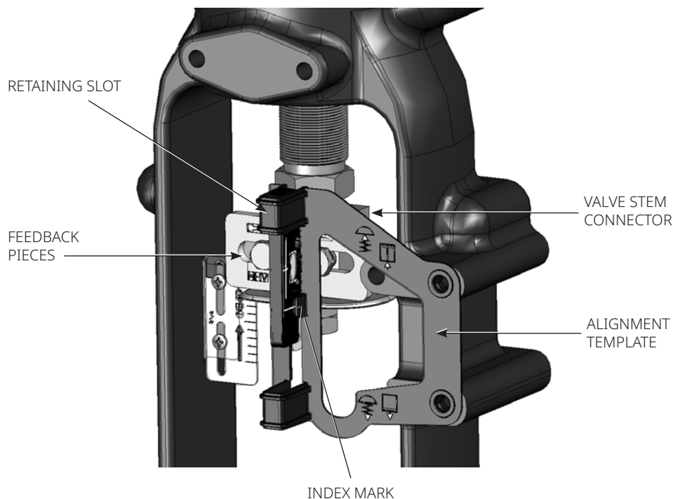
Figure 8. Air-to-Close Magnet Assembly Alignment
