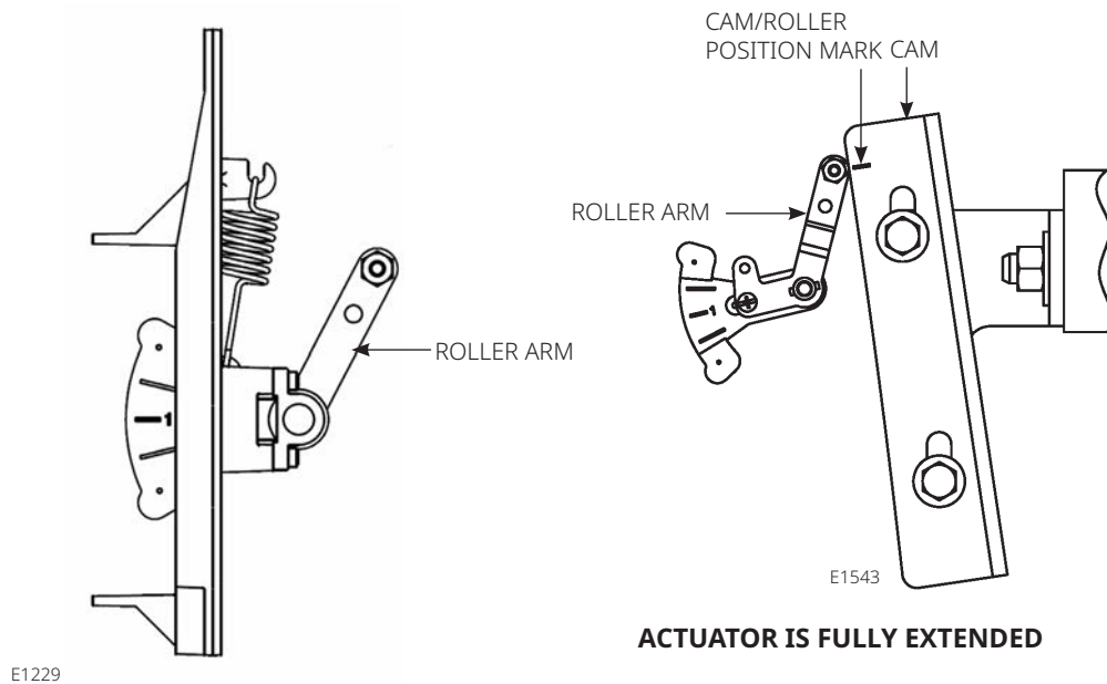
Figure 5. Roller Arm Variation used for Sliding-Stem (Linear) Actuators over 210 mm / 8.25 in. Travel
