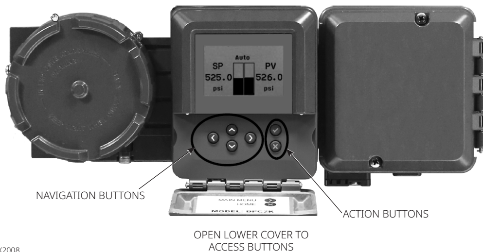
Figure 27. Local User Interface
