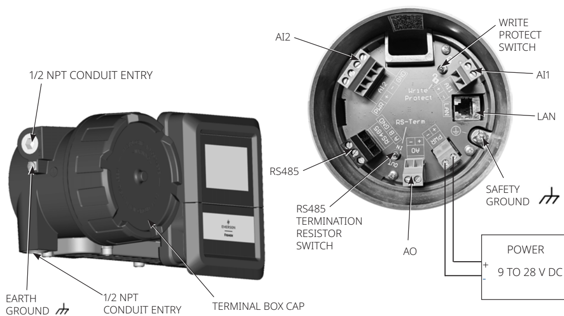
Figure 16. Terminals, Connections, and Grounds
