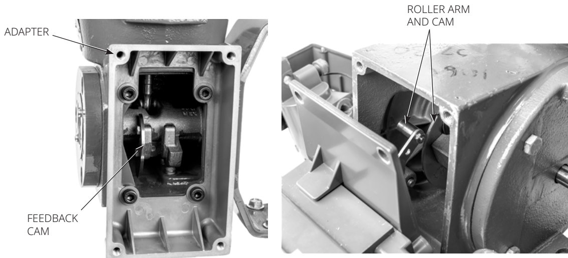
Figure 11. Integral Mounted Fisher Actuators
