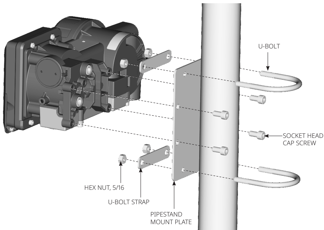
Figure 12. Pipestand Mounting Kit
