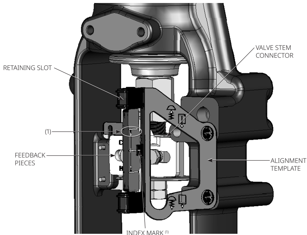
Figure 6. Air-to-Open Magnet Assembly Alignment
