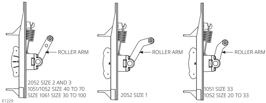
Figure 10. Rotary Actuator Mounting Variations
