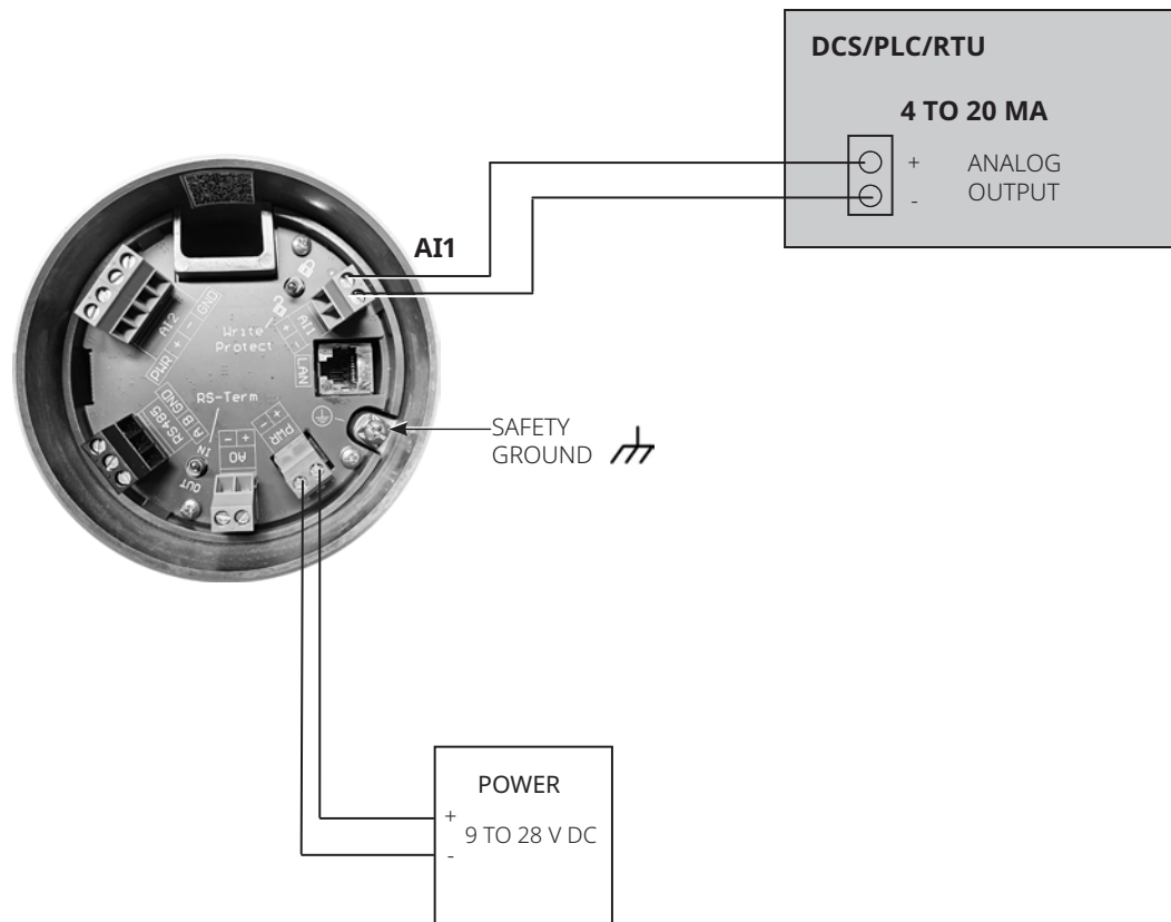
Figure 22. Remote Setpoints (Connecting with DCS, PLC, RTU's)
