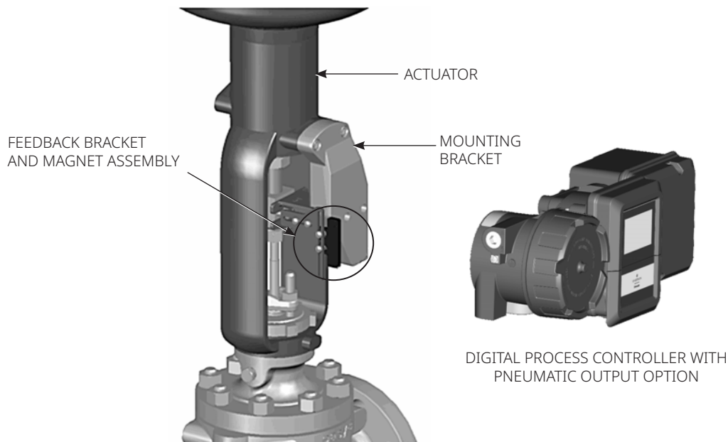
Figure 2. Mounting Parts for Sliding-Stem Actuator with Up to 210 mm / 8.25 in. Travel
