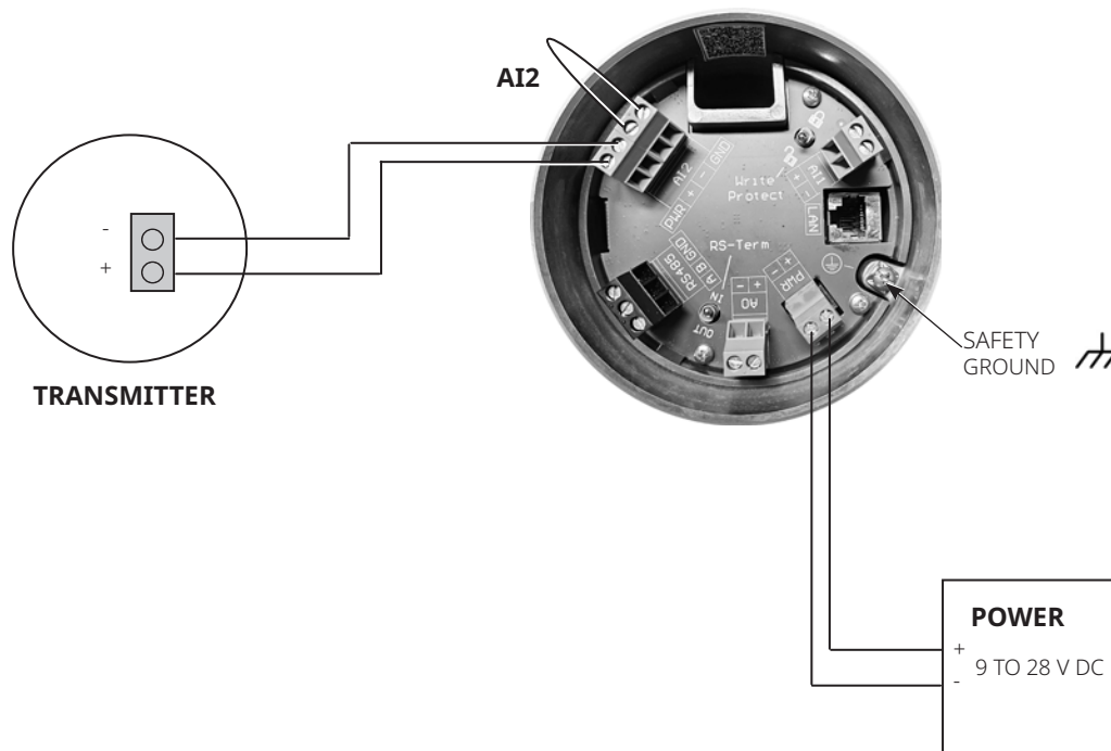
Figure 18. Loop Powered Transmitters
