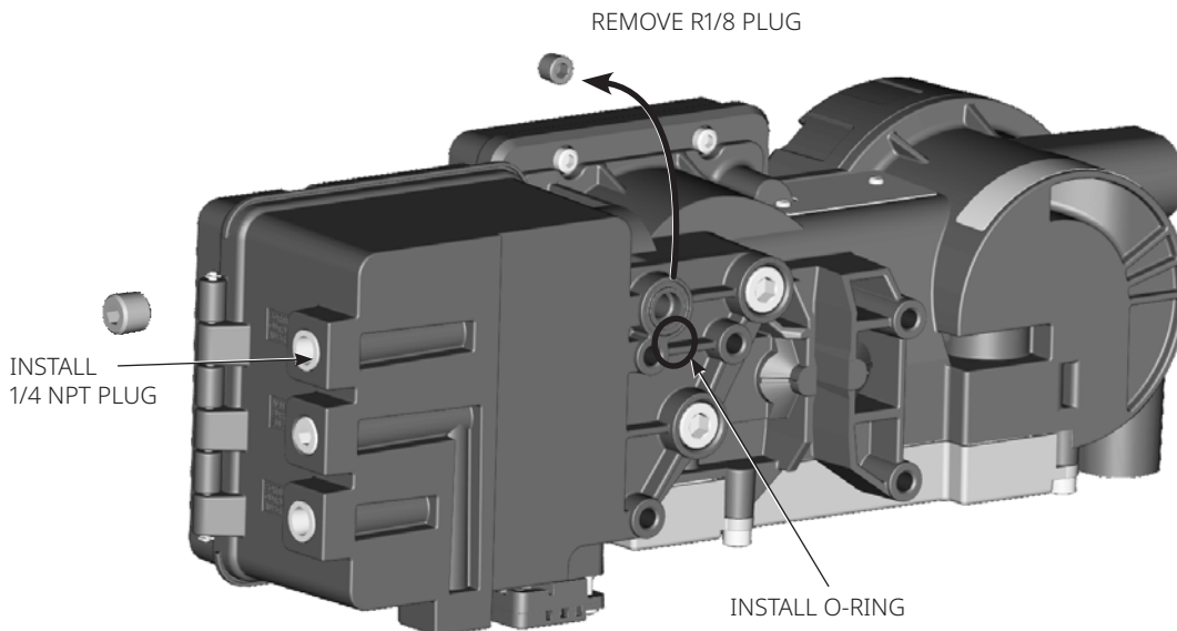
Figure 7. Modifications for Integral Mounted Actuator; Air-to-Open Construction Only
