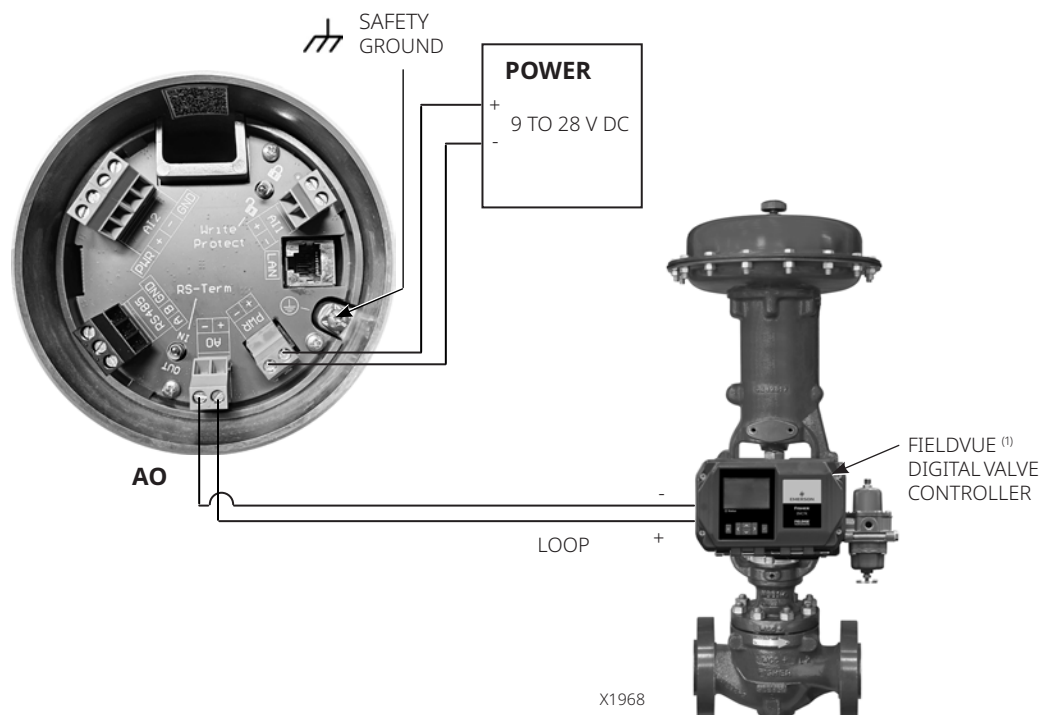
Figure 23. Analog Output Wiring Schematic, with FIELDVUE Digital Valve Controller
