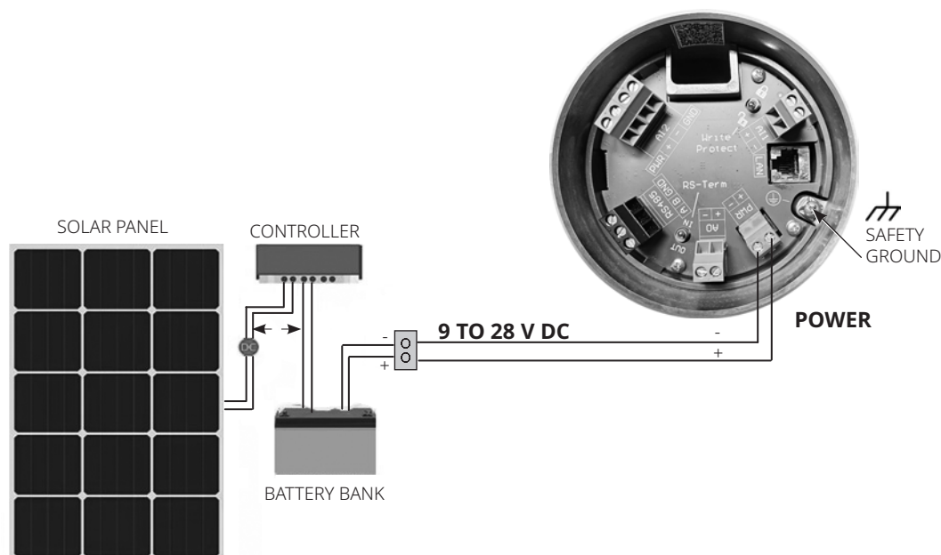
Figure 17. Power Using a Solar Panel
