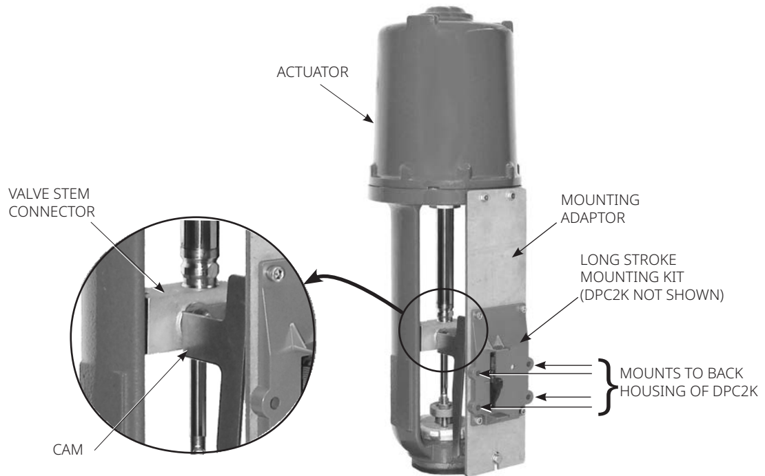
Figure 4. Mounting on Sliding-Stem (Linear) Actuators over 210 mm / 8.25 in. Travel
