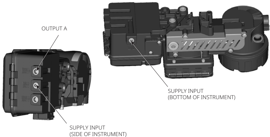
Figure 13. Supply Inputs and Outputs
