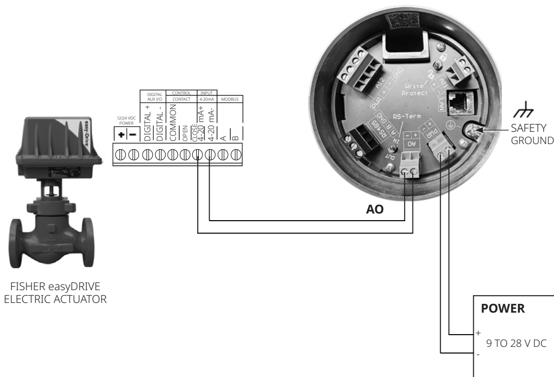
Figure 24. Analog Output Wiring Schematic, with Fisher easyDrive Electric Actuator
