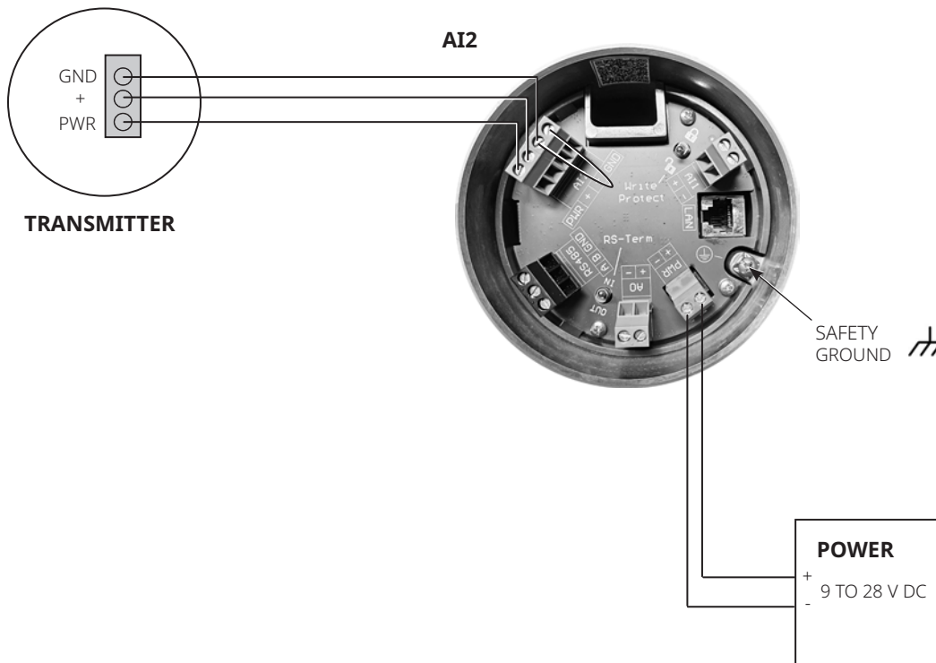
Figure 19. External DPC2K Powered 3-Wire Transmitters
