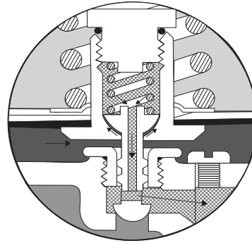
RESTRICTOR IN OPEN POSITION
