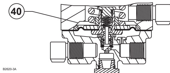
Figure 6. Types 6358EB and 6358EBH Pilots (continued)
