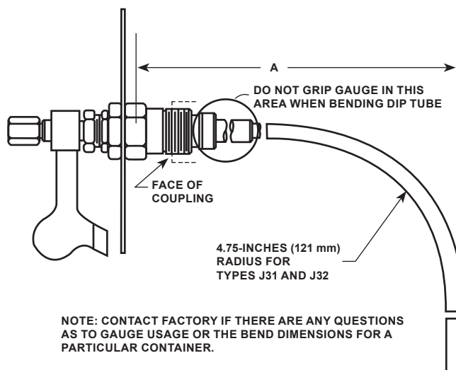
Figure 2. Types J31 and J32 Rotary Gauge Installation Schematic
