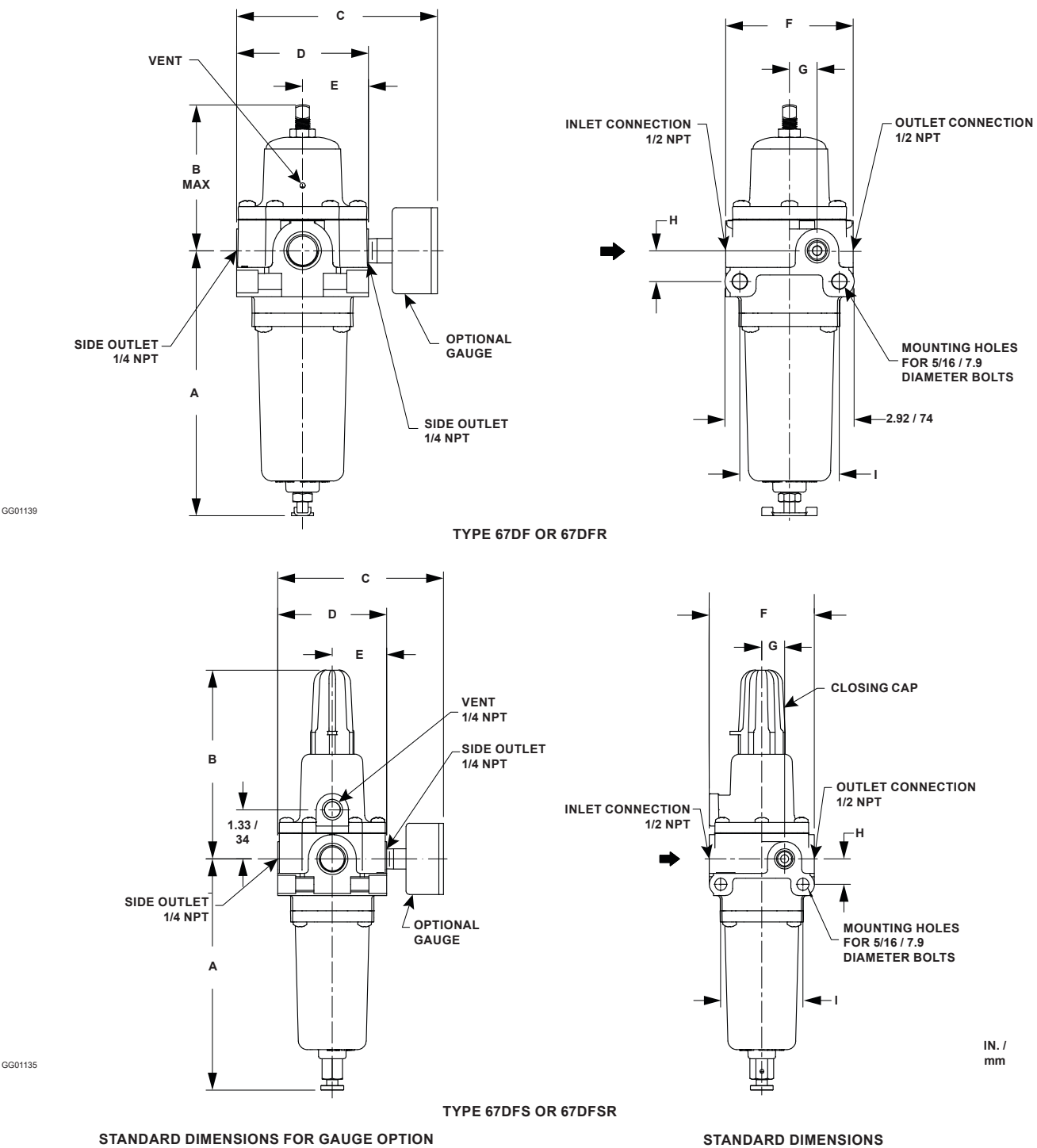
Figure 5. Types 67DF, 67DFR, 67DFS and 67DFSR Dimensions
