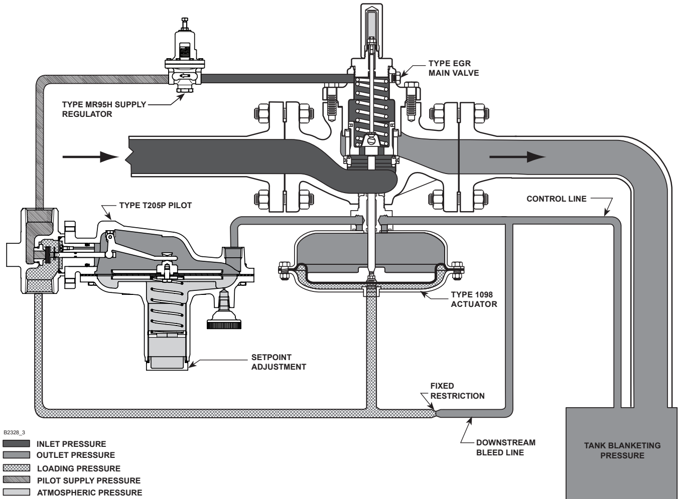
Figure 2. Operational Schematic
