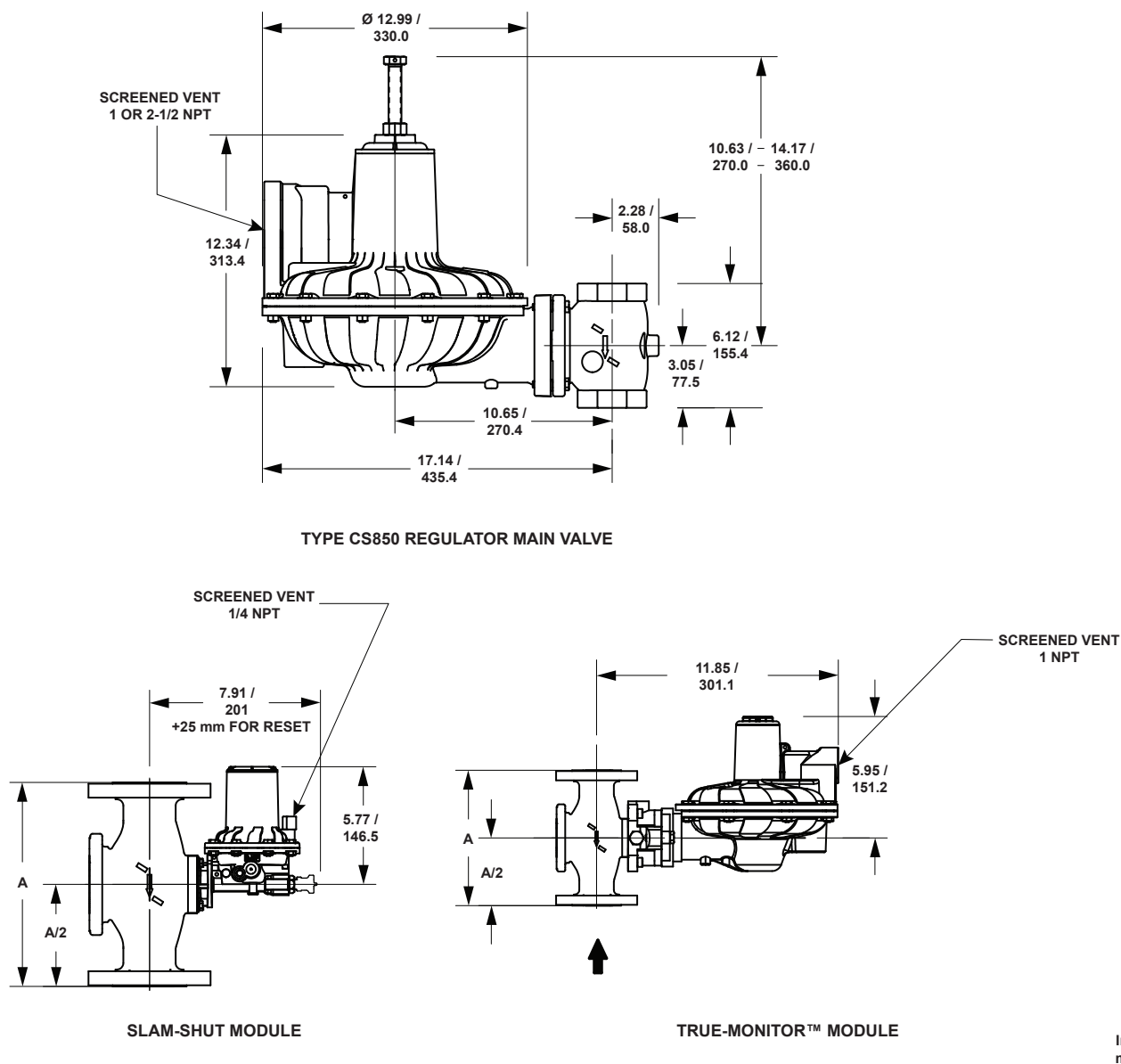
Figure 22. Dimensions (continued)
