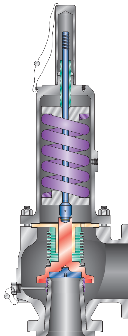
SERIES JBS-E (with metal-to-metal seat)
