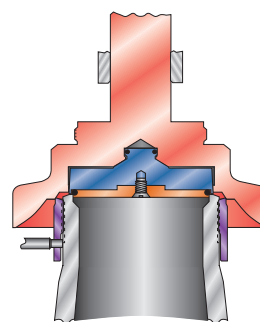
SERIES JLTJOS-E (with O-ring seat)
