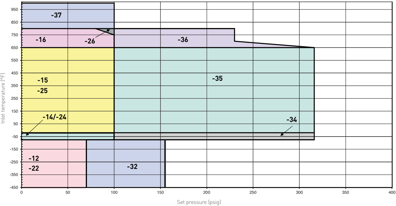
PRESSURE/TEMPERATURE LIMIT CHART W Orifice, 60.75 sq.in. [39193 sq.mm] API effective area
