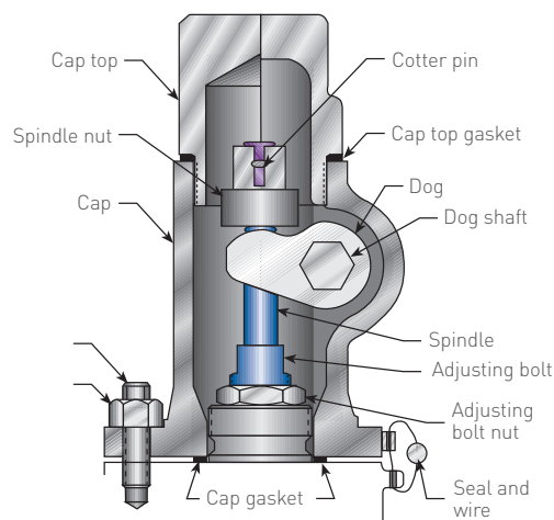
Packed lifting lever Type D
