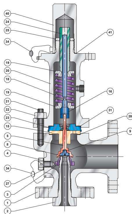
Series JDS-E (with Diaphragm)
