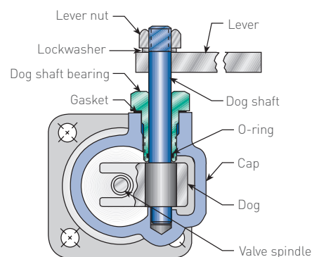
Packed lifting lever Type D (top view)
