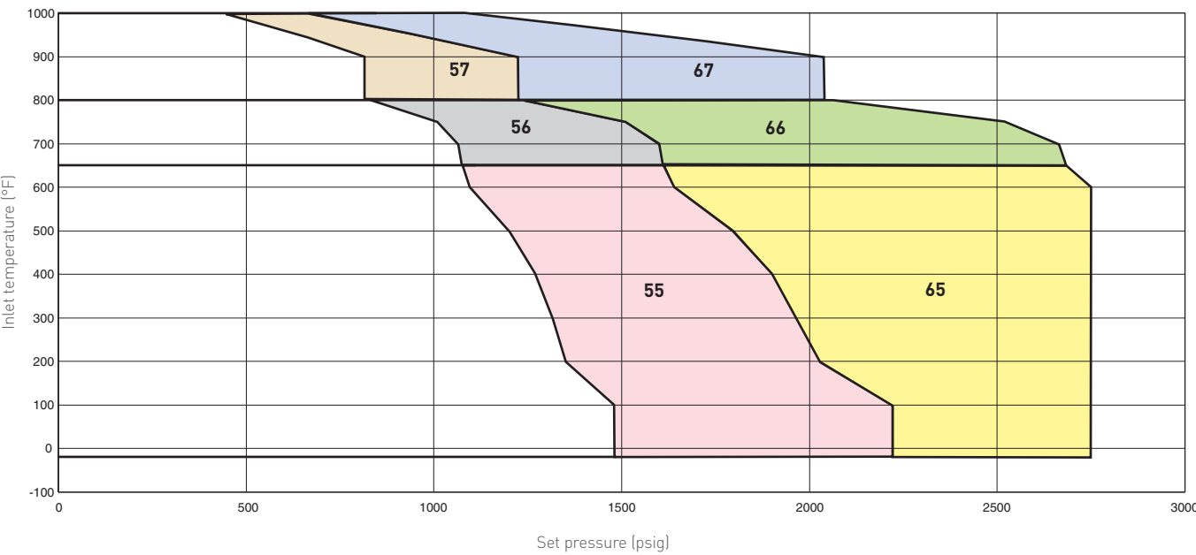
PRESSURE/TEMPERATURE LIMIT CHART - ANSI CLASS 900, CLASS 1500 H Orifice, 0.785 sq.in. (506 sq.mm) API effective area
