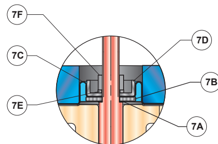
SERIES JDS-E (WITH DIAPHRAGM)
