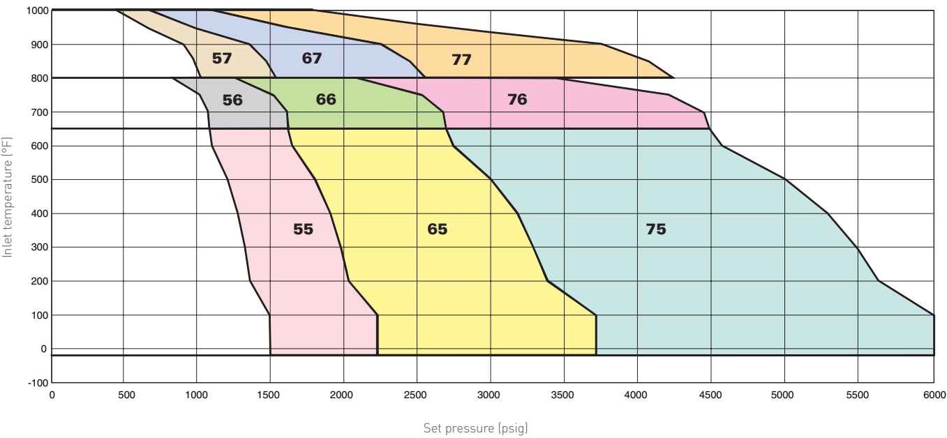
PRESSURE/TEMPERATURE LIMIT CHART - ANSI CLASS 900, CLASS 1500, CLASS 2500 E Orifice, 0.196 sq.in. [126 sq.mm] API effective area
