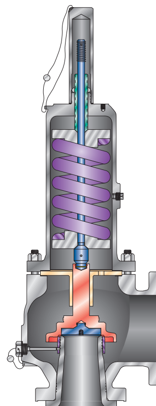
SERIES JOS-E (with metal-to-metal seat)
