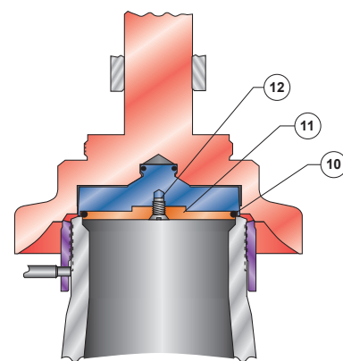
Series JLTJDS-E (with O-ring seat)
