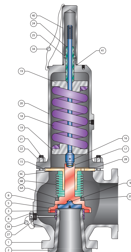
SERIES JBS-E (with bellows)
