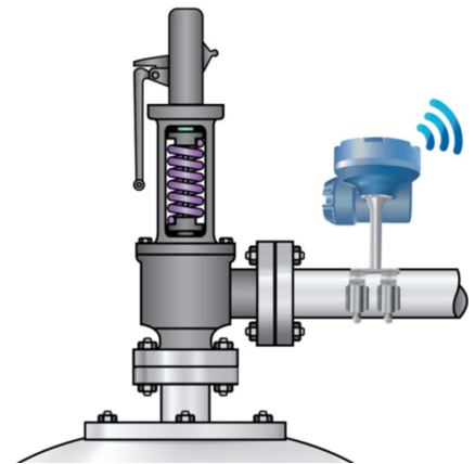
Installation of Acoustic Monitoring using Rosemount™ 708 on a Direct Spring Valve
