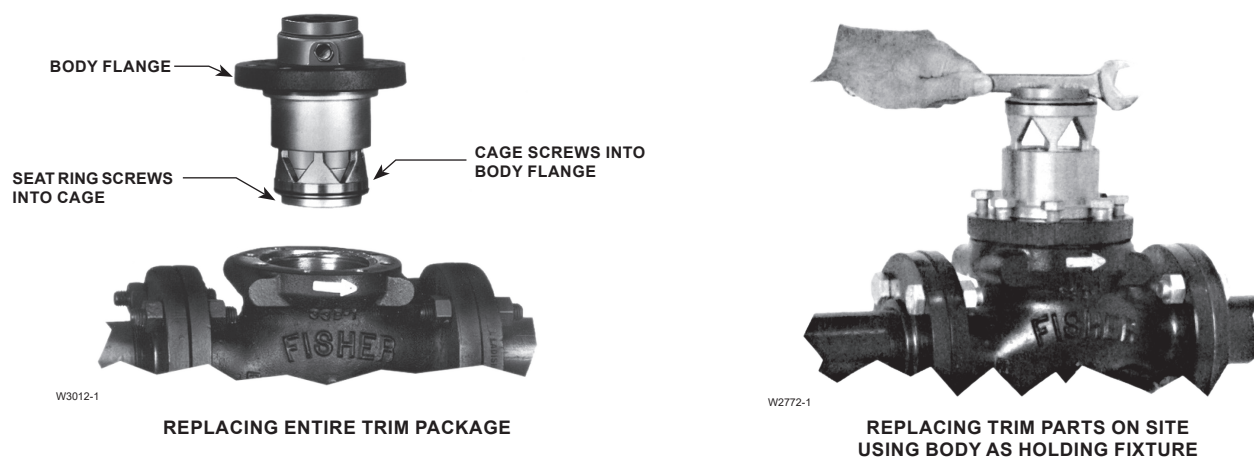
Figure 3. Easy-Maintenance Trim
