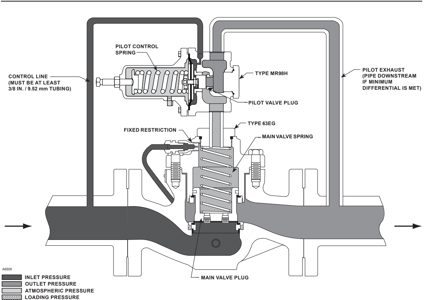
Figure 2. Operational Schematic
