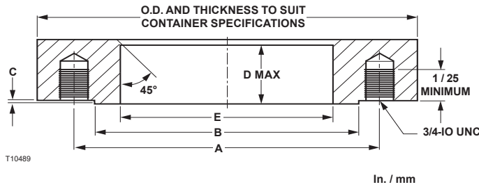
Figure 3. Tank Flange Dimensions
