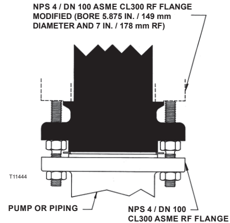
Figure 4. Valve Installation Schematic
