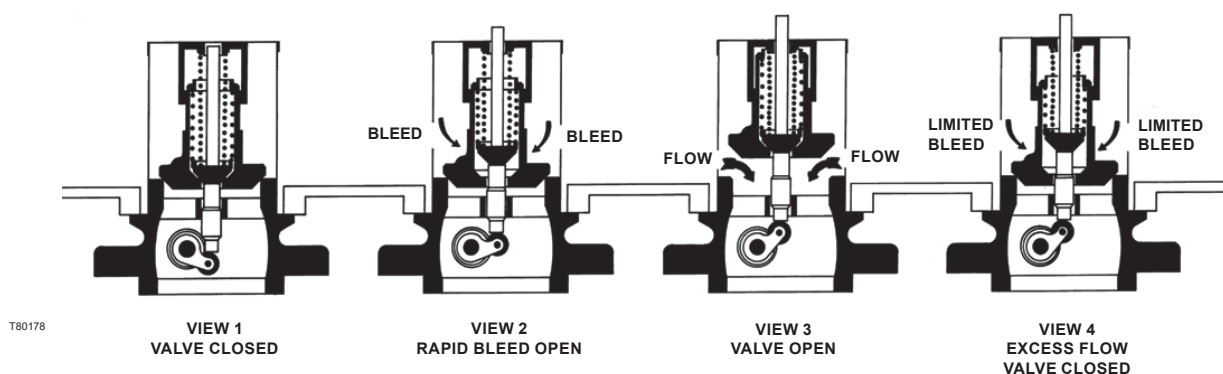
Figure 2. Operational Schematic
