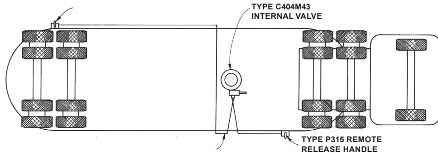
Figure 6. Type P315 Installation Schematic
