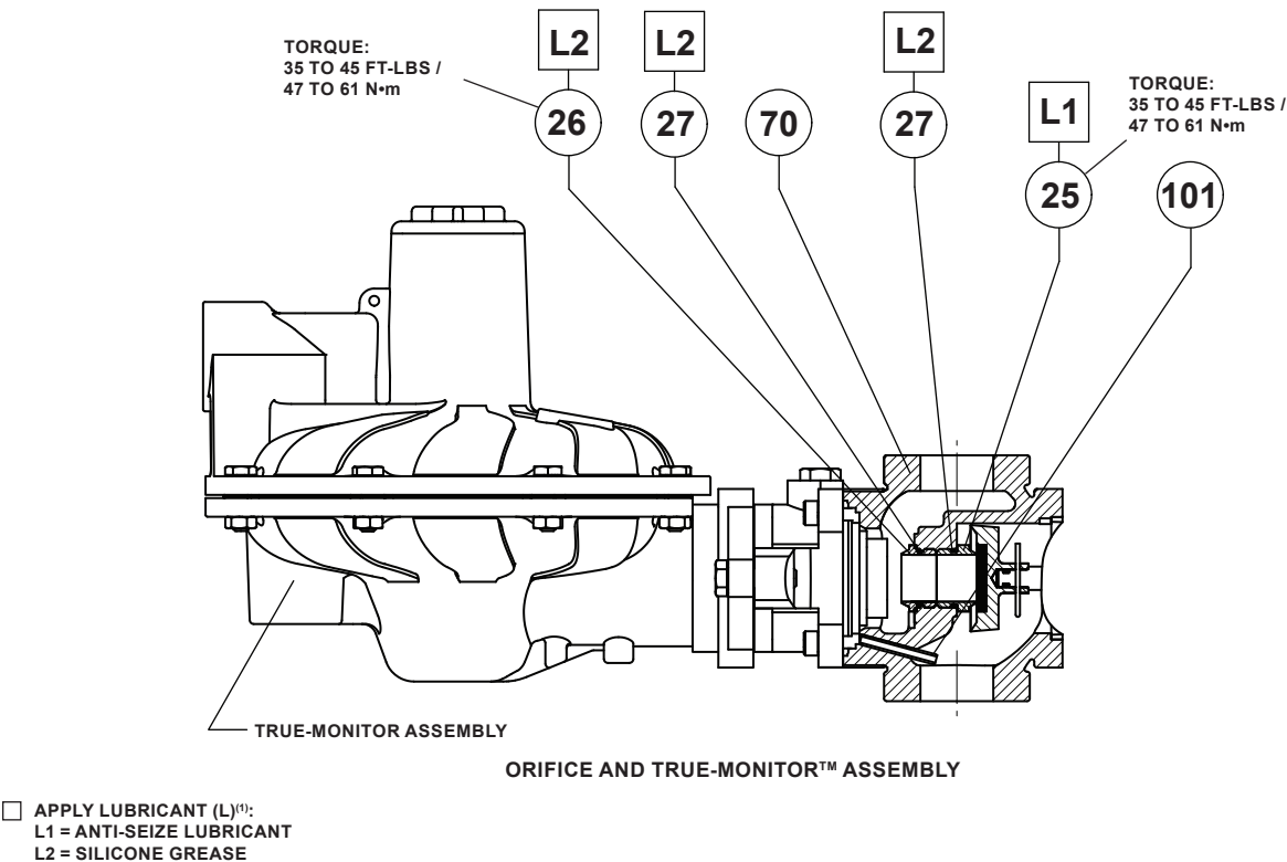
Figure 11. CS400 Series Slam shut and Integral Monitor Modules
