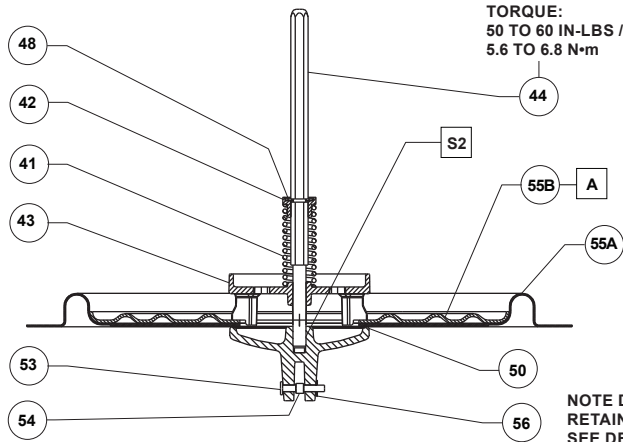
TYPE CS800/CS820 STANDARD/HIGH CAPACITY RELIEF
