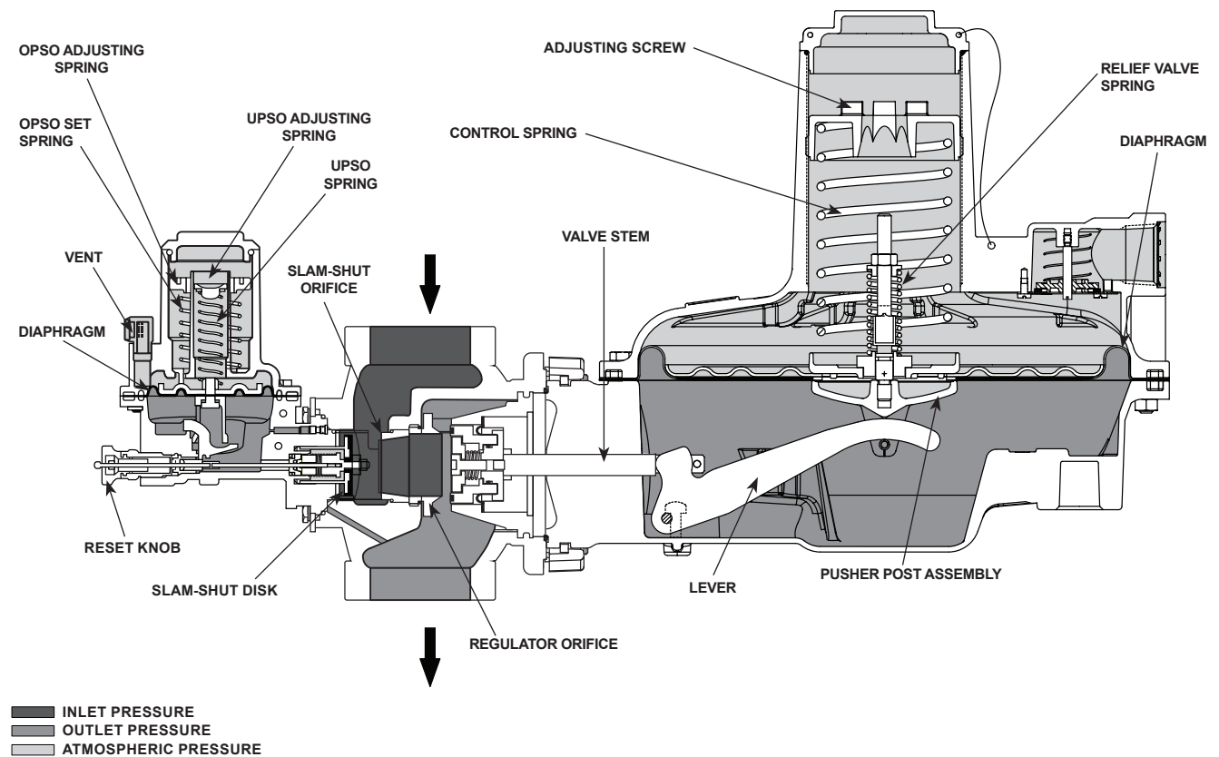
Figure 5. Type CS804IT Internally Registered Regulator with Slam-shut Module Operational Schematic
