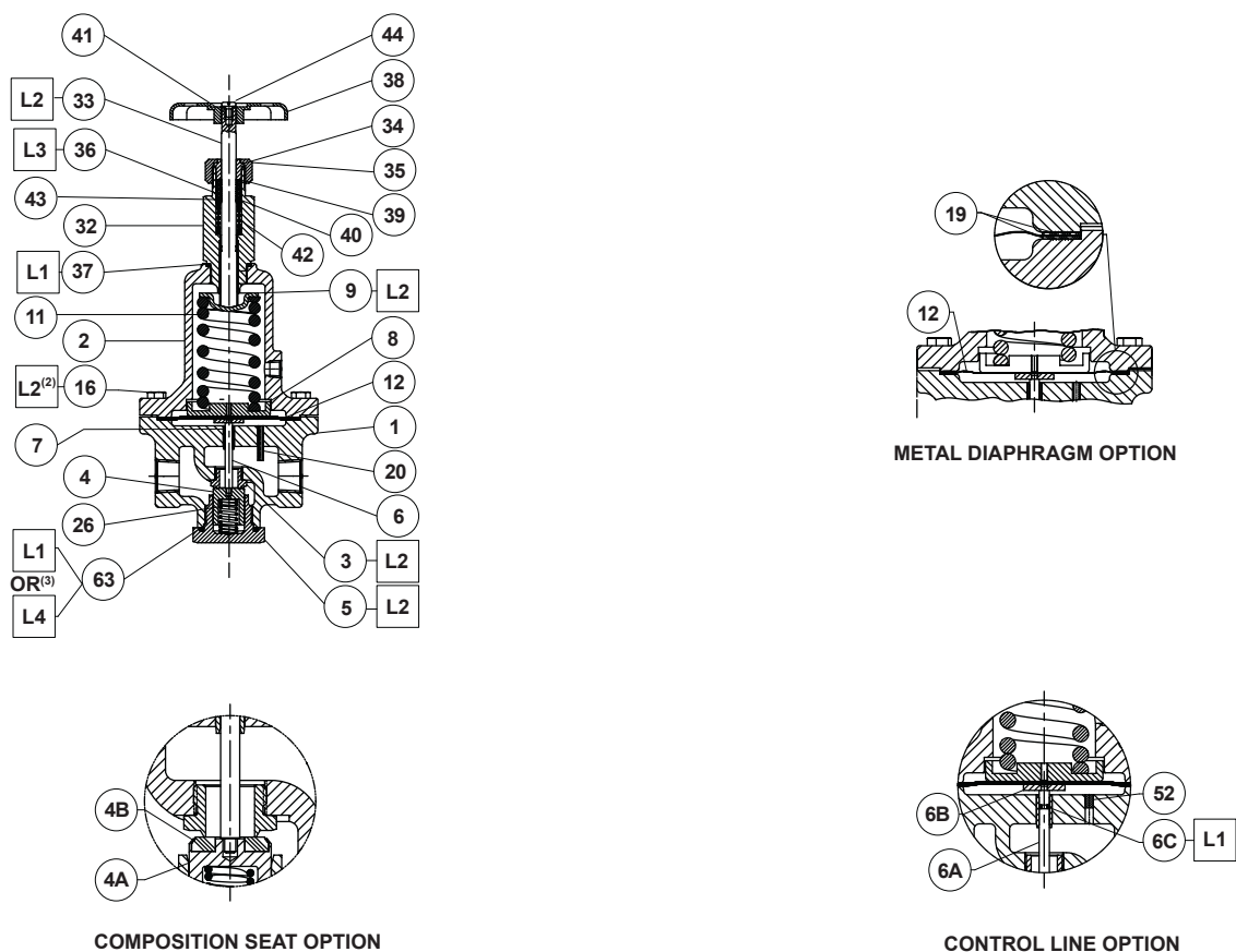
GF04918 APPLY LUBRICANT (1) : L1 = GENERAL PURPOSE PTFE OR LITHIUM GREASE L2 = ANTI-SEIZE COMPOUND L4 = GRAPHITE SEALANT 1. Lubricants and sealants must be selected such that they meet the temperature requirements. 2. Apply L2 (anti-seize compound) on key 16 for Stainless steel bolts. 3. Apply L4 (graphite sealant) instead of L1 (general purpose PTFE or lithium grease) on key 63 for graphite ring.
