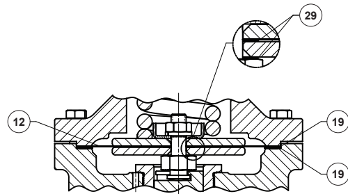
METAL DIAPHRAGM OPTION
