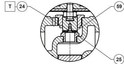
COMPOSITE SEAT OPTION
