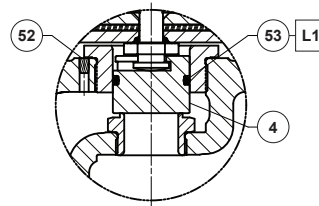
CONTROL LINE OPTION
