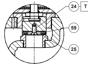
COMPOSITE SEAT OPTION
