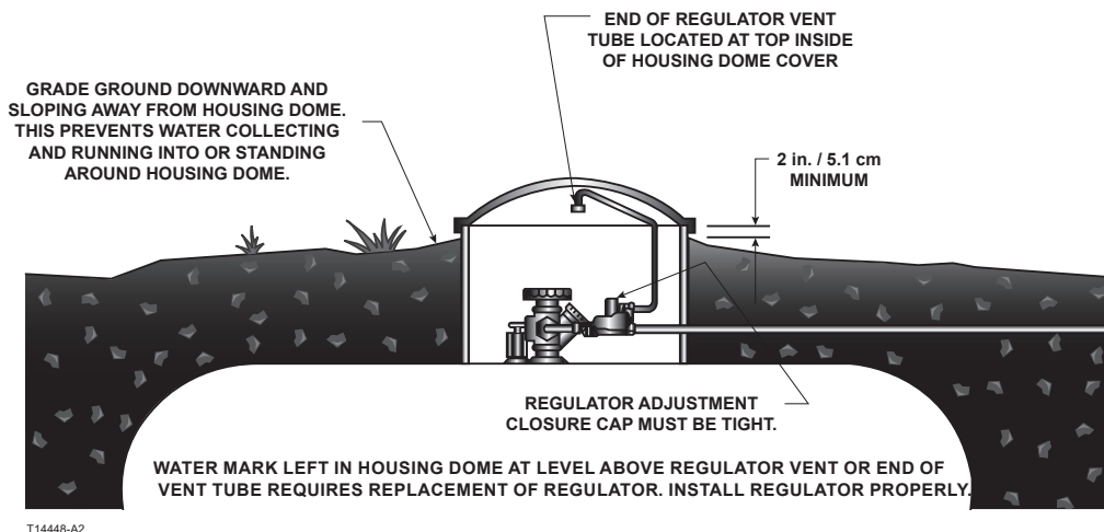
Figure 5. Underground Installation
