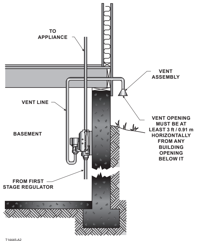
Figure 4. Basement Installation
