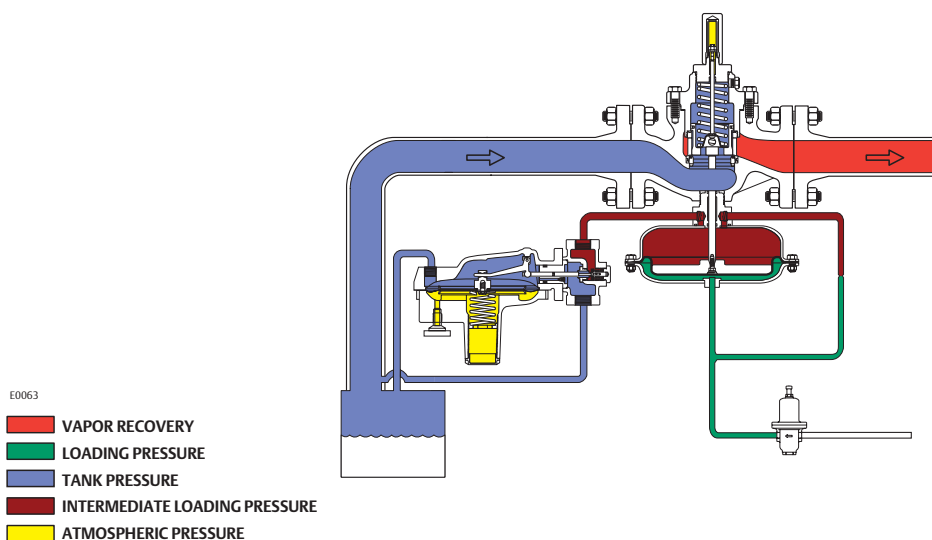
Figure 2. Operational Schematic
