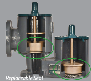
Replaceable Seat
