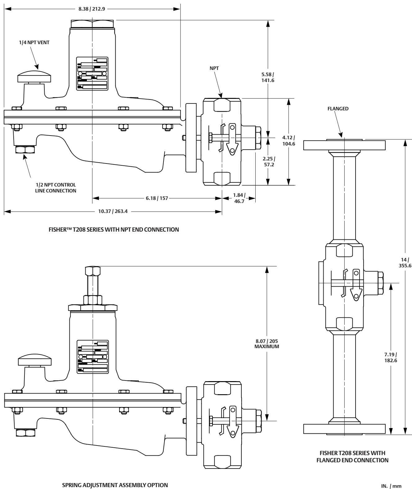
Figure 4. Dimensions
