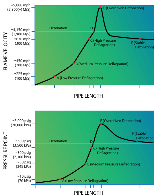
Figure 10. Conceptual graphs showing flame velocity and pressure of a flame front at points along a long pipe, beginning with ignition at a closed end. All scales are logarithmic.
