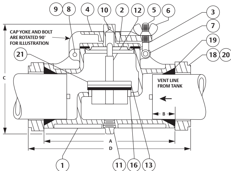
Figure 2. Enardo™ 800-PSO In-Line Vent Valve Dimensions
