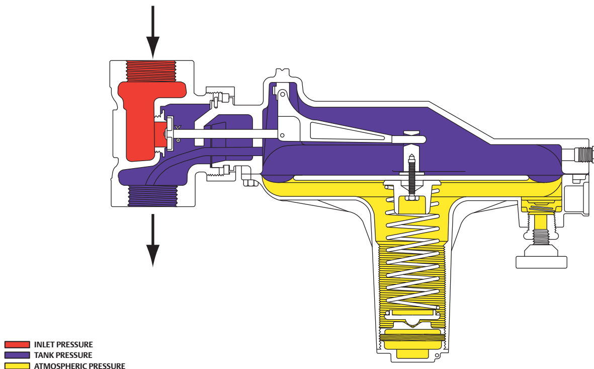
Figure 2. Operational Schematic
