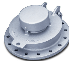
Figure 1. Enardo A
