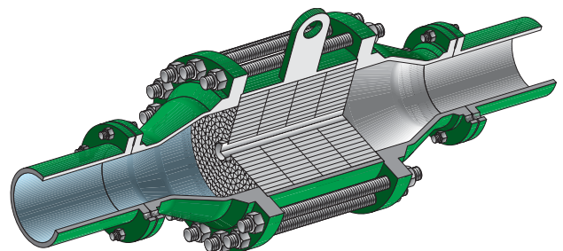
Figure 5. A typical In-line Flame Arrester.
