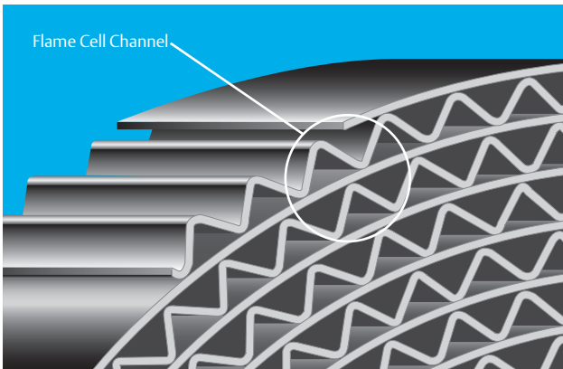
Figure 2. Concept of flame arrester element, featuring a crimped wound metal ribbon element
