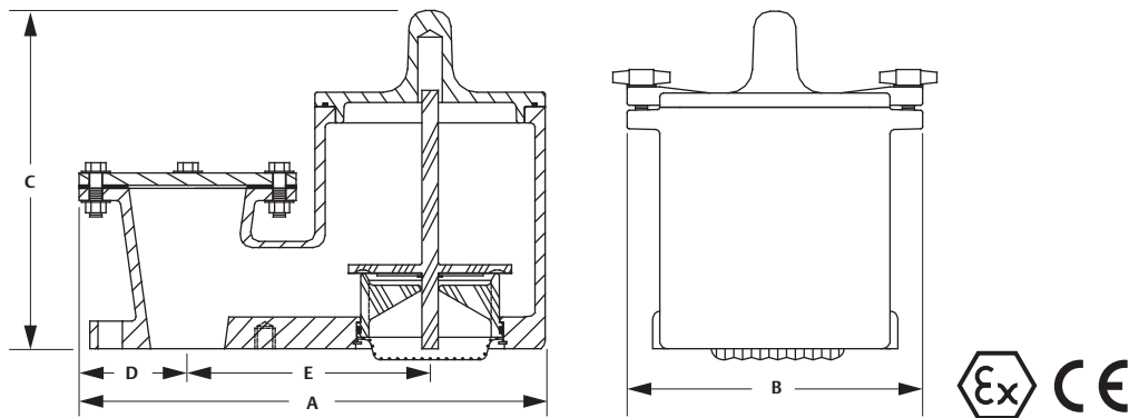
Figure 2. Enardo™ 952 Dimensions
