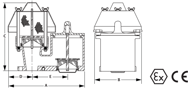
Figure 2. Enardo™ 950 Dimensions
