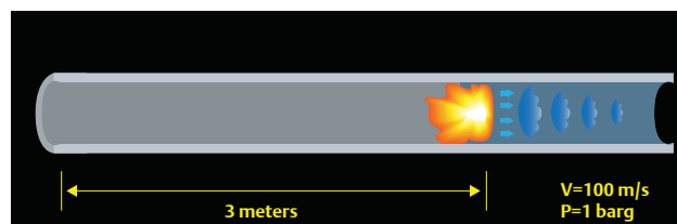
Figure 11. Concept of low-pressure deflagration confined in a pipe, showing typical distance from ignition point.
