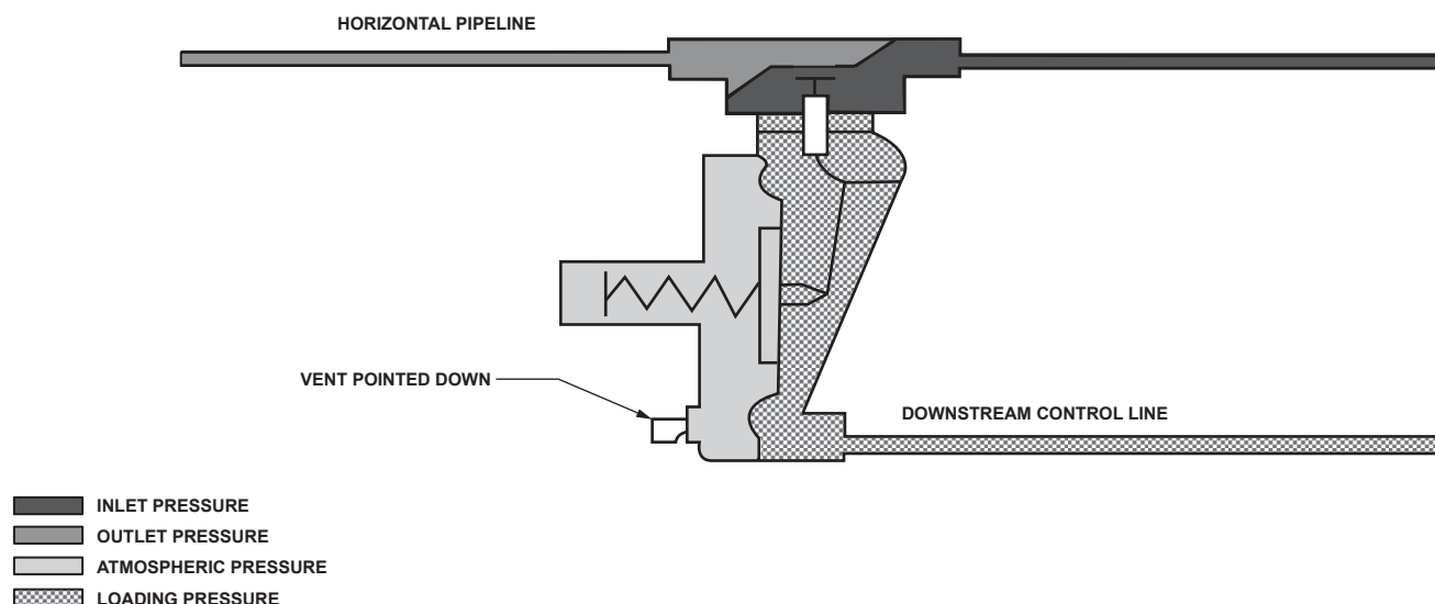
Figure 3. Type T205B Actuator Casing Drainage
