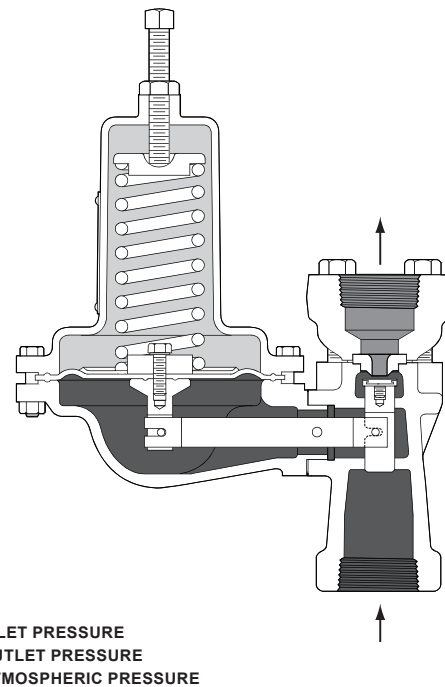
Figure 3. Type 630R Relief Valve Operational Schematic
