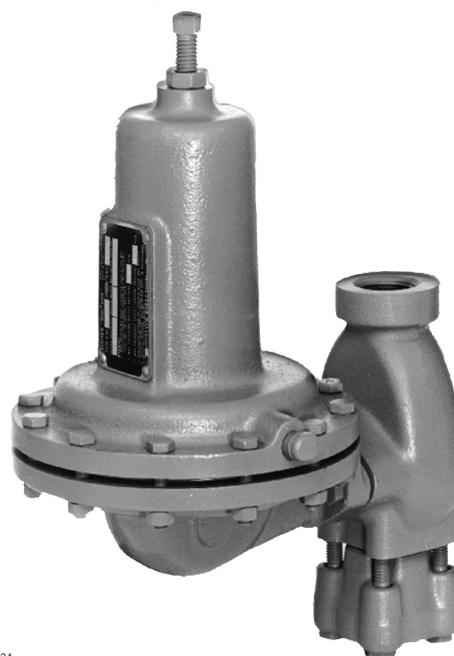
Figure 1. Spring-Loaded Type 630 Regulator
