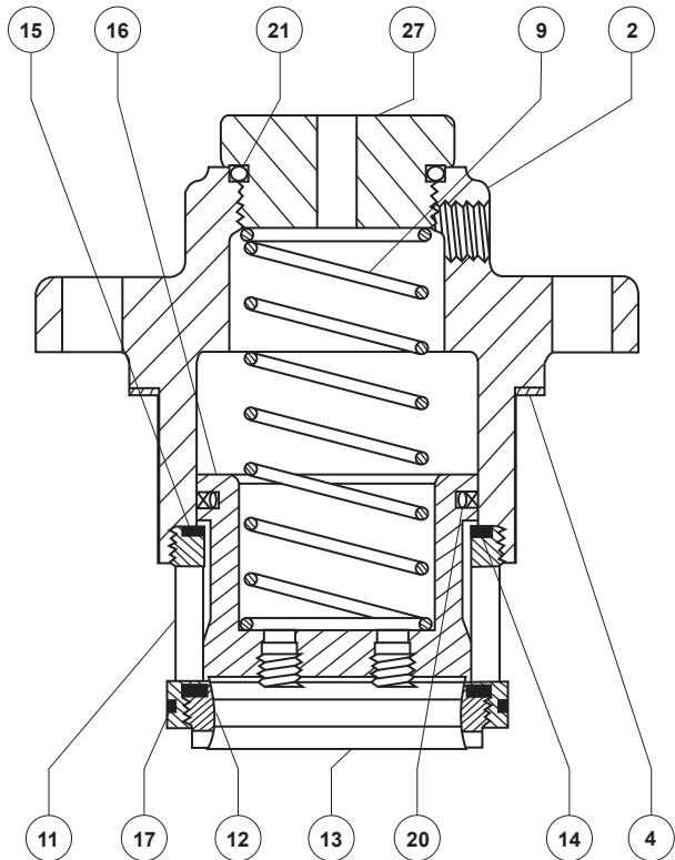
Figure 4. Type 63EG Main Valve
