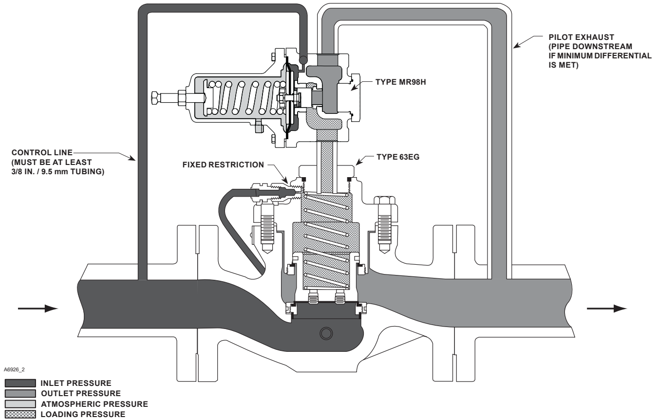
Figure 2. Operational Schematic
