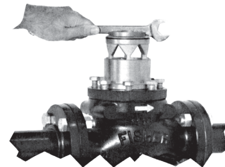
REPLACING TRIM PARTS ON SITE USING BODY AS HOLDING FIXTURE
