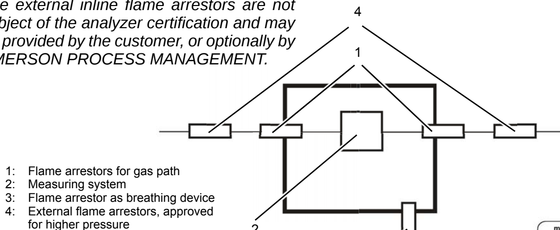
Fig. 2-8: Exemplary diagram for a single channel instrument for high gas pressure
