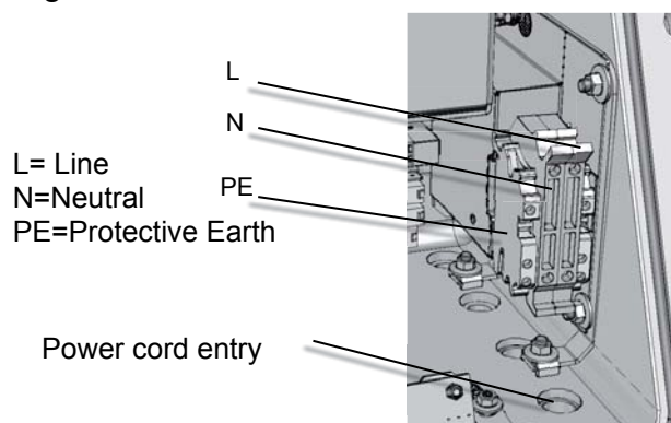
Fig. 2-15: Power terminals
