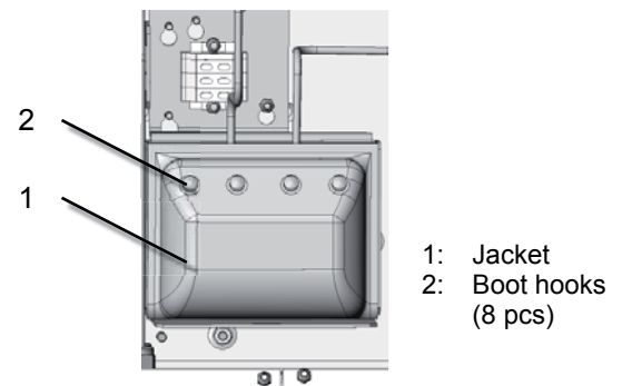
Fig. 4-10: Heated jacket
