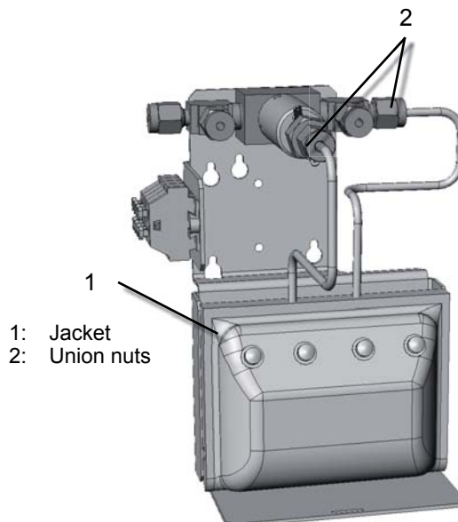
Fig. 4-6: Heated jacket
