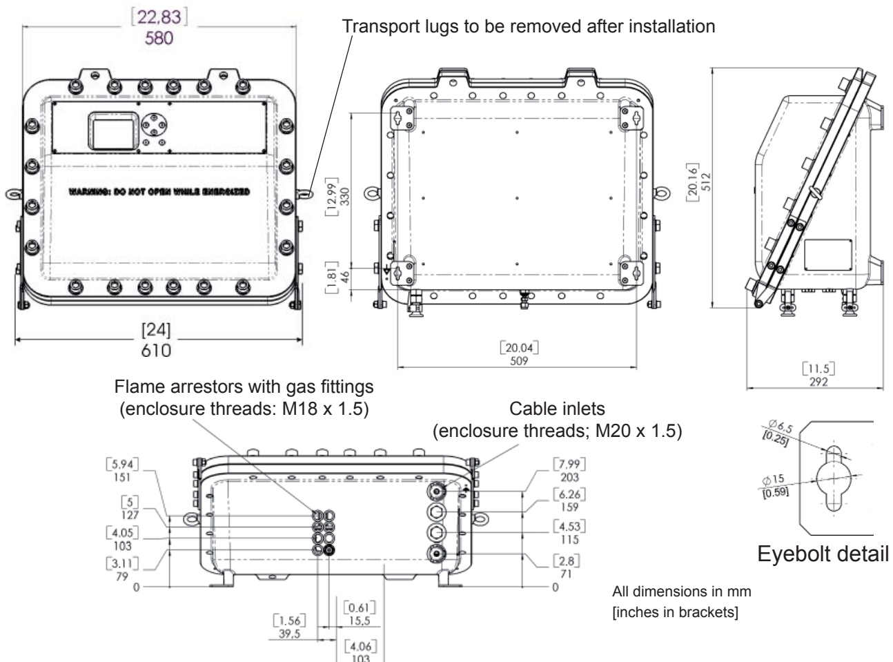
Fig. 2-2: Dimensions
