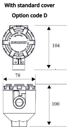
Figure 11: Connection Head Dimensional Drawing
