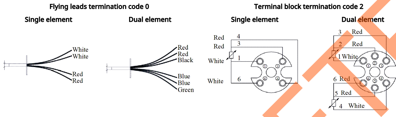
Figure 4: Rosemount 1067 RTD Lead Wire Configuration
