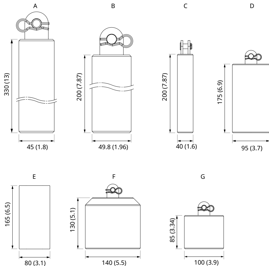
Figure 14: Standard Weights
