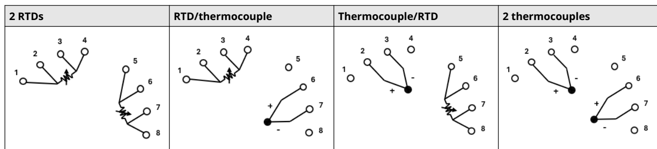
Figure 7: Dual sensor wiring diagram
