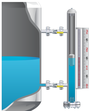
Figure 2.10.1 Illustration showing a magnetic level indicator
