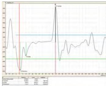
Figure 2: Echo plots shows a strong, reliable surface signal during all process conditions
