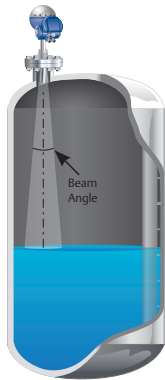
Figure 6.6.3: Beam width angle for the Rosemount 5600
