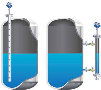
Figure 5.11.1: Example of a bypass chamber mount (right) and a stilling well mount (left).
