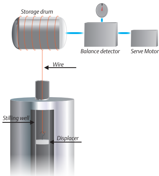
Figure 2.12.1 Illustration showing the servo powered level gauge
