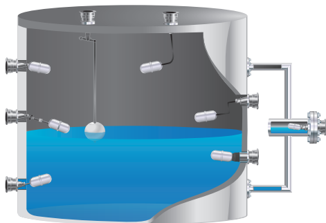
Figure 9.2.1: Float switch installation
