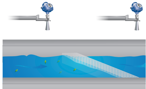
Figure 4.16.1: Non-contacting radar mounted over water flow with intake water screens.
