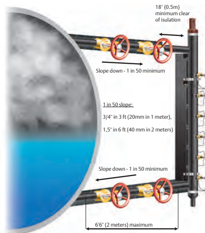
Figure 10.1.3: For optimum performance, process connections must be inclined
