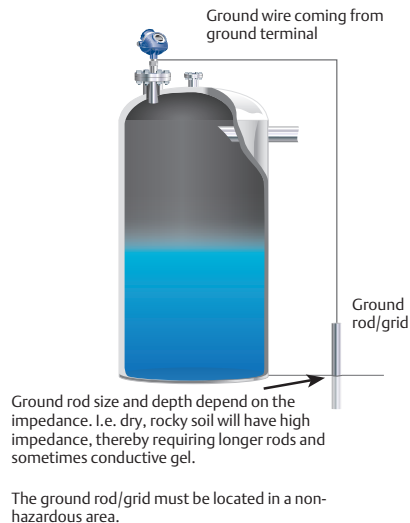
Figure 12.5.4: External ground connection
