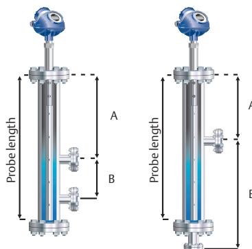
Figure 5.12.4: Side to side and side to bottom chambers for DVC probes.
