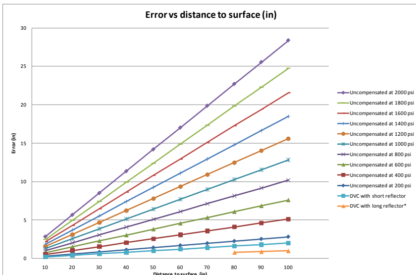
Figure 12.1.8: Error vs distance to surface
