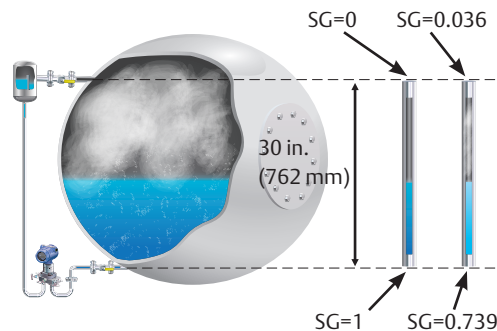
Figure 12.1.6: Density changes in a wet leg DP installation
