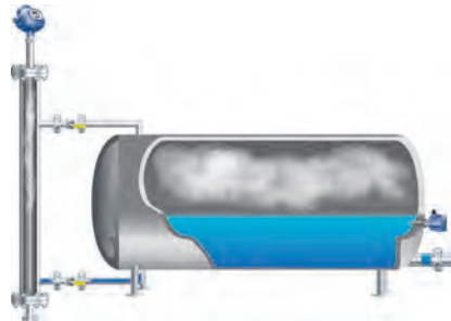
Figure 4.11.1: Gland steam condenser level with guided wave radar and vibrating fork switch
