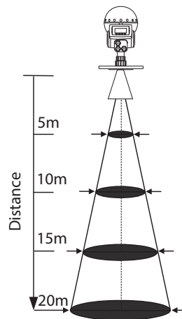
Figure 6.6.4: Beam width distance for the Rosemount 5600
