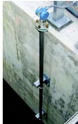
Guided Wave Radar Installed
