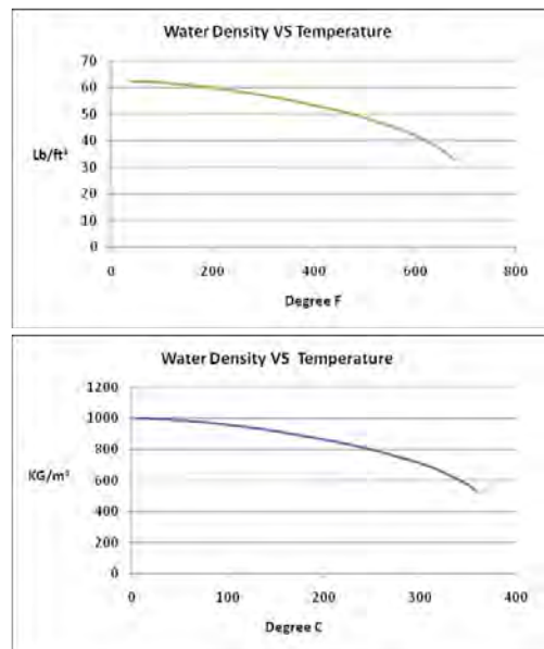
Figure 12.1.2: Water density depending on temperature, in English and Metric units
