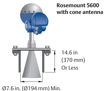
Figure 6.13.2: Tank connection, non-contacting radar for measuring solids
