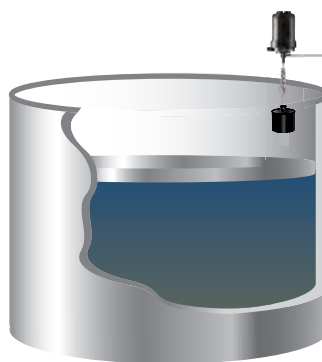
Figure 9.2.2: Floating roof tank alarm switch installation
