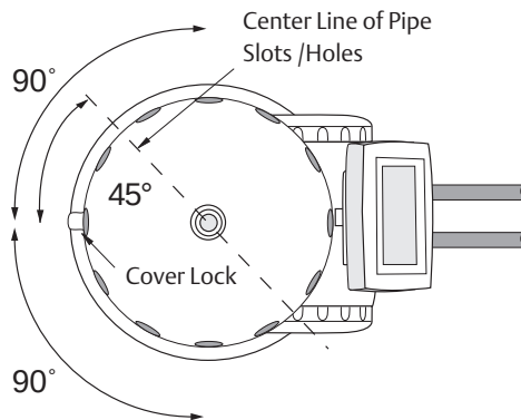
Figure 6.10.5: Orientation of the 5600 head
