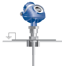
Figure 5.16.5: Installation with metal sheet in non-metallic vessels
