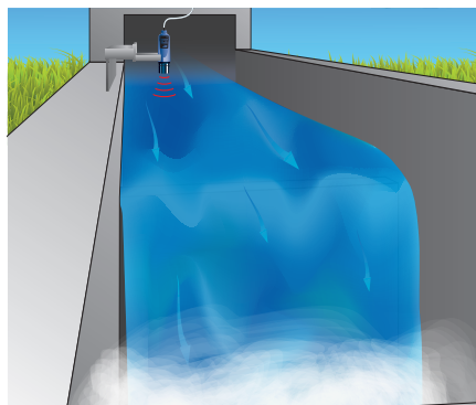
Figure 8.1.4: Measuring open channel flow with a 3108 ultrasonic transmitter
