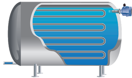
Figure 4.20.1: Closed cooling water tanks with vibrating fork switch to ensure adequate water level
