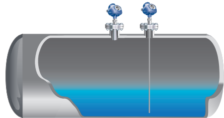
Figure 4.44.1: Water wash tank level with non-contacting or guided wave radar
