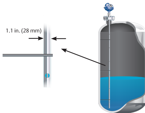
Figure 5.13.3: Coaxial fixed to the tank wall
