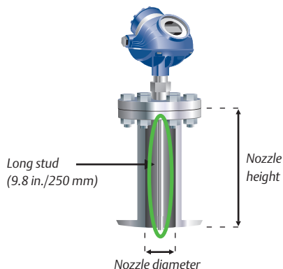
Figure 5.16.4: Recommended mounting position, nozzle
