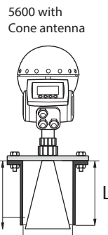
Figure 6.4.6: Nozzle requirements for Rosemount non-contacting radars
