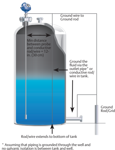
Figure 12.5.5: Non-metal tank with connection to ground
