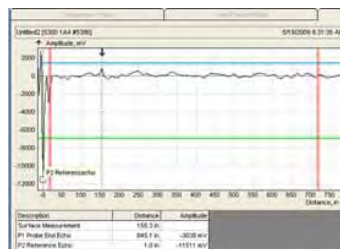
Figure 3. In cases of weak surface signal, Probe End Projection uses the probe length and the dielectric of the material to determine the product surface.
