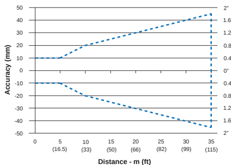
Figure 6.10.6: Performance and measuring range
