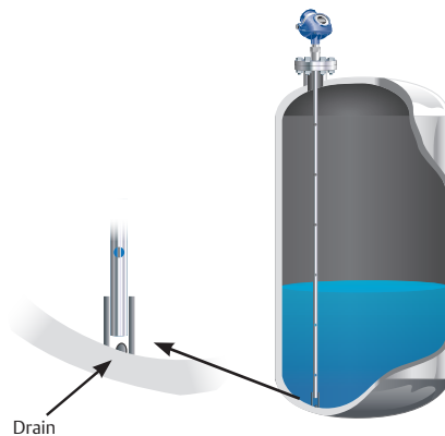
Figure 5.13.4: Coaxial with a welded tube at tank bottom
