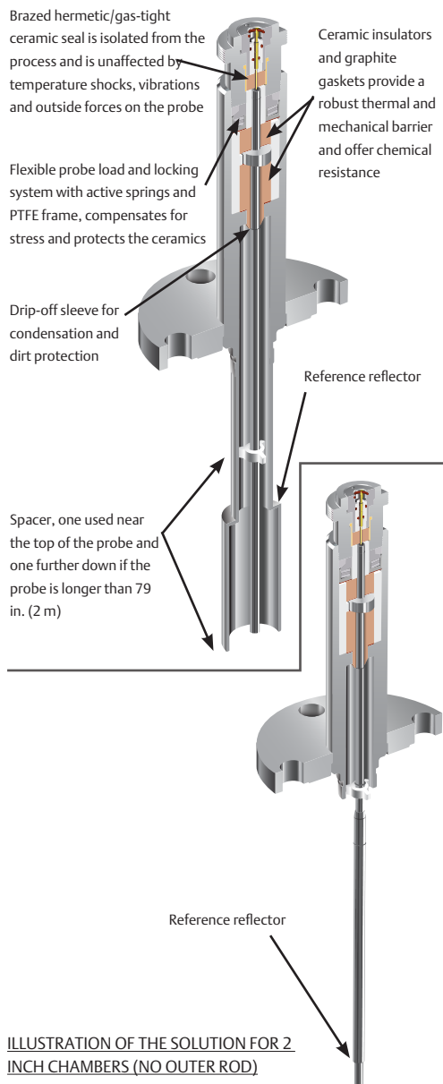
Figure 5.18.4: HTHP seal
