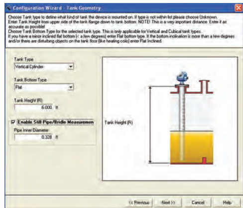
Figure 5.11.12: Transmitter configuration wizard
