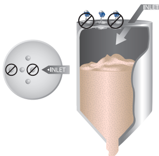
Figure 6.13.3: Radar location, non-contacting radar for measuring solids
