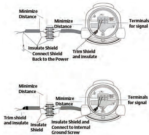
Figure 12.5.2: Possible field connections of Rosemount 3300, 5400, or 5300 series level transmitters
