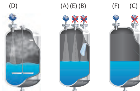
Figure 6.3.1: It is important to consider the proper mounting location
