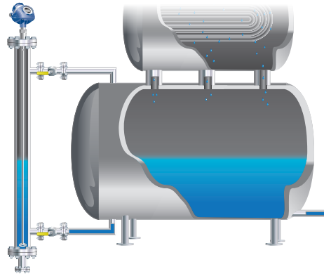
Figure 4.10.1: Deaerator level with guided wave radar
