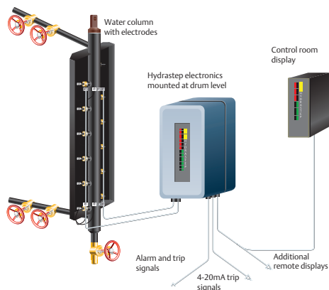
Figure 10.1.2: Typical Hydrastep installation
