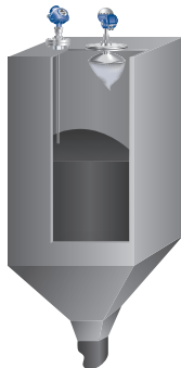
Figure 4.33.1: Ash hopper or fly ash with guided wave radar or non-contacting
