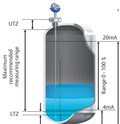
Figure 5.2.1: Illustration showing how the measuring range is related to the transition zones
