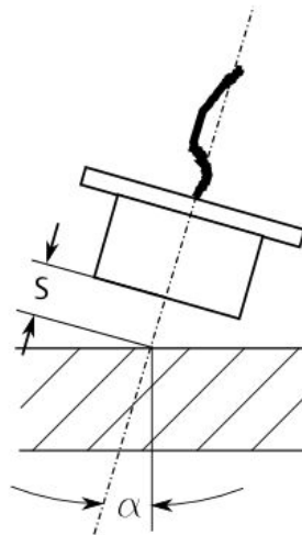
Figure 4-4: Maximum axial tilting if using PR 6426
