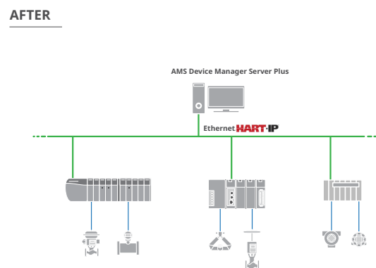
Figure 2. Implementation using HART-IP Interface
