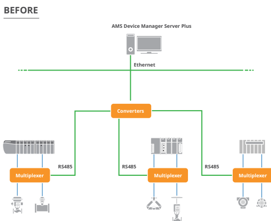
Figure 1. Traditional implementation using multiplexers
