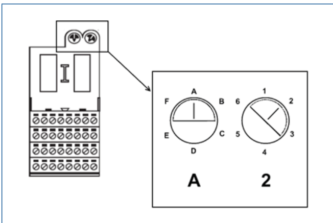
Terminal Block Keying Example.
