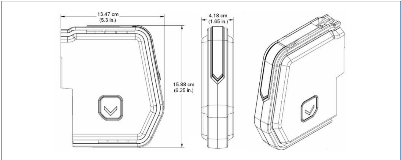
S-series Profibus DP card dimensions.
