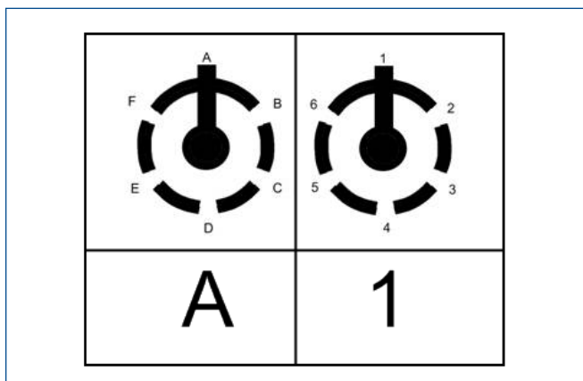
Keying Position for HART AI, 4-20 mA, 8-channel.
