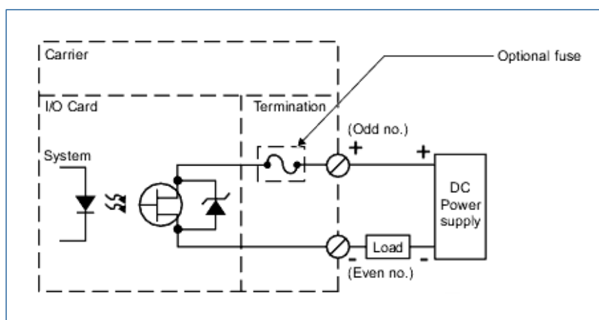
Simplified Circuit and Connection Diagram for DO Card, 8-channel, 24V DC, Isolated.
