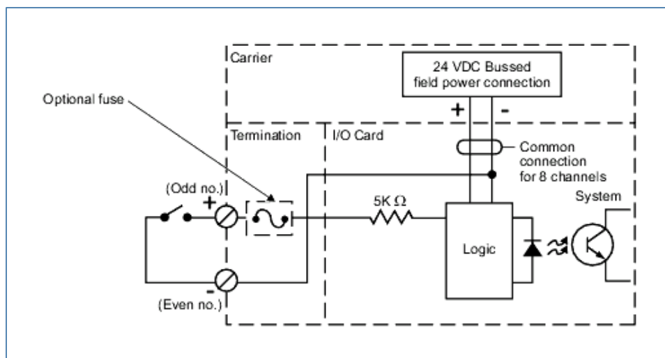
Simplified Circuit and Connection Diagram for DI Card, 8-channel, 24V DC, Dry Contact.
