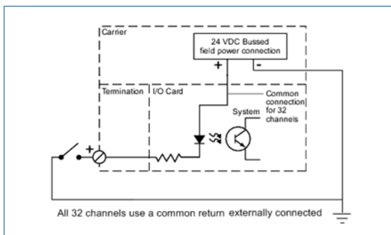
Simplified Circuit and Connection Diagram for DI Card, 32-channel, 24V DC, Dry Contact.
