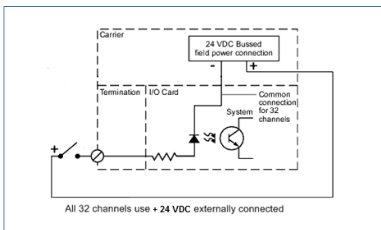
Simplified Circuit and Connection Diagram for Simplex DI Plus Card, 32-channel, 24V DC, Dry Contact.
