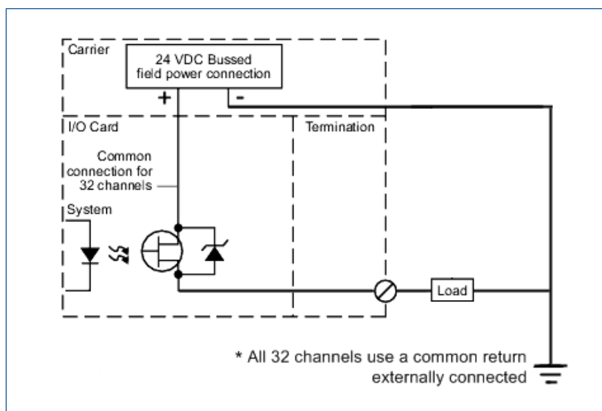
Simplified Circuit and Connection Diagram for Simplex DO (Plus) Card, 32-channel, 24V DC, High-Side.
