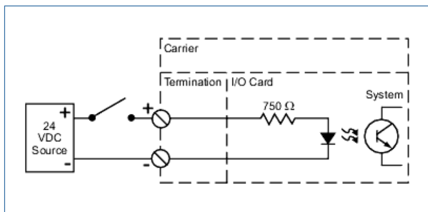
Simplified Circuit and Connection Diagram for PCI Card, 4 Channel, 24V DC, Isolated.
