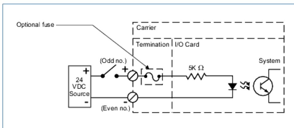
Simplified Circuit and Connection Diagram for DI Card, 8-channel, 24V DC, Isolated.
