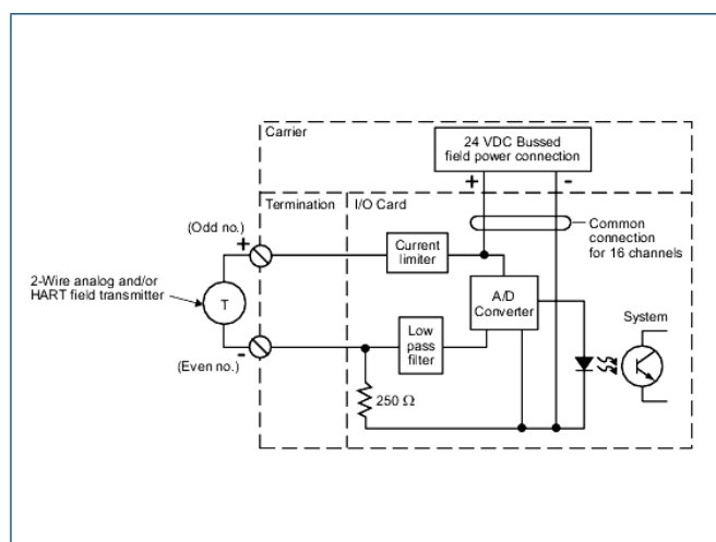
Simplified Circuit and Connection Diagram for Simplex AI Card, 16-channel, 4 to 20 mA, HART.
