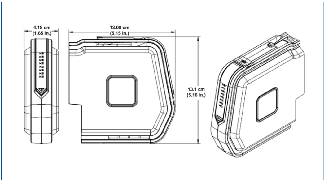
S-series Traditional I/O Interface Enclosure.
