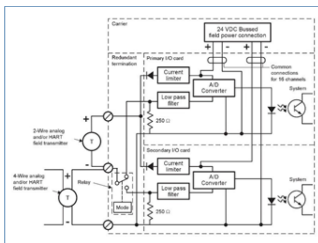
Simplified Circuit and Connection Diagram for Redundant AI Plus Card, 16-channel, 4 to 20 mA, HART.
