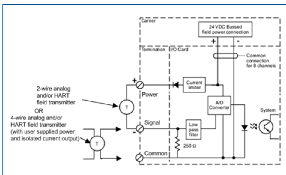
Simplified Circuit and Connection Diagram for AI Card, 8-channel, 4 to 20 mA, HART.
