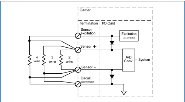
Simplified Circuit Diagram for RTD Input Card, 8 Channels.
