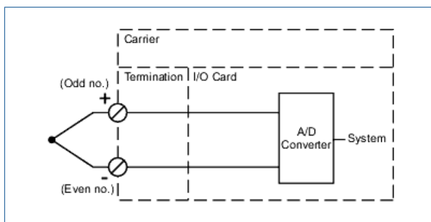
Simplified Circuit Diagram of Thermocouple/mV Card, 8 Channels.
