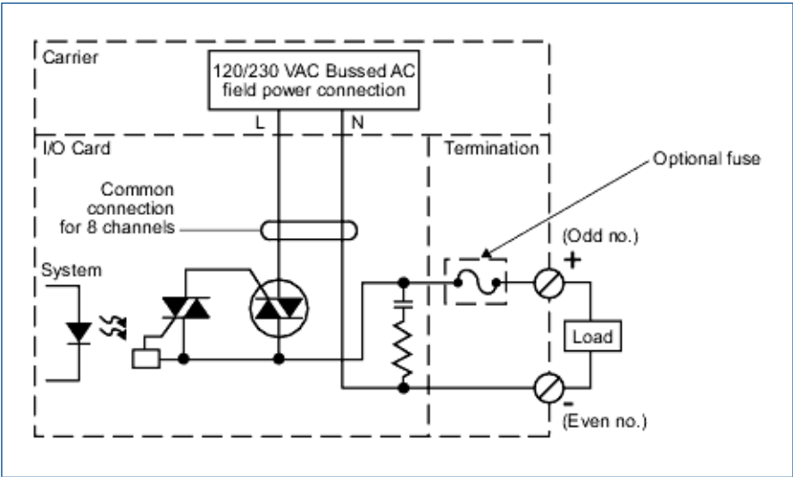
Simplified Circuit and Connection Diagram for DO Card, 8-channel, 120/230V AC, High Side.
