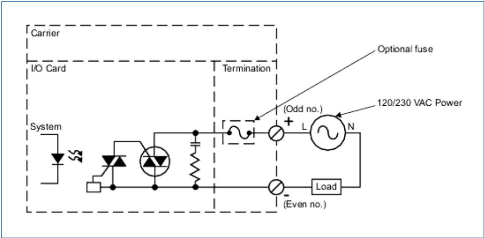
Simplified Circuit and Connection Diagram for DO Card, 8-channel, 120/230V AC, Isolated.
