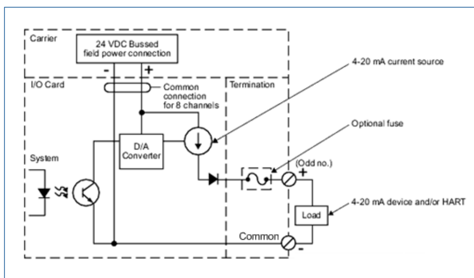
Simplified Circuit and Connection Diagram for Simplex AO Card, 8-channel, 4 to 20 mA, HART.
