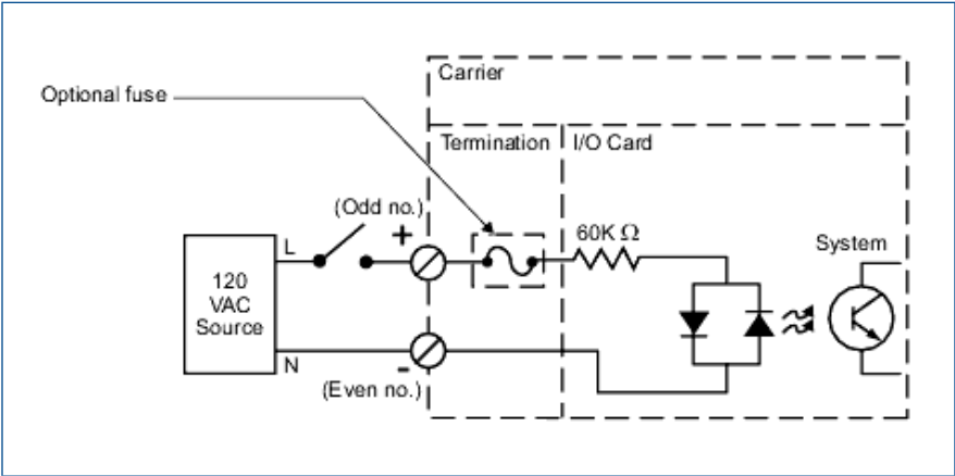
Simplified Circuit and Connection Diagram for DI Card, 8-channel, 120V AC, Isolated.
