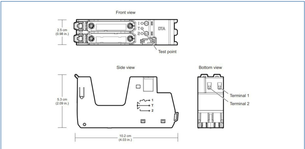
LS CHARM Redundant DTA Relay Terminal Block.
