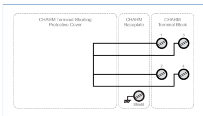
Simplified Circuit and Connection Diagram for CHARM Terminal-Shorting Protection Cover.
