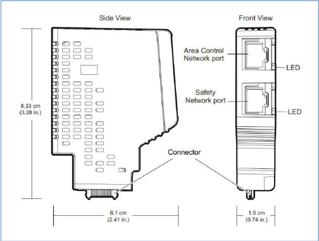
SZ Controller Ethernet Isolation Port or Keylock Ethernet Isolation Port.
