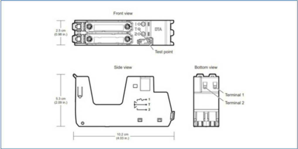
LS CHARM Redundant DTA Relay Terminal Block.
