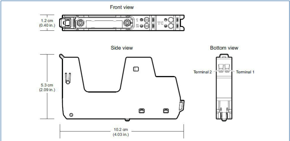
CHARM Thermocouple / mV Terminal Block.
