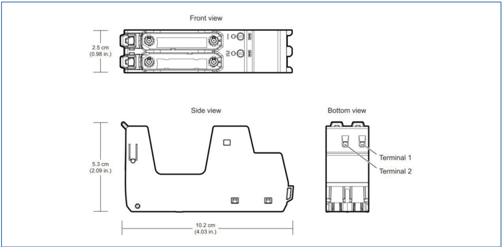
LS CHARM Redundant Terminal Block.
