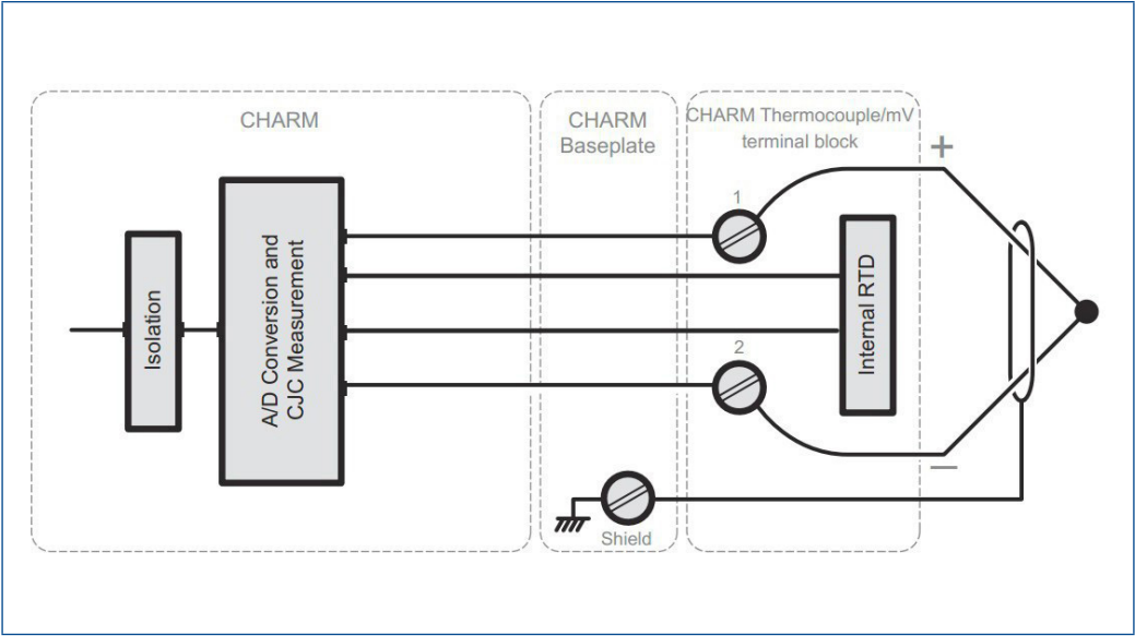
Simplified Circuit and Connection Diagram for LS Thermocouple/mV CHARM with Thermocouple/mV Terminal Block.
