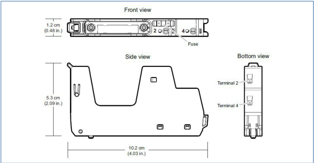
CHARM Fused Injected Power Terminal Block.
