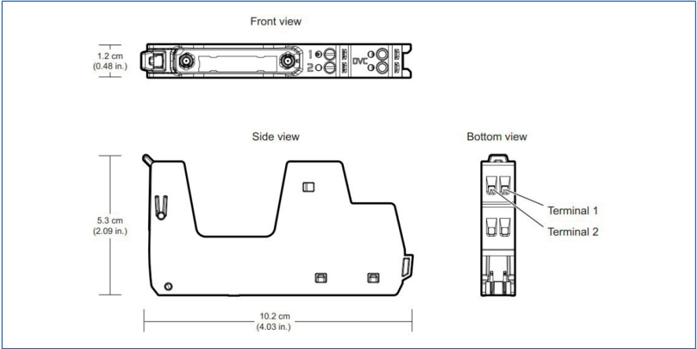
LS CHARM DVC Terminal Block.
