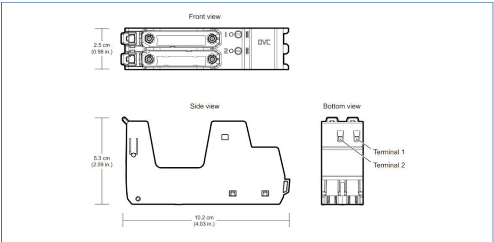
LS CHARM Redundant DVC Terminal Block.
