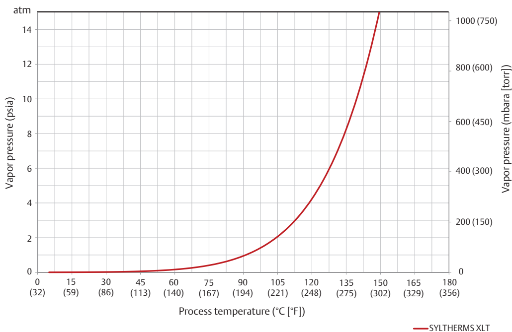
Figure 1-5. SYLTHERM XLT Vapor Pressure Curve
