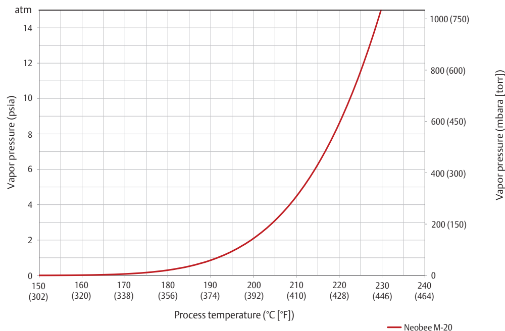
Figure 1-7. Neobee M-20 Vapor Pressure Curve
