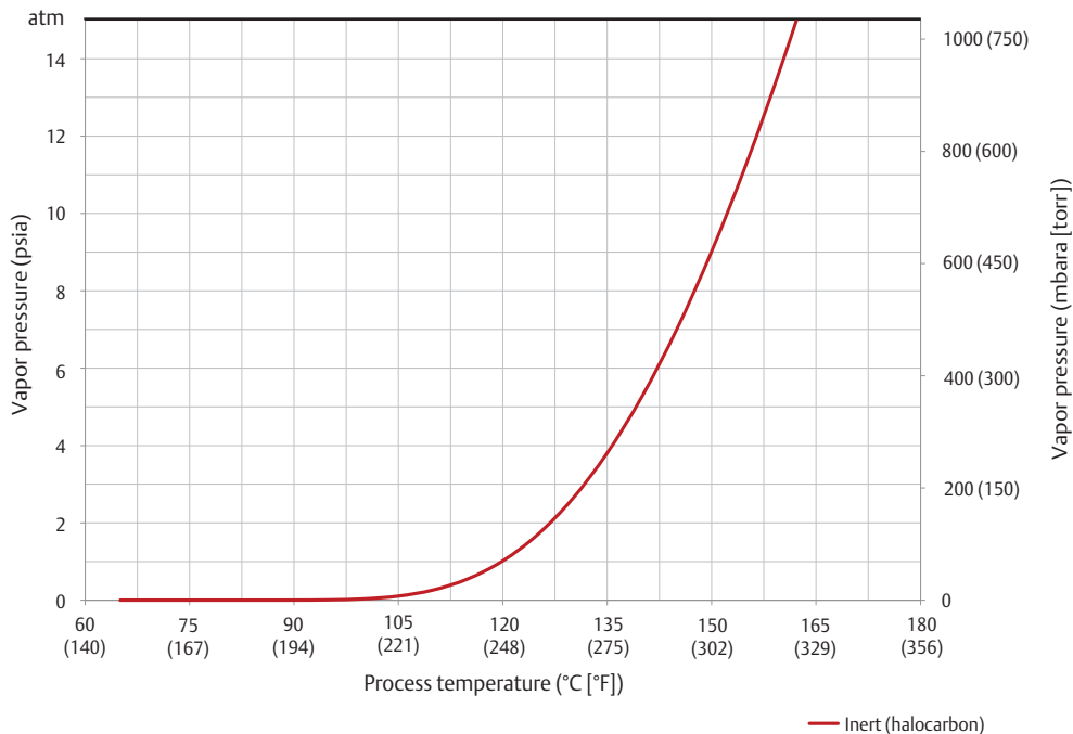
Figure 1-6. Inert (Halocarbon) Vapor Pressure Curve
