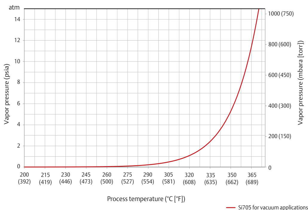
Figure 1-3. Silicone 705 for Vacuum Applications Vapor Pressure Curve
