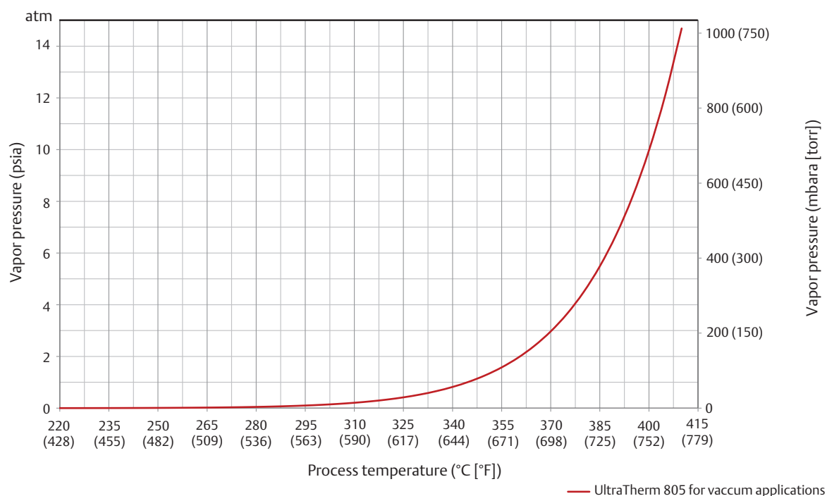
Figure 1-4 UltraTherm 805 for Vacuum Applications Vapor Pressure Curve
